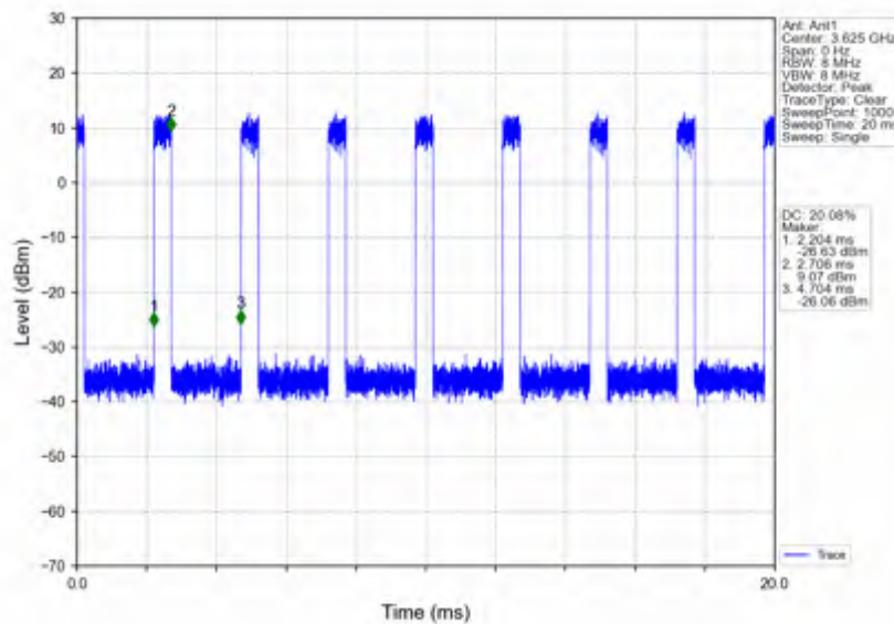
n78d_30kHz_SISO_NTNV_100MHz_CP-OFDM 64 QAM_3624.99MHz_Inner_Full
