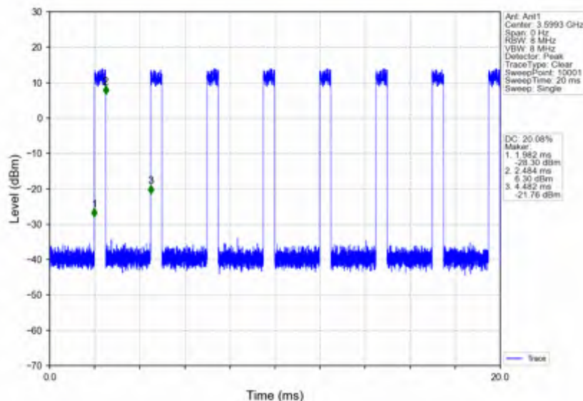
n78d_30kHz_SISO_NTNV_100MHz_DFT-s-OFDM QPSK_3600MHz_Inner_Full
