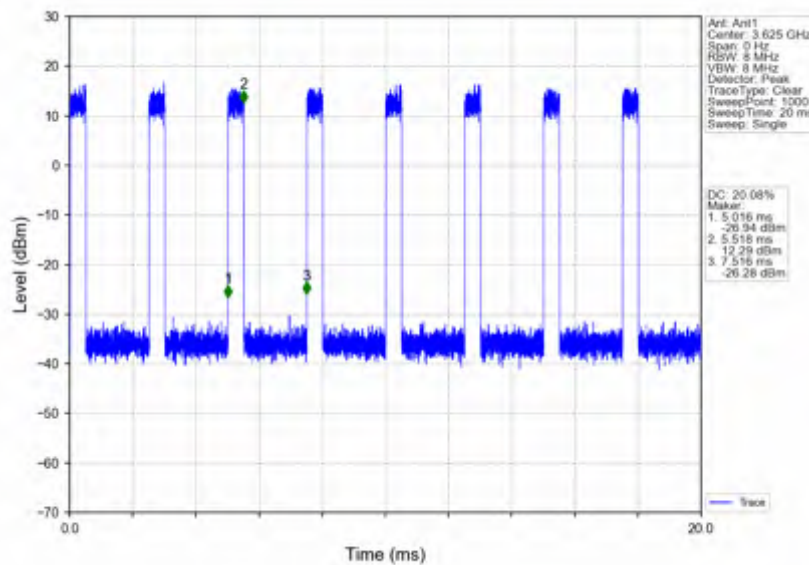
n78d_30kHz_SISO_NTNV_100MHz_CP-OFDM_16_QAM_3624.99MHz_Inner_Full
