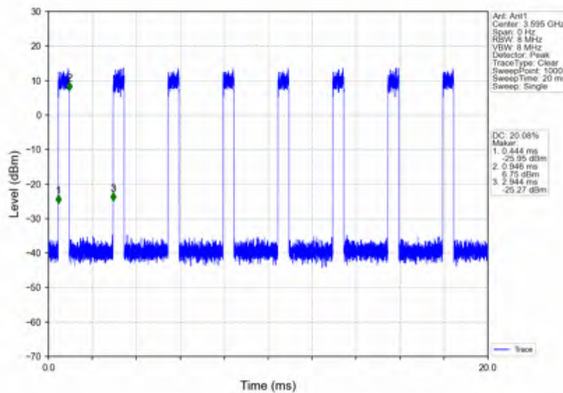
n78d_30kHz_SISO_NTNV_90MHz_CP-OFDM QPSK_3595.02MHz_Inner_Full
