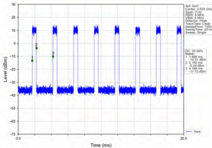
n78d_30kHz_SISO_NTNV_90MHz_CP-OFDM_256_QAM_3624.99MHz_Inner_Full
