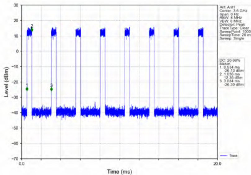
n78d_30kHz_SISO_NTNV_100MHz_CP-OFDM_QPSK_3600MHz_Inner_Full
