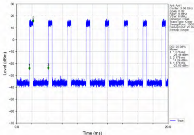
n78d_30kHz_SISO_NTNV_80MHz_CP-OFDM_256_QAM_3660MHz_Inner_Full
