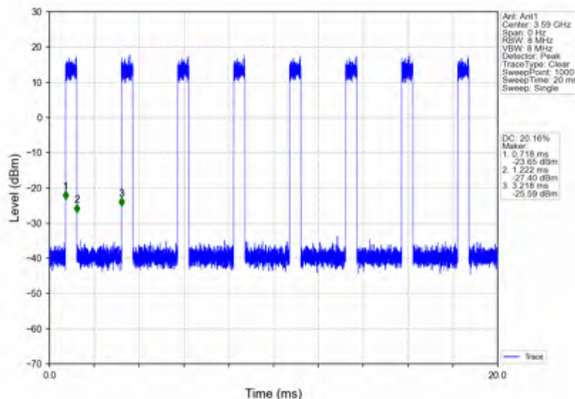
n78d_30kHz_SISO_NTNV_80MHz_CP-OFDM 64 QAM_3590.01MHz_Inner_Full
