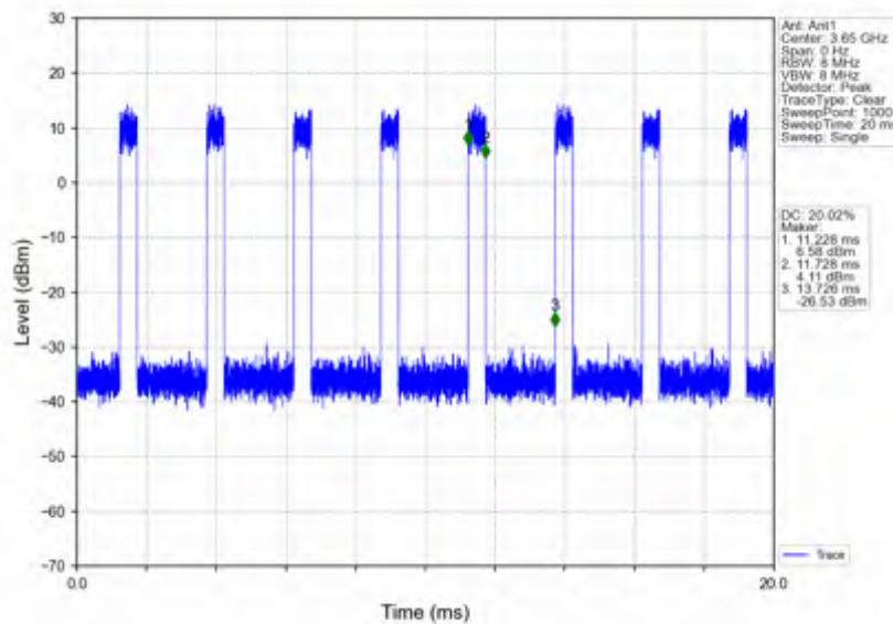
n78d_30kHz_SISO_NTNV_100MHz_CP-OFDM 64 QAM_3649.98MHz_Inner_Full
