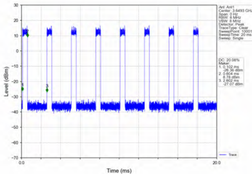
n78d_30kHz_SISO_NTNV_100MHz_DFT-s-OFDM 64 QAM_3649.98MHz_Inner_Full
