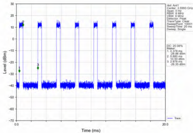
n78d_30kHz_SISO_NTNV_100MHz_DFT-s-OFDM 64 QAM_3600MHz_Inner_Full
