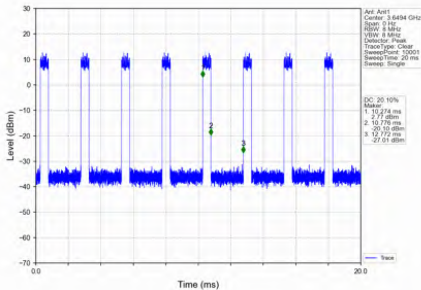
n78d_30kHz_SISO_NTNV_100MHz_DFT-s-OFDM QPSK_3649.98MHz_Inner_Full
