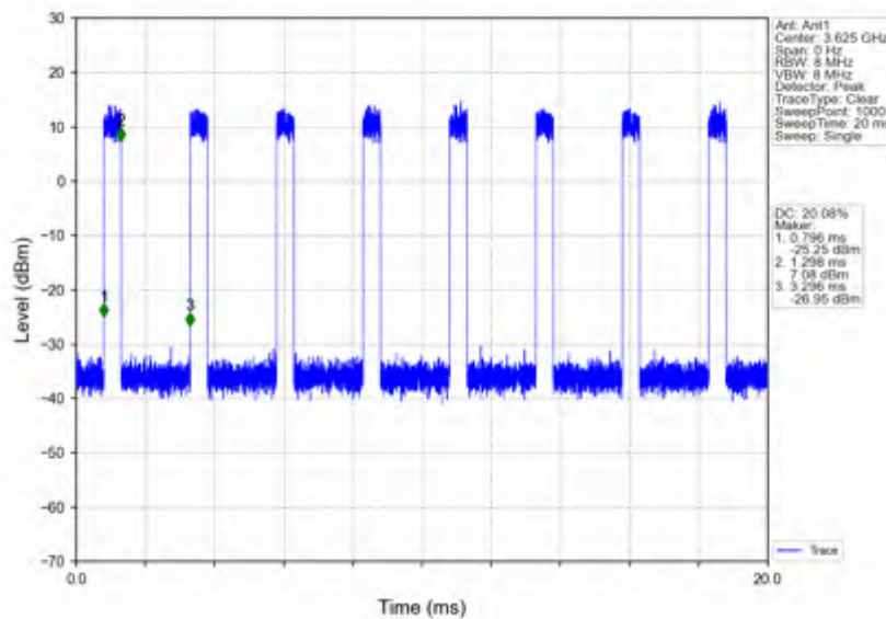
n78d_30kHz_SISO_NTNV_80MHz_CP-OFDM_256_QAM_3624.99MHz_Inner_Full
