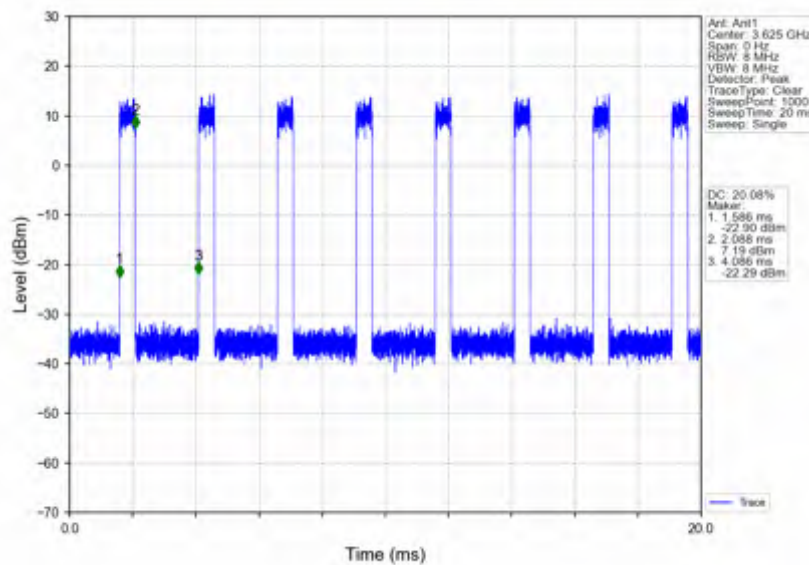
n78d_30kHz_SISO_NTNV_90MHz_CP-OFDM QPSK_3624.99MHz_Inner_Full
