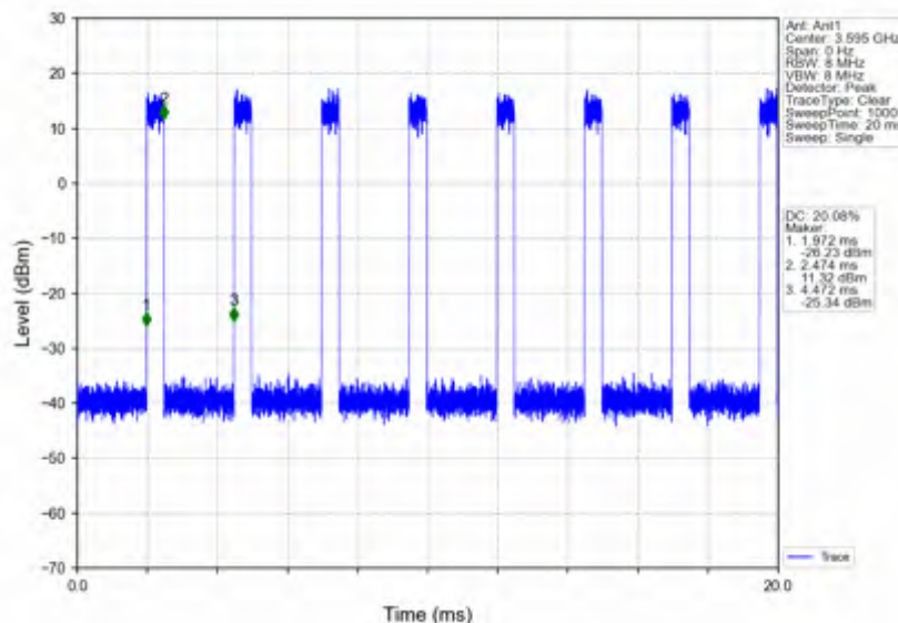
n78d_30kHz_SISO_NTNV_90MHz_CP-OFDM 64 QAM_3595.02MHz_Inner_Full
