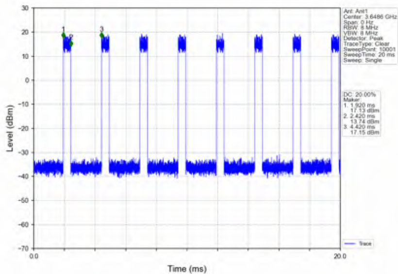
n78d_30kHz_SISO_NTNV_100MHz_DFT-s-OFDM_QPSK_3600MHz_Inner_1RB_Right
