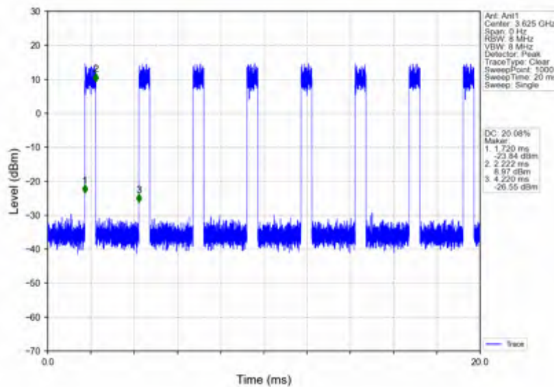
n78d_30kHz_SISO_NTNV_90MHz_CP-OFDM 16 QAM 3624.99MHz_Inner_Full
