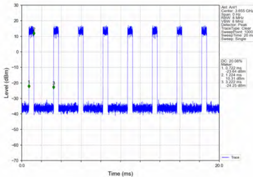
n78d_30kHz_SISO_NTNV_90MHz_CP-OFDM 64 QAM_3654.99MHz_Inner_Full
