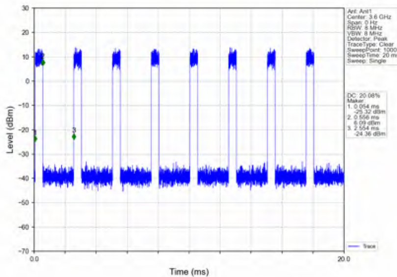
n78d_30kHz_SISO_NTNV_100MHz_CP-OFDM 64 QAM_3600MHz_Inner_Full
