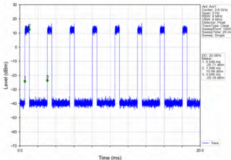
n78d_30kHz_SISO_NTNV_100MHz_CP-OFDM_16_QAM_3600MHz_Inner_Full
