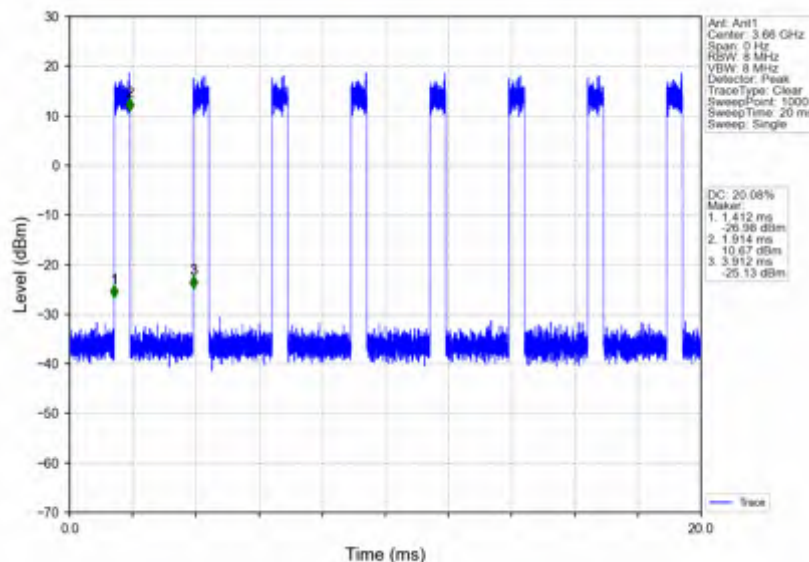
n78d_30kHz_SISO_NTNV_80MHz_CP-OFDM 64 QAM_3660MHz_Inner_Full
