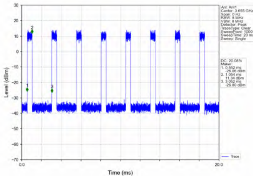
n78d 30kHz SISO NTNV 90MHz CP-OFDM 256 QAM 3654.99MHz Inner Full
