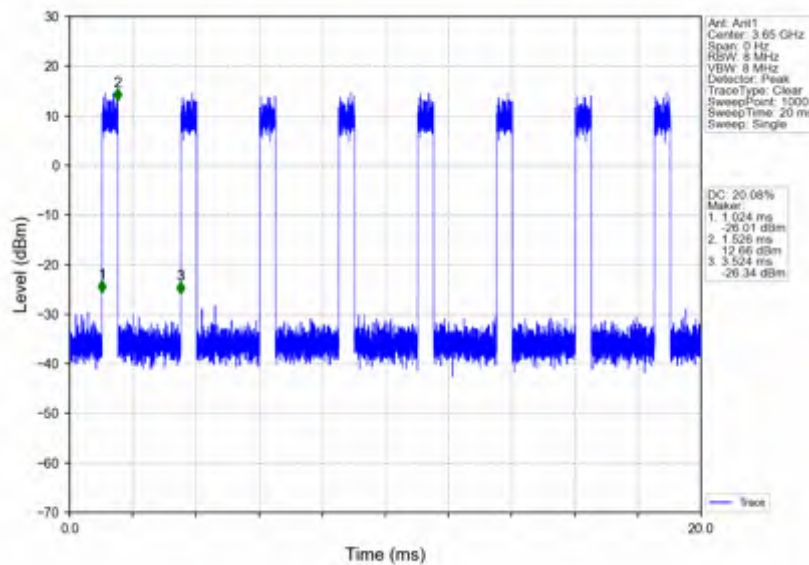
n78d_30kHz_SISO_NTNV_100MHz_CP-OFDM_16_QAM_3649.98MHz_Inner_Full
