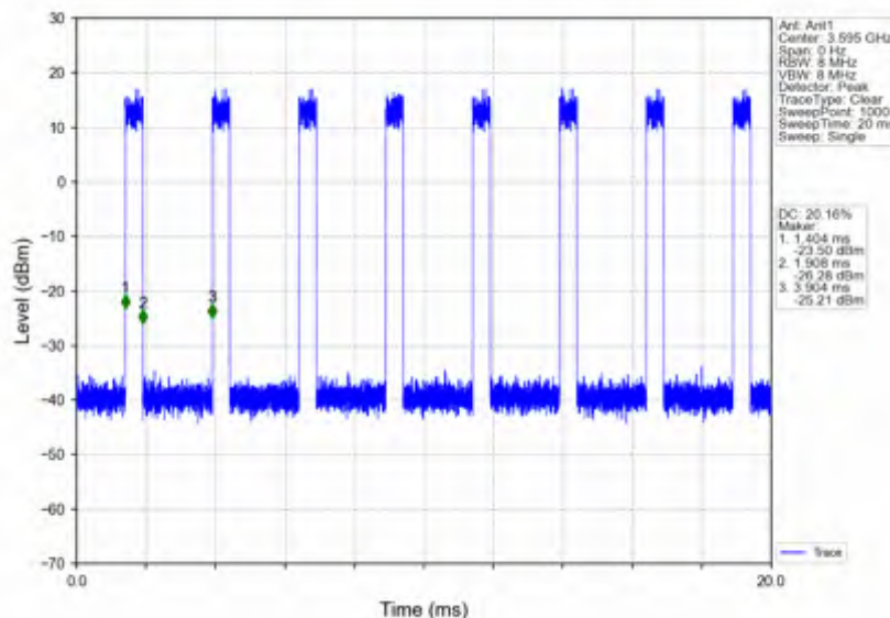
n78d_30kHz_SISO_NTNV_90MHz_CP-OFDM 16 QAM 3595.02MHz_Inner_Full
