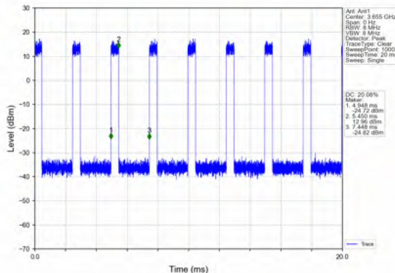
n78d_30kHz_SISO_NTNV_90MHz_CP-OFDM QPSK_3654.99MHz_Inner_Full
