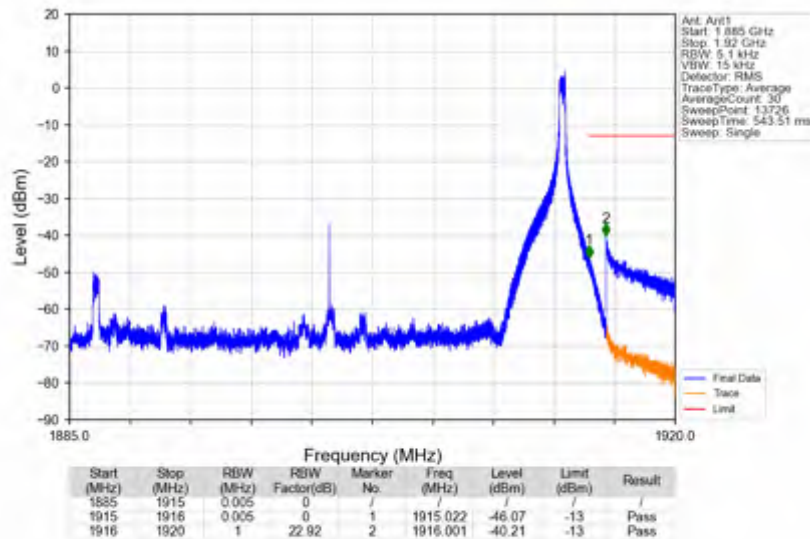
n25_30kHz_SISO_NTNV_30MHz_DFT-s-OFDM PI/2 BPSK_1900MHz_Inner_1RB_Right
