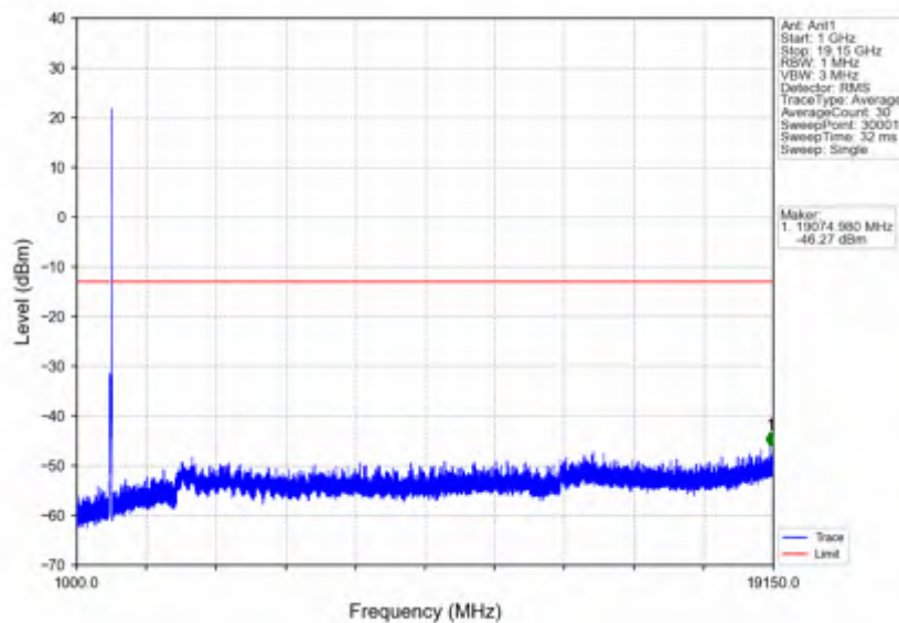
n25_30kHz_SISO_NTNV_30MHz_DFT-s-OFDM PI/2 BPSK_1900MHz_Outer_Full
