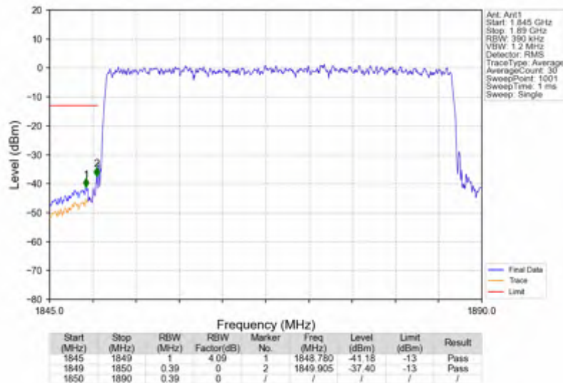
n25_30kHz_SISO_NTNV_40MHz_DFT-s-OFDM PI/2 BPSK_1870MHz_Outer_Full
