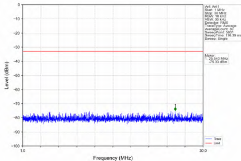
n25_30kHz_SISO_NTNV_30MHz_DFT-s-OFDM PI/2 BPSK_1900MHz_Outer_Full
