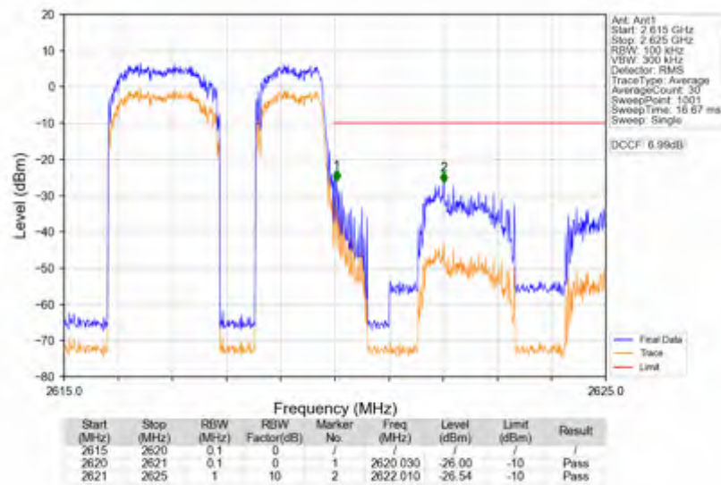
n38_15kHz_SISO_NTNV_5MHz_DFT-s-OFDM PI/2 BPSK_2617.5MHz_Outer_Full
