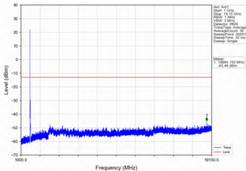
n25_30kHz_SISO_NTNV_40MHz_DFT-s-OFDM PI/2 BPSK_1870MHz_Outer_Full
