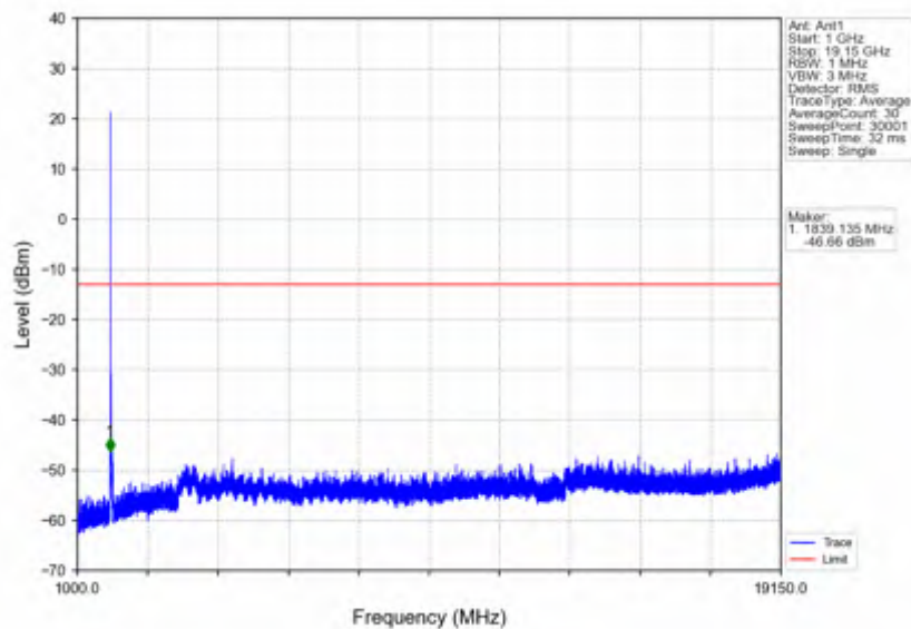
n25_30kHz_SISO_NTNV_25MHz_DFT-s-OFDM PI/2 BPSK_1862.5MHz_Outer_Full
