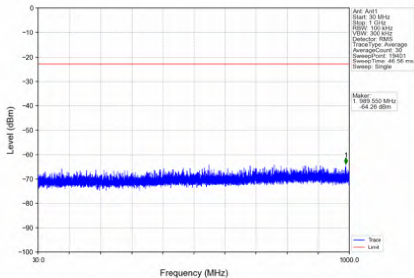
n25 30kHz SISO NTNV 40MHz CP-OFDM QPSK 1895MHz Outer Full
