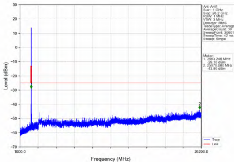
n38_15kHz_SISO_NTNV_5MHz_DFT-s-OFDM PI/2 BPSK_2572.5MHz_Outer_Full
