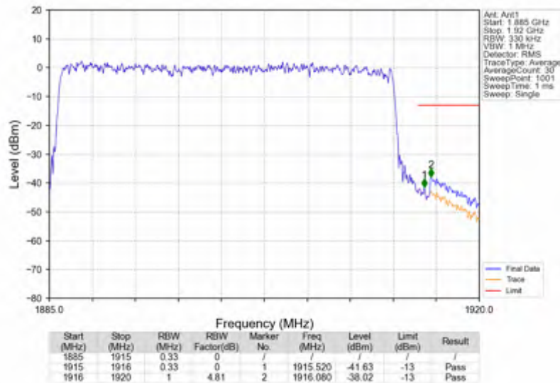
n25_30kHz_SISO_NTNV_30MHz_DFT-s-OFDM PI/2 BPSK_1900MHz_Outer_Full
