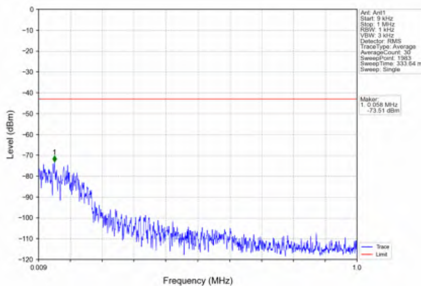
n38_15kHz_SISO_NTNV_5MHz_CP-OFDM QPSK 2572.5MHz_Edge_1RB_Left
