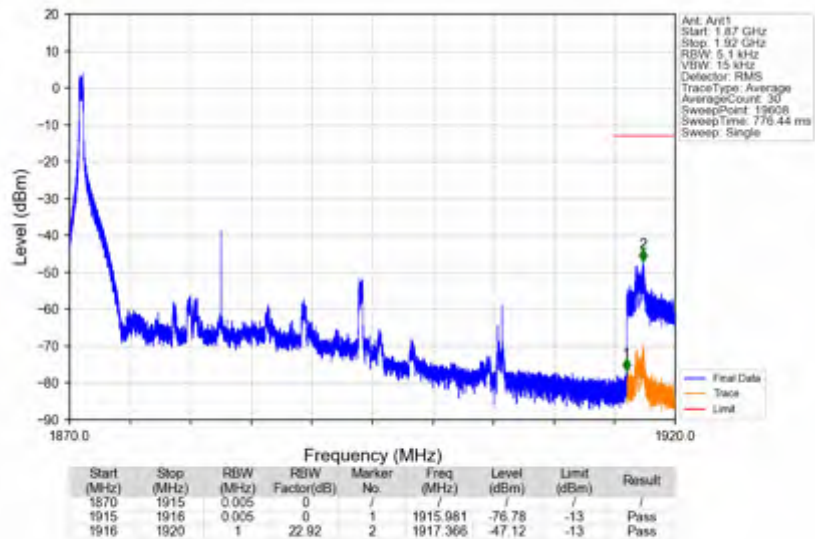
n25_30kHz_SISO_NTNV_25MHz_DFT-s-OFDM PI/2 BPSK_1882.5MHz_Edge_1RB_Left
