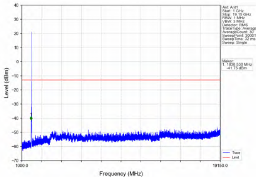
n25_30kHz_SISO_NTNV_40MHz_DFT-s-OFDM PI/2 BPSK_1895MHz_Outer_Full
