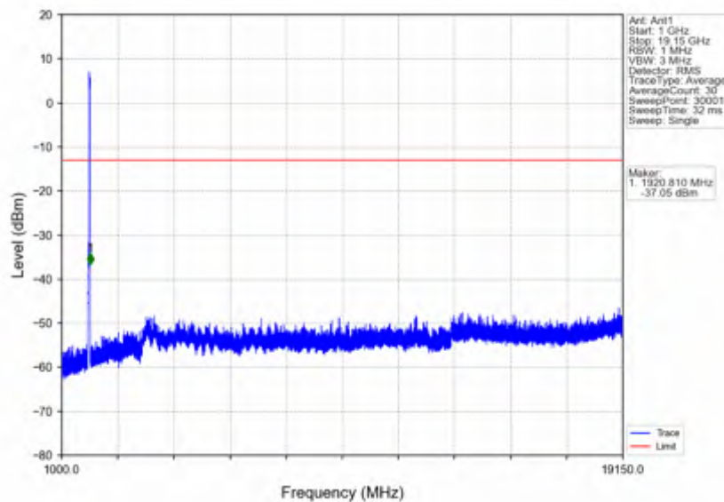
n25 30kHz SISO NTNV 40MHz CP-OFDM QPSK 1895MHz Outer Full
