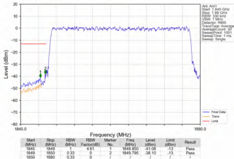
n25_30kHz_SISO_NTNV_30MHz_DFT-s-OFDM PI/2 BPSK_1865MHz_Outer_Full
