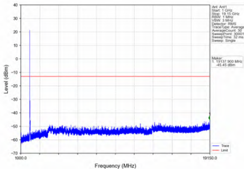
n25_30kHz_SISO_NTNV_30MHz_DFT-s-OFDM PI/2 BPSK_1865MHz_Outer_Full
