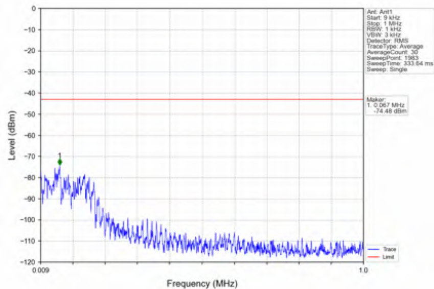
n38_15kHz_SISO_NTNV_5MHz_DFT-s-OFDM PI/2 BPSK_2617.5MHz_Edge_1RB_Right
