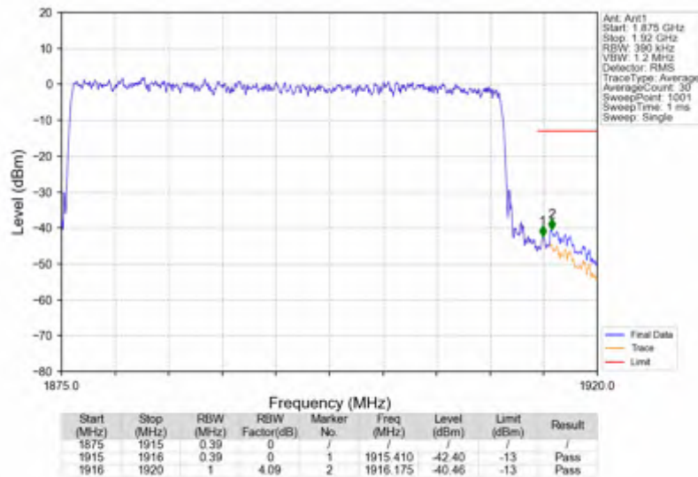
n25_30kHz_SISO_NTNV_40MHz_DFT-s-OFDM PI/2 BPSK_1895MHz_Outer_Full
