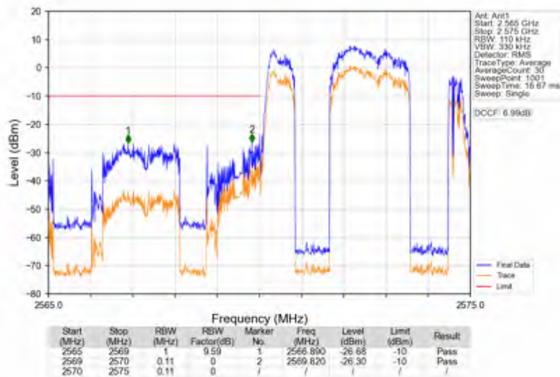
n38_15kHz_SISO_NTNV_5MHz_DFT-s-OFDM PI/2 BPSK_2572.5MHz_Outer_Full
