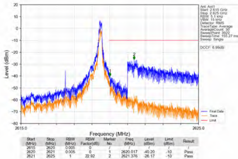
n38_15kHz_SISO_NTNV_5MHz_DFT-s-OFDM PI/2 BPSK_2617.5MHz_Inner_1RB_Right
