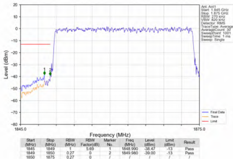
n25_30kHz_SISO_NTNV_25MHz_DFT-s-OFDM PI/2 BPSK_1862.5MHz_Outer_Full
