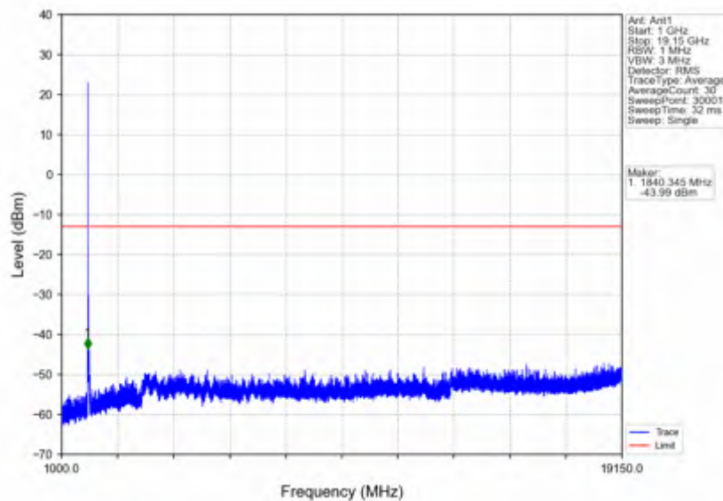
n25_30kHz_SISO_NTNV_25MHz_DFT-s-OFDM PI/2 BPSK_1882.5MHz_Edge_1RB_Left
