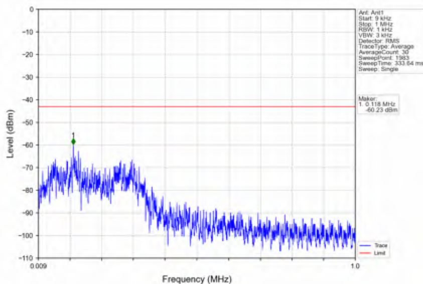
n25_30kHz_SISO_NTNV_25MHz_DFT-s-OFDM PI/2 BPSK_1862.5MHz_Edge_1RB_Left
