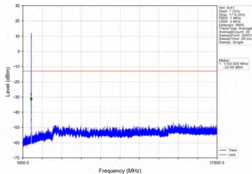
n66 30kHz SISO NTN 15MHz CP-OFDM QPSK 1717.5MHz Outer Full
