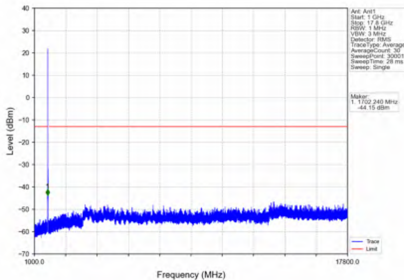
n66_30kHz_SISO_NTNV_10MHz_DFT-s-OFDM PI/2 BPSK_1715MHz_Outer_Full
