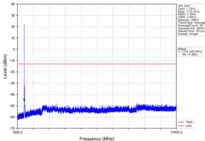
n66_15kHz_SISO_NTNV_40MHz_DFT-s-OFDM PI/2 BPSK_1745MHz_Edge_1RB_Left
