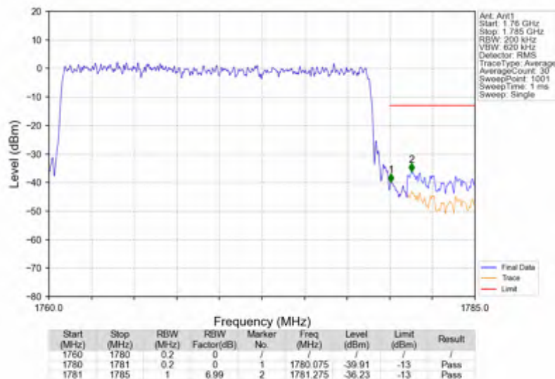
n66_30kHz_SISO_NTNV_20MHz_DFT-s-OFDM PI/2 BPSK_1770MHz_Outer_Full
