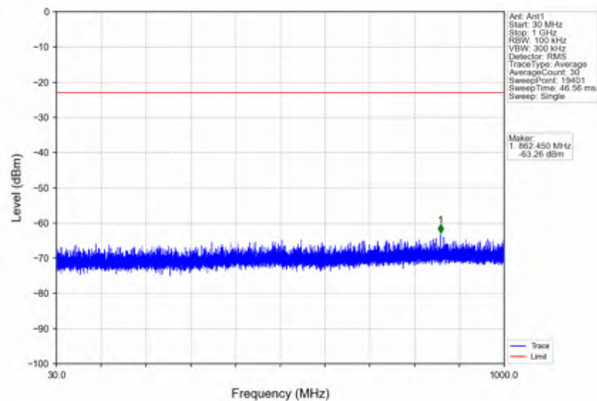
n66 30kHz SISO NTN 15MHz CP-OFDM QPSK 1717.5MHz Outer Full
