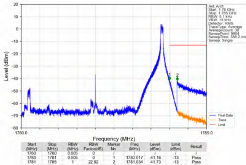
n66_30kHz_SISO_NTNV_20MHz_DFT-s-OFDM PI/2 BPSK_1770MHz_Edge_1RB_Right
