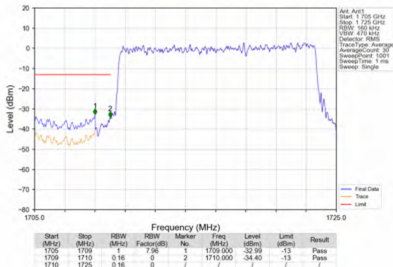
n66_30kHz_SISO_NTNV_15MHz_DFT-s-OFDM PI/2 BPSK_1717.5MHz_Outer_Full
