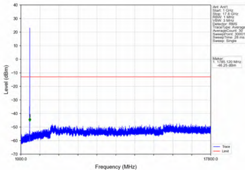
n66_30kHz_SISO_NTNV_10MHz_DFT-s-OFDM PI/2 BPSK_1775MHz_Outer_Full
