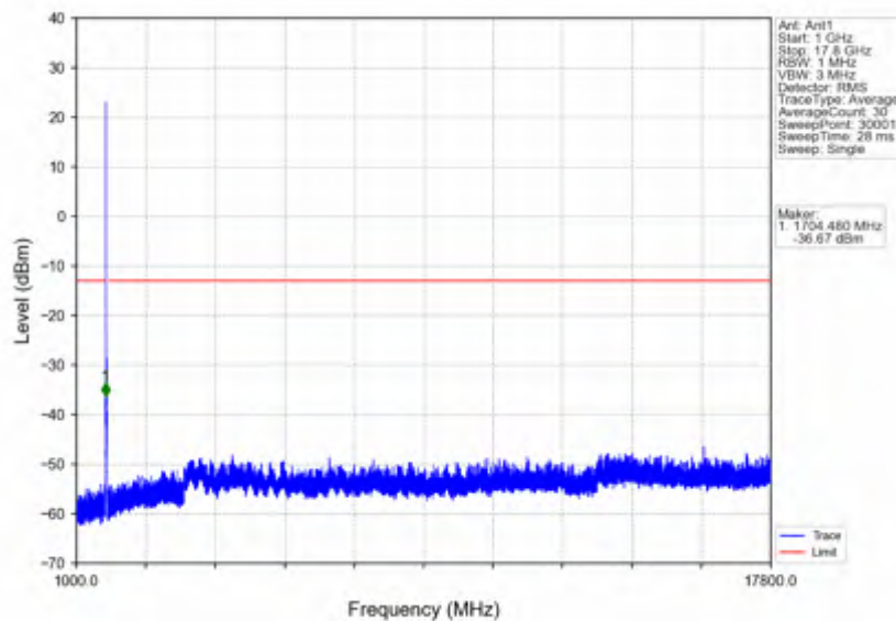
n66_30kHz_SISO_NTNV_15MHz_DFT-s-OFDM PI/2 BPSK_1745MHz_Edge_1RB_Left
