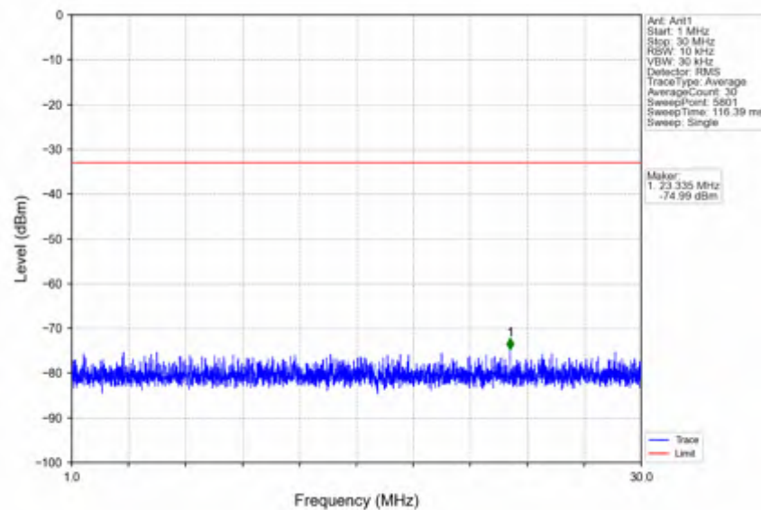
n66 30kHz SISO NTNV 20MHz DFT-s-OFDM PI/2 BPSK 1770MHz Outer Full
