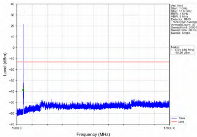
n66_30kHz_SISO_NTNV_20MHz_DFT-s-OFDM PI/2 BPSK_1720MHz_Outer_Full
