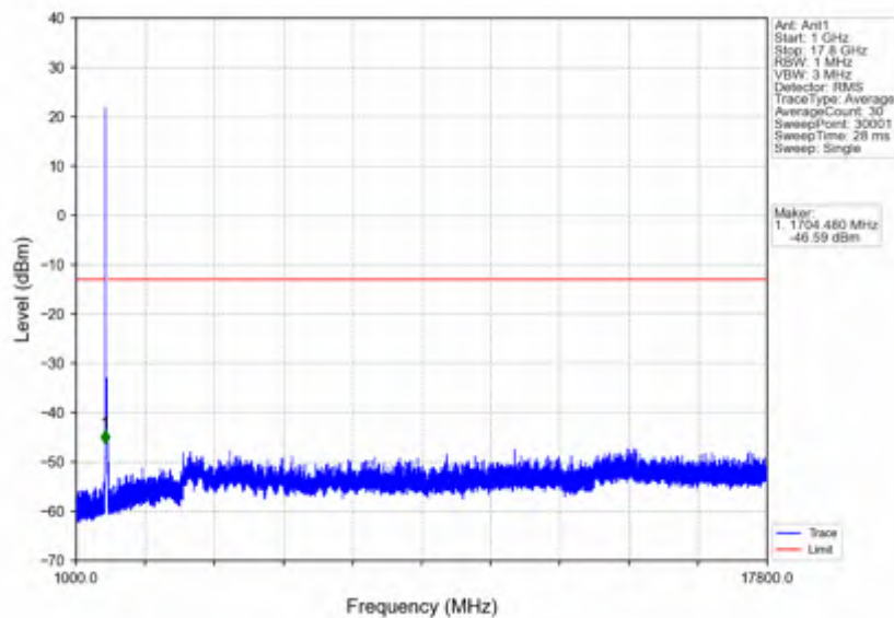
n66_15kHz_SISO_NTNV_40MHz_DFT-s-OFDM PI/2 BPSK_1730MHz_Outer_Full
