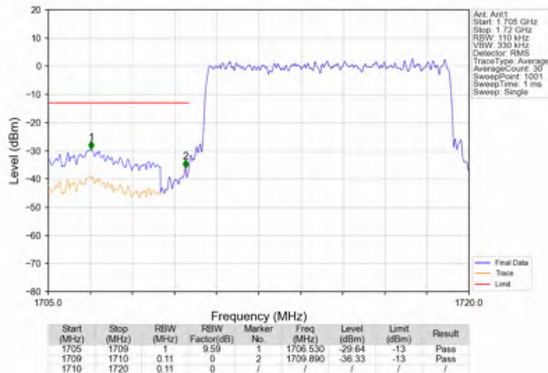
n66_30kHz_SISO_NTNV_10MHz_DFT-s-OFDM PI/2 BPSK_1715MHz_Outer_Full
