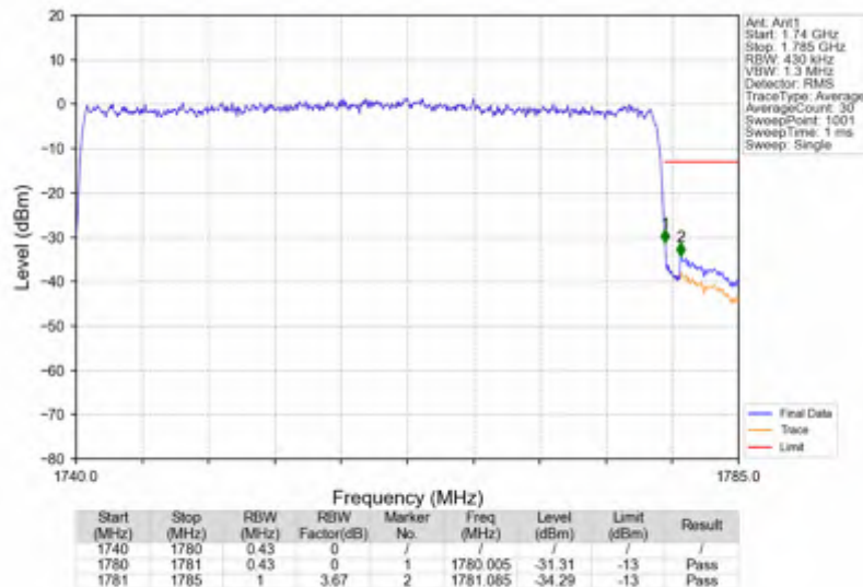
n66_15kHz_SISO_NTNV_40MHz_DFT-s-OFDM PI/2 BPSK_1760MHz_Outer_Full
