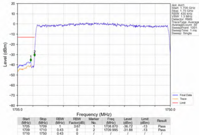
n66_15kHz_SISO_NTNV_40MHz_DFT-s-OFDM PI/2 BPSK_1730MHz_Outer_Full
