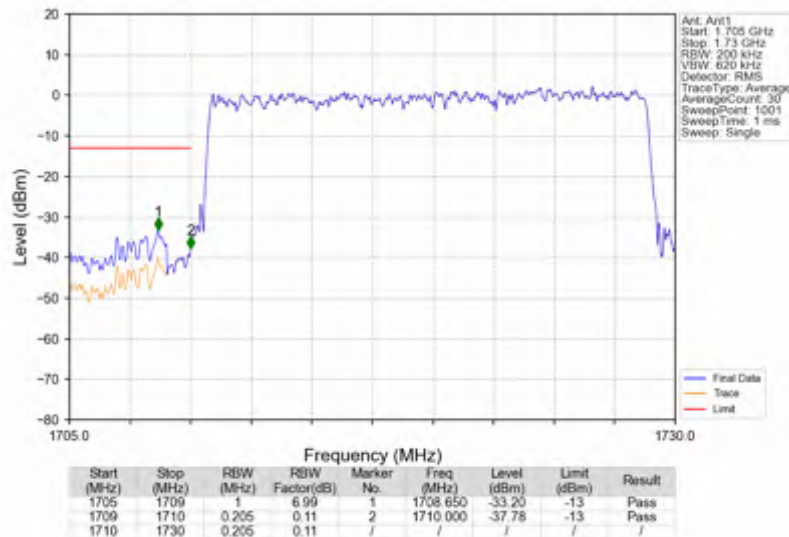
n66_30kHz_SISO_NTNV_20MHz_DFT-s-OFDM PI/2 BPSK_1720MHz_Outer_Full
