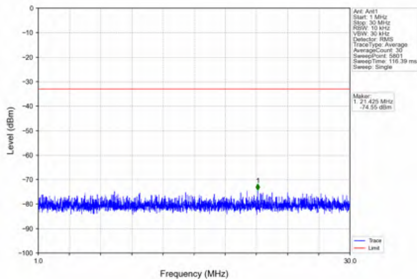
n66_30kHz_SISO_NTNV_10MHz_DFT-s-OFDM PI/2 BPSK_1715MHz_Edge_1RB_Left
