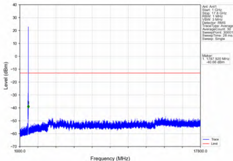
n66_30kHz_SISO_NTNV_20MHz_DFT-s-OFDM PI/2 BPSK_1770MHz_Outer_Full
