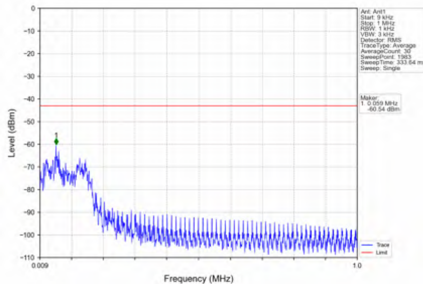
n66_15kHz_SISO_NTNV_40MHz_DFT-s-OFDM PI/2 BPSK_1745MHz_Edge_1RB_Left
