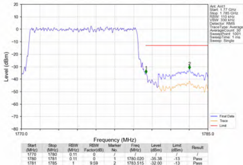
n66_30kHz_SISO_NTNV_10MHz_DFT-s-OFDM PI/2 BPSK_1775MHz_Outer_Full
