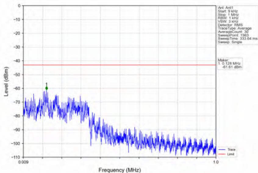
n66_30kHz_SISO_NTNV_15MHz_DFT-s-OFDM PI/2 BPSK_1717.5MHz_Edge_1RB_Left
