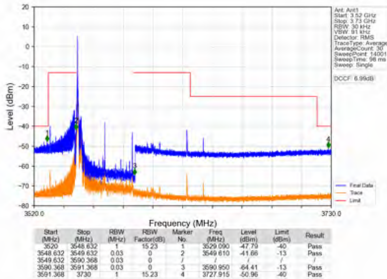
n78d_15kHz_SISO_NTNV_40MHz_DFT-s-OFDM QPSK_3570MHz_Edge_1RB_Left
