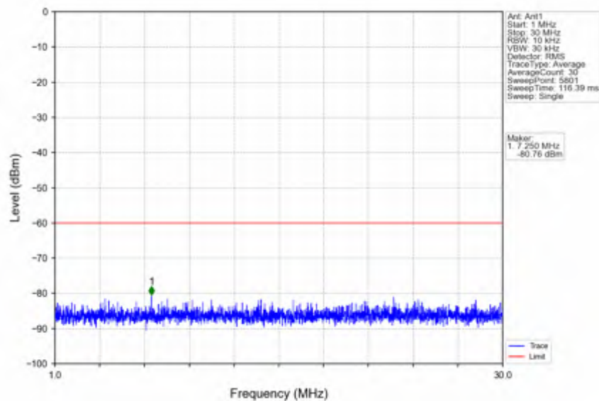
n78d_15kHz_SISO_NTNV_30MHz_DFT-s-OFDM_QPSK_3625.005MHz_Edge_1RB_Left
