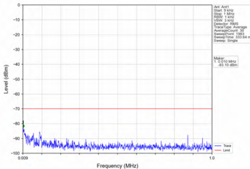
n78d_15kHz_SISO_NTNV_50MHz_DFT-s-OFDM_QPSK_3675MHz_Outer_Full
