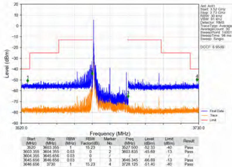
n78d_15kHz_SISO_NTNV_40MHz_DFT-s-OFDM QPSK_3625.005MHz_Edge_1RB_Left
