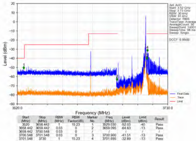
n78d_15kHz_SISO_NTNV_40MHz_DFT-s-OFDM QPSK_3679.995MHz_Inner_1RB_Right
