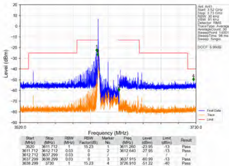
n78d_15kHz_SISO_NTNV_25MHz_CP-OFDM QPSK_3625.005MHz_Edge_1RB_Left
