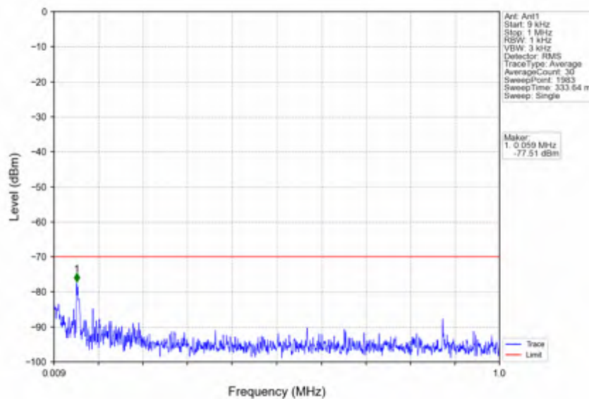
n78d_15kHz_SISO_NTNV_25MHz_DFT-s-OFDM QPSK_3625.005MHz_Edge_1RB_Left
