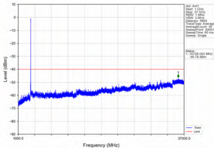
n78d_15kHz_SISO_NTNV_25MHz_DFT-s-OFDM QPSK_3687.495MHz_Inner_1RB_Right
