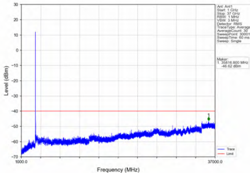
n78d_15kHz_SISO_NTNV_25MHz_CP-OFDM_QPSK_3625.005MHz_Edge_1RB_Left
