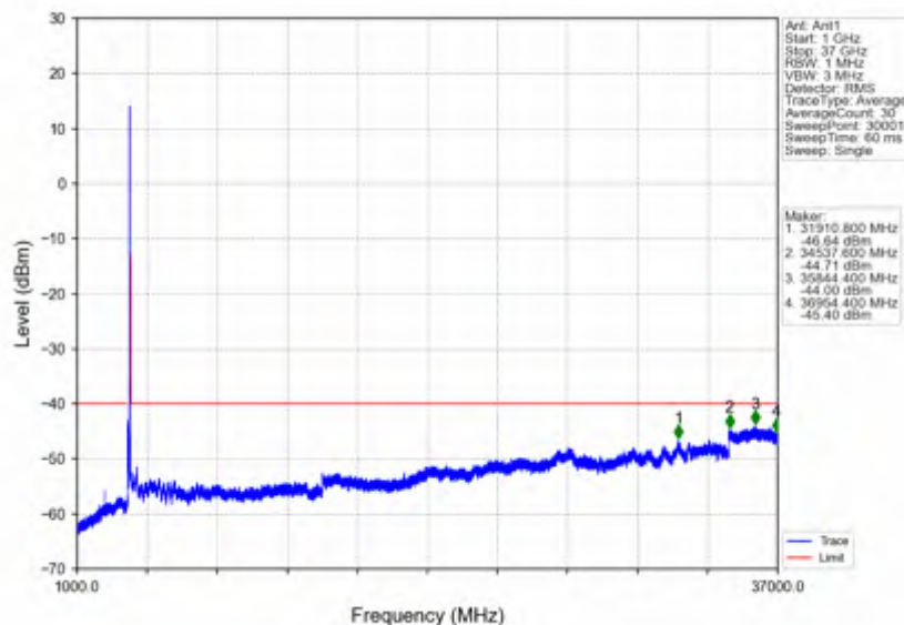
n78d_15kHz_SISO_NTNV_50MHz_DFT-s-OFDM QPSK_3575.01MHz_Edge_1RB_Left
