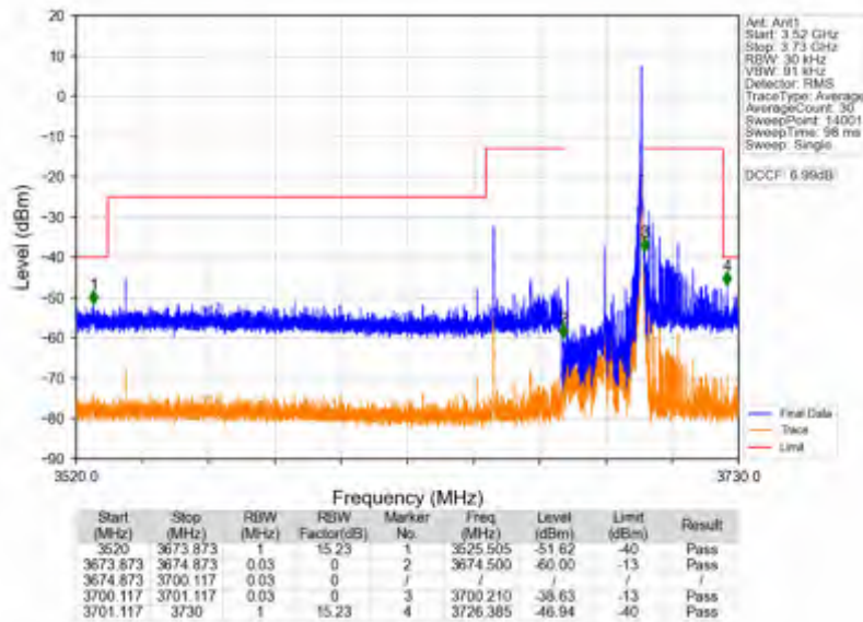
n78d_15kHz_SISO_NTNV_25MHz_DFT-s-OFDM QPSK_3687.495MHz_Inner_1RB_Right
