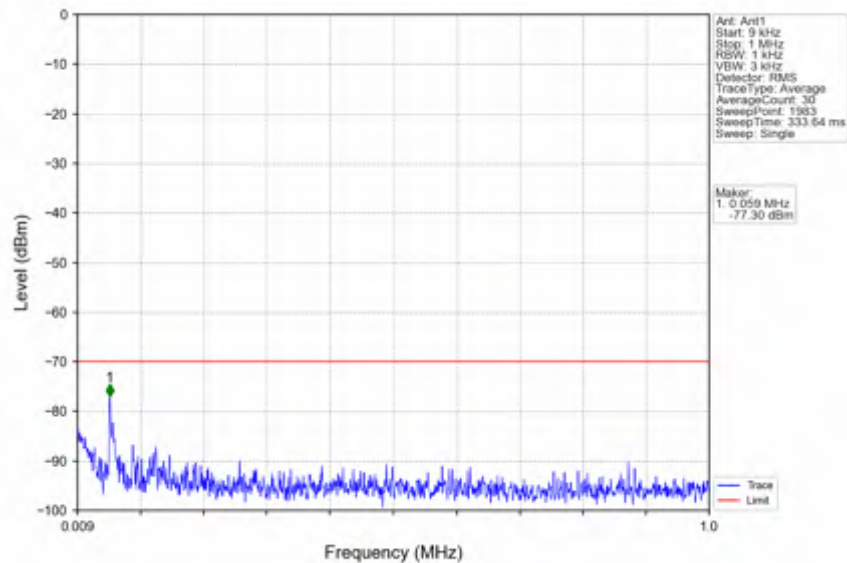
n78d_15kHz_SISO_NTNV_25MHz_DFT-s-OFDM QPSK_3562.5MHz_Edge_1RB_Left
