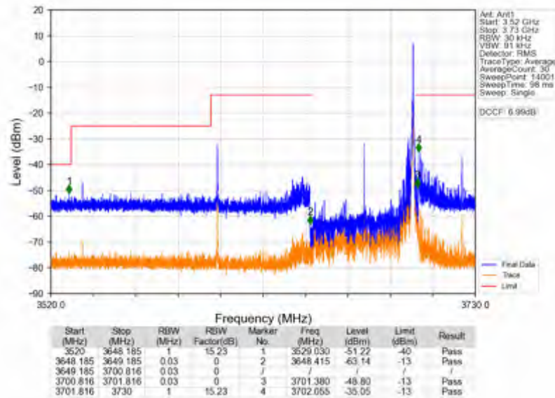
n78d_15kHz_SISO_NTNV_50MHz_CP-OFDM QPSK_3675MHz_Edge_1RB_Right
