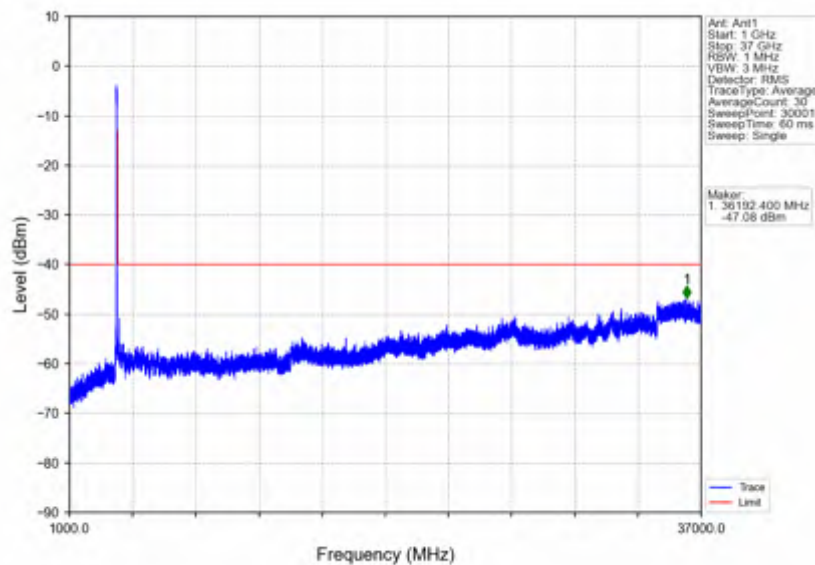
n78d_15kHz_SISO_NTNV_40MHz_DFT-s-OFDM QPSK_3679.995MHz_Inner_1RB_Right
