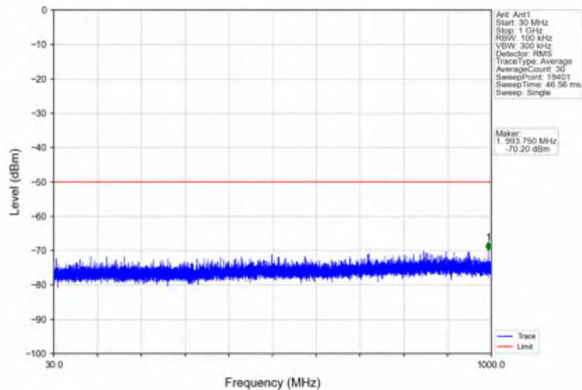
n78d_15kHz_SISO_NTNV_40MHz_CP-OFDM_QPSK_3570MHz_Edge_1RB_Left
