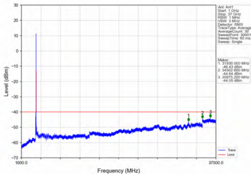
n78d_15kHz_SISO_NTNV_40MHz_DFT-s-OFDM QPSK_3570MHz_Edge_1RB_Left
