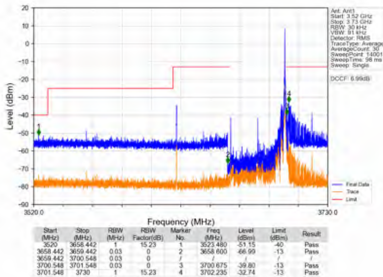
n78d_15kHz_SISO_NTNV_40MHz_DFT-s-OFDM QPSK_3679.995MHz_Edge_1RB_Right
