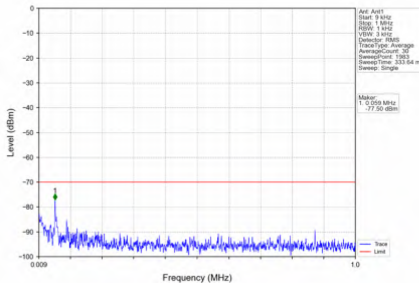
n78d_15kHz_SISO_NTNV_25MHz_DFT-s-OFDM QPSK_3562.5MHz_Outer_Full
