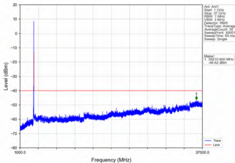
n78d_15kHz_SISO_NTNV_40MHz_CP-OFDM QPSK_3679.995MHz_Outer_Full
