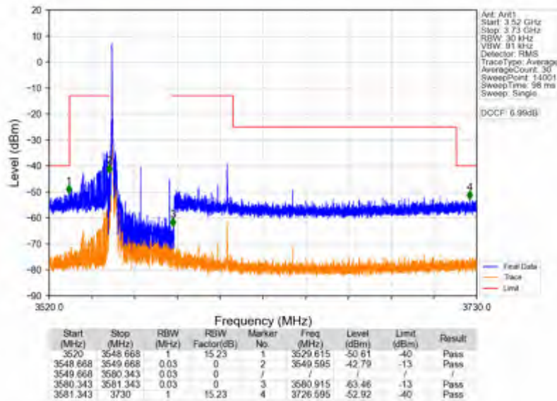
n78d_15kHz_SISO_NTNV_30MHz_DFT-s-OFDM QPSK_3565.005MHz_Inner_1RB_Left
