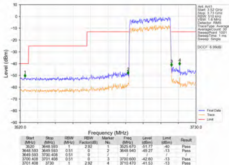
n78d 15kHz SISO NTNV 50MHz DFT-s-OFDM PI/2 BPSK 3675MHz Outer Full
