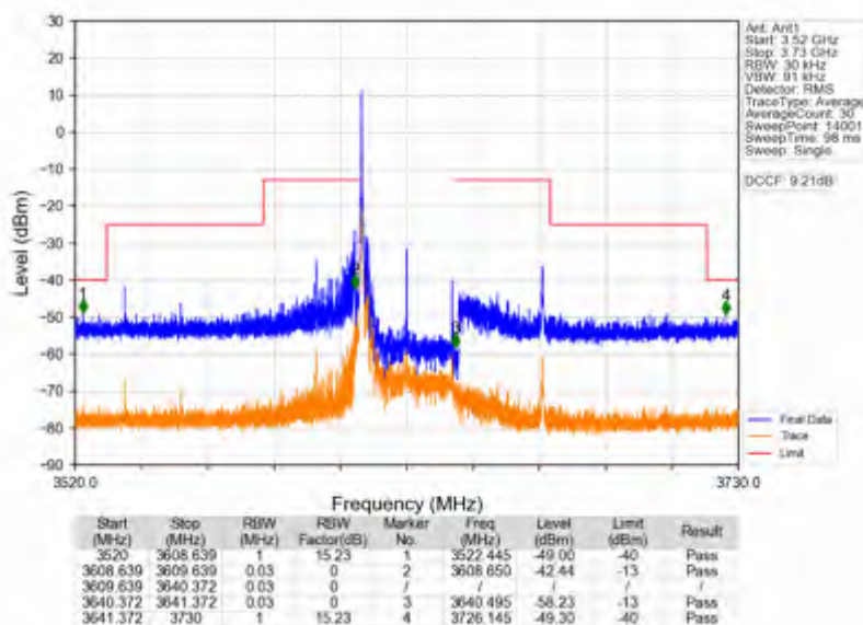
n78d_15kHz_SISO_NTNV_30MHz_CP-OFDM_QPSK_3625.005MHz_Edge_1RB_Left
