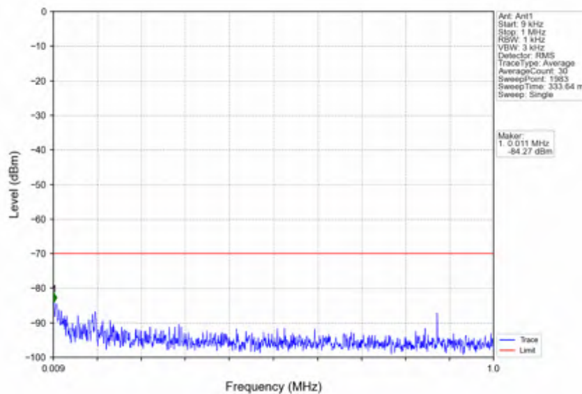
n78d_15kHz_SISO_NTNV_30MHz_DFT-s-OFDM_QPSK_3684.99MHz_Outer_Full
