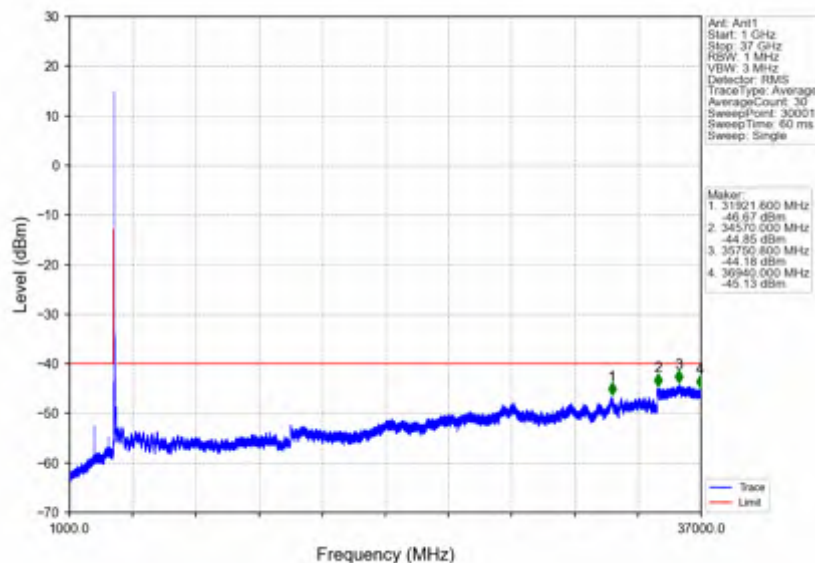
n78d_15kHz_SISO_NTNV_50MHz_CP-OFDM QPSK_3575.01MHz_Outer_Full
