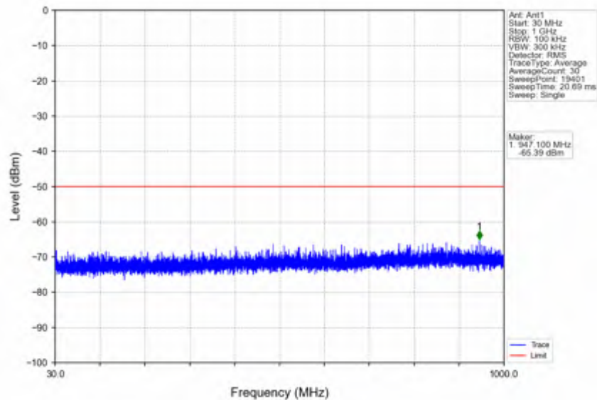
n78d_15kHz_SISO_NTNV_40MHz_CP-OFDM_QPSK_3570MHz_Outer_Full
