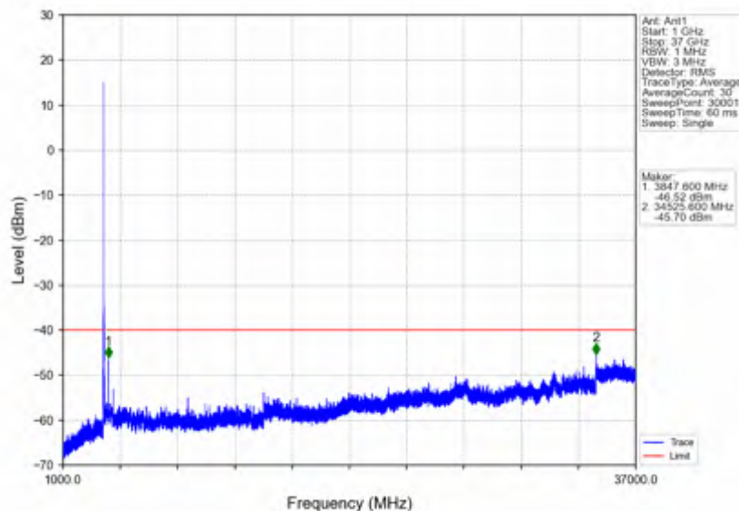
n78d_15kHz_SISO_NTNV_25MHz_CP-OFDM QPSK_3562.5MHz_Outer_Full
