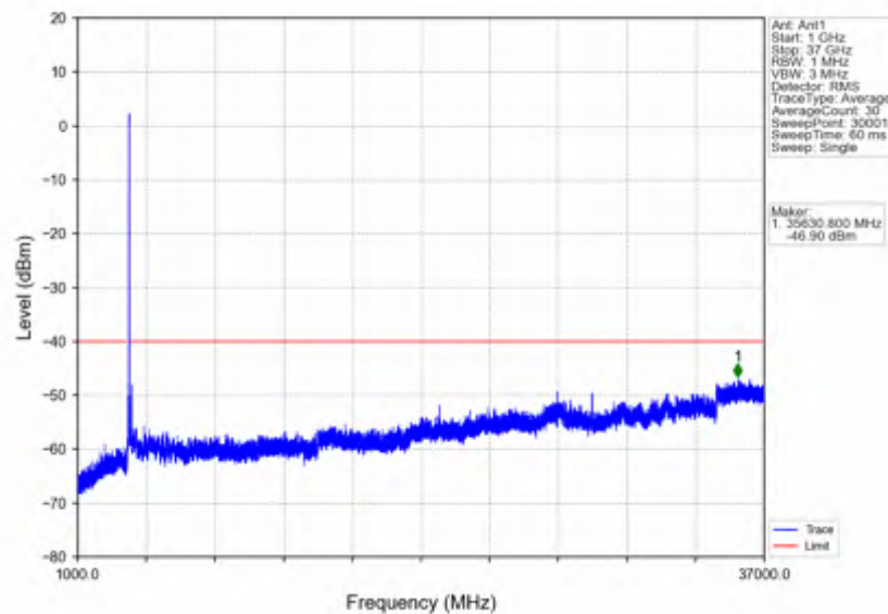
n78d_15kHz_SISO_NTNV_30MHz_CP-OFDM QPSK_3684.99MHz_Outer_Full
