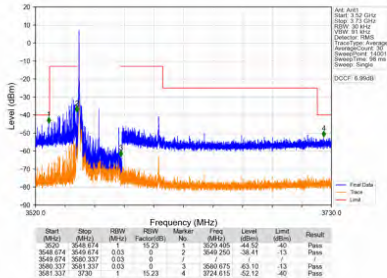
n78d_15kHz_SISO_NTNV_30MHz_CP-OFDM_QPSK_3565.005MHz_Inner_1RB_Left
