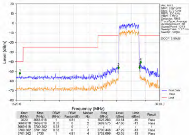
n78d_15kHz_SISO_NTNV_30MHz_CP-OFDM QPSK_3684.99MHz_Outer_Full
