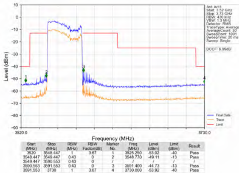
n78d_15kHz_SISO_NTNV_40MHz_CP-OFDM QPSK_3570MHz_Outer_Full
