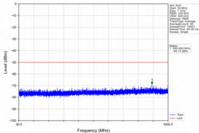
n78d_15kHz_SISO_NTNV_50MHz_CP-OFDM_QPSK_3625.005MHz_Edge_1RB_Left
