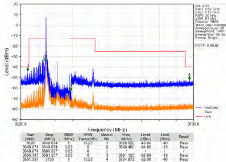
n78d_15kHz_SISO_NTNV_30MHz_CP-OFDM_QPSK_3565.005MHz_Edge_1RB_Left
