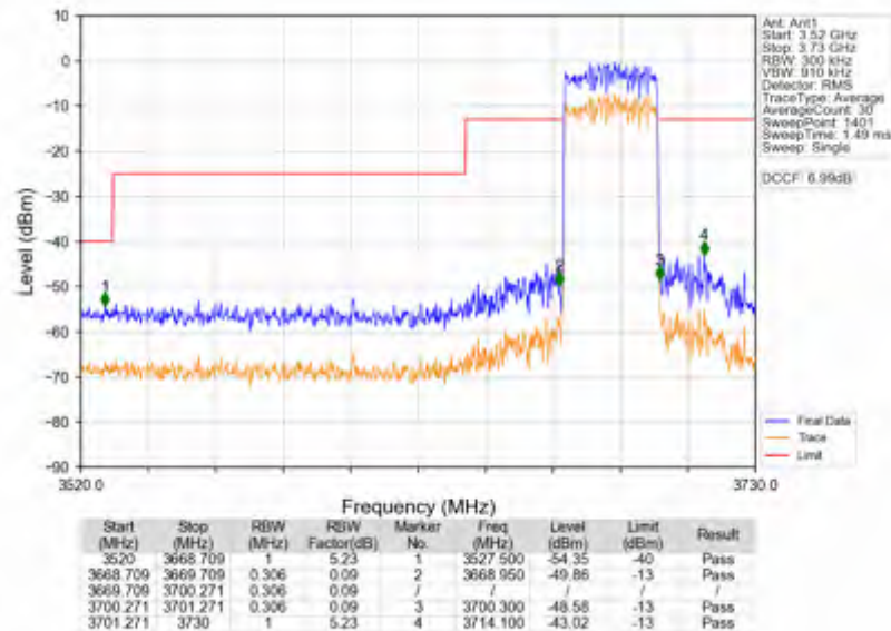
n78d_15kHz_SISO_NTNV_30MHz_DFT-s-OFDM_QPSK_3684.99MHz_Outer_Full
