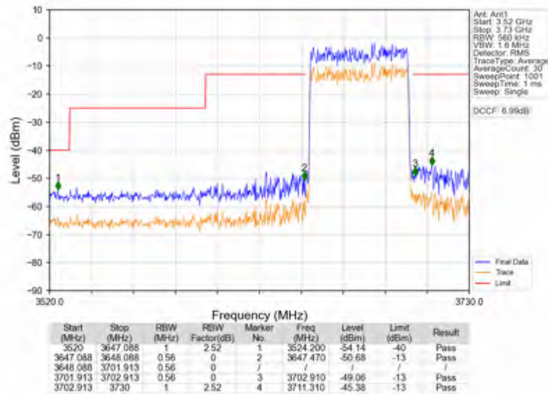
n78d_15kHz_SISO_NTNV_50MHz_DFT-s-OFDM_QPSK_3675MHz_Outer_Full
