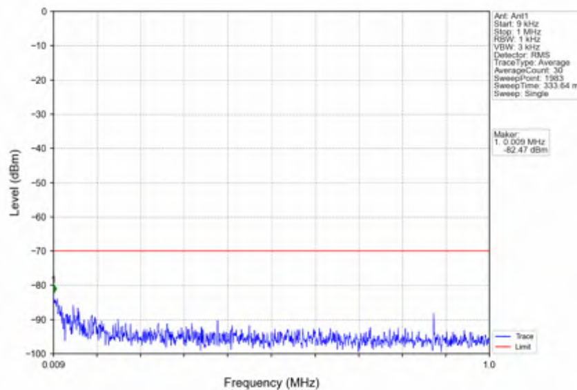
n78d_15kHz_SISO_NTNV_40MHz_DFT-s-OFDM QPSK_3679.995MHz_Outer_Full
