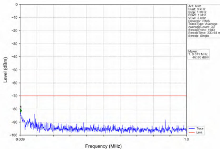
n78d_15kHz_SISO_NTNV_50MHz_DFT-s-OFDM QPSK_3625.005MHz_Edge_1RB_Left
