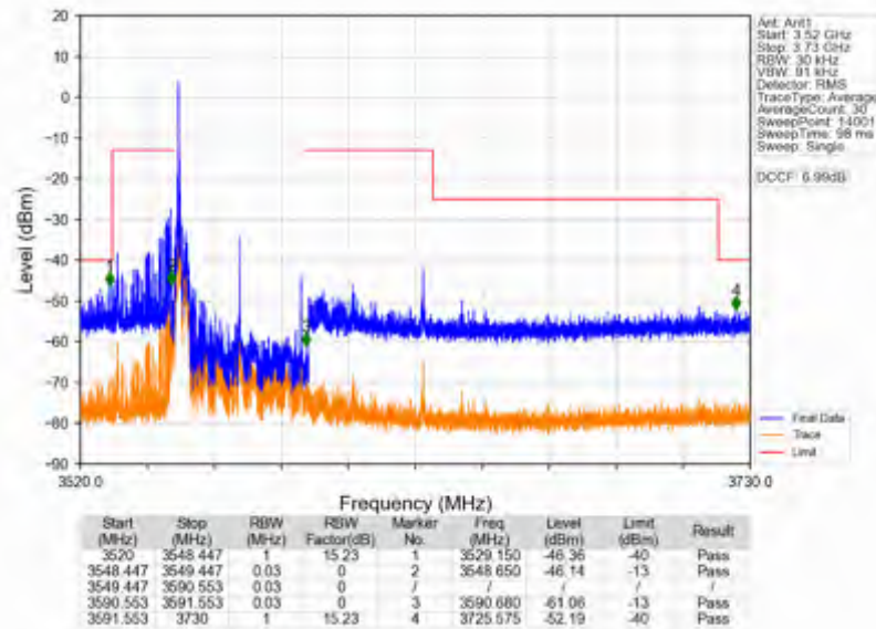
n78d_15kHz_SISO_NTV_40MHz_CP-OFDM_QPSK_3570MHz_Inner_1RB_Left
