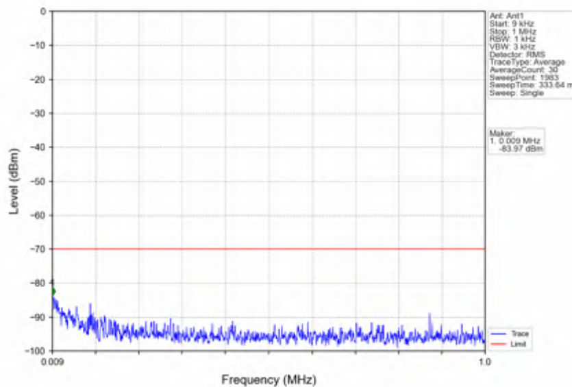
n78d_15kHz_SISO_NTNV_40MHz_DFT-s-OFDM QPSK_3625.005MHz_Edge_1RB_Left
