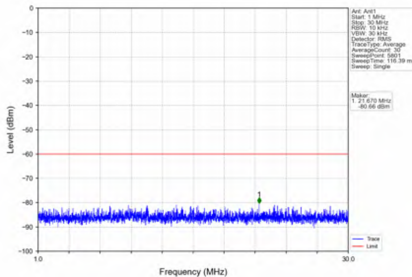
n78d_15kHz_SISO_NTNV_50MHz_DFT-s-OFDM_QPSK_3575.01MHz_Outer_Full
