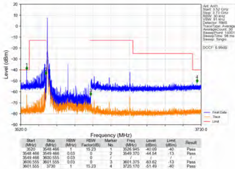
n78d_15kHz_SISO_NTNV_50MHz_DFT-s-OFDM_QPSK_3575.01MHz_Inner_1RB_Left
