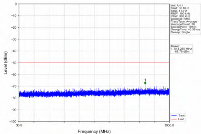
n78d_15kHz_SISO_NTNV_30MHz_CP-OFDM_QPSK_3565.005MHz_Inner_1RB_Left
