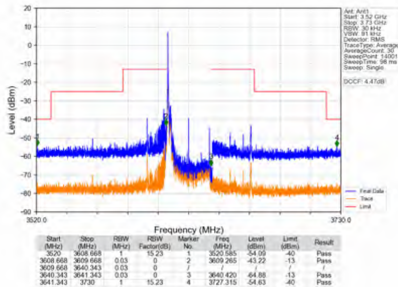
n78d_15kHz_SISO_NTNV_30MHz_DFT-s-OFDM QPSK_3625.005MHz_Edge_1RB_Left
