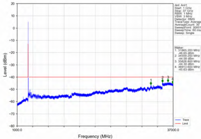
n78d_15kHz_SISO_NTNV_40MHz_DFT-s-OFDM PI/2 BPSK_3625.005MHz_Edge_1RB_Left
