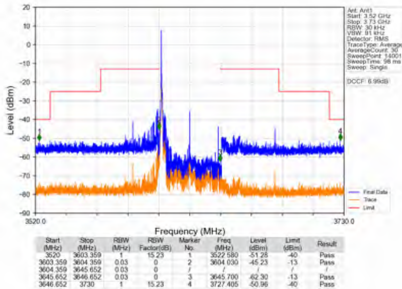
n78d_15kHz_SISO_NTNV_40MHz_CP-OFDM QPSK_3625.005MHz_Edge_1RB_Left
