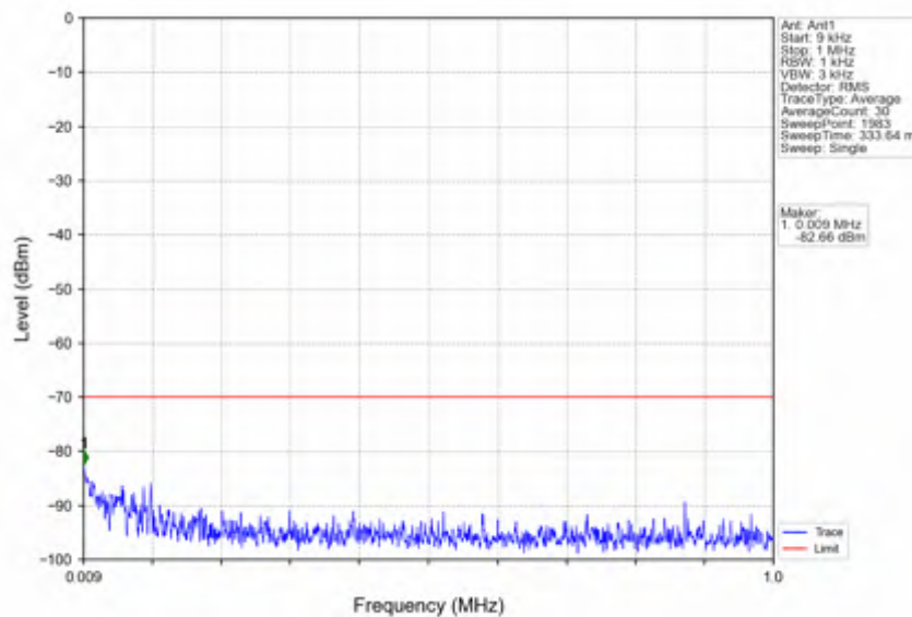
n78d_15kHz_SISO_NTNV_40MHz_CP-OFDM_QPSK_3570MHz_Edge_1RB_Left
