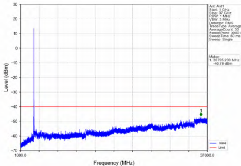
n78d_15kHz_SISO_NTNV_25MHz_DFT-s-OFDM_QPSK_3562.5MHz_Edge_1RB_Left
