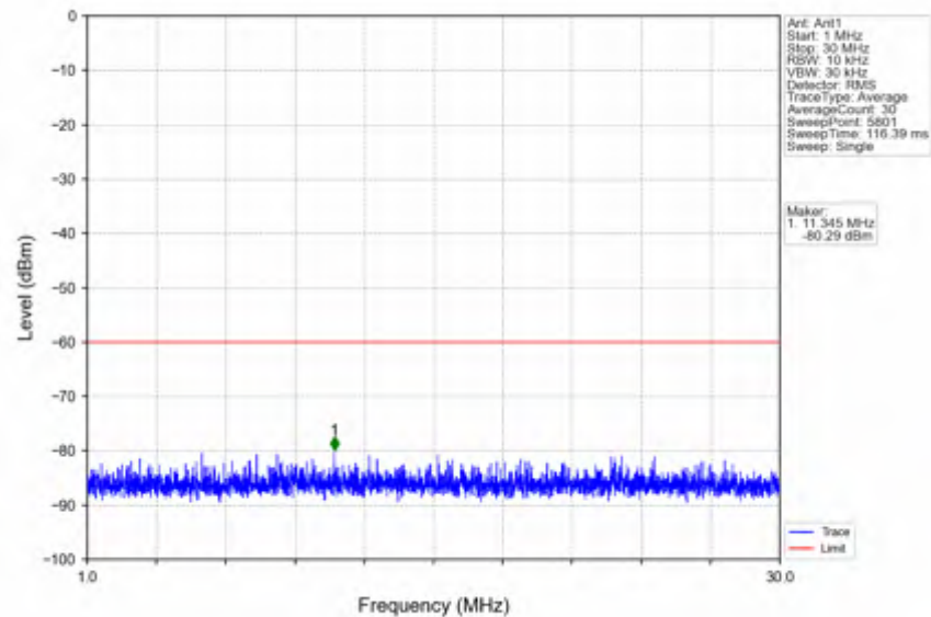
n78d_15kHz_SISO_NTNV_50MHz_DFT-s-OFDM QPSK_3675MHz_Edge_1RB_Right
