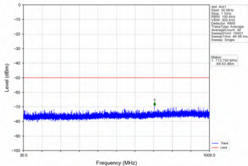
n78d_15kHz_SISO_NTNV_50MHz_DFT-s-OFDM QPSK_3675MHz_Inner_1RB_Right
