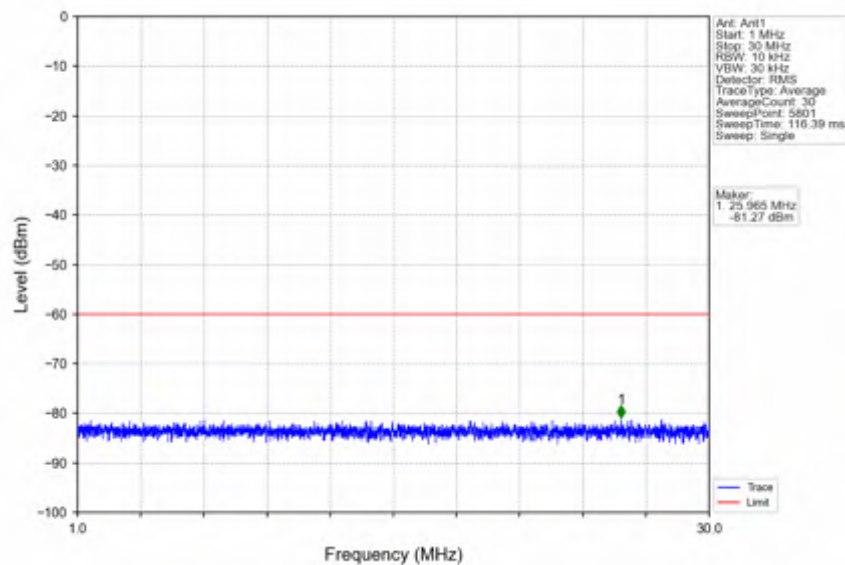
n78d_15kHz_SISO_NTNV_40MHz_DFT-s-OFDM PI/2 BPSK_3570MHz_Edge_1RB_Left
