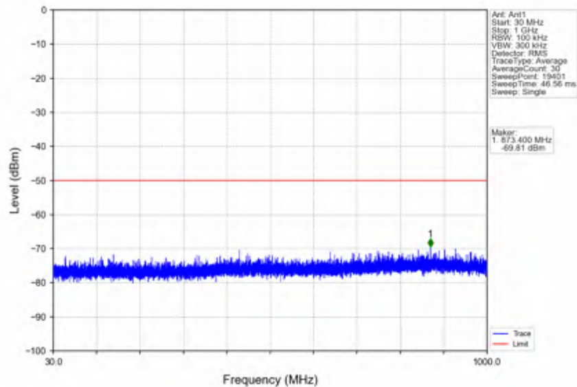
n78d_15kHz_SISO_NTNV_50MHz_DFT-s-OFDM QPSK_3675MHz_Edge_1RB_Right
