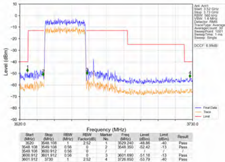
n78d_15kHz_SISO_NTNV_50MHz_DFT-s-OFDM_QPSK_3575.01MHz_Outer_Full
