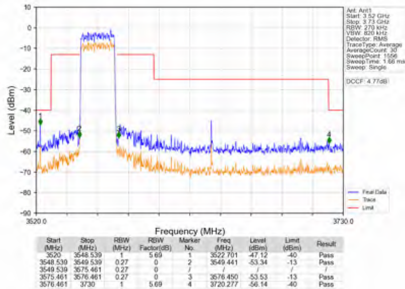
n78d_15kHz_SISO_NTNV_25MHz_DFT-s-OFDM QPSK_3562.5MHz_Outer_Full
