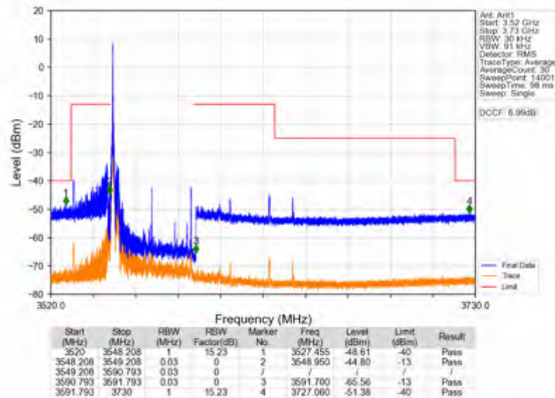
n78d_15kHz_SISO_NTNV_40MHz_DFT-s-OFDM_PI/2_BPSK_3570MHz_Edge_1RB_Left
