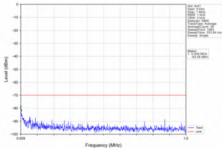
n78d_15kHz_SISO_NTNV_30MHz_DFT-s-OFDM QPSK_3684.99MHz_Inner_1RB_Right
