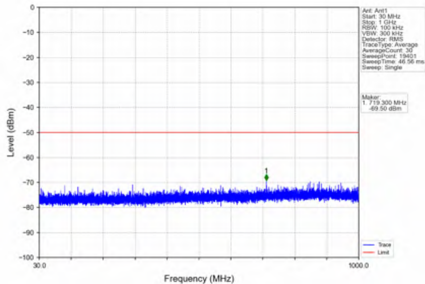
n78d_15kHz_SISO_NTNV_30MHz_DFT-s-OFDM_QPSK_3684.99MHz_Outer_Full
