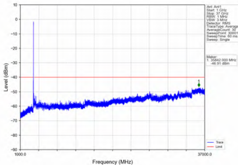
n78d_15kHz_SISO_NTNV_30MHz_DFT-s-OFDM QPSK_3565.005MHz_Inner_1RB_Left
