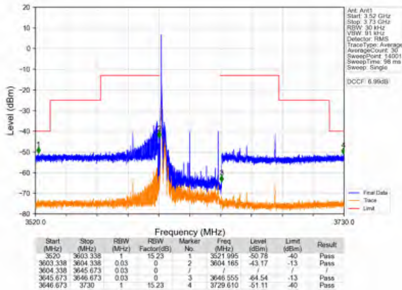
n78d_15kHz_SISO_NTNV_40MHz_DFT-s-OFDM PI/2 BPSK_3625.005MHz_Edge_1RB_Left
