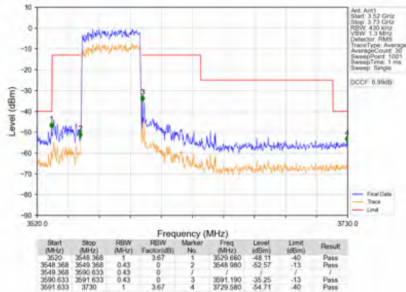
n78d_15kHz_SISO_NTNV_40MHz_DFT-s-OFDM_QPSK_3570MHz_Outer_Full
