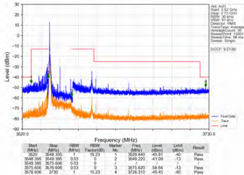
n78d_15kHz_SISO_NTNV_25MHz_CP-OFDM QPSK_3562.5MHz_Edge_1RB_Left
