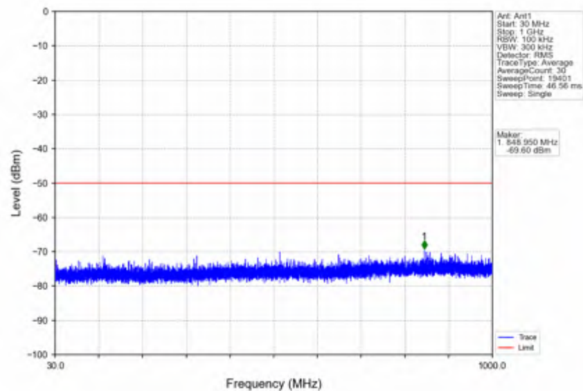
n78d_15kHz_SISO_NTNV_30MHz_DFT-s-OFDM_QPSK_3565.005MHz_Inner_1RB_Left
