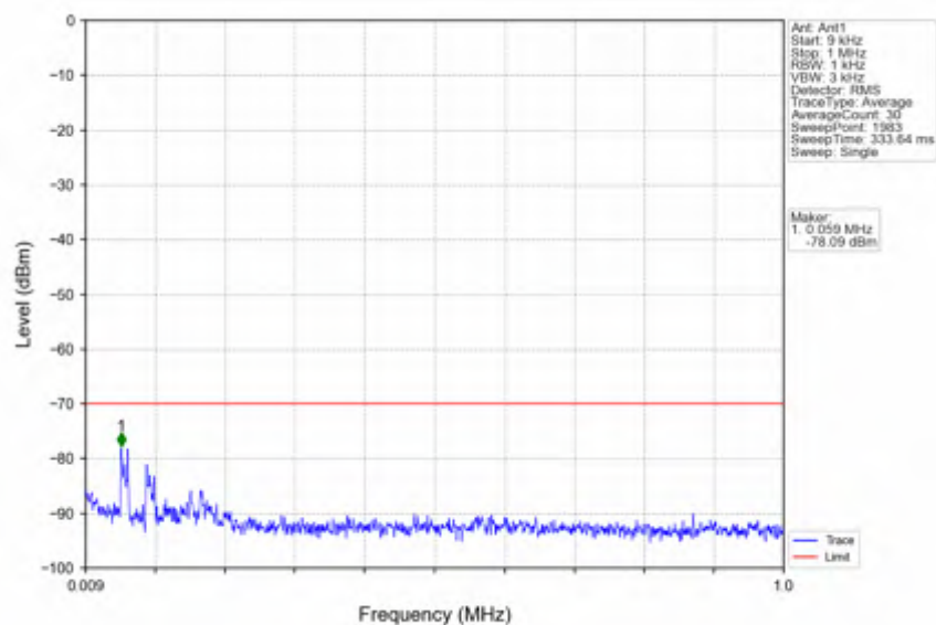
n78d_15kHz_SISO_NTNV_50MHz_DFT-s-OFDM PI/2 BPSK_3575.01MHz_Edge_1RB_Left
