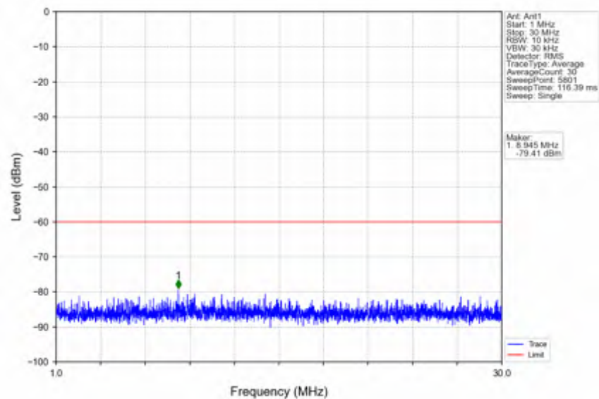
n78d_15kHz_SISO_NTNV_30MHz_DFT-s-OFDM QPSK_3684.99MHz_Edge_1RB_Right
