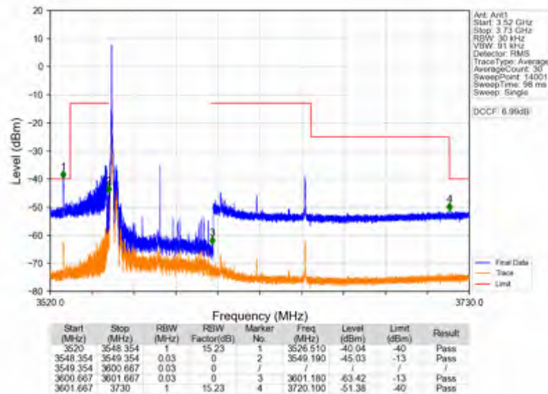
n78d_15kHz_SISO_NTNV_50MHz_DFT-s-OFDM PI/2 BPSK_3575.01MHz_Edge_1RB_Left
