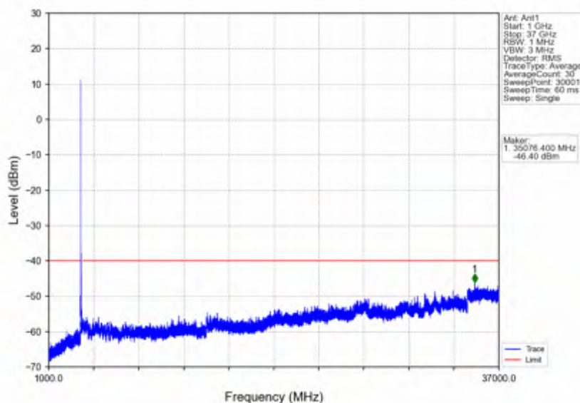
n78d_15kHz_SISO_NTNV_30MHz_CP-OFDM QPSK_3565.005MHz_Outer_Full
