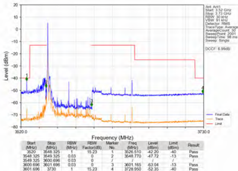
n78d_15kHz_SISO_NTNV_50MHz_DFT-s-OFDM QPSK_3575.01MHz_Edge_1RB_Left
