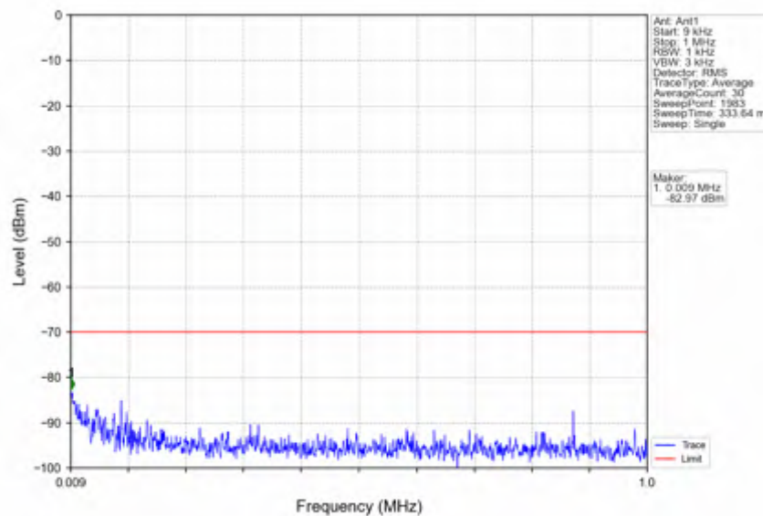
n78d_15kHz_SISO_NTNV_30MHz_CP-OFDM_QPSK_3565.005MHz_Edge_1RB_Left
