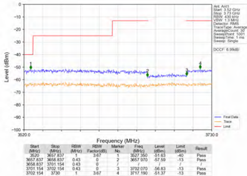
n78d_15kHz_SISO_NTNV_40MHz_DFT-s-OFDM PI/2 BPSK_3679.995MHz_Outer_Full
