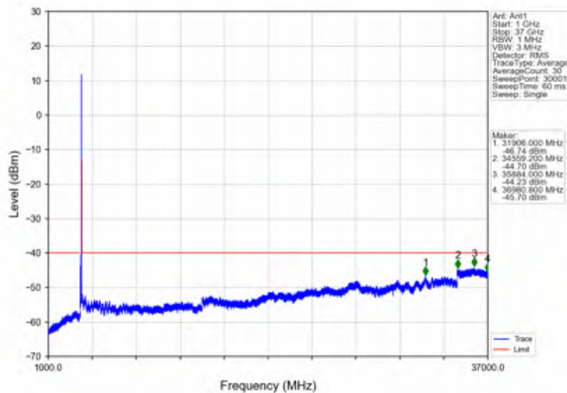
n78d_15kHz_SISO_NTNV_40MHz_DFT-s-OFDM PI/2 BPSK_3679.995MHz_Outer_Full
