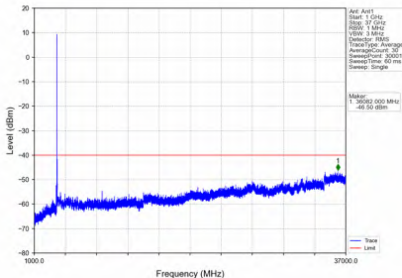
n78d_15kHz_SISO_NTNV_40MHz_DFT-s-OFDM QPSK_3679.995MHz_Edge_1RB_Right
