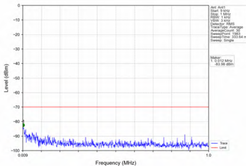
n78d_15kHz_SISO_NTNV_30MHz_DFT-s-OFDM QPSK_3625.005MHz_Edge_1RB_Left
