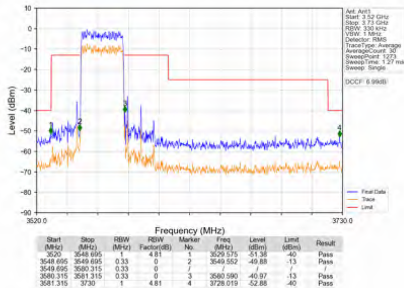
n78d_15kHz_SISO_NTNV_30MHz_DFT-s-OFDM QPSK_3565.005MHz_Outer_Full
