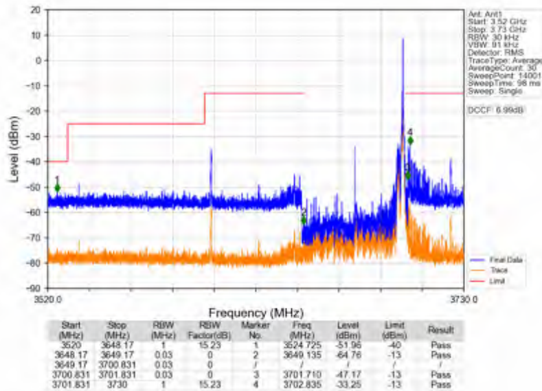
n78d_15kHz_SISO_NTNV_50MHz_DFT-s-OFDM QPSK_3675MHz_Edge_1RB_Right
