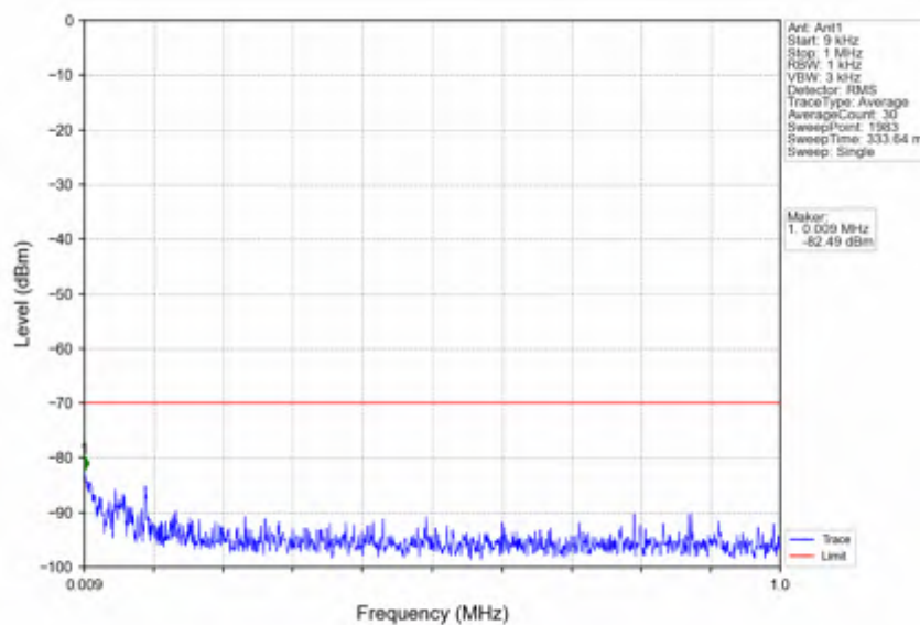
n78d_15kHz_SISO_NTV_40MHz_CP-OFDM_QPSK_3570MHz_Inner_1RB_Left
