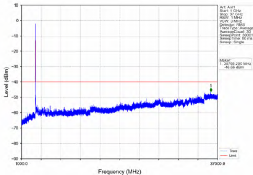
n78d_15kHz_SISO_NTNV_50MHz_DFT-s-OFDM_QPSK_3575.01MHz_Inner_1RB_Left
