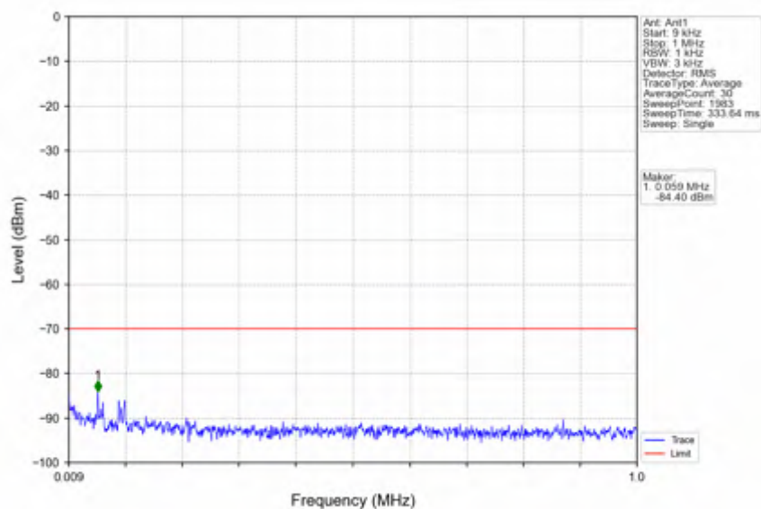
n78d_15kHz_SISO_NTNV_40MHz_DFT-s-OFDM_PI/2_BPSK_3570MHz_Edge_1RB_Left
