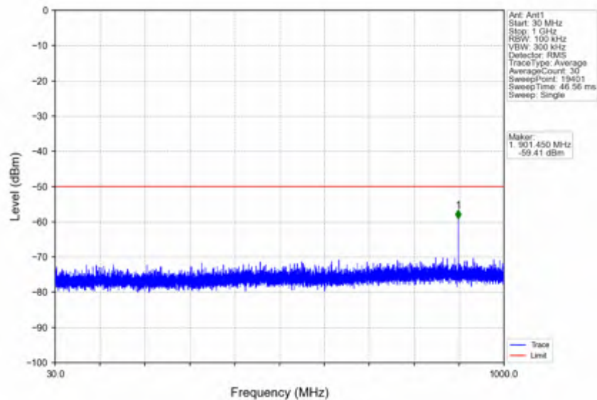
n78d_15kHz_SISO_NTNV_30MHz_DFT-s-OFDM QPSK_3684.99MHz_Edge_1RB_Right
