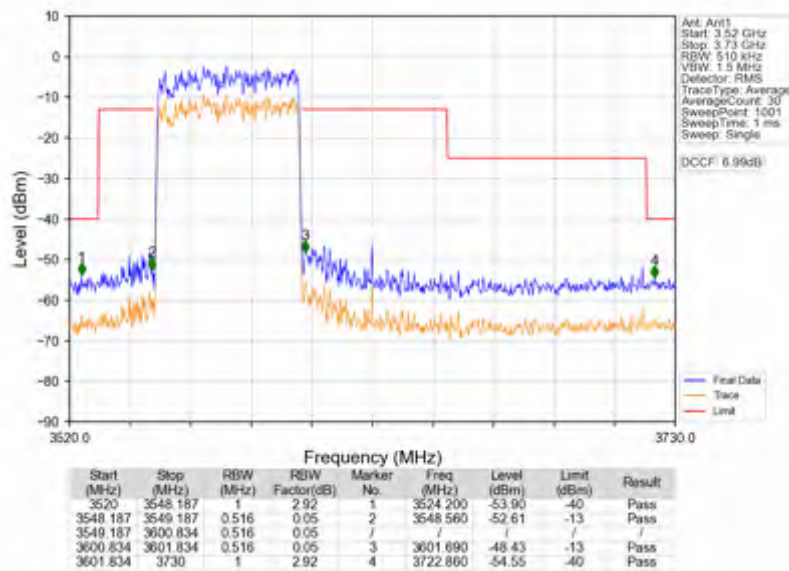
n78d_15kHz_SISO_NTNV_50MHz_CP-OFDM QPSK_3575.01MHz_Outer_Full
