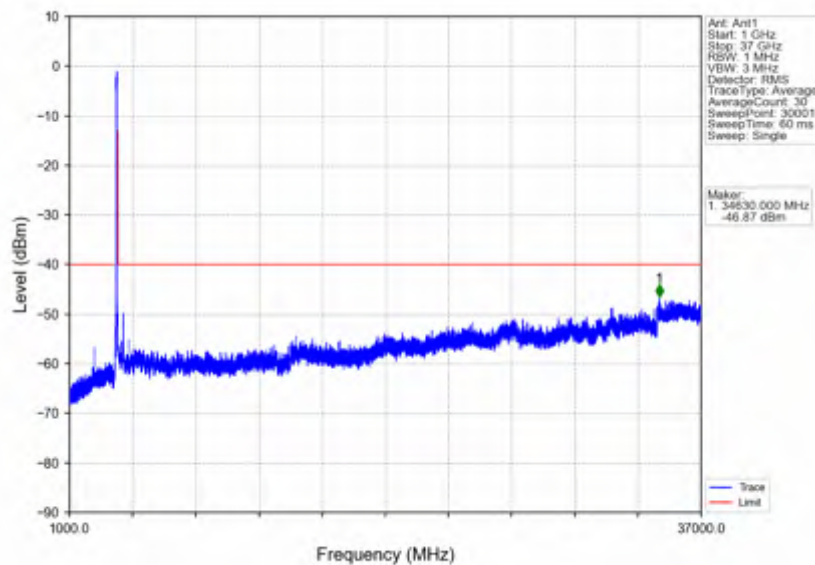
n78d_15kHz_SISO_NTNV_50MHz_DFT-s-OFDM QPSK_3675MHz_Inner_1RB_Right
