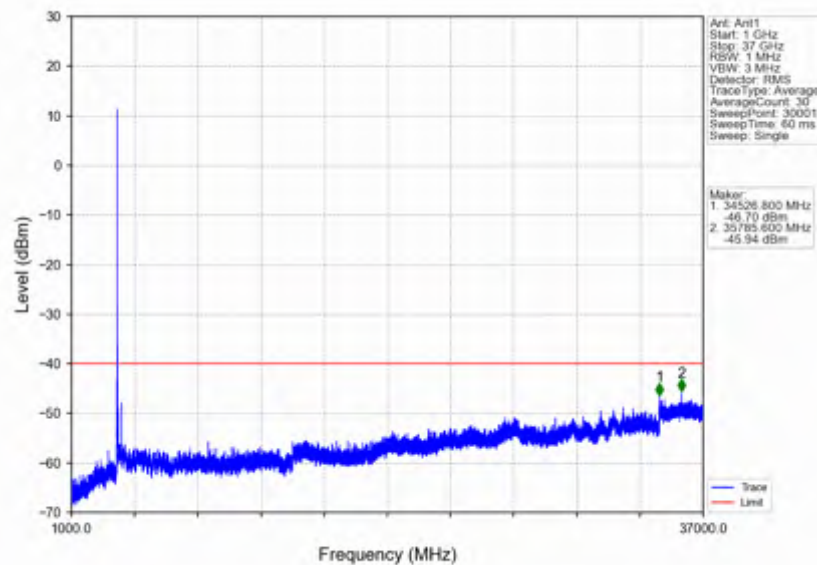
n78d_15kHz_SISO_NTNV_50MHz_CP-OFDM_QPSK_3625.005MHz_Edge_1RB_Left
