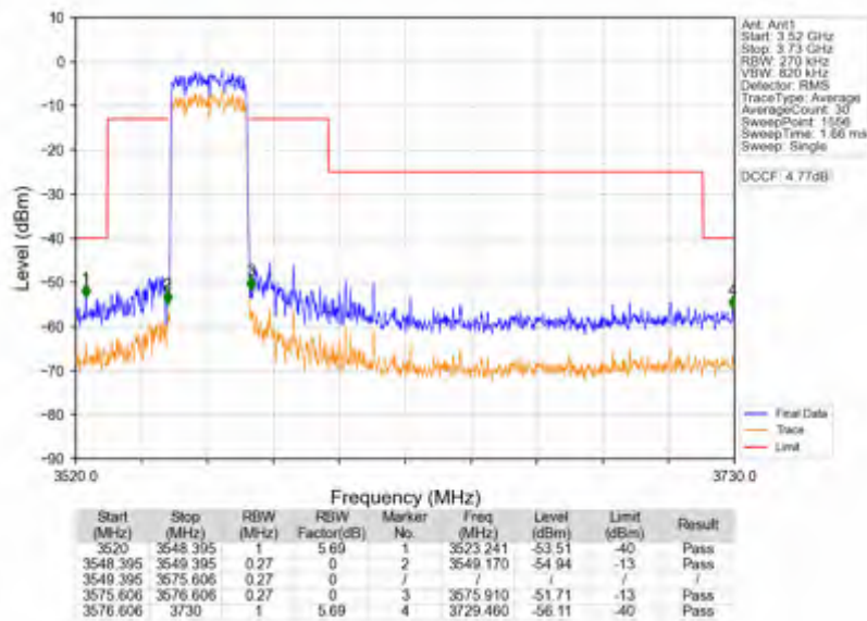
n78d_15kHz_SISO_NTNV_25MHz_CP-OFDM QPSK_3562.5MHz_Outer_Full
