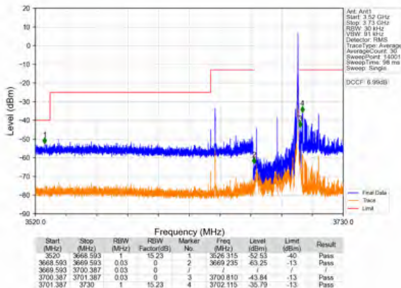
n78d_15kHz_SISO_NTNV_30MHz_DFT-s-OFDM_QPSK_3684.99MHz_Inner_1RB_Right
