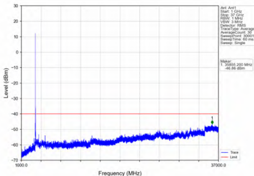
n78d_15kHz_SISO_NTNV_30MHz_CP-OFDM_QPSK_3625.005MHz_Edge_1RB_Left
