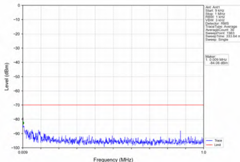
n78d_15kHz_SISO_NTNV_30MHz_DFT-s-OFDM QPSK_3565.005MHz_Outer_Full
