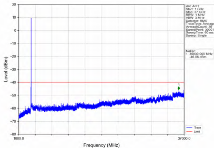
n78d_15kHz_SISO_NTNV_30MHz_DFT-s-OFDM QPSK_3684.99MHz_Inner_1RB_Right
