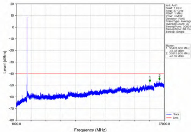
n78d_15kHz_SISO_NTNV_25MHz_DFT-s-OFDM QPSK_3687.495MHz_Edge_1RB_Right
