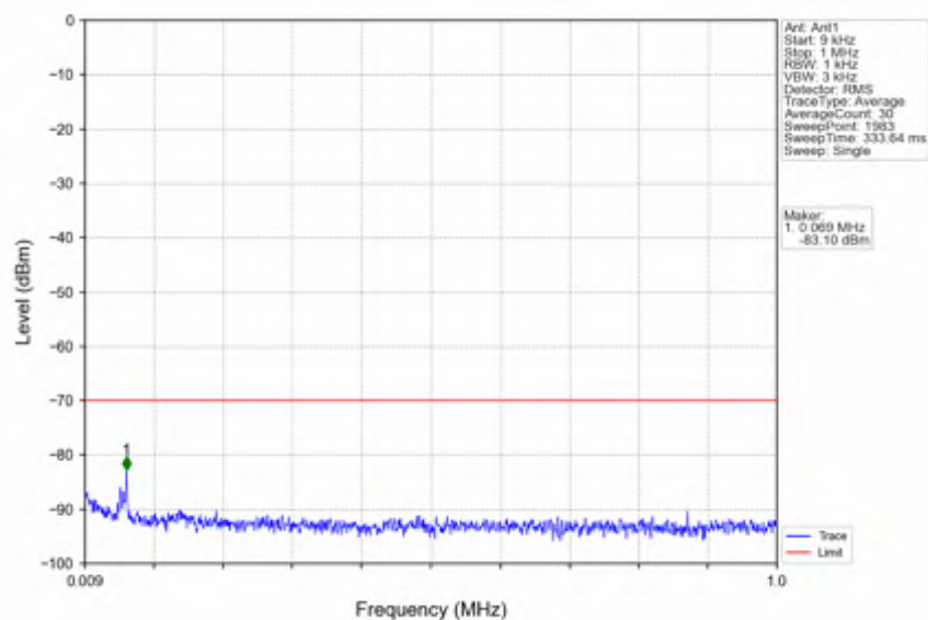
n78d_15kHz_SISO_NTNV_30MHz_DFT-s-OFDM_PI/2_BPSK_3565.005MHz_Edge_1RB_Left
