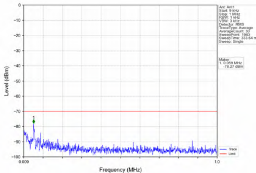
n78d_15kHz_SISO_NTNV_25MHz_CP-OFDM QPSK_3562.5MHz_Edge_1RB_Left
