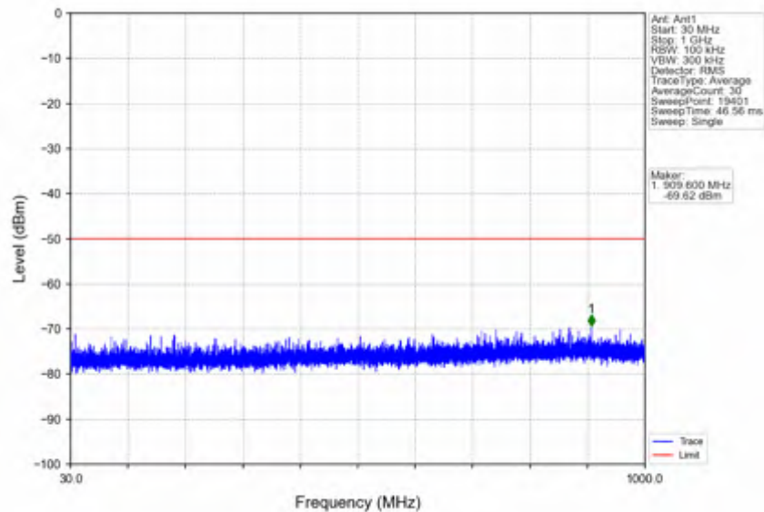
n78d_15kHz_SISO_NTNV_25MHz_CP-OFDM_QPSK_3625.005MHz_Edge_1RB_Left
