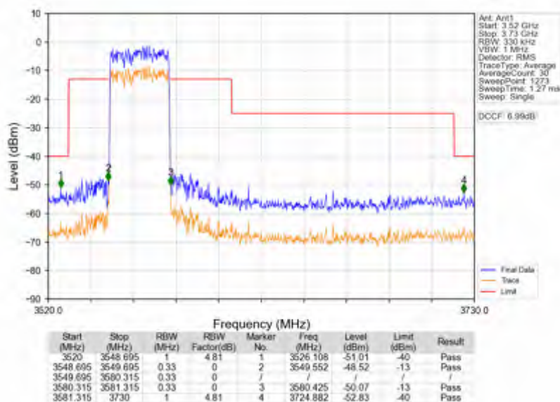
n78d_15kHz_SISO_NTNV_30MHz_CP-OFDM QPSK_3565.005MHz_Outer_Full
