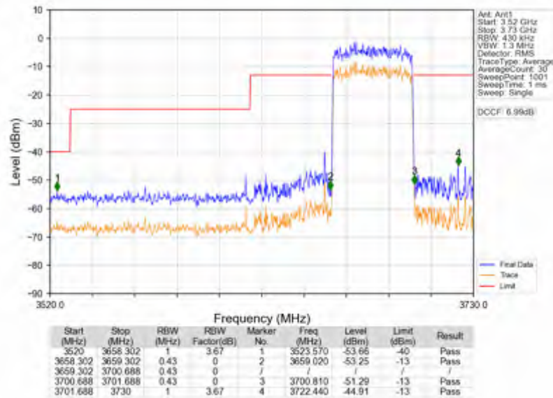
n78d_15kHz_SISO_NTNV_40MHz_DFT-s-OFDM QPSK_3679.995MHz_Outer_Full
