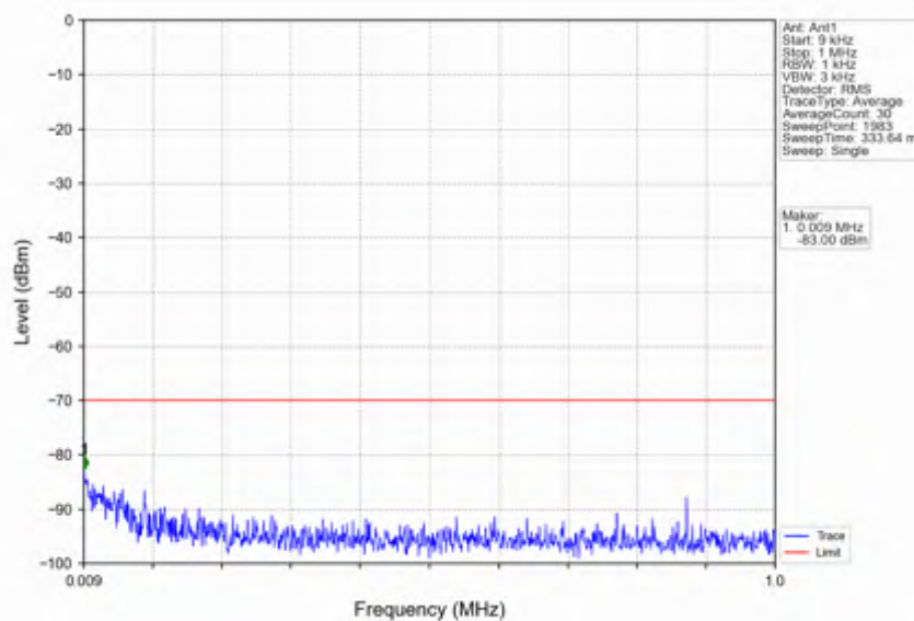
n78d_15kHz_SISO_NTNV_30MHz_CP-OFDM_QPSK_3565.005MHz_Inner_1RB_Left
