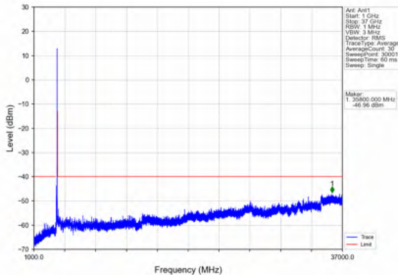
n78d_15kHz_SISO_NTNV_50MHz_DFT-s-OFDM QPSK_3675MHz_Edge_1RB_Right
