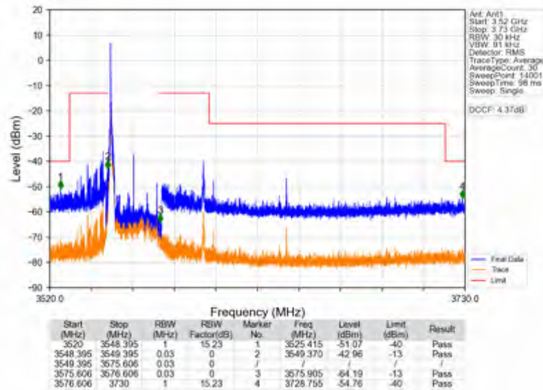
n78d_15kHz_SISO_NTNV_25MHz_CP-OFDM QPSK_3562.5MHz_Inner_1RB_Left
