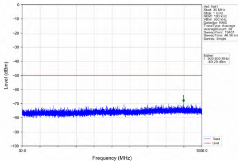
n78d_15kHz_SISO_NTNV_30MHz_DFT-s-OFDM_QPSK_3625.005MHz_Edge_1RB_Left
