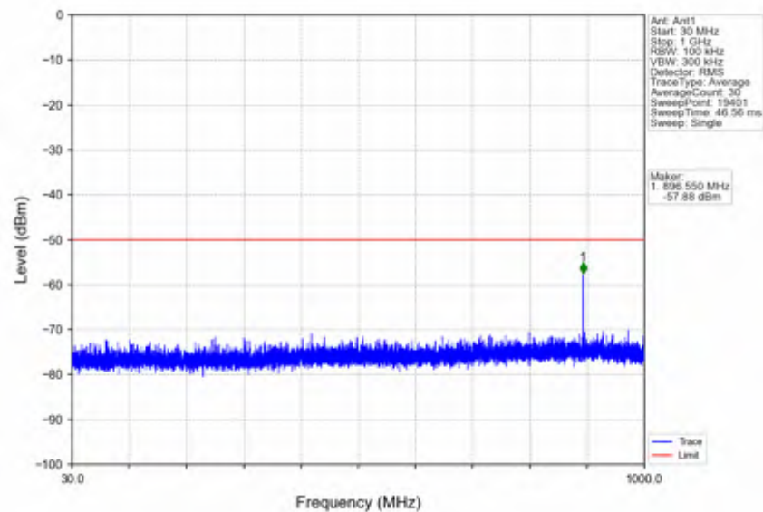
n78d_15kHz_SISO_NTNV_30MHz_DFT-s-OFDM QPSK_3684.99MHz_Inner_1RB_Right
