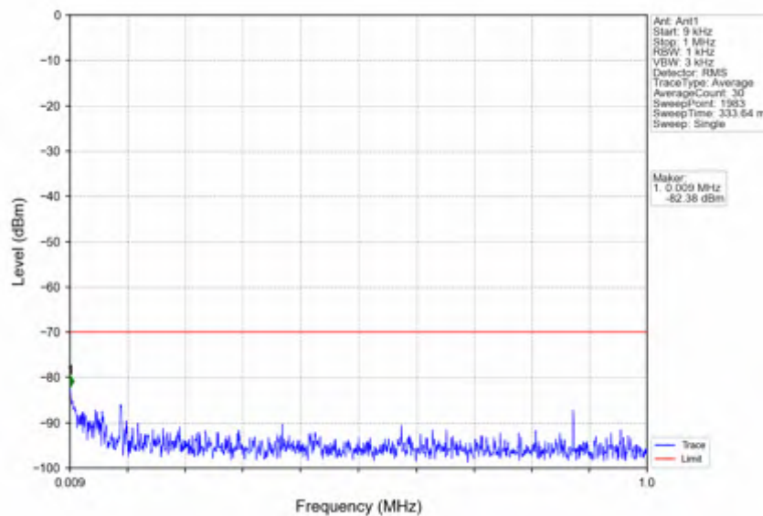
n78d_15kHz_SISO_NTNV_50MHz_DFT-s-OFDM_QPSK_3575.01MHz_Outer_Full
