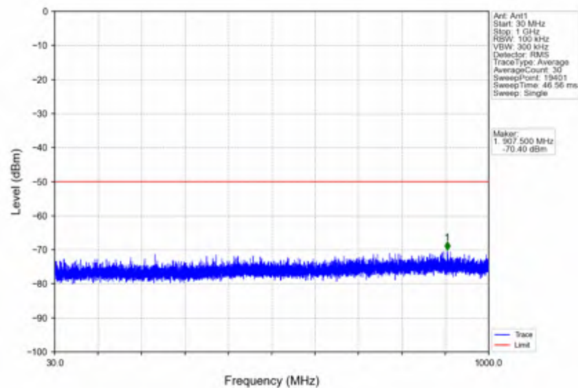
n78d_15kHz_SISO_NTNV_25MHz_DFT-s-OFDM_QPSK_3562.5MHz_Outer_Full
