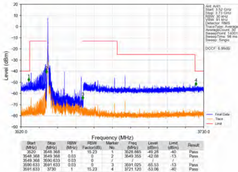
n78d_15kHz_SISO_NTNV_40MHz_DFT-s-OFDM_QPSK_3570MHz_Inner_1RB_Left
