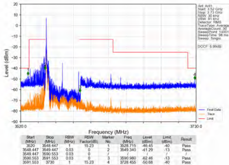
n78d_15kHz_SISO_NTNV_40MHz_CP-OFDM_QPSK_3570MHz_Edge_1RB_Left
