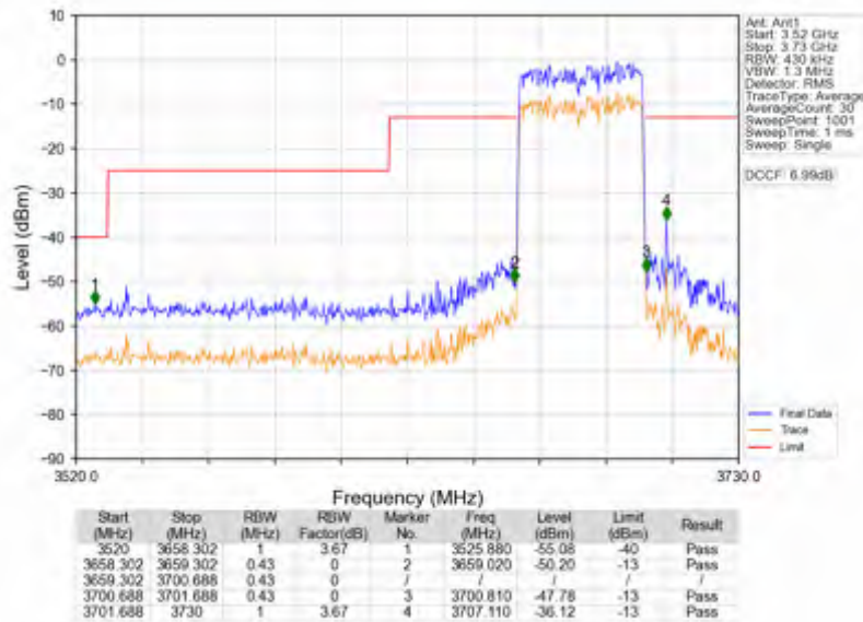
n78d_15kHz_SISO_NTNV_40MHz_CP-OFDM QPSK_3679.995MHz_Outer_Full
