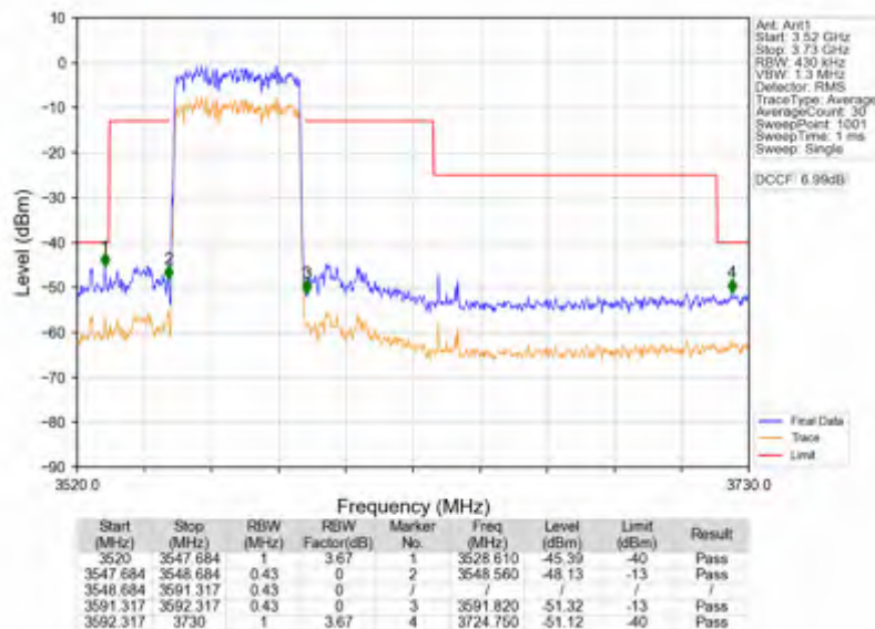
n78d_15kHz_SISO_NTNV_40MHz_DFT-s-OFDM PI/2 BPSK_3570MHz_Outer_Full
