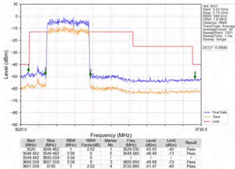
n78d_15kHz_SISO_NTNV_50MHz_DFT-s-OFDM_PI/2_BPSK_3575.01MHz_Outer_Full
