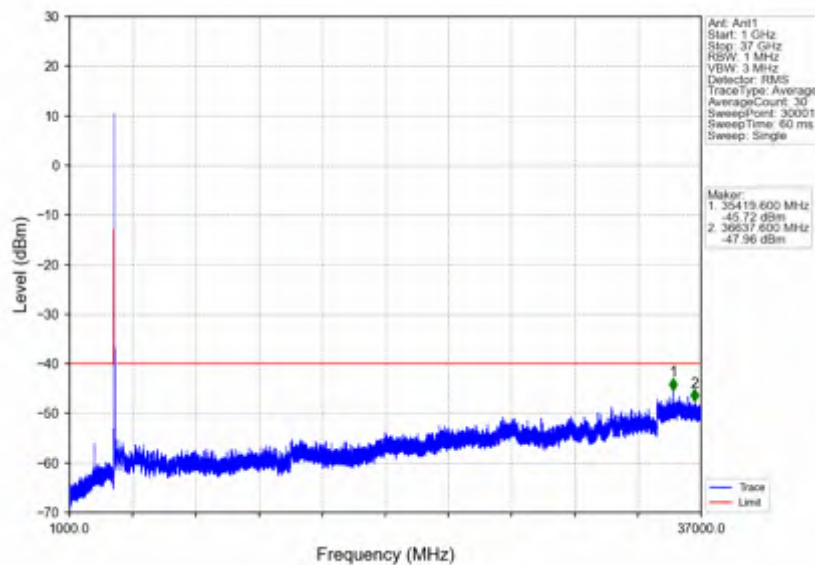
n78d_15kHz_SISO_NTNV_40MHz_CP-OFDM QPSK_3625.005MHz_Edge_1RB_Left
