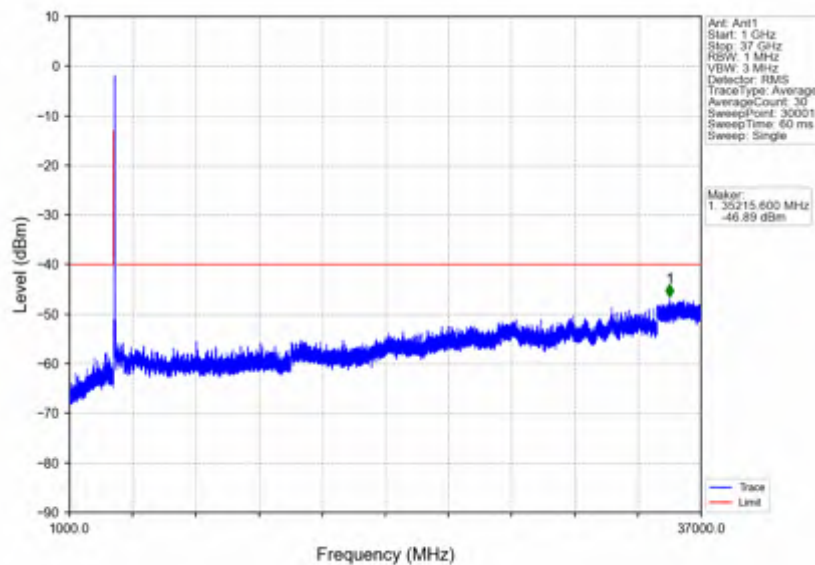
n78d_15kHz_SISO_NTNV_40MHz_DFT-s-OFDM_QPSK_3570MHz_Inner_1RB_Left
