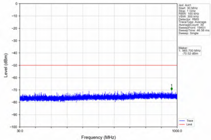
n78d_15kHz_SISO_NTNV_25MHz_CP-OFDM QPSK_3562.5MHz_Inner_1RB_Left
