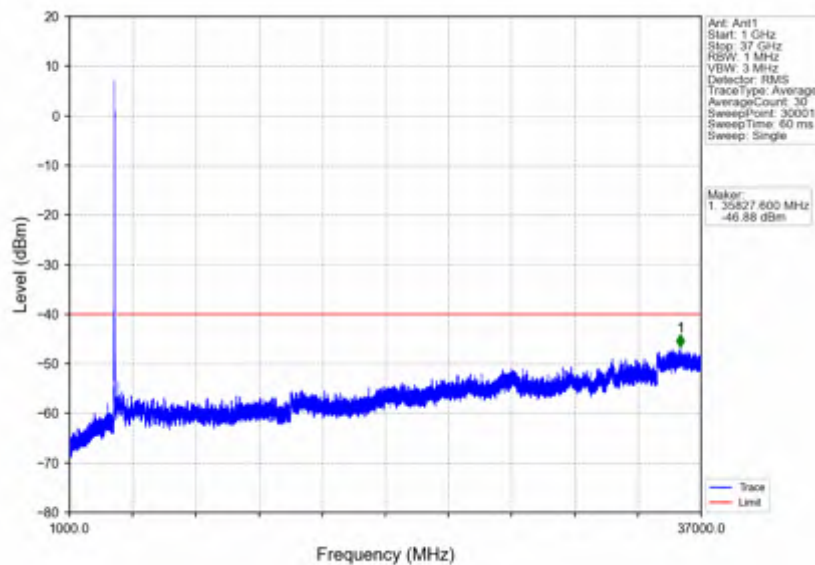
n78d_15kHz_SISO_NTNV_25MHz_DFT-s-OFDM QPSK_3562.5MHz_Inner_1RB_Left
