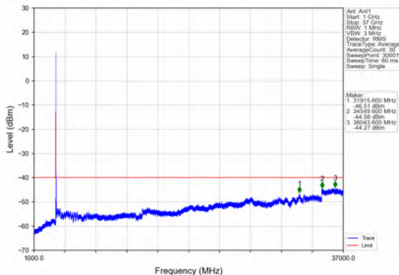
n78d_15kHz_SISO_NTNV_40MHz_DFT-s-OFDM PI/2 BPSK_3570MHz_Outer_Full
