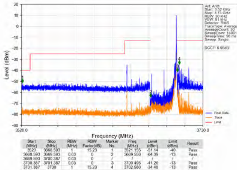
n78d_15kHz_SISO_NTNV_30MHz_DFT-s-OFDM QPSK_3684.99MHz_Edge_1RB_Right
