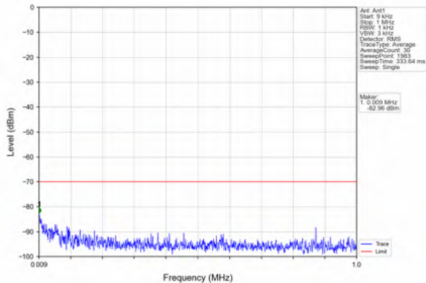
n78d_15kHz_SISO_NTNV_30MHz_DFT-s-OFDM QPSK_3565.005MHz_Edge_1RB_Left
