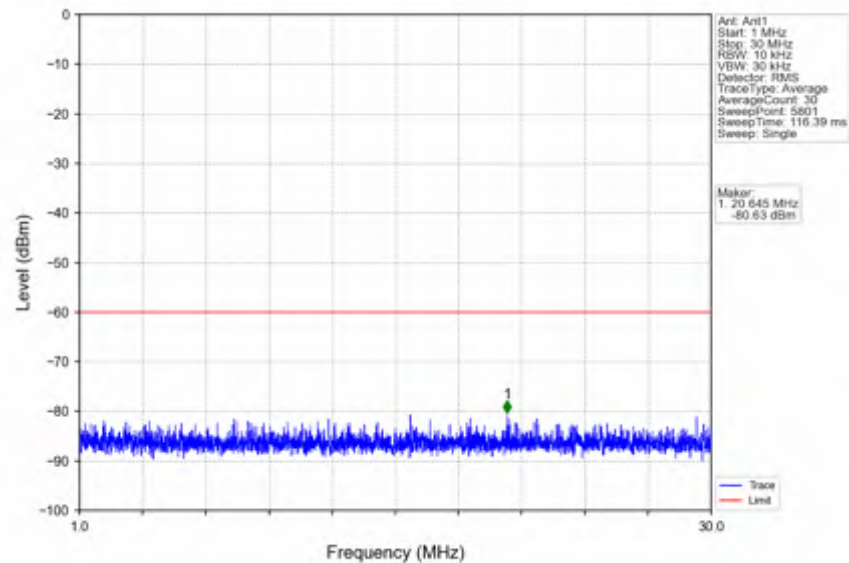
n78d_15kHz_SISO_NTNV_30MHz_CP-OFDM_QPSK_3625.005MHz_Edge_1RB_Left
