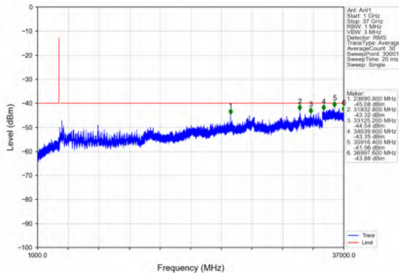
n78d_15kHz_SISO_NTNV_40MHz_CP-OFDM_QPSK_3570MHz_Outer_Full
