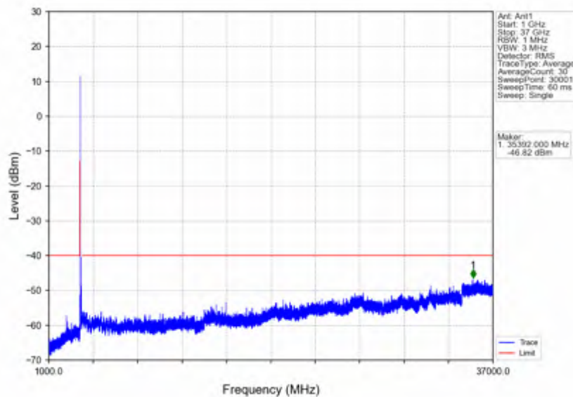
n78d_15kHz_SISO_NTNV_40MHz_CP-OFDM QPSK_3570MHz_Outer_Full
