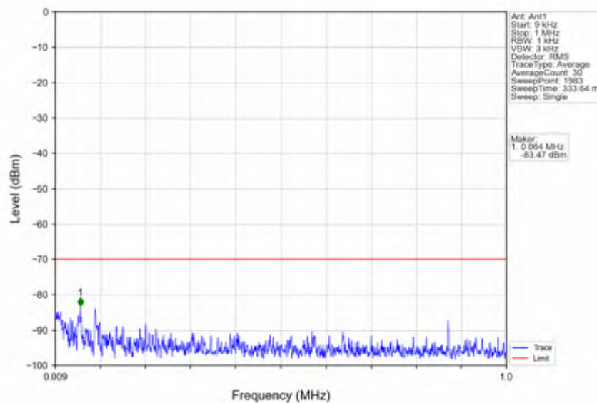
n78d_15kHz_SISO_NTNV_25MHz_DFT-s-OFDM QPSK_3687.495MHz_Outer_Full
