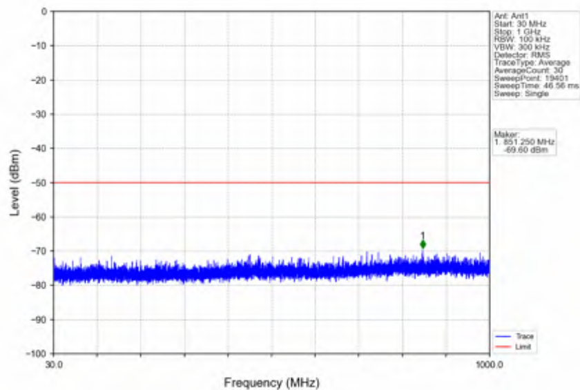
n78d_15kHz_SISO_NTNV_30MHz_CP-OFDM QPSK_3684.99MHz_Outer_Full
