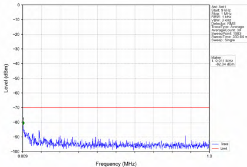
n78d_15kHz_SISO_NTNV_40MHz_DFT-s-OFDM_QPSK_3570MHz_Outer_Full
