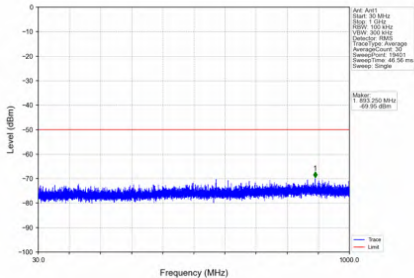
n78d_15kHz_SISO_NTNV_25MHz_DFT-s-OFDM_QPSK_3562.5MHz_Edge_1RB_Left
