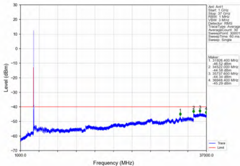
n78d_15kHz_SISO_NTNV_50MHz_DFT-s-OFDM_PI/2_BPSK_3575.01MHz_Outer_Full
