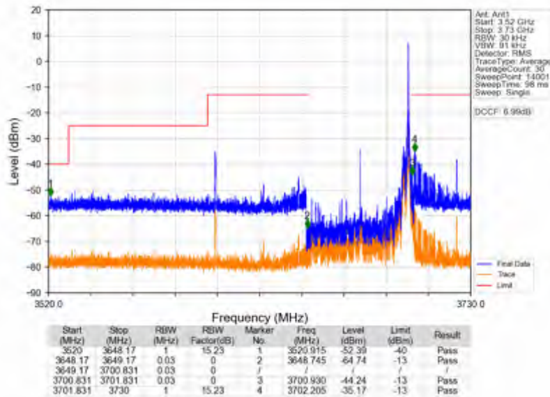
n78d_15kHz_SISO_NTNV_50MHz_DFT-s-OFDM QPSK_3675MHz_Inner_1RB_Right
