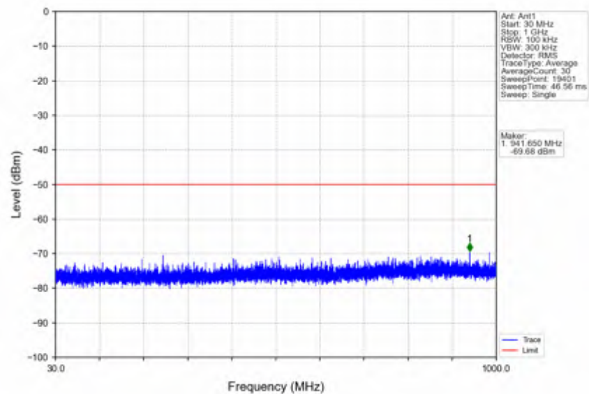
n78d_15kHz_SISO_NTNV_40MHz_DFT-s-OFDM_QPSK_3570MHz_Outer_Full
