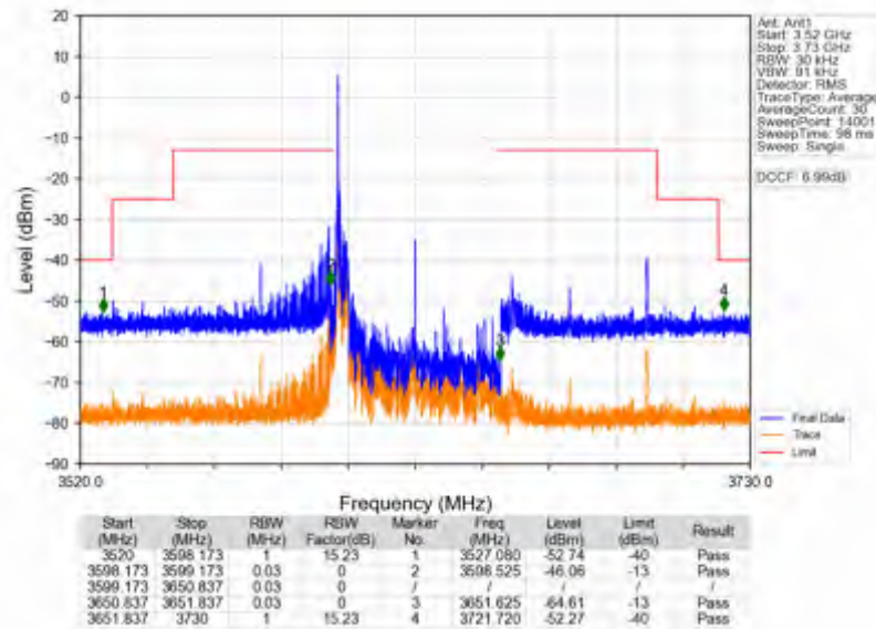
n78d_15kHz_SISO_NTNV_50MHz_DFT-s-OFDM QPSK_3625.005MHz_Edge_1RB_Left
