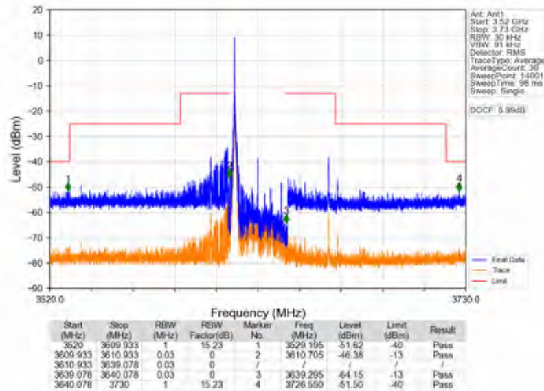
n78d_15kHz_SISO_NTNV_25MHz_DFT-s-OFDM QPSK_3625.005MHz_Edge_1RB_Left
