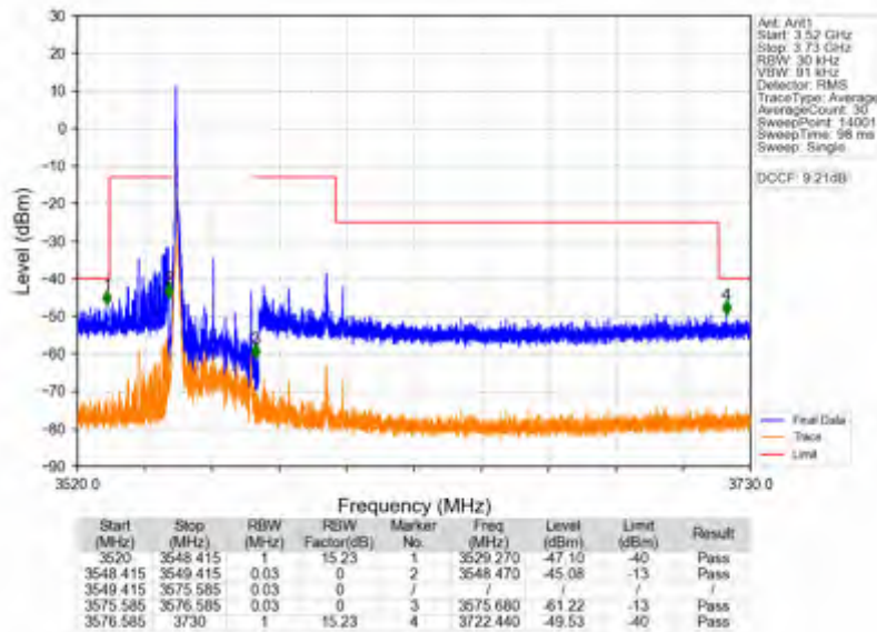
n78d_15kHz_SISO_NTNV_25MHz_DFT-s-OFDM QPSK_3562.5MHz_Inner_1RB_Left
