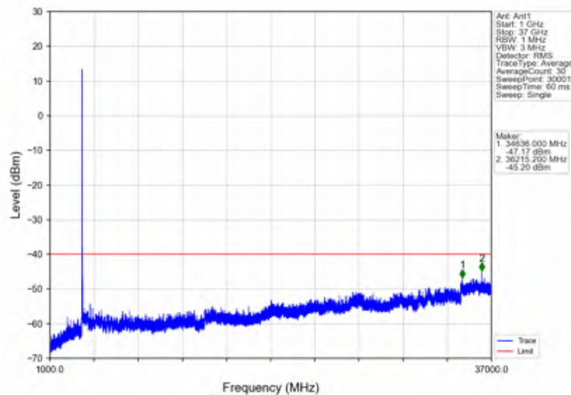
n78d_15kHz_SISO_NTNV_30MHz_DFT-s-OFDM QPSK_3684.99MHz_Edge_1RB_Right
