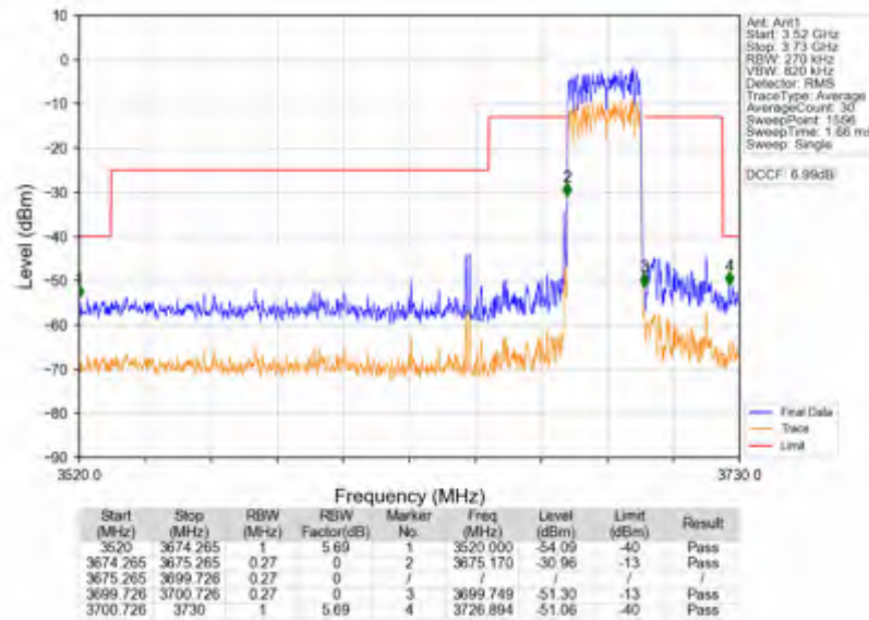
n78d_15kHz_SISO_NTNV_25MHz_DFT-s-OFDM QPSK_3687.495MHz_Outer_Full
