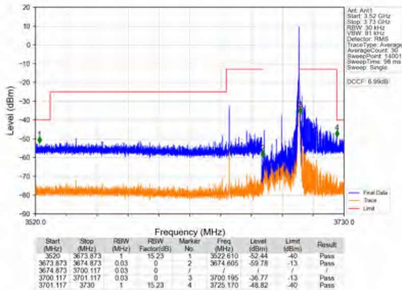
n78d_15kHz_SISO_NTNV_25MHz_DFT-s-OFDM QPSK_3687.495MHz_Edge_1RB_Right
