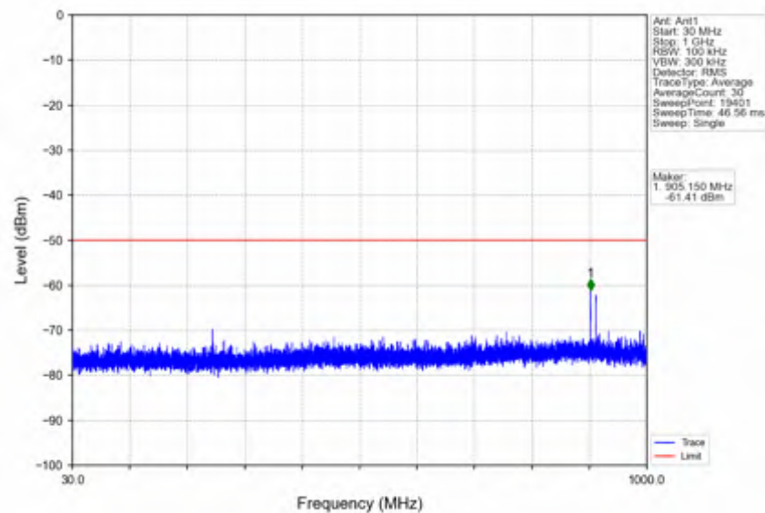
n78d_15kHz_SISO_NTNV_50MHz_CP-OFDM QPSK_3675MHz_Edge_1RB_Right
