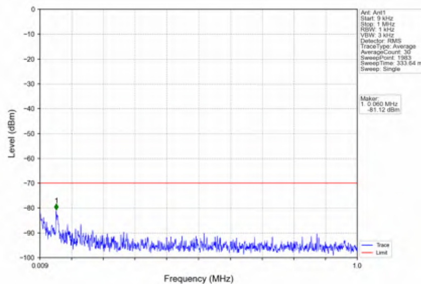
n78d_15kHz_SISO_NTNV_25MHz_CP-OFDM QPSK_3562.5MHz_Inner_1RB_Left
