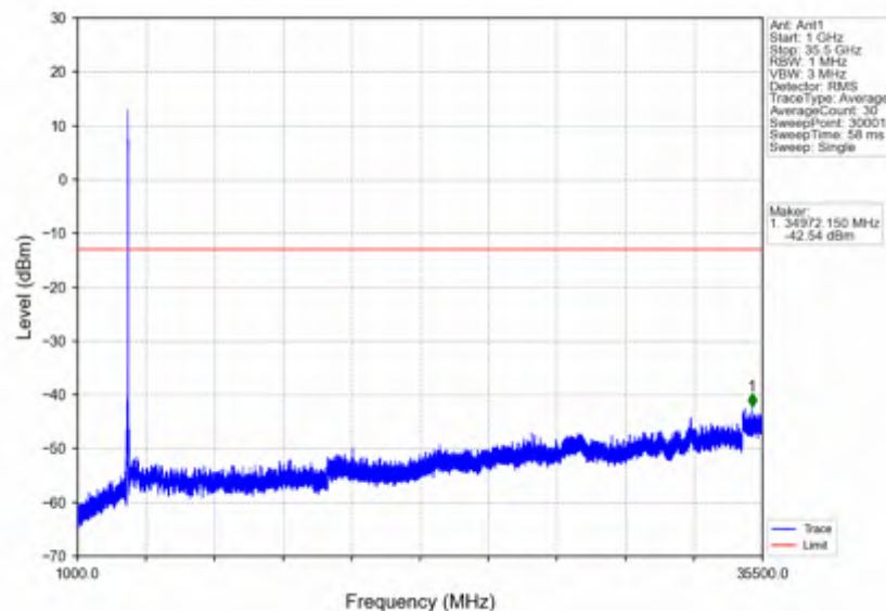
n78e_15kHz_SISO_NTNV_25MHz_DFT-s-OFDM QPSK_3537.495MHz_Inner_1RB_Right
