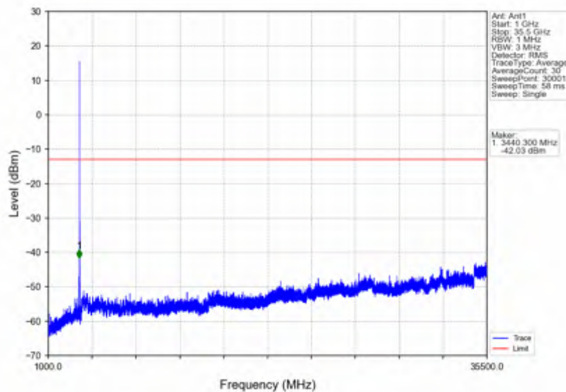
n78e_15kHz_SISO_NTNV_20MHz_CP-OFDM QPSK_3460.005MHz_Outer_Full
