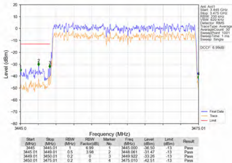
n78e_15kHz_SISO_NTNV_25MHz_CP-OFDM QPSK_3462.51MHz_Outer_Full
