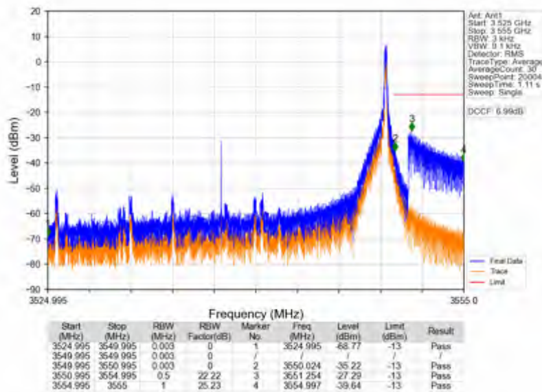
n78e_15kHz_SISO_NTNV_25MHz_DFT-s-OFDM QPSK_3537.495MHz_Edge_1RB_Right
