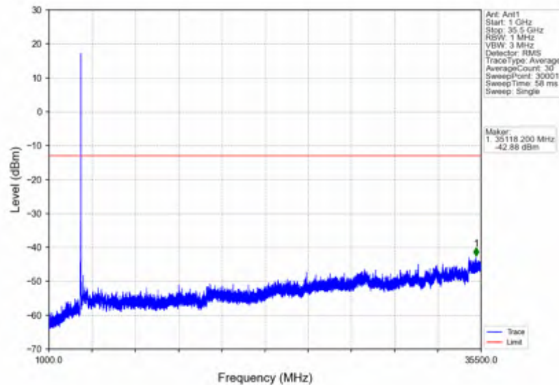
n78e_15kHz_SISO_NTNV_30MHz_DFT-s-OFDM QPSK_3534.99MHz_Edge_1RB_Right
