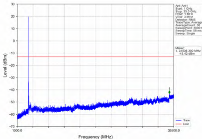
n78e_15kHz_SISO_NTNV_25MHz_DFT-s-OFDM QPSK_3537.495MHz_Edge_1RB_Right
