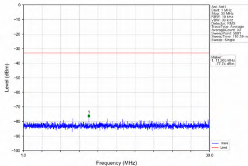
n78e_15kHz_SISO_NTNV_20MHz_CP-OFDM_QPSK_3540MHz_Inner_1RB_Right
