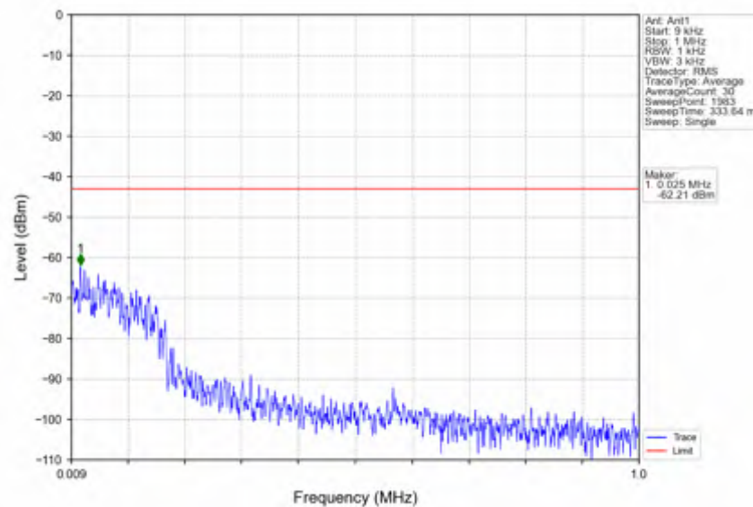
n78e_15kHz_SISO_NTNV_20MHz_CP-OFDM_QPSK_3540MHz_Edge_1RB_Right
