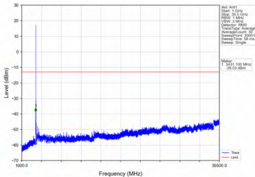
n78e_15kHz_SISO_NTNV_25MHz_CP-OFDM QPSK_3462.51MHz_Outer_Full
