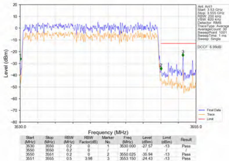
n78e_15kHz_SISO_NTNV_20MHz_CP-OFDM QPSK_3540MHz_Outer_Full
