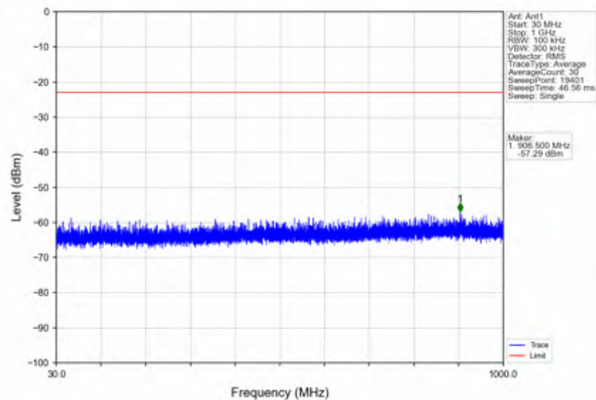
n78e_15kHz_SISO_NTNV_25MHz_CP-OFDM_QPSK_3499.995MHz_Edge_1RB_Left
