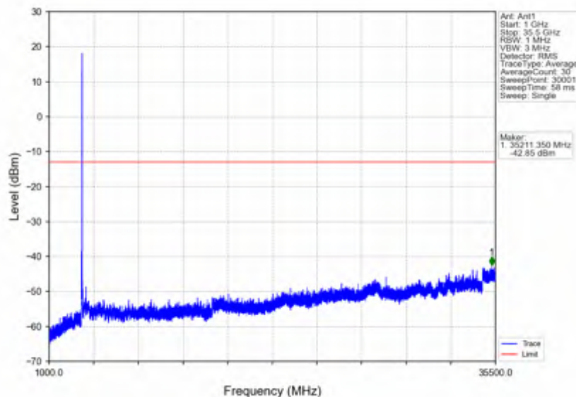
n78e_15kHz_SISO_NTNV_25MHz_CP-OFDM QPSK_3537.495MHz_Outer_Full
