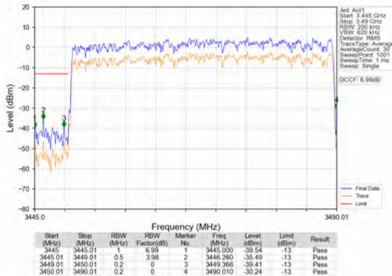
n78e_15kHz_SISO_NTNV_40MHz_DFT-s-OFDM_QPSK_3470.01MHz_Outer_Full
