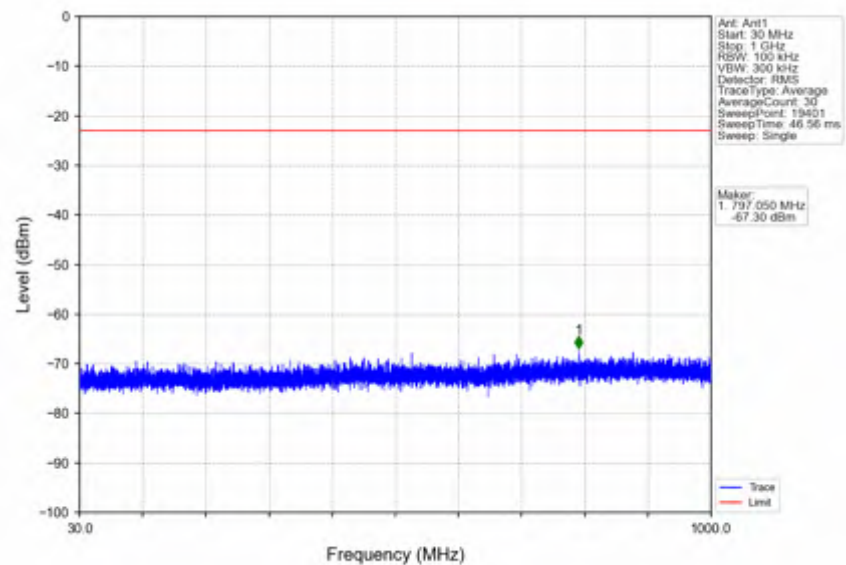
n78e_15kHz_SISO_NTNV_30MHz_DFT-s-OFDM_QPSK_3465MHz_Outer_Full
