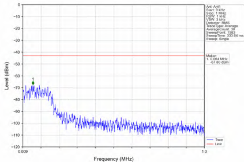
n78e_15kHz_SISO_NTNV_20MHz_DFT-s-OFDM QPSK_3460.005MHz_Edge_1RB_Left
