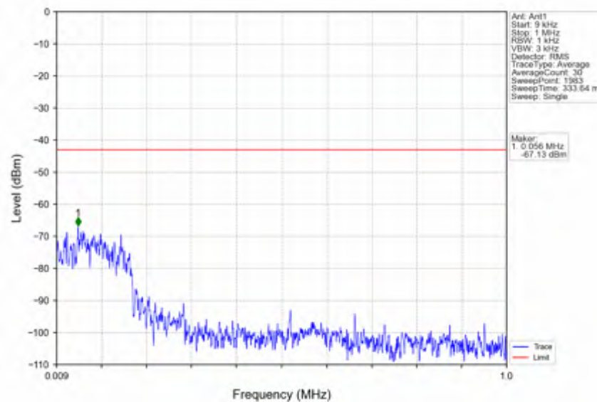
n78e_15kHz_SISO_NTNV_25MHz_DFT-s-OFDM QPSK_3499.995MHz_Edge_1RB_Left
