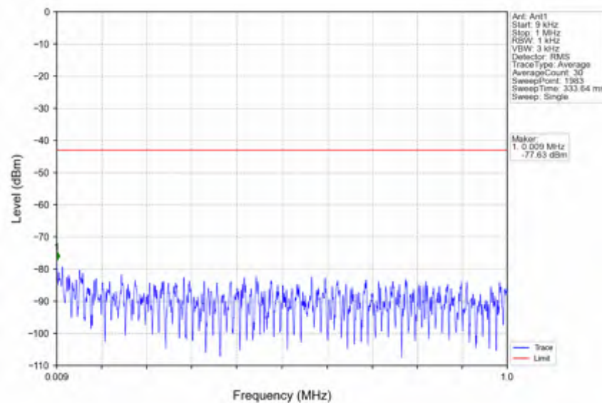
n78e_15kHz_SISO_NTNV_25MHz_CP-OFDM_QPSK_3537.495MHz_Outer_Full
