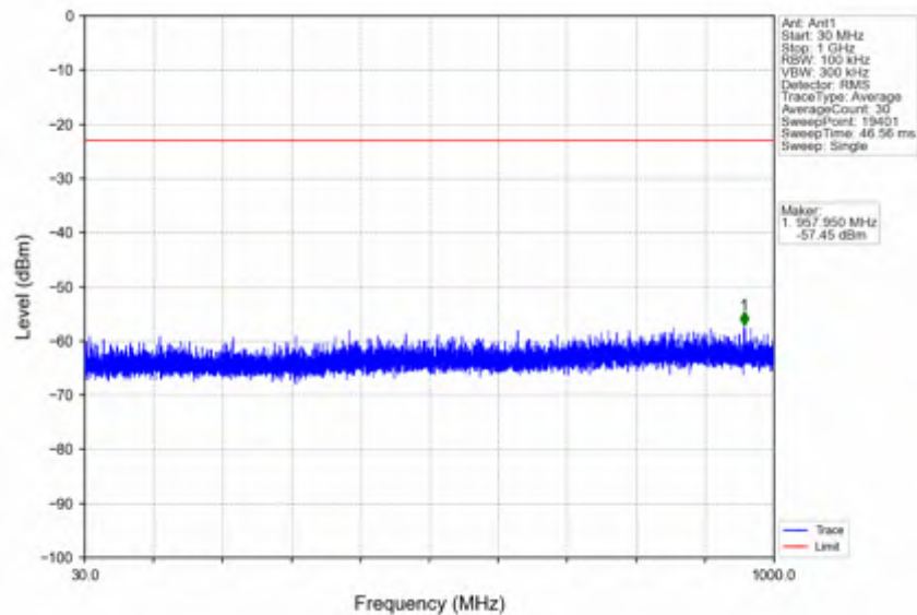
n78e_15kHz_SISO_NTNV_20MHz_DFT-s-OFDM QPSK_3540MHz_Edge_1RB_Right
