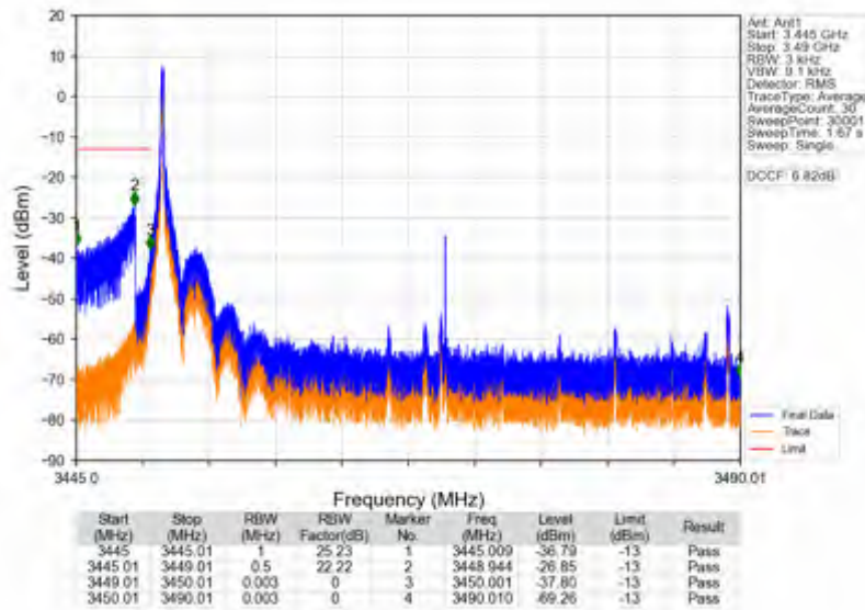
n78e_15kHz_SISO_NTNV_40MHz_DFT-s-OFDM_QPSK_3470.01MHz_Inner_1RB_Left
