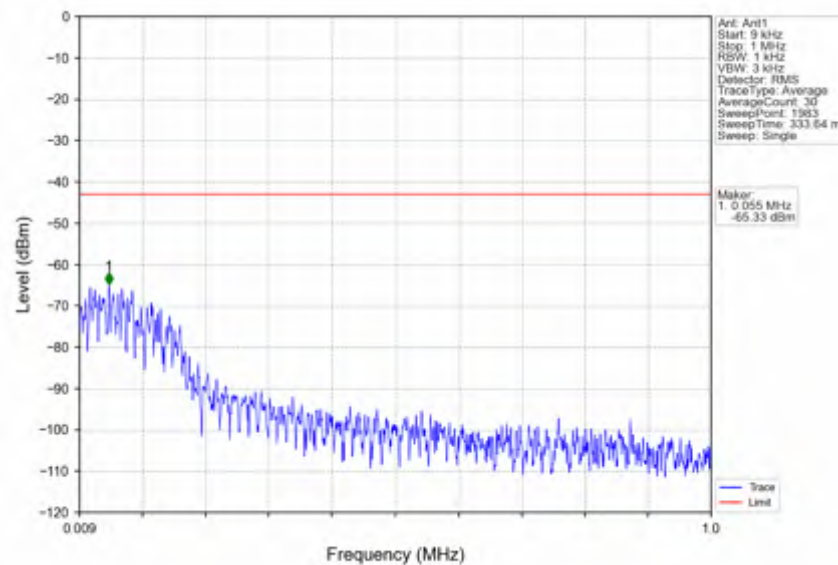
n78e_15kHz_SISO_NTNV_20MHz_CP-OFDM_QPSK_3540MHz_Inner_1RB_Right
