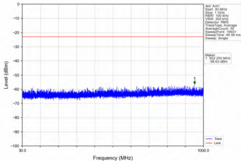
n78e_15kHz_SISO_NTNV_30MHz_CP-OFDM QPSK_3534.99MHz_Edge_1RB_Right
