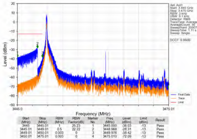
n78e_15kHz_SISO_NTNV_25MHz_DFT-s-OFDM_QPSK_3462.51MHz_Inner_1RB_Left
