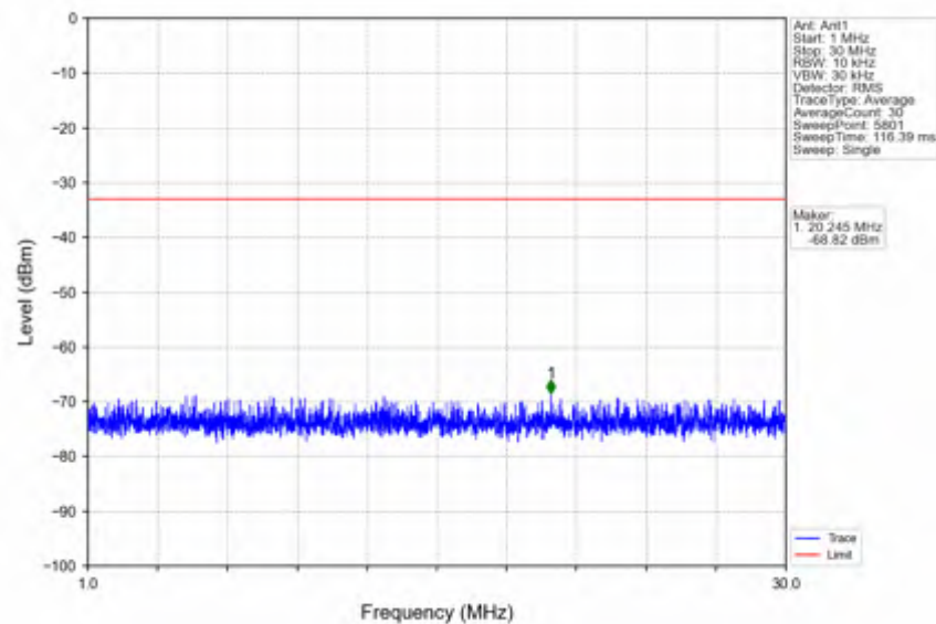
n78e_15kHz_SISO_NTNV_30MHz_DFT-s-OFDM QPSK_3499.995MHz_Edge_1RB_Left
