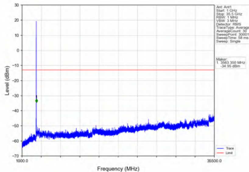
n78e_15kHz_SISO_NTNV_30MHz_DFT-s-OFDM_QPSK_3534.99MHz_Inner_1RB_Right
