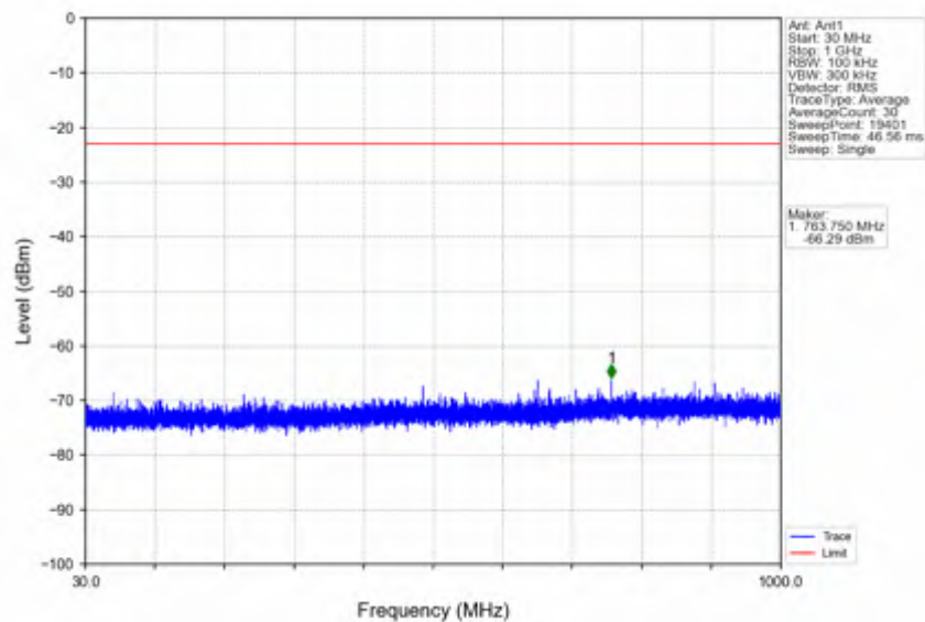
n78e_15kHz_SISO_NTNV_20MHz_CP-OFDM_QPSK_3540MHz_Outer_Full
