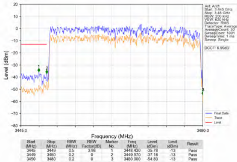
n78e_15kHz_SISO_NTNV_30MHz_CP-OFDM_QPSK_3465MHz_Outer_Full
