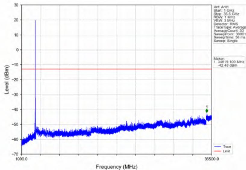
n78e_15kHz_SISO_NTNV_20MHz_DFT-s-OFDM QPSK_3540MHz_Edge_1RB_Right
