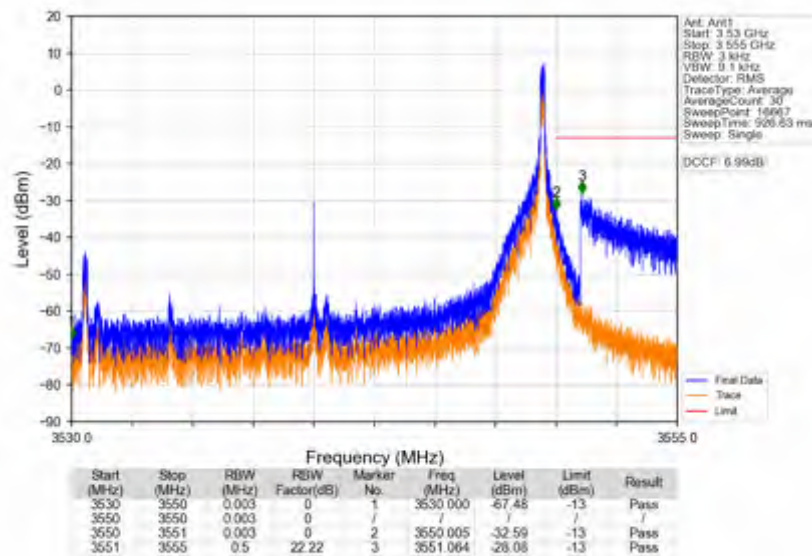
n78e_15kHz_SISO_NTNV_20MHz_DFT-s-OFDM QPSK_3540MHz_Edge_1RB_Right
