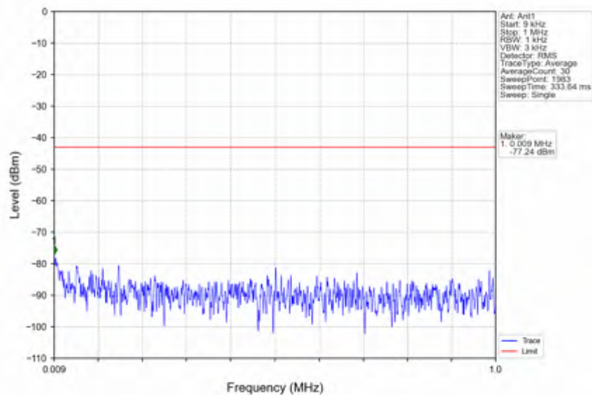
n78e_15kHz_SISO_NTNV_30MHz_CP-OFDM_QPSK_3465MHz_Outer_Full
