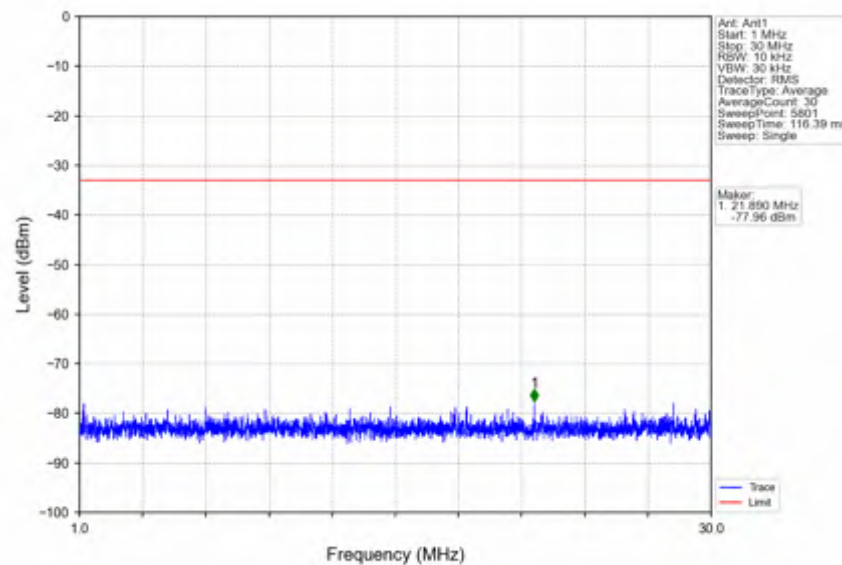
n78e_15kHz_SISO_NTNV_25MHz_CP-OFDM_QPSK_3462.51MHz_Outer_Full
