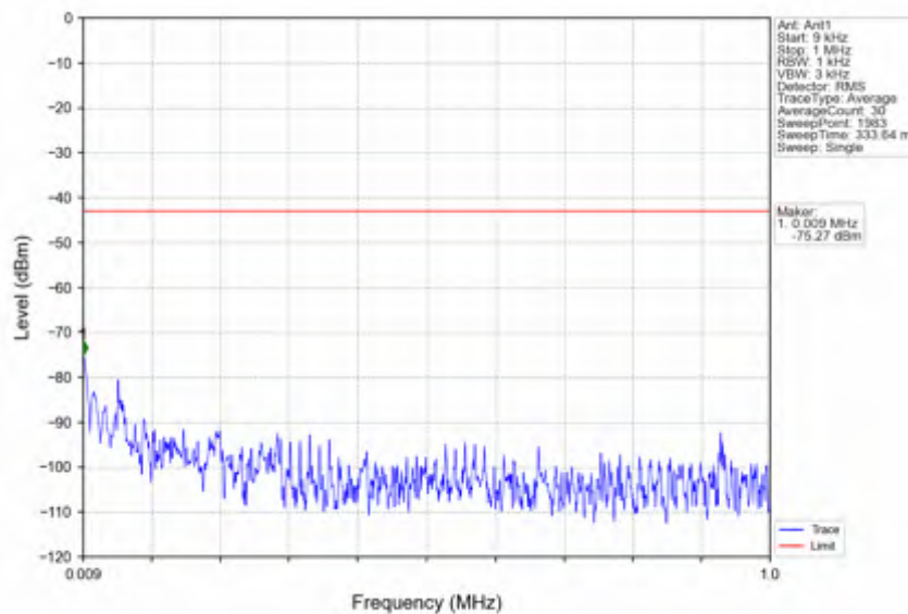
n78e_15kHz_SISO_NTNV_40MHz_DFT-s-OFDM_QPSK_3470.01MHz_Outer_Full
