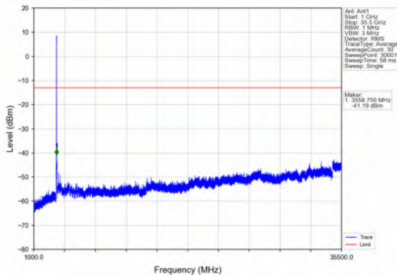
n78e_15kHz_SISO_NTNV_30MHz_DFT-s-OFDM_QPSK_3534.99MHz_Inner_1RB_Right
