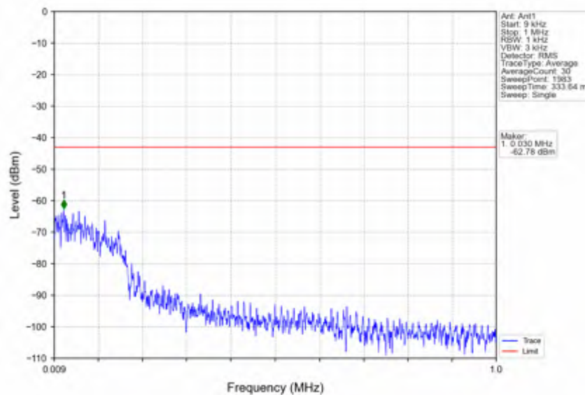
n78e_15kHz_SISO_NTNV_30MHz_CP-OFDM_QPSK_3465MHz_Edge_1RB_Left
