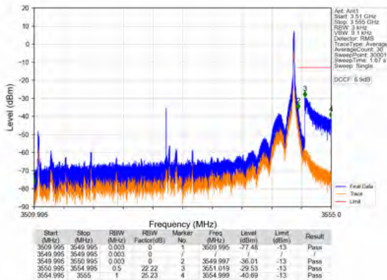
n78e_15kHz_SISO_NTNV_40MHz_DFT-s-OFDM_QPSK_3529.995MHz_Edge_1RB_Right
