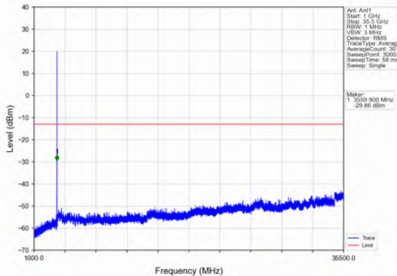
n78e_15kHz_SISO_NTNV_20MHz_DFT-s-OFDM QPSK_3540MHz_Edge_1RB_Right
