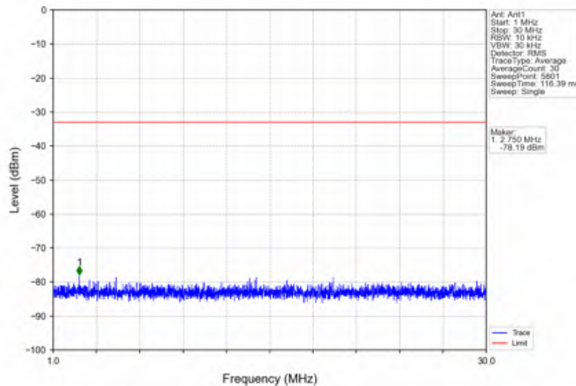
n78e_15kHz_SISO_NTNV_25MHz_DFT-s-OFDM_QPSK_3462.51MHz_Outer_Full
