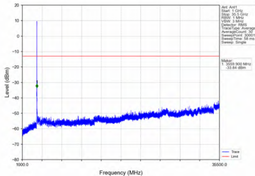
n78e_15kHz_SISO_NTNV_30MHz_CP-OFDM_QPSK_3534.99MHz_Outer_Full
