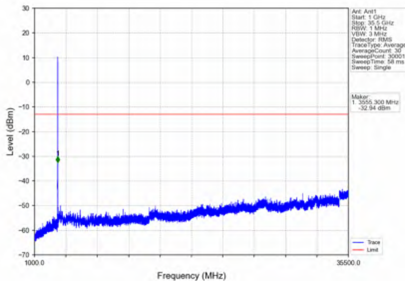
n78e_15kHz_SISO_NTNV_20MHz_CP-OFDM_QPSK_3540MHz_Outer_Full
