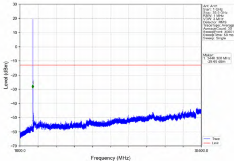
n78e_15kHz_SISO_NTNV_20MHz_DFT-s-OFDM QPSK_3460.005MHz_Edge_1RB_Left
