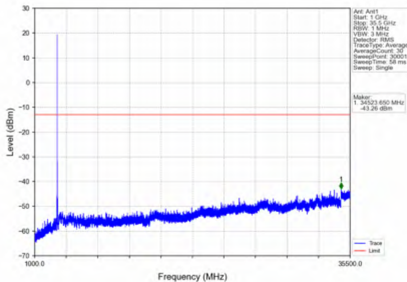
n78e_15kHz_SISO_NTNV_25MHz_DFT-s-OFDM_PI/2_BPSK_3462.51MHz_Outer_Full
