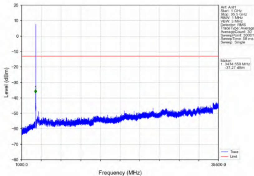
n78e_15kHz_SISO_NTNV_40MHz_DFT-s-OFDM_QPSK_3470.01MHz_Inner_1RB_Left
