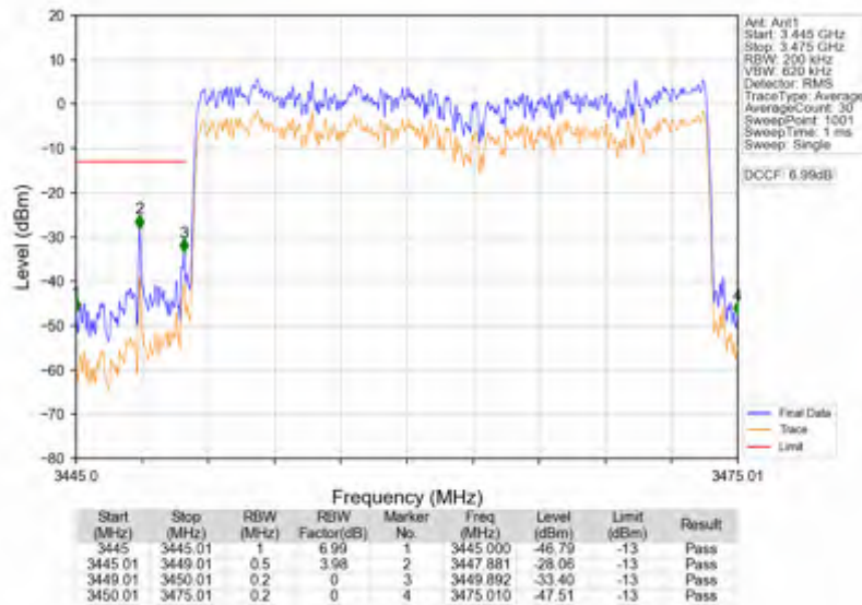
n78e_15kHz_SISO_NTNV_25MHz_DFT-s-OFDM_PI/2_BPSK_3462.51MHz_Outer_Full
