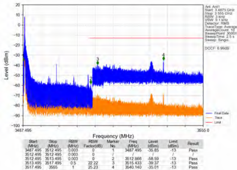
n78e_15kHz_SISO_NTNV_25MHz_CP-OFDM QPSK_3499.995MHz_Edge_1RB_Left
