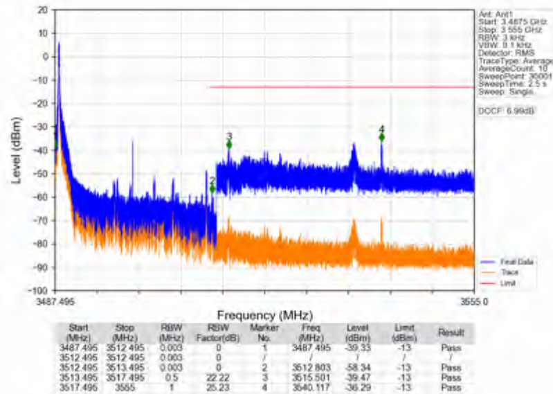
n78e_15kHz_SISO_NTNV_25MHz_DFT-s-OFDM QPSK_3499.995MHz_Edge_1RB_Left
