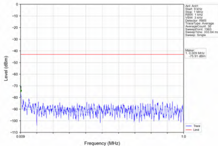
n78e_15kHz_SISO_NTNV_30MHz_CP-OFDM QPSK_3534.99MHz_Outer_Full
