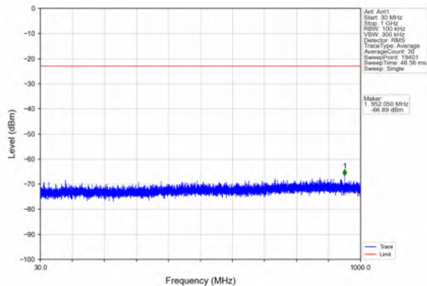
n78e_15kHz_SISO_NTNV_30MHz_DFT-s-OFDM_QPSK_3534.99MHz_Inner_1RB_Right
