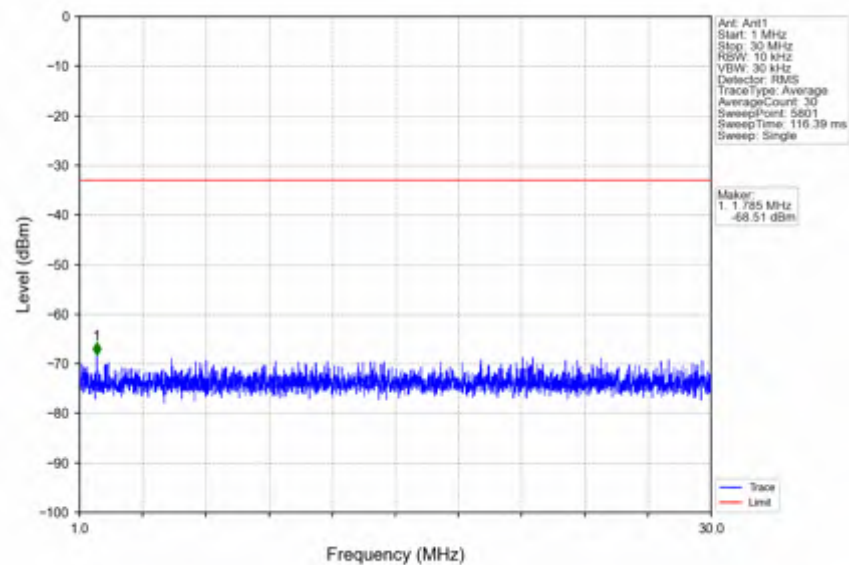
n78e_15kHz_SISO_NTNV_20MHz_DFT-s-OFDM_QPSK_3540MHz_Edge_1RB_Right
