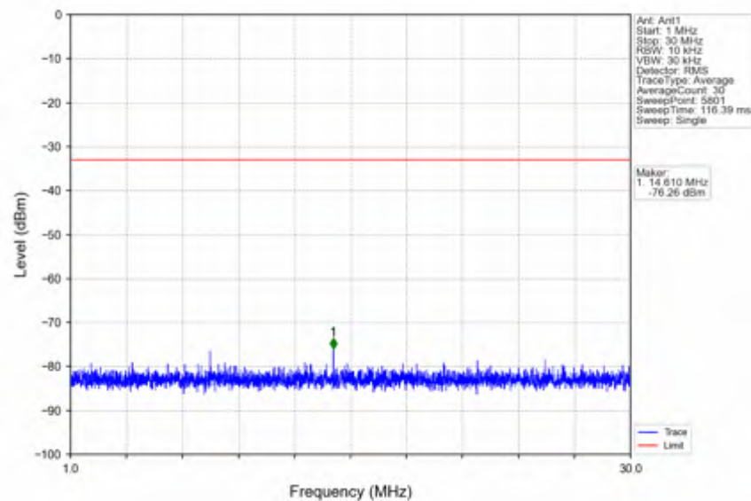
n78e_15kHz_SISO_NTNV_25MHz_DFT-s-OFDM QPSK_3537.495MHz_Outer_Full
