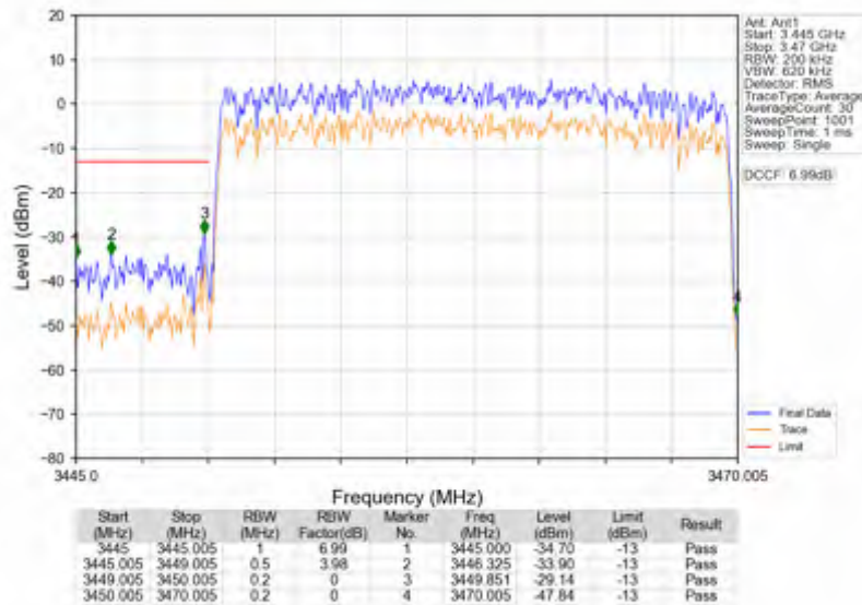
n78e_15kHz_SISO_NTNV_20MHz_CP-OFDM QPSK_3460.005MHz_Outer_Full
