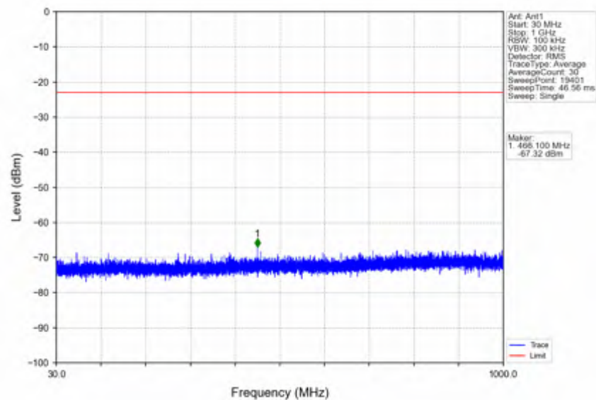
n78e_15kHz_SISO_NTNV_25MHz_DFT-s-OFDM QPSK_3537.495MHz_Outer_Full
