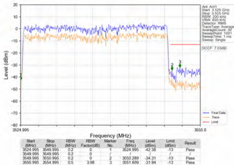
n78e_15kHz_SISO_NTNV_25MHz_CP-OFDM QPSK_3537.495MHz_Outer_Full
