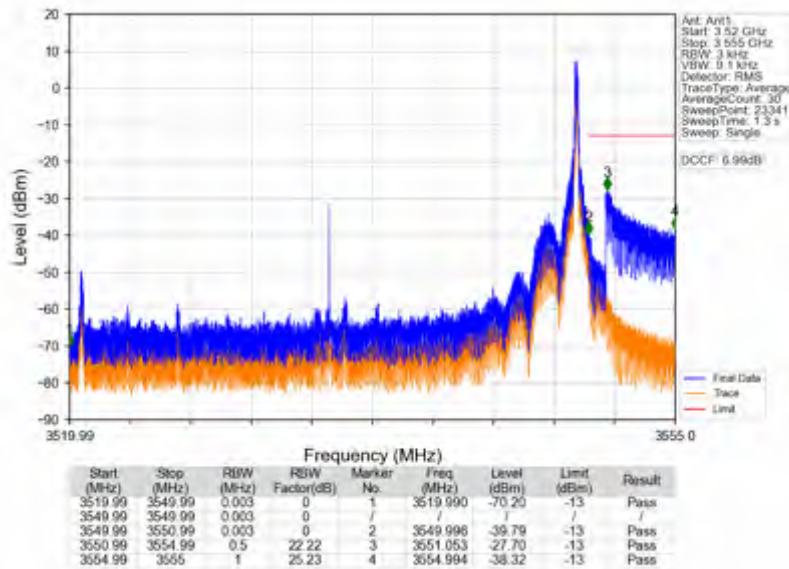
n78e_15kHz_SISO_NTNV_30MHz_DFT-s-OFDM_QPSK_3534.99MHz_Edge_1RB_Right
