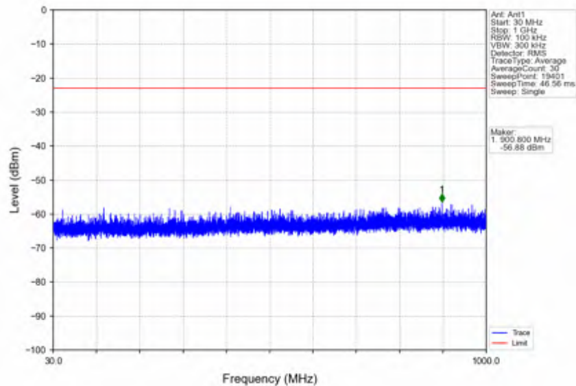
n78e_15kHz_SISO_NTNV_30MHz_DFT-s-OFDM QPSK_3534.99MHz_Edge_1RB_Right
