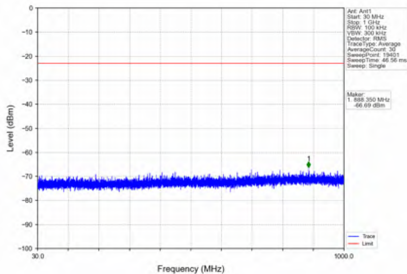
n78e_15kHz_SISO_NTNV_30MHz_DFT-s-OFDM_QPSK_3534.99MHz_Outer_Full
