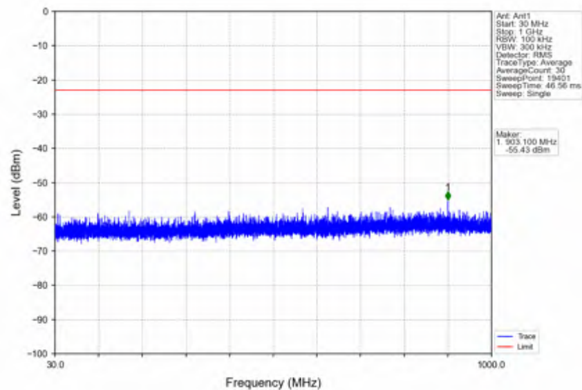
n78e_15kHz_SISO_NTNV_30MHz_DFT-s-OFDM QPSK_3499.995MHz_Edge_1RB_Left
