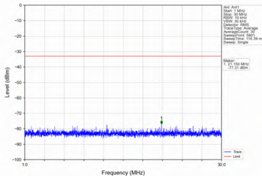
n78e_15kHz_SISO_NTNV_20MHz_DFT-s-OFDM_QPSK_3540MHz_Outer_Full
