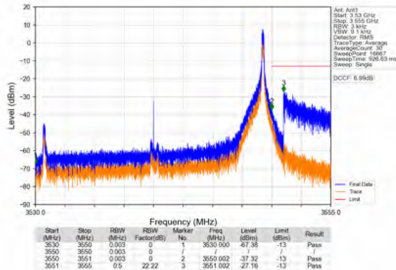
n78e_15kHz_SISO_NTNV_20MHz_CP-OFDM_QPSK_3540MHz_Inner_1RB_Right
