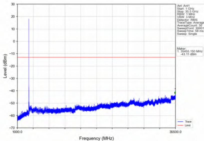
n78e_15kHz_SISO_NTNV_40MHz_DFT-s-OFDM_QPSK_3529.995MHz_Edge_1RB_Right
