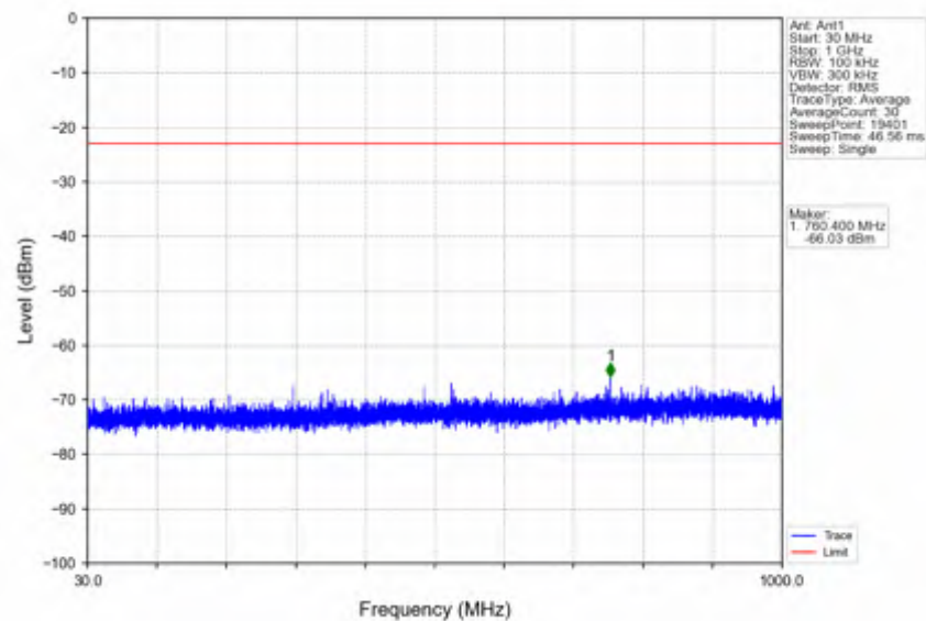
n78e_15kHz_SISO_NTNV_20MHz_DFT-s-OFDM QPSK_3540MHz_Inner_1RB_Right
