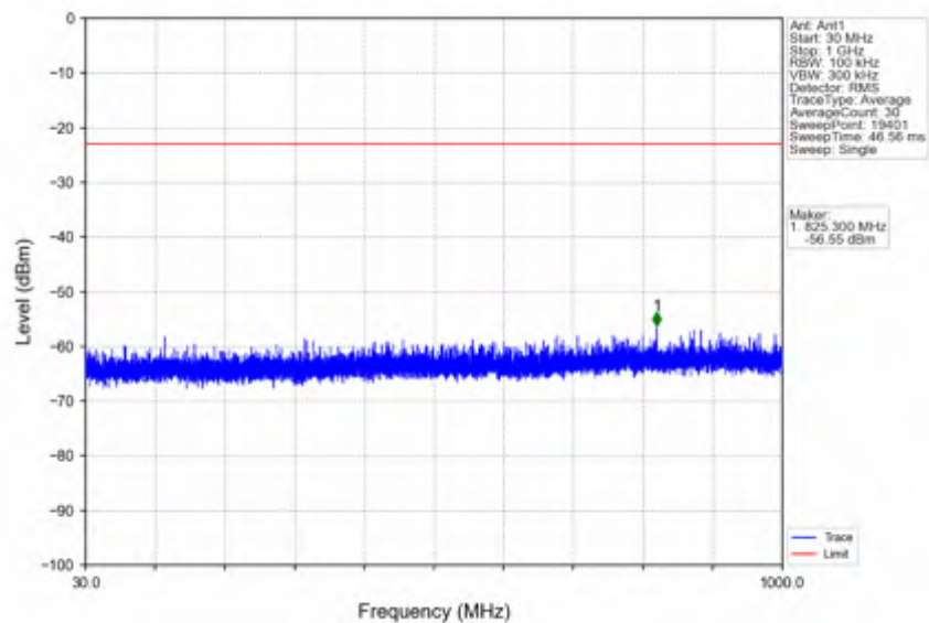
n78e_15kHz_SISO_NTNV_30MHz_CP-OFDM_QPSK_3465MHz_Edge_1RB_Left
