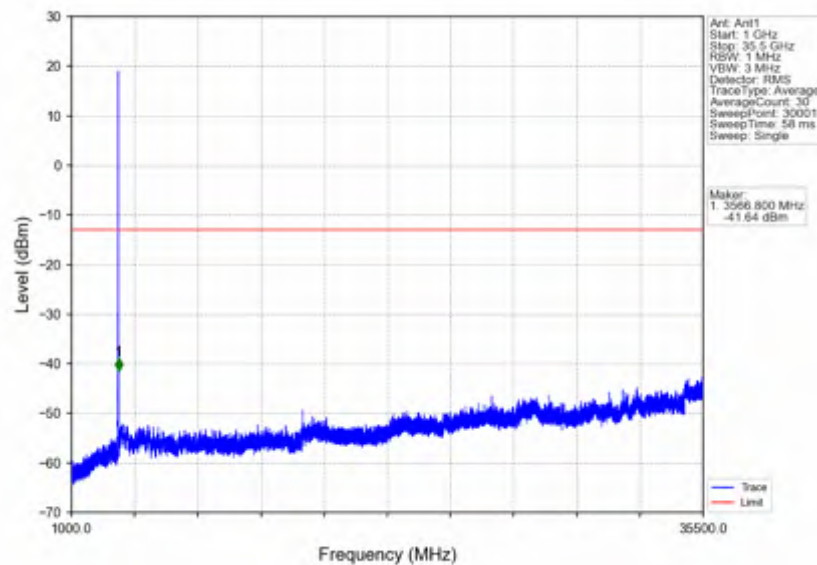
n78e_15kHz_SISO_NTNV_20MHz_DFT-s-OFDM QPSK_3540MHz_Inner_1RB_Right
