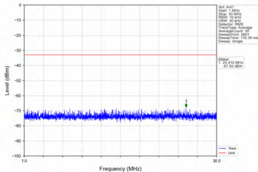
n78e_15kHz_SISO_NTNV_20MHz_CP-OFDM_QPSK_3460.005MHz_Edge_1RB_Left
