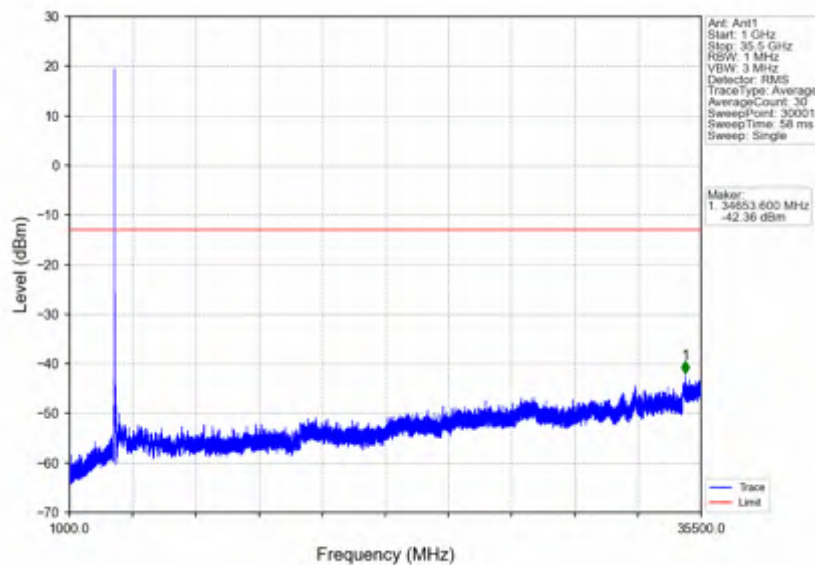
n78e_15kHz_SISO_NTNV_25MHz_CP-OFDM QPSK_3499.995MHz_Edge_1RB_Left
