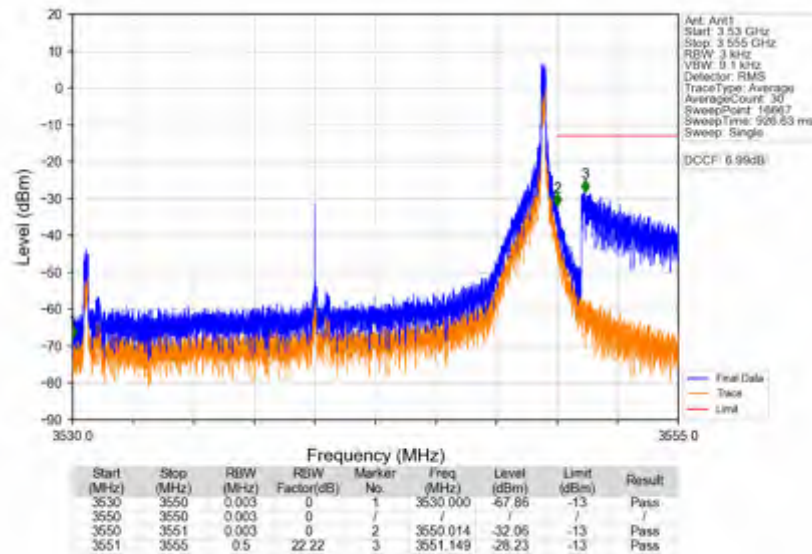
n78e_15kHz_SISO_NTNV_20MHz_CP-OFDM_QPSK_3540MHz_Edge_1RB_Right
