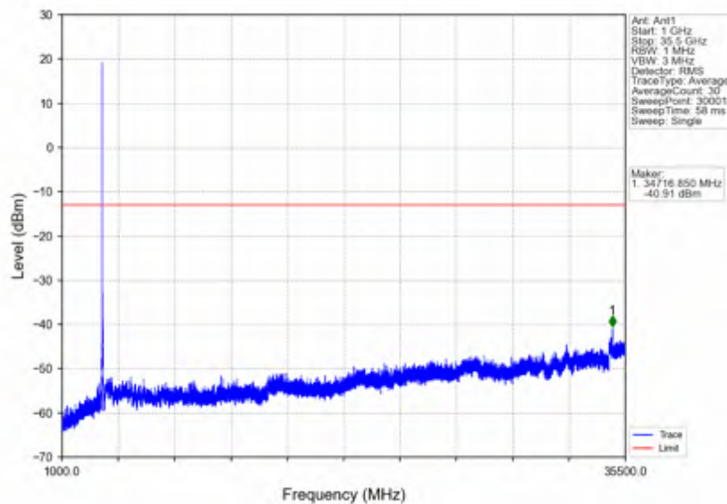
n78e_15kHz_SISO_NTNV_30MHz_CP-OFDM_QPSK_3465MHz_Outer_Full
