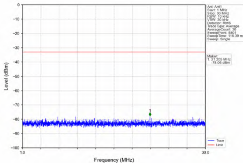
n78e_15kHz_SISO_NTNV_40MHz_DFT-s-OFDM_QPSK_3470.01MHz_Outer_Full
