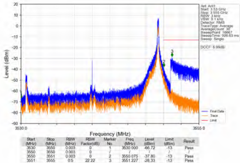
n78e_15kHz_SISO_NTNV_20MHz_DFT-s-OFDM QPSK_3540MHz_Inner_1RB_Right
