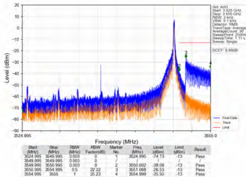
n78e_15kHz_SISO_NTNV_25MHz_DFT-s-OFDM QPSK_3537.495MHz_Inner_1RB_Right
