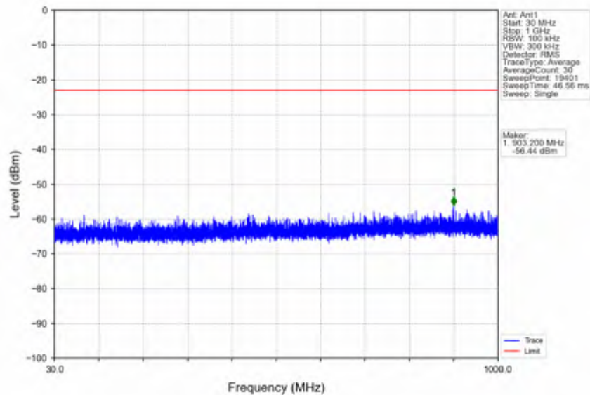
n78e_15kHz_SISO_NTNV_20MHz_DFT-s-OFDM QPSK_3460.005MHz_Edge_1RB_Left
