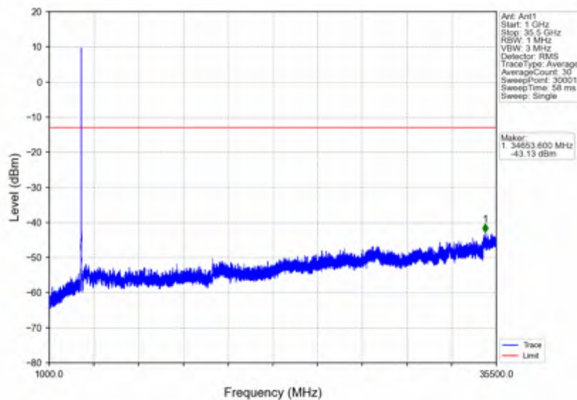
n78e_15kHz_SISO_NTNV_25MHz_DFT-s-OFDM_QPSK_3462.51MHz_Inner_1RB_Left
