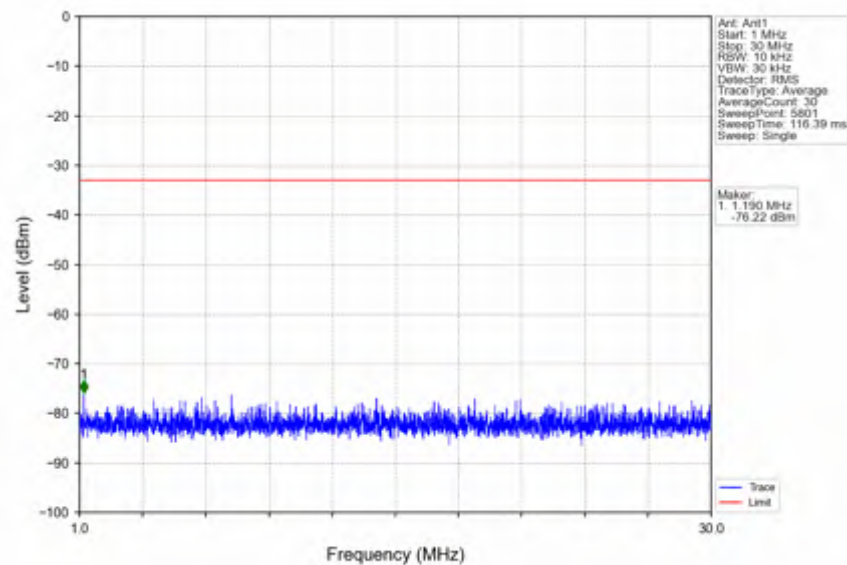
n78e_30kHz_SISO_NTNV_10MHz_CP-OFDM QPSK_3544.98MHz_Outer_Full
