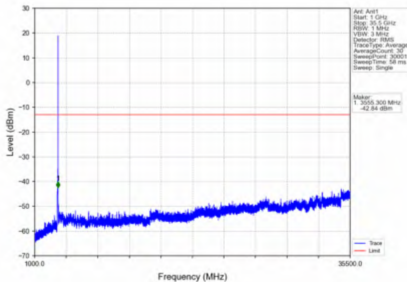
n78e_15kHz_SISO_NTNV_50MHz_CP-OFDM QPSK_3525MHz_Outer_Full
