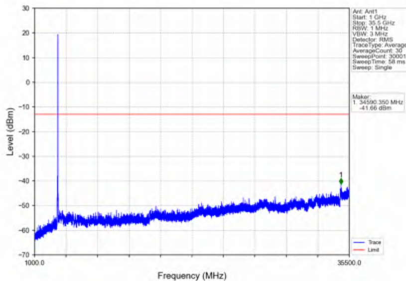
n78e_15kHz_SISO_NTNV_50MHz_DFT-s-OFDM PI/2 BPSK_3525MHz_Outer_Full
