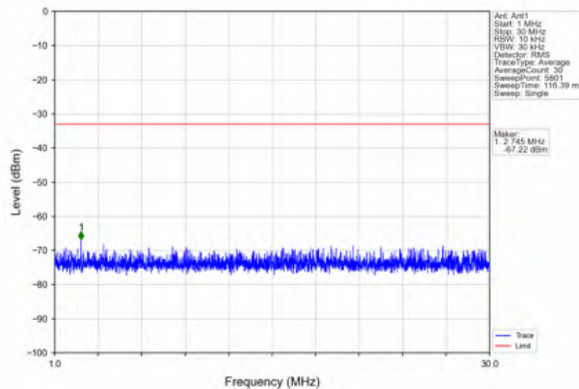
n78e_30kHz_SISO_NTNV_15MHz_CP-OFDM QPSK_3457.5MHz_Edge_1RB_Left
