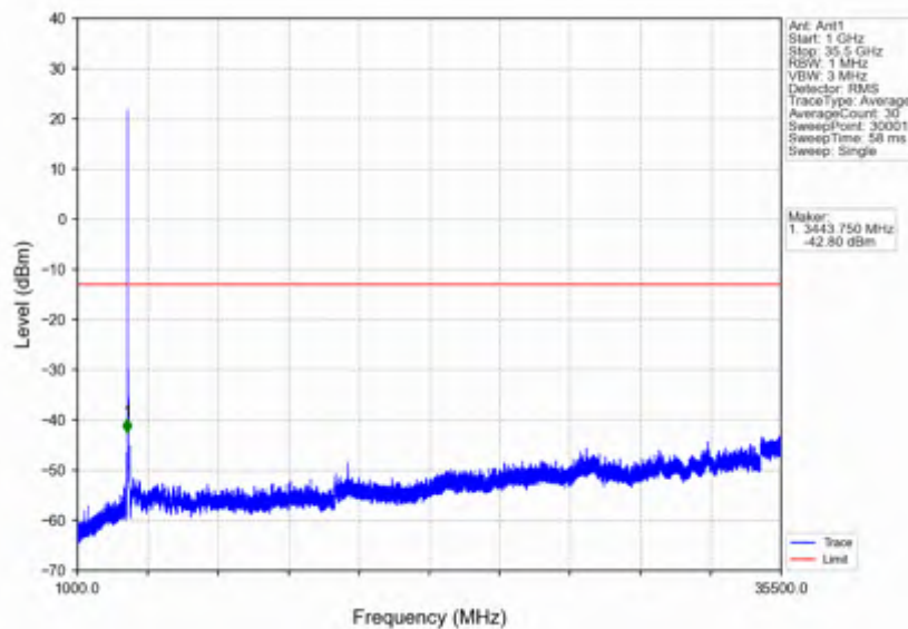
n78e_15kHz_SISO_NTNV_50MHz_CP-OFDM QPSK_3475.005MHz_Outer_Full
