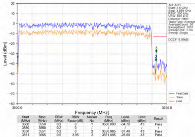
n78e_15kHz_SISO_NTNV_50MHz_CP-OFDM QPSK_3525MHz_Outer_Full
