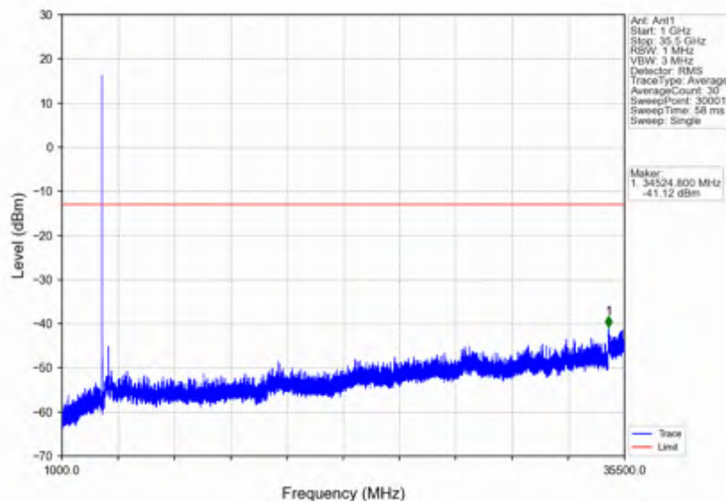
n78e_30kHz_SISO_NTNV_10MHz_CP-OFDM QPSK_3455.01MHz_Outer_Full
