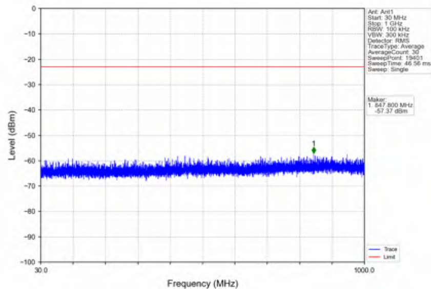
n78e_30kHz_SISO_NTNV_15MHz_CP-OFDM QPSK_3542.49MHz_Edge_1RB_Right
