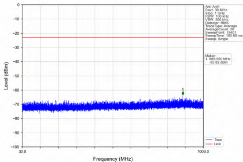
n78e_30kHz_SISO_NTNV_15MHz_DFT-s-OFDM QPSK_3457.5MHz_Inner_1RB_Left
