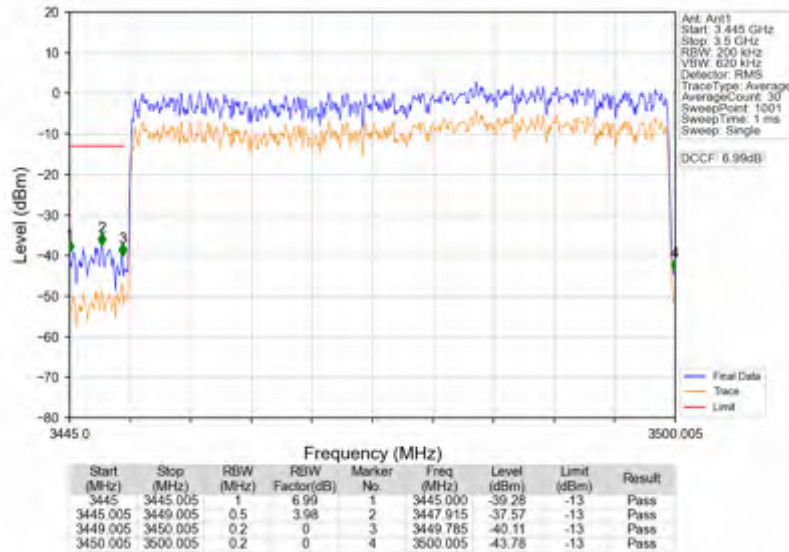
n78e_15kHz_SISO_NTNV_50MHz_CP-OFDM QPSK_3475.005MHz_Outer_Full
