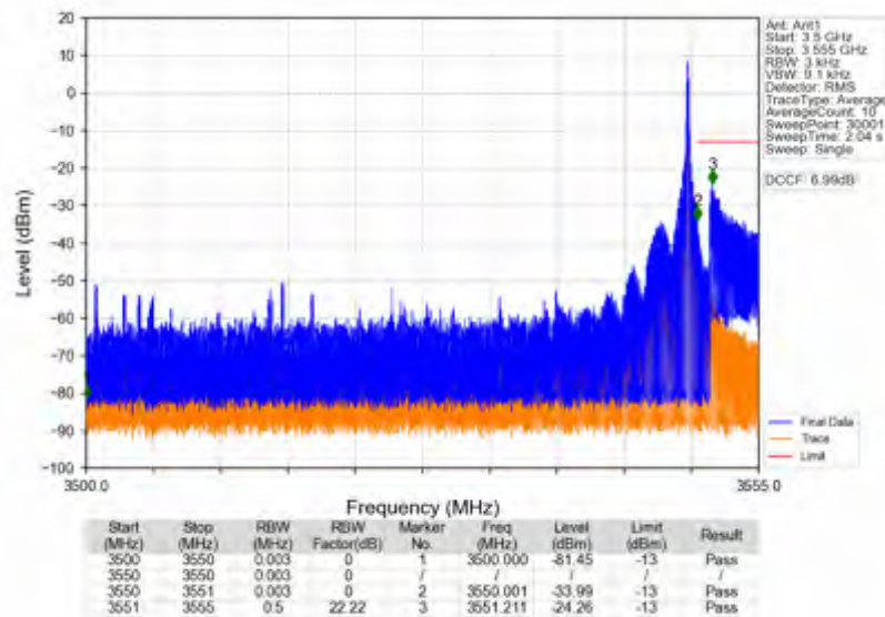
n78e_15kHz_SISO_NTNV_50MHz_DFT-s-OFDM QPSK_3525MHz_Edge_1RB_Right
