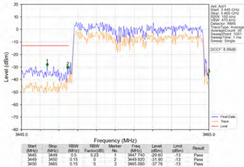
n78e_30kHz_SISO_NTNV_15MHz_CP-OFDM QPSK_3457.5MHz_Outer_Full
