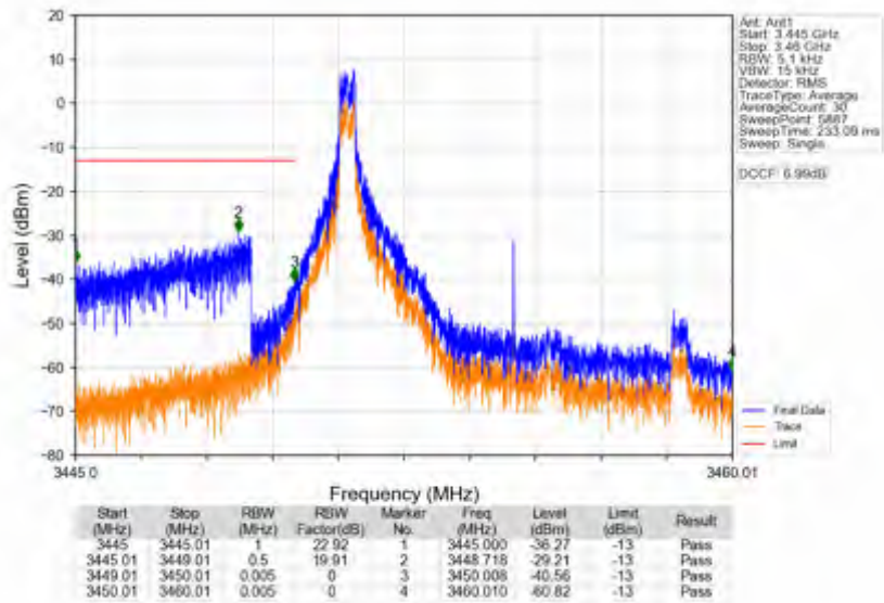
n78e_30kHz_SISO_NTNV_10MHz_DFT-s-OFDM_QPSK_3455.01MHz_Inner_1RB_Left
