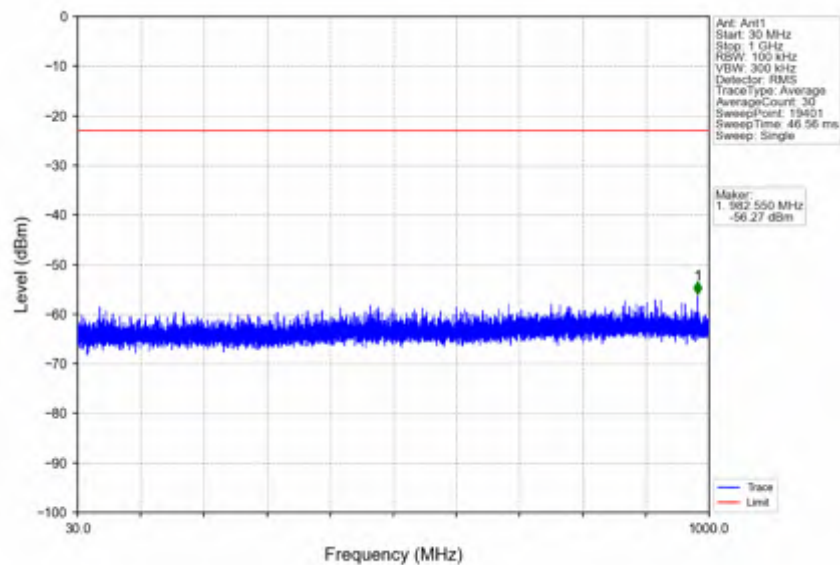
n78e_30kHz_SISO_NTNV_15MHz_DFT-s-OFDM_QPSK_3500.01MHz_Edge_1RB_Left
