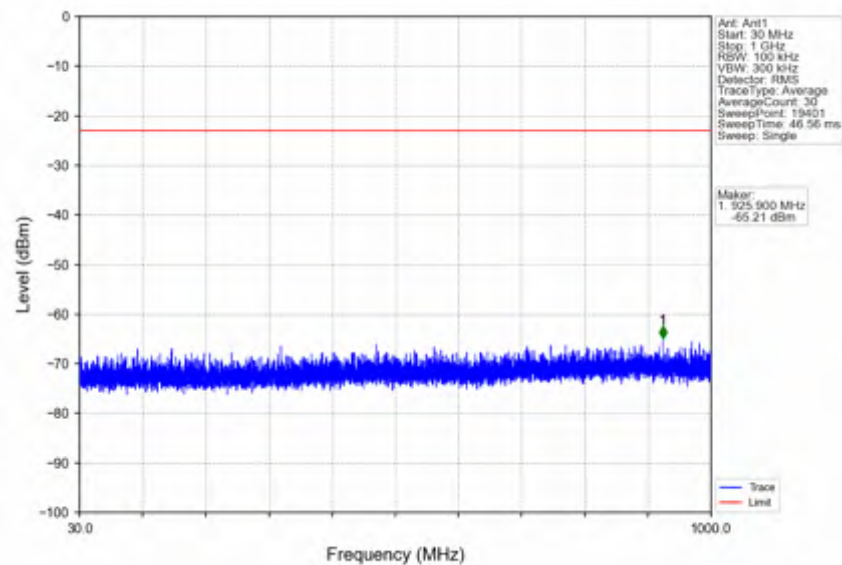
n78e_30kHz_SISO_NTNV_10MHz_CP-OFDM QPSK_3544.98MHz_Inner_1RB_Right
