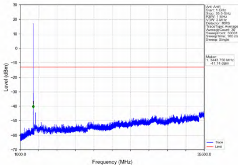
n78e_30kHz_SISO_NTNV_15MHz_CP-OFDM QPSK_3457.5MHz_Outer_Full
