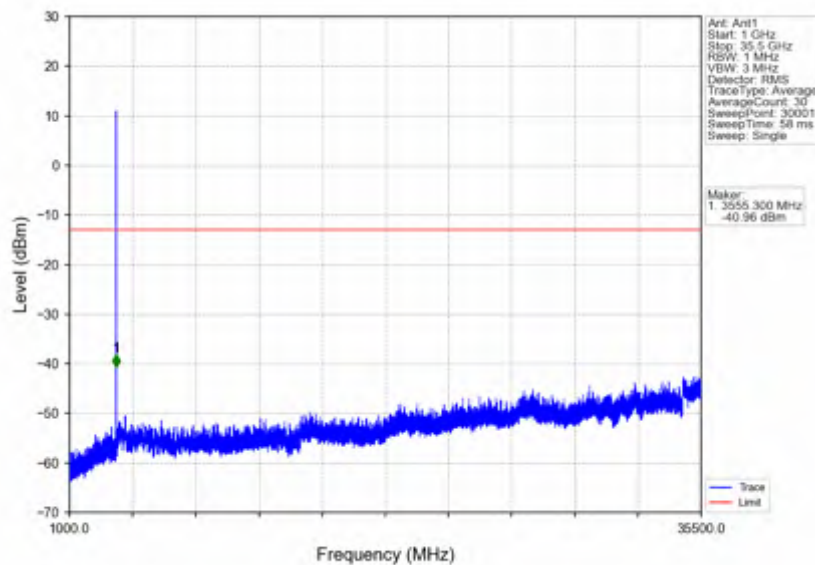
n78e_30kHz_SISO_NTNV_10MHz_DFT-s-OFDM_QPSK_3544.98MHz_Inner_1RB_Right
