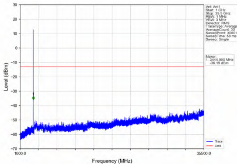
n78e_30kHz_SISO_NTNV_10MHz_DFT-s-OFDM_QPSK_3455.01MHz_Inner_1RB_Left
