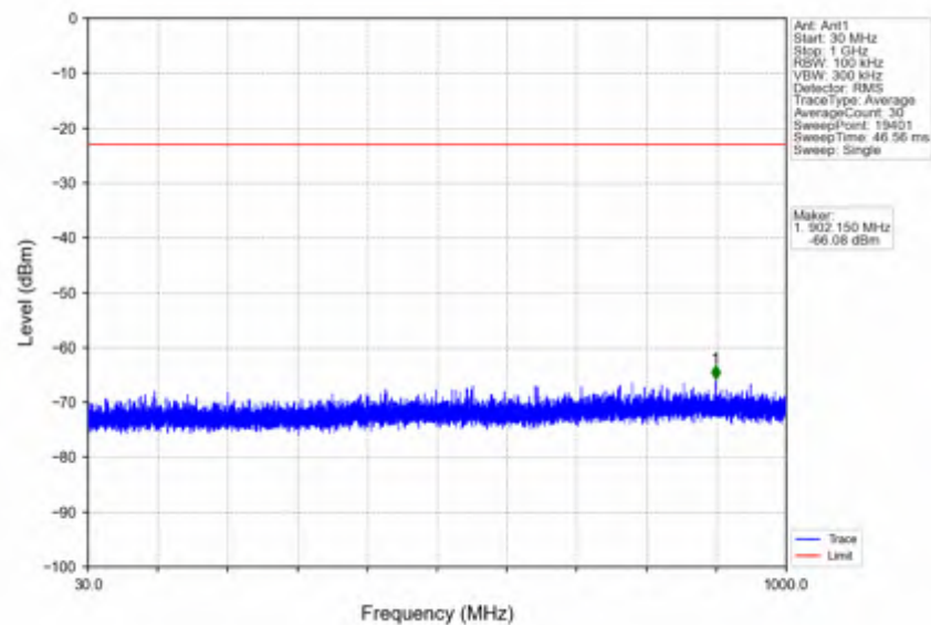
n78e_15kHz_SISO_NTNV_50MHz_DFT-s-OFDM QPSK_3525MHz_Inner_1RB_Right
