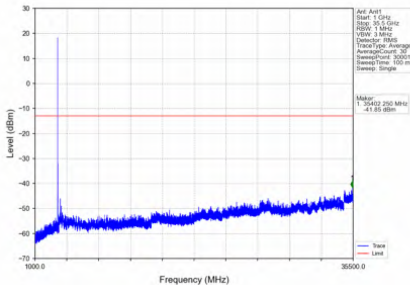
n78e_30kHz_SISO_NTNV_15MHz_DFT-s-OFDM QPSK_3457.5MHz_Edge_1RB_Left
