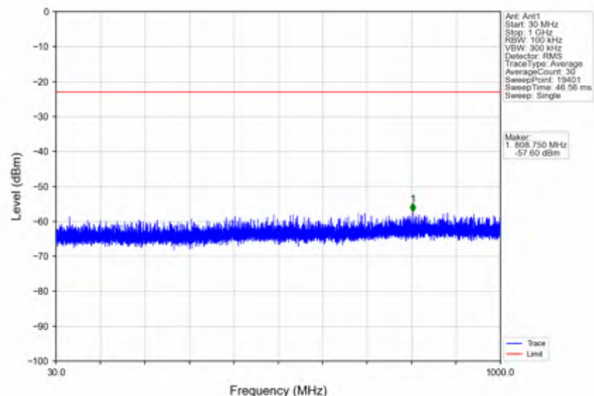
n78e_30kHz_SISO_NTNV_10MHz_CP-OFDM QPSK_3544.98MHz_Edge_1RB_Right
