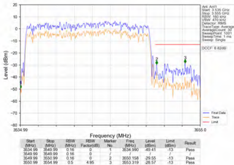
n78e_30kHz_SISO_NTNV_15MHz_CP-OFDM QPSK_3542.49MHz_Outer_Full
