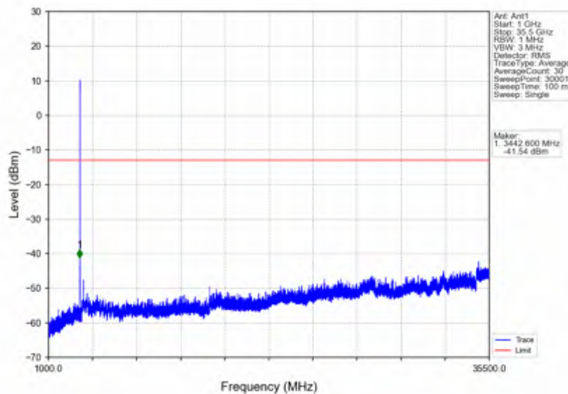
n78e_30kHz_SISO_NTNV_15MHz_DFT-s-OFDM QPSK_3457.5MHz_Inner_1RB_Left
