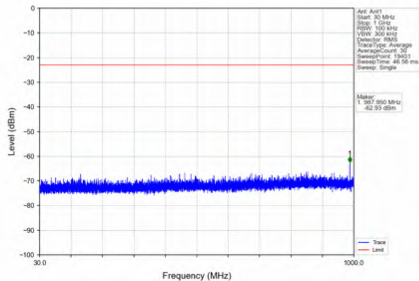
n78e_15kHz_SISO_NTNV_50MHz_CP-OFDM QPSK_3525MHz_Edge_1RB_Right
