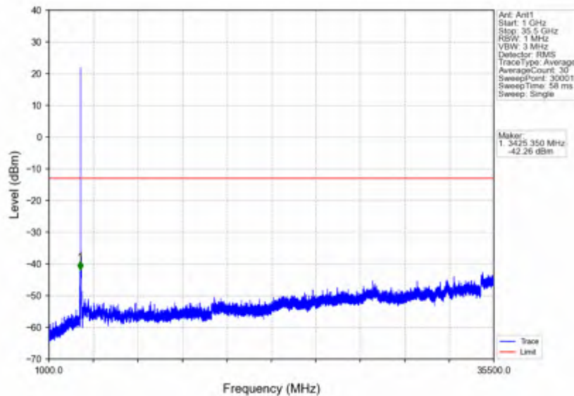
n78e_15kHz_SISO_NTNV_50MHz_DFT-s-OFDM_QPSK_3475.005MHz_Edge_1RB_Left
