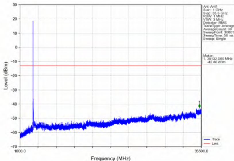
n78e_15kHz_SISO_NTNV_50MHz_DFT-s-OFDM QPSK_3525MHz_Edge_1RB_Right
