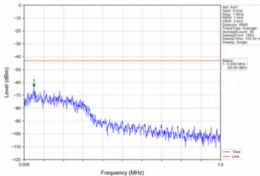
n78e_30kHz_SISO_NTNV_15MHz_CP-OFDM_QPSK_3457.5MHz_Inner_1RB_Left
