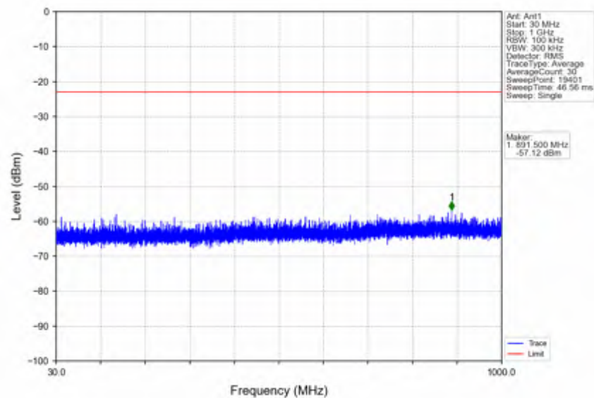
n78e_30kHz_SISO_NTNV_15MHz_DFT-s-OFDM QPSK_3542.49MHz_Edge_1RB_Right
