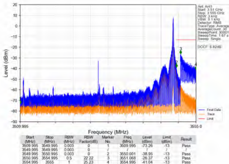
n78e_15kHz_SISO_NTNV_40MHz_DFT-s-OFDM QPSK_3529.995MHz_Inner_1RB_Right
