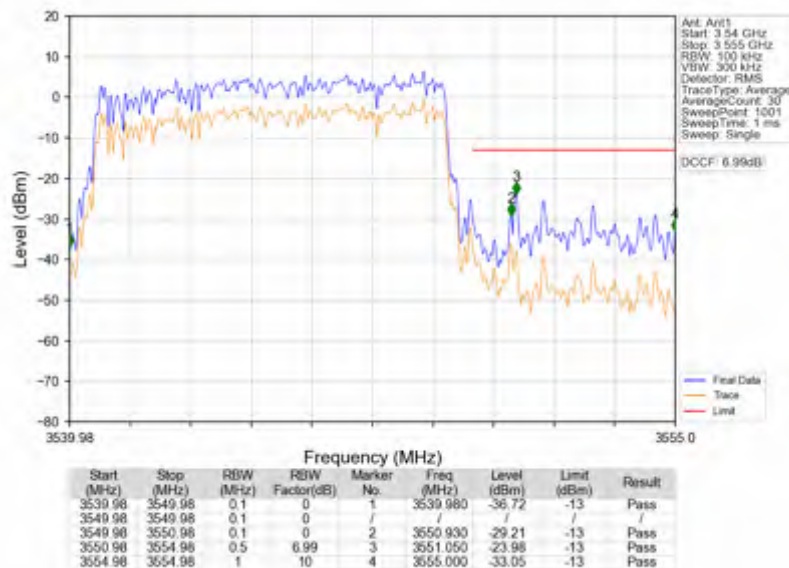
n78e_30kHz_SISO_NTNV_10MHz_CP-OFDM QPSK_3544.98MHz_Outer_Full
