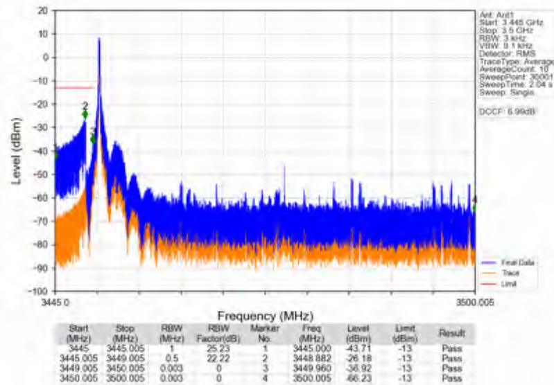
n78e_15kHz_SISO_NTNV_50MHz_DFT-s-OFDM_PI/2_BPSK_3475.005MHz_Edge_1RB_Left
