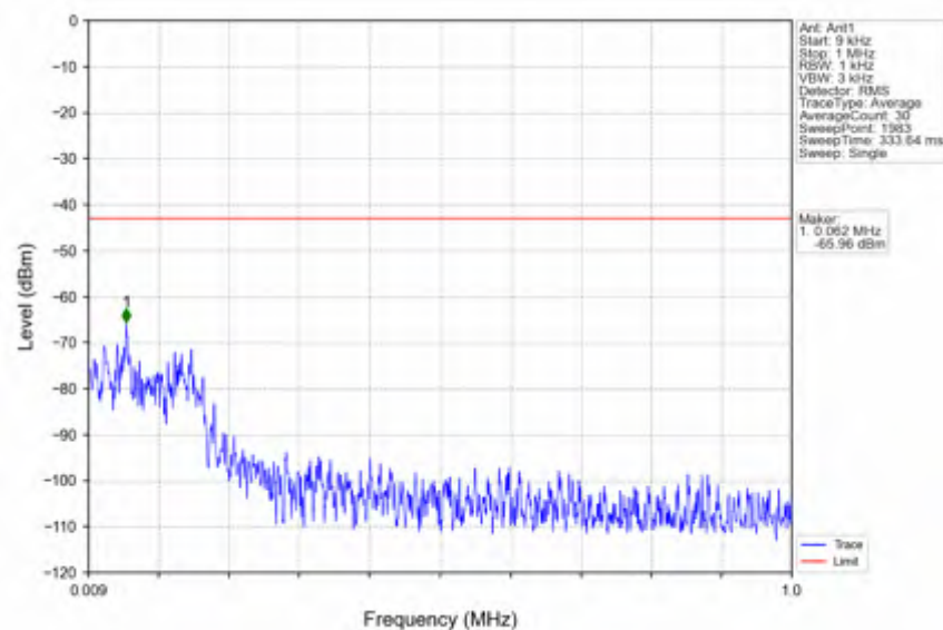
n78e_15kHz_SISO_NTNV_50MHz_DFT-s-OFDM_PI/2_BPSK_3475.005MHz_Edge_1RB_Left
