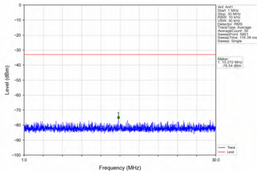
n78e_30kHz_SISO_NTNV_10MHz_CP-OFDM QPSK_3544.98MHz_Inner_1RB_Right
