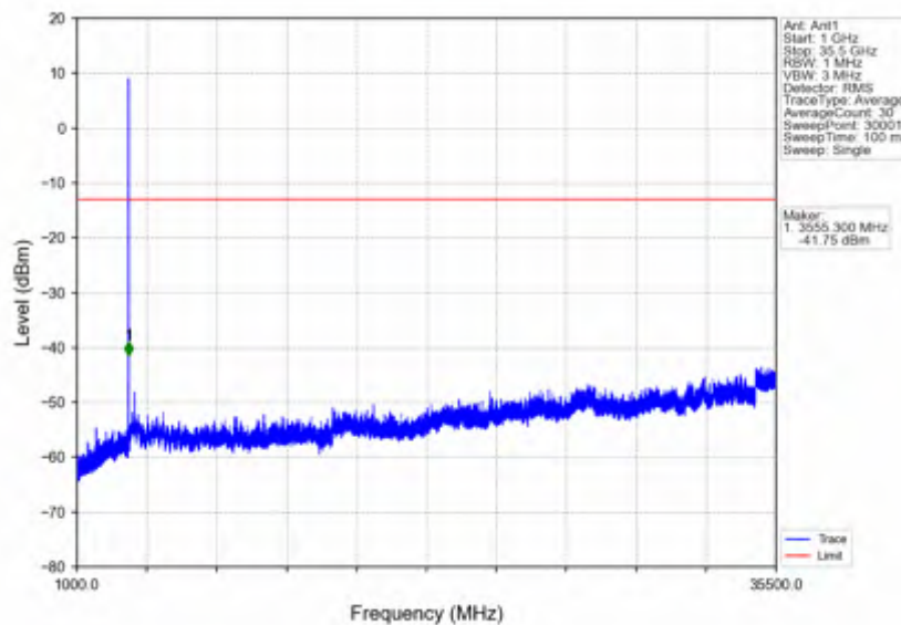
n78e_30kHz_SISO_NTNV_15MHz_DFT-s-OFDM_QPSK_3542.49MHz_Inner_1RB_Right
