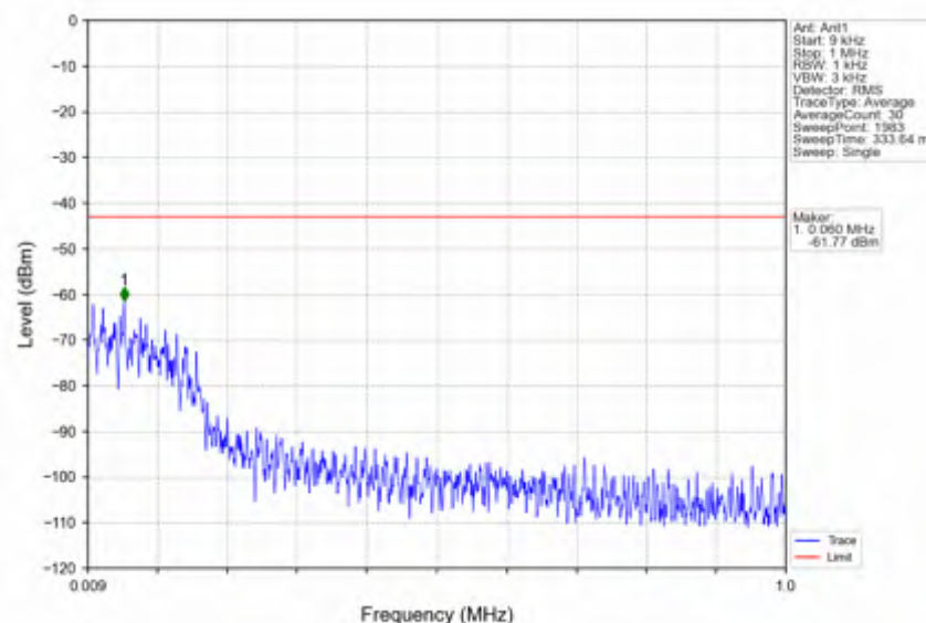
n78e_15kHz_SISO_NTNV_50MHz_CP-OFDM QPSK_3525MHz_Edge_1RB_Right
