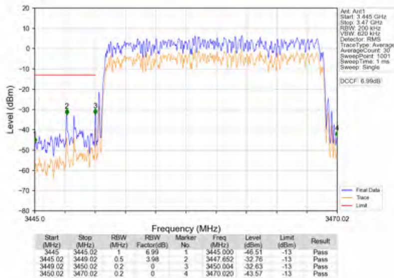
n78e_30kHz_SISO_NTNV_20MHz_DFT-s-OFDM PI/2 BPSK_3460.02MHz_Outer_Full
