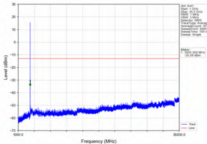
n78e_30kHz_SISO_NTNV_15MHz_DFT-s-OFDM QPSK_3542.49MHz_Edge_1RB_Right
