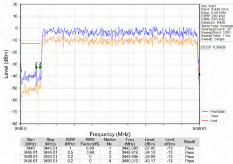
n78e_15kHz_SISO_NTNV_40MHz_CP-OFDM_QPSK_3470.01MHz_Outer_Full
