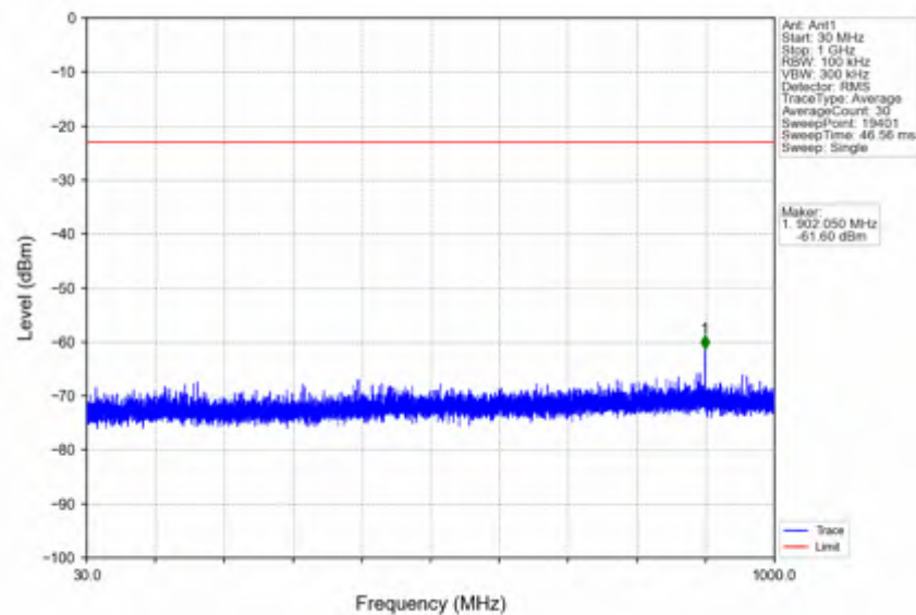
n78e_15kHz_SISO_NTNV_50MHz_DFT-s-OFDM_QPSK_3525MHz_Outer_Full
