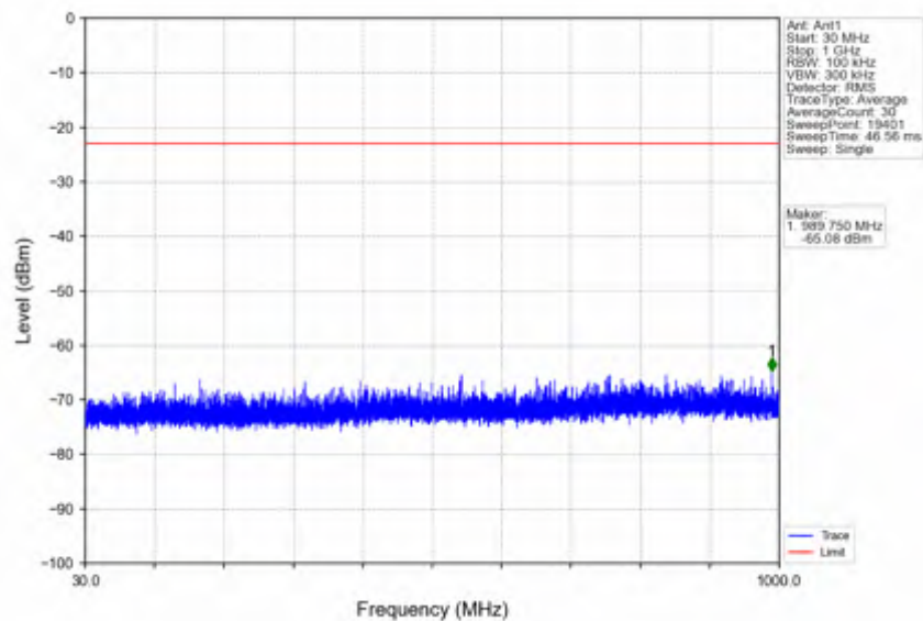
n78e_30kHz_SISO_NTNV_10MHz_DFT-s-OFDM_QPSK_3455.01MHz_Outer_Full
