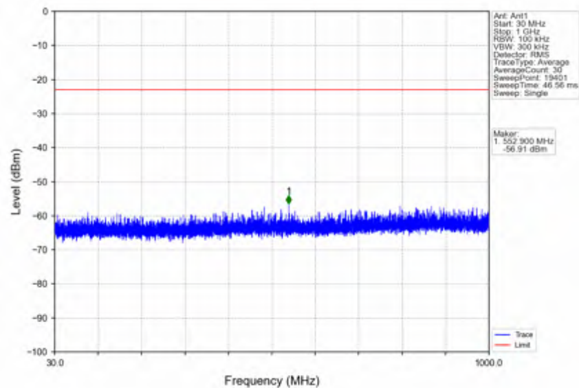
n78e_30kHz_SISO_NTNV_10MHz_DFT-s-OFDM QPSK_3544.98MHz_Edge_1RB_Right
