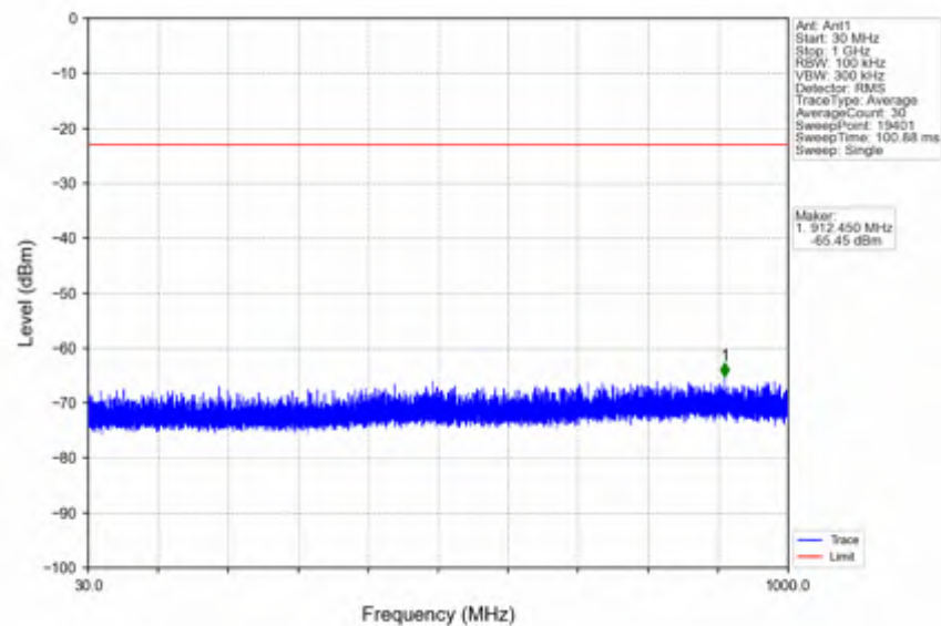
n78e_30kHz_SISO_NTNV_15MHz_DFT-s-OFDM_QPSK_3542.49MHz_Outer_Full
