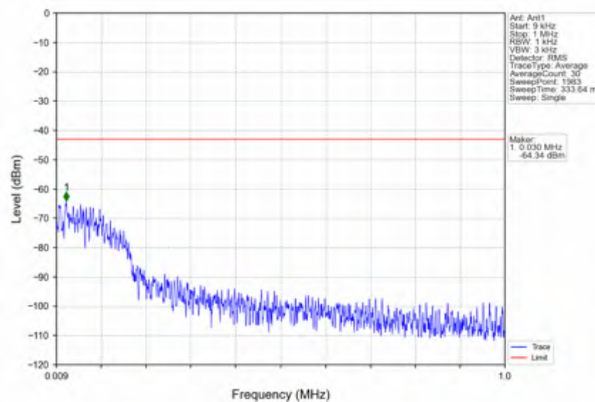
n78e_15kHz_SISO_NTNV_50MHz_CP-OFDM_QPSK_3525MHz_Inner_1RB_Right
