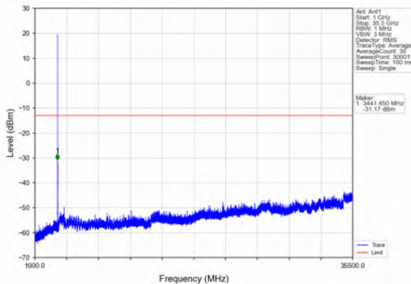
n78e_30kHz_SISO_NTNV_20MHz_DFT-s-OFDM PI/2 BPSK_3460.02MHz_Outer_Full
