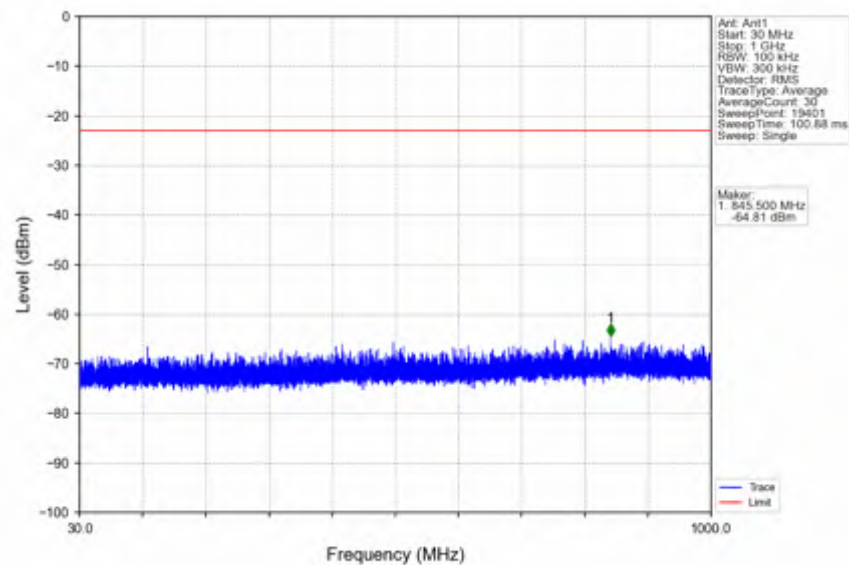
n78e_30kHz_SISO_NTNV_15MHz_DFT-s-OFDM QPSK_3457.5MHz_Outer_Full
