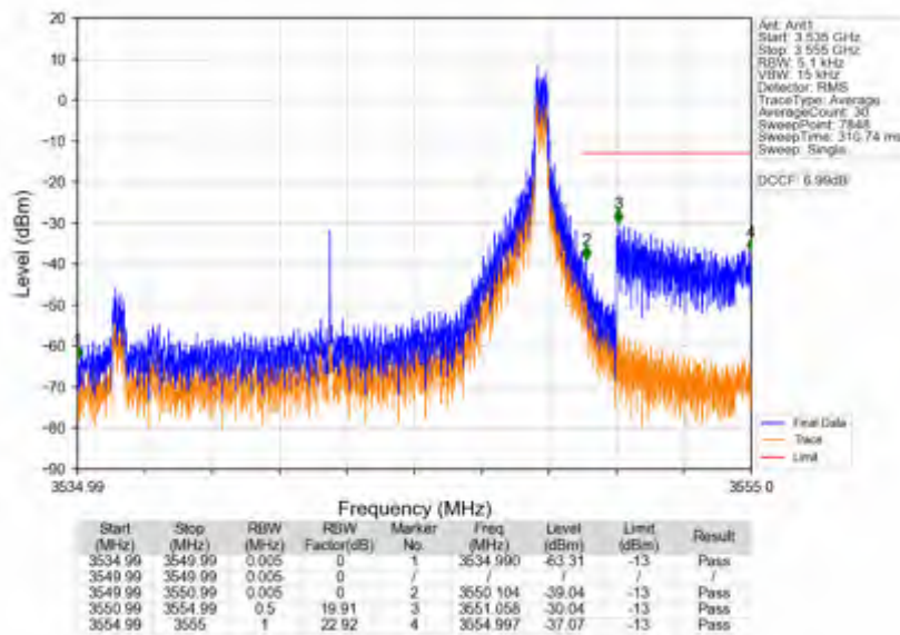
n78e_30kHz_SISO_NTNV_15MHz_DFT-s-OFDM_QPSK_3542.49MHz_Inner_1RB_Right
