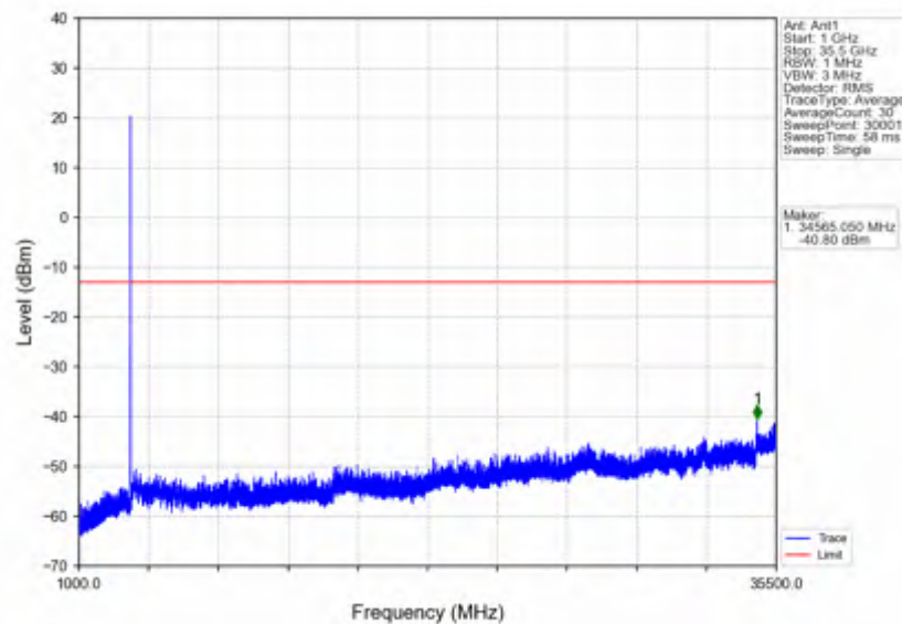
n78e_30kHz_SISO_NTNV_10MHz_DFT-s-OFDM QPSK_3544.98MHz_Edge_1RB_Right
