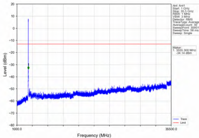
n78e 15kHz SISO NTV 50MHz CP-OFDM QPSK 3525MHz Outer Full
