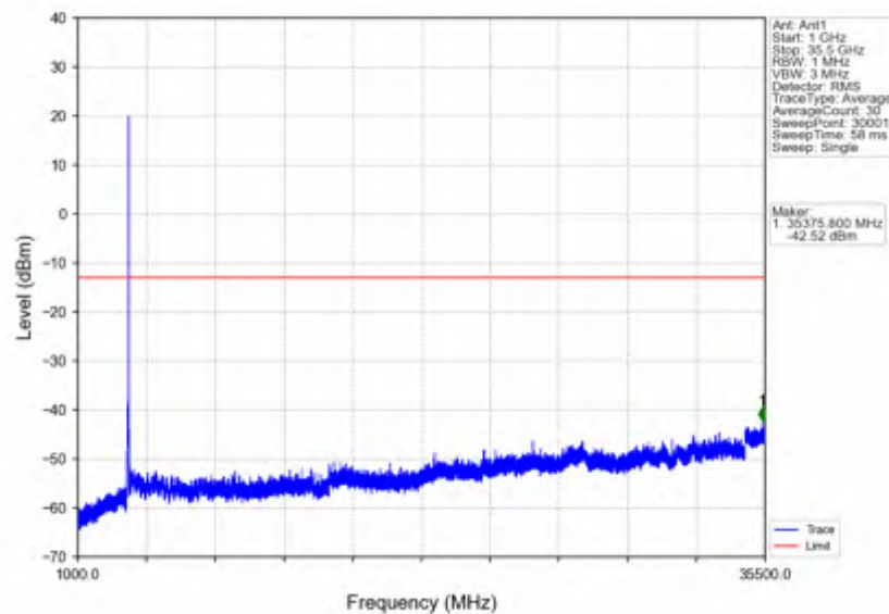
n78e_15kHz_SISO_NTNV_50MHz_DFT-s-OFDM QPSK_3525MHz_Inner_1RB_Right
