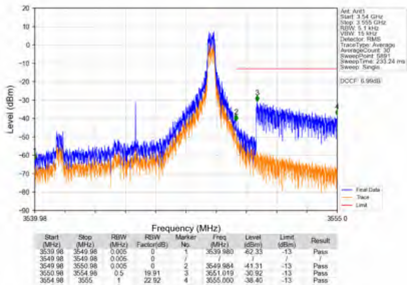
n78e_30kHz_SISO_NTNV_10MHz_DFT-s-OFDM_QPSK_3544.98MHz_Inner_1RB_Right
