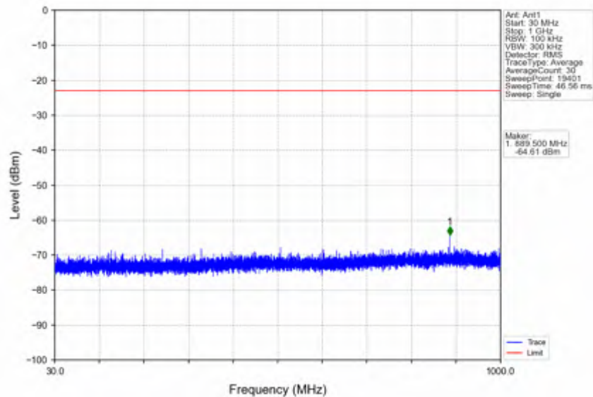
n78e_15kHz_SISO_NTNV_50MHz_DFT-s-OFDM_QPSK_3475.005MHz_Edge_1RB_Left
