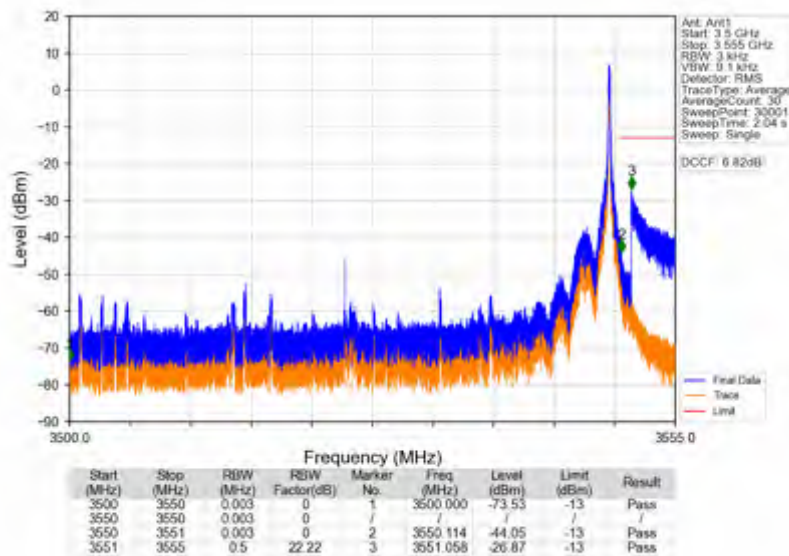
n78e_15kHz_SISO_NTNV_50MHz_DFT-s-OFDM QPSK_3525MHz_Inner_1RB_Right
