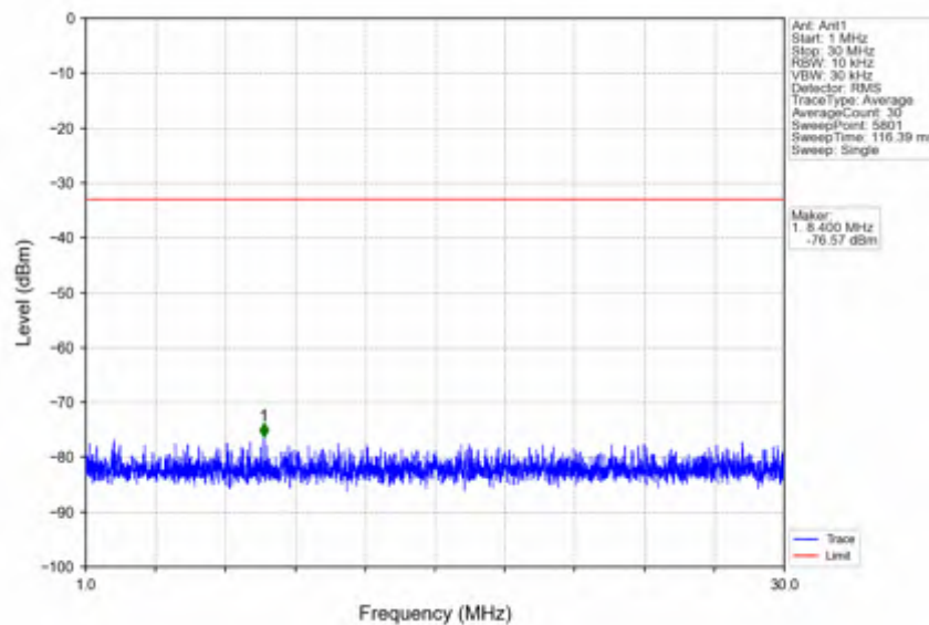
n78e_30kHz_SISO_NTNV_10MHz_DFT-s-OFDM_QPSK_3544.98MHz_Outer_Full
