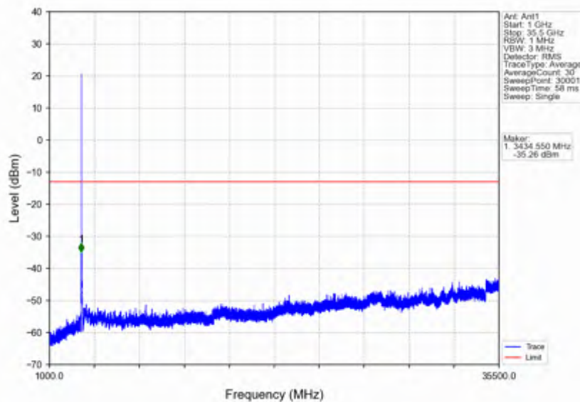
n78e_15kHz_SISO_NTNV_40MHz_CP-OFDM_QPSK_3470.01MHz_Outer_Full
