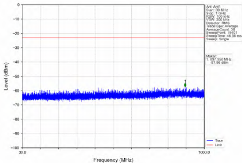
n78e_30kHz_SISO_NTNV_15MHz_DFT-s-OFDM QPSK_3457.5MHz_Edge_1RB_Left
