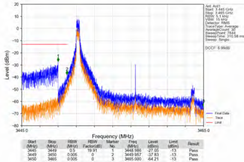
n78e_30kHz_SISO_NTNV_15MHz_CP-OFDM_QPSK_3457.5MHz_Inner_1RB_Left
