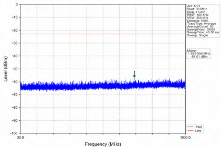
n78e_30kHz_SISO_NTNV_10MHz_DFT-s-OFDM_QPSK_3500.01MHz_Edge_1RB_Left
