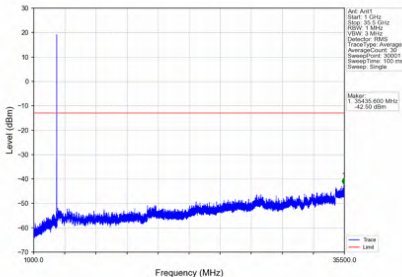
n78e_30kHz_SISO_NTNV_15MHz_CP-OFDM QPSK_3542.49MHz_Outer_Full
