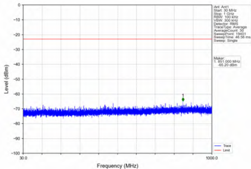
n78e 15kHz SISO NTV 50MHz CP-OFDM QPSK 3525MHz Outer Full
