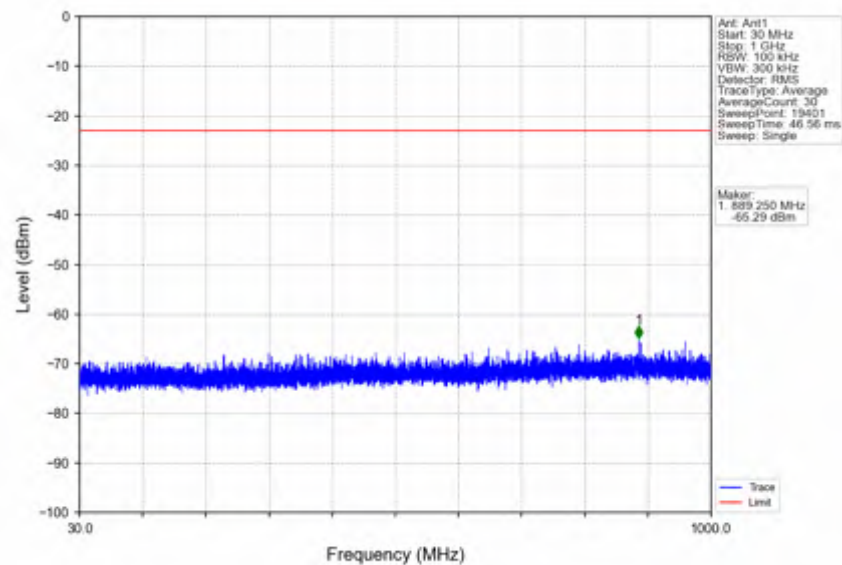
n78e_15kHz_SISO_NTNV_50MHz_DFT-s-OFDM QPSK_3525MHz_Edge_1RB_Right
