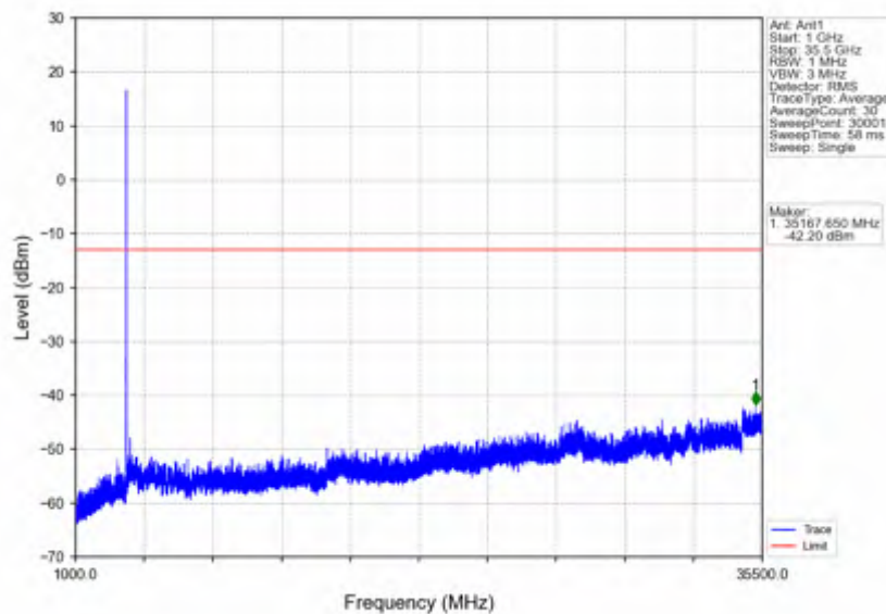
n78e_30kHz_SISO_NTNV_10MHz_CP-OFDM QPSK_3544.98MHz_Outer_Full
