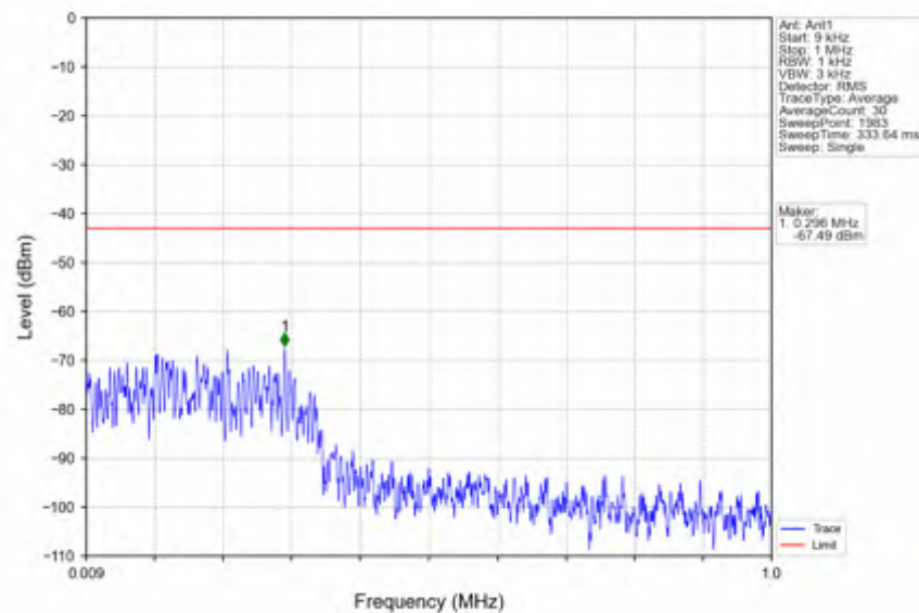
n78e_30kHz_SISO_NTNV_15MHz_DFT-s-OFDM QPSK_3457.5MHz_Edge_1RB_Left
