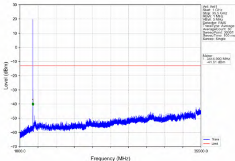
n78e_30kHz_SISO_NTNV_15MHz_CP-OFDM QPSK_3500.01MHz_Edge_1RB_Left
