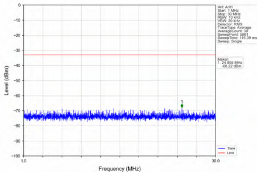
n78e_30kHz_SISO_NTNV_15MHz_DFT-s-OFDM_QPSK_3500.01MHz_Edge_1RB_Left
