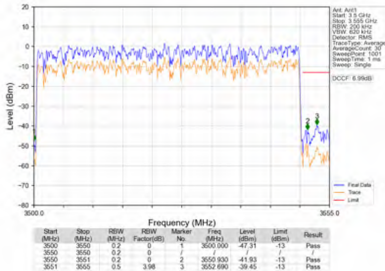
n78e_15kHz_SISO_NTNV_50MHz_DFT-s-OFDM PI/2 BPSK_3525MHz_Outer_Full
