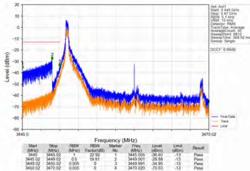
n78e_30kHz_SISO_NTNV_20MHz_DFT-s-OFDM PI/2 BPSK_3460.02MHz_Edge_1RB_Left
