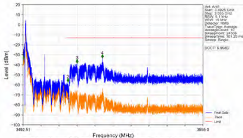
n78e_30kHz_SISO_NTNV_15MHz_CP-OFDM QPSK_3500.01MHz_Edge_1RB_Left
