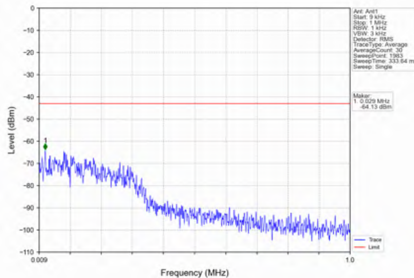
n78e_30kHz_SISO_NTV_15MHz_CP-OFDM QPSK_3500.01MHz_Edge_1RB_Left
