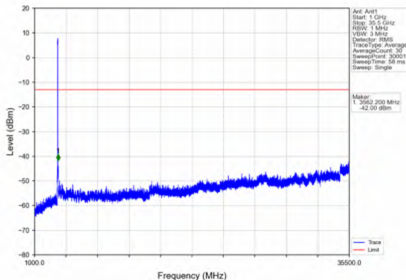
n78e_15kHz_SISO_NTNV_40MHz_DFT-s-OFDM QPSK_3529.995MHz_Inner_1RB_Right
