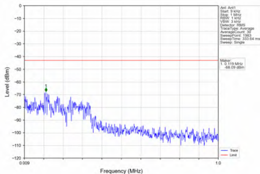
n78e_30kHz_SISO_NTNV_20MHz_DFT-s-OFDM PI/2 BPSK_3460.02MHz_Edge_1RB_Left
