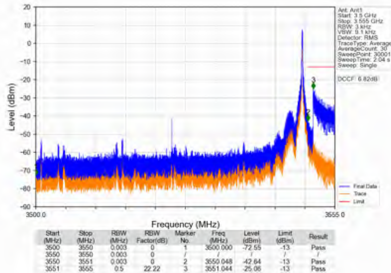
n78e_15kHz_SISO_NTNV_50MHz_CP-OFDM_QPSK_3525MHz_Inner_1RB_Right
