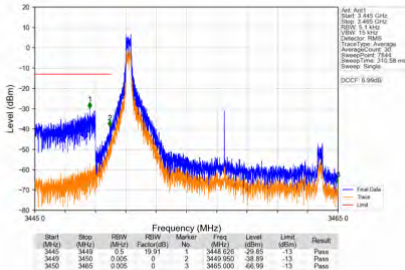
n78e_30kHz_SISO_NTNV_15MHz_DFT-s-OFDM QPSK_3457.5MHz_Inner_1RB_Left
