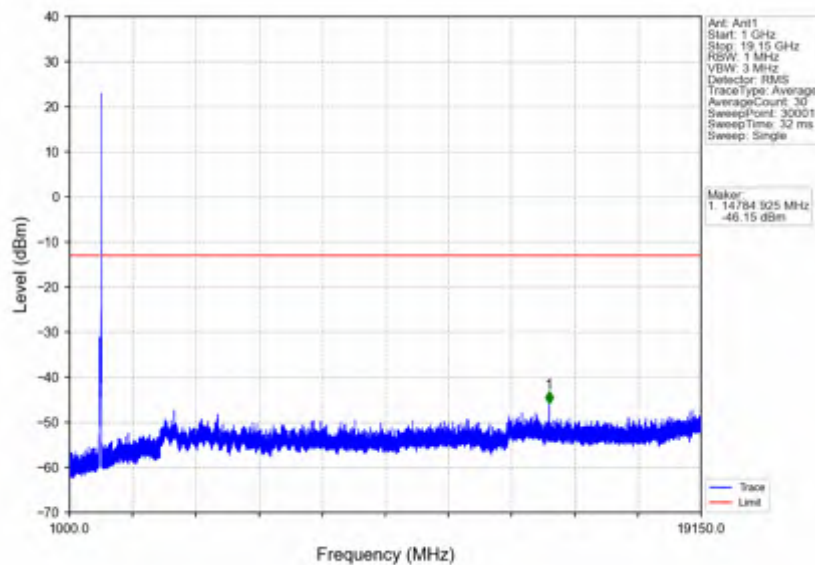
n25_15kHz_SISO_NTNV_30MHz_DFT-s-OFDM PI/2 BPSK_1900MHz_Outer_Full
