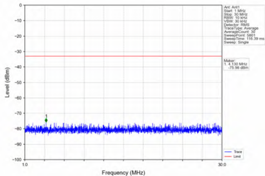
n25_15kHz_SISO_NTNV_25MHz_CP-OFDM_QPSK_1902.5MHz_Outer_Full
