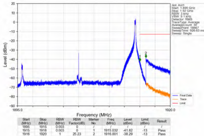
n25_15kHz_SISO_NTNV_20MHz_CP-OFDM QPSK_1905MHz_Inner_1RB_Right
