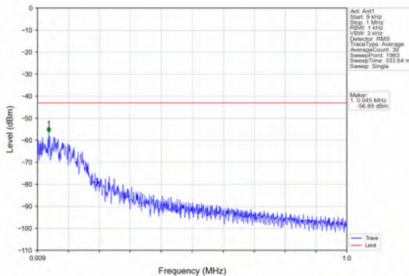
n25_15kHz_SISO_NTNV_25MHz_CP-OFDM_QPSK_1902.5MHz_Inner_1RB_Right
