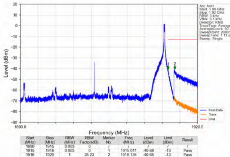
n25_15kHz_SISO_NTNV_25MHz_CP-OFDM_QPSK_1902.5MHz_Edge_1RB_Right
