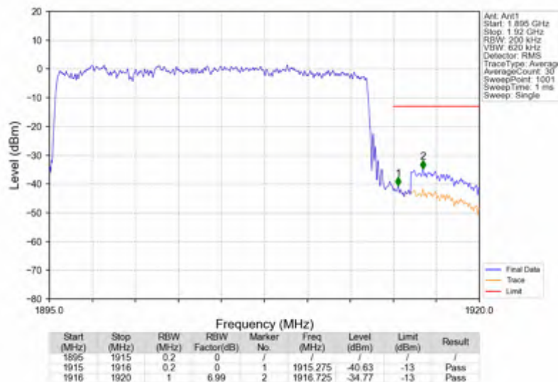
n25_15kHz_SISO_NTNV_20MHz_DFT-s-OFDM_QPSK_1905MHz_Outer_Full
