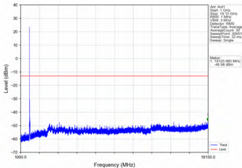
n25_15kHz_SISO_NTNV_25MHz_DFT-s-OFDM PI/2 BPSK_1882.5MHz_Edge_1RB_Left
