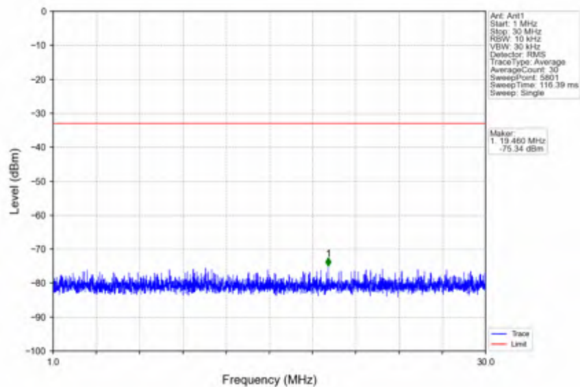
n25_15kHz_SISO_NTNV_30MHz_CP-OFDM QPSK_1900MHz_Outer_Full
