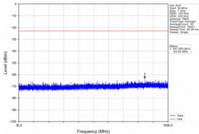
n25_15kHz_SISO_NTNV_25MHz_CP-OFDM QPSK_1862.5MHz_Outer_Full
