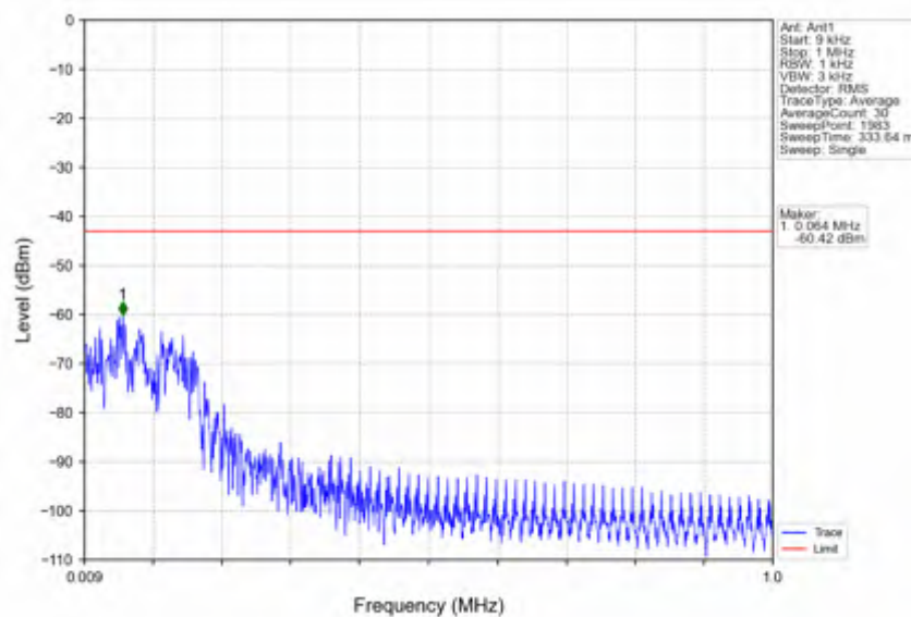
n25_15kHz_SISO_NTNV_20MHz_DFT-s-OFDM PI/2 BPSK_1905MHz_Inner_1RB_Right
