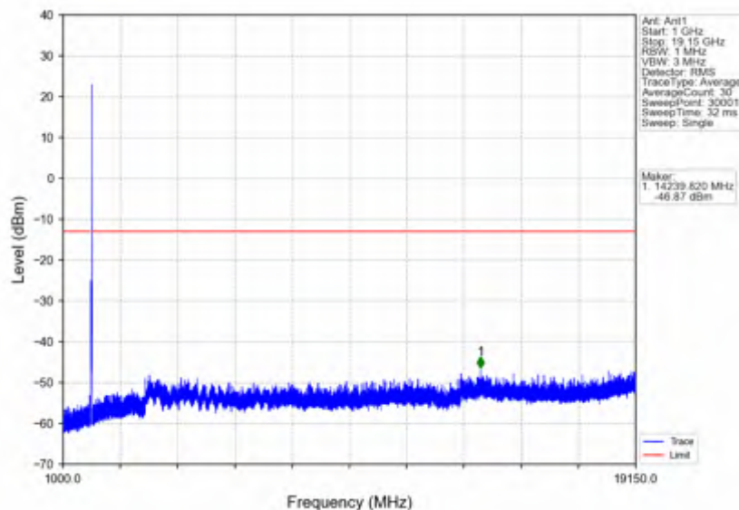
n25_15kHz_SISO_NTNV_20MHz_DFT-s-OFDM QPSK_1860MHz_Edge_1RB_Left
