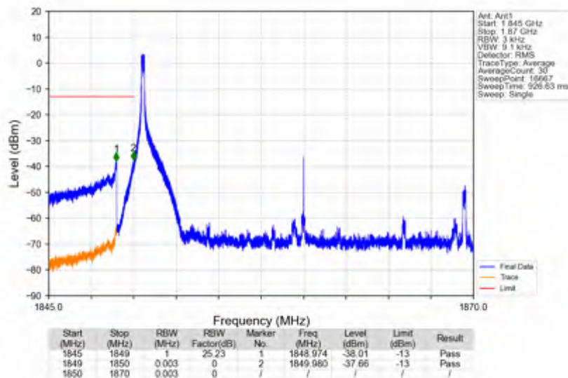
n25_15kHz_SISO_NTNV_20MHz_DFT-s-OFDM QPSK_1860MHz_Edge_1RB_Left
