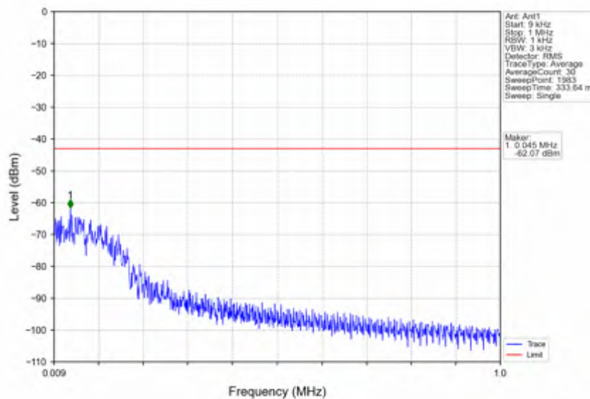
n25_15kHz_SISO_NTNV_25MHz_CP-OFDM_QPSK_1862.5MHz_Edge_1RB_Left
