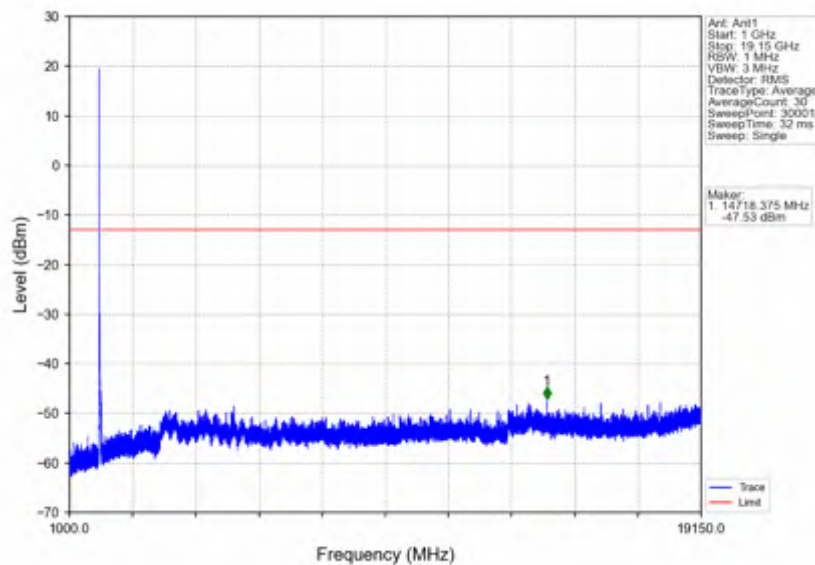
n25_15kHz_SISO_NTV_25MHz_CP-OFDM QPSK_1862.5MHz_Outer_Full
