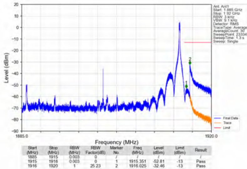
n25_15kHz_SISO_NTNV_30MHz_DFT-s-OFDM PI/2 BPSK_1900MHz_Inner_1RB_Right
