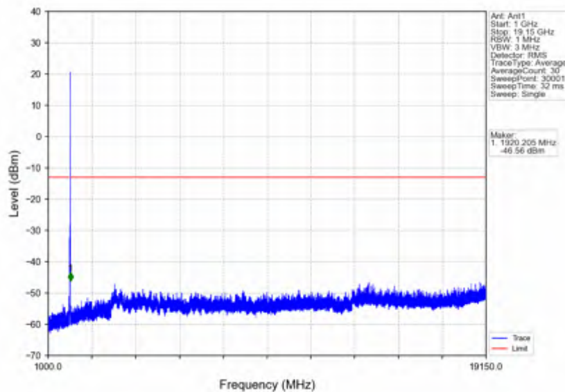
n25_15kHz_SISO_NTNV_15MHz_CP-OFDM QPSK_1907.5MHz_Outer_Full
