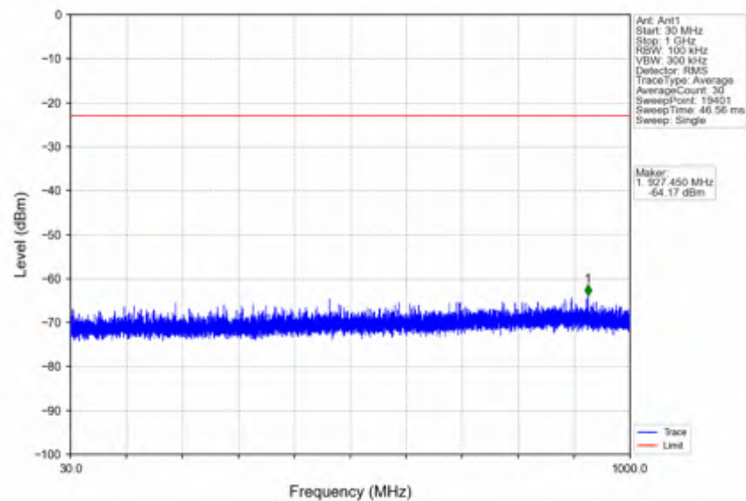
n25 15kHz SISO NTNV 25MHz CP-OFDM QPSK 1902.5MHz Outer Full
