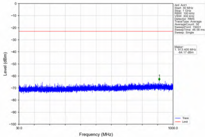
n25_15kHz_SISO_NTNV_30MHz_CP-OFDM QPSK_1900MHz_Outer_Full
