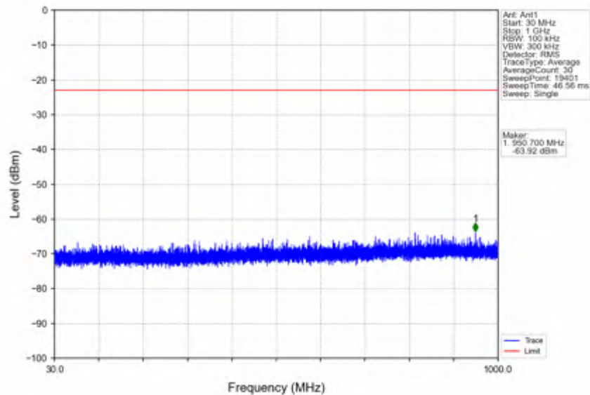
n25_15kHz_SISO_NTNV_30MHz_DFT-s-OFDM QPSK_1900MHz_Inner_1RB_Right
