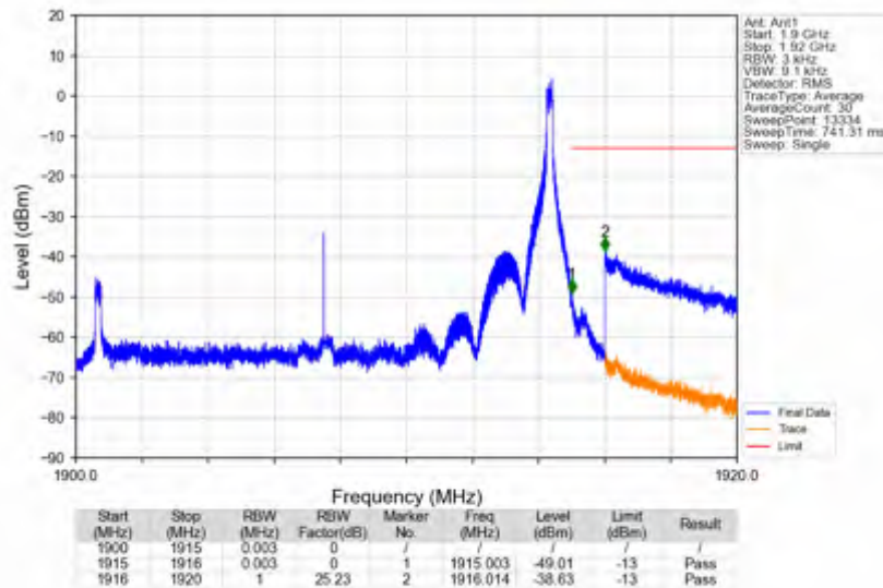
n25_15kHz_SISO_NTNV_15MHz_CP-OFDM_QPSK_1907.5MHz_Inner_1RB_Right
