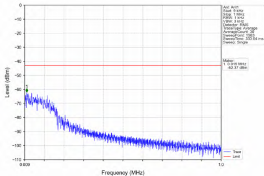
n25_15kHz_SISO_NTNV_20MHz_CP-OFDM_QPSK_1882.5MHz_Edge_1RB_Left
