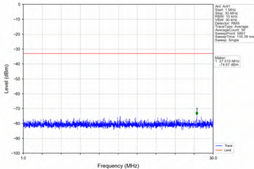
n25_15kHz_SISO_NTNV_25MHz_CP-OFDM QPSK_1902.5MHz_Inner_1RB_Right
