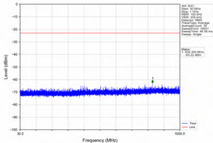
n25_15kHz_SISO_NTNV_30MHz_CP-OFDM QPSK_1882.5MHz_Edge_1RB_Left
