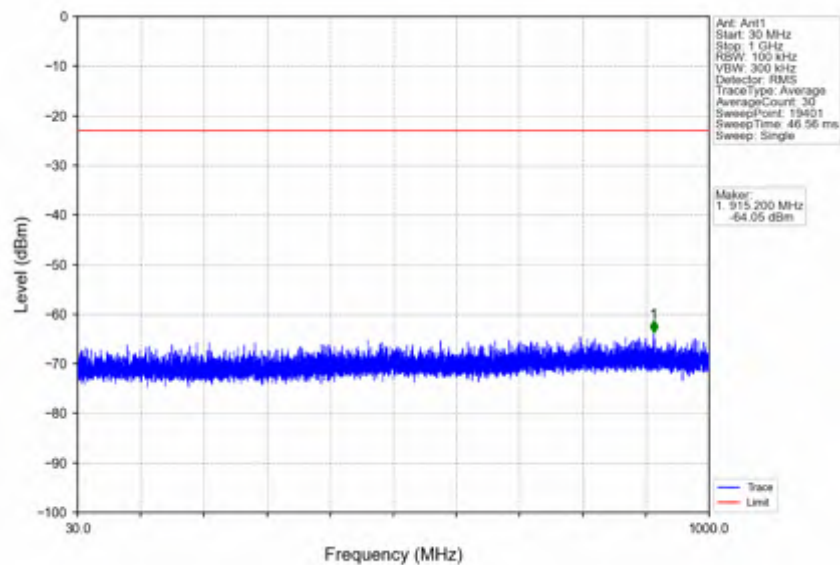
n25_15kHz_SISO_NTNV_20MHz_DFT-s-OFDM QPSK_1905MHz_Inner_1RB_Right
