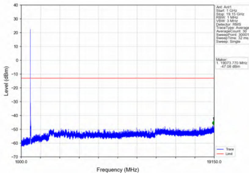
n25_15kHz_SISO_NTNV_25MHz_DFT-s-OFDM PI/2 BPSK_1862.5MHz_Outer_Full
