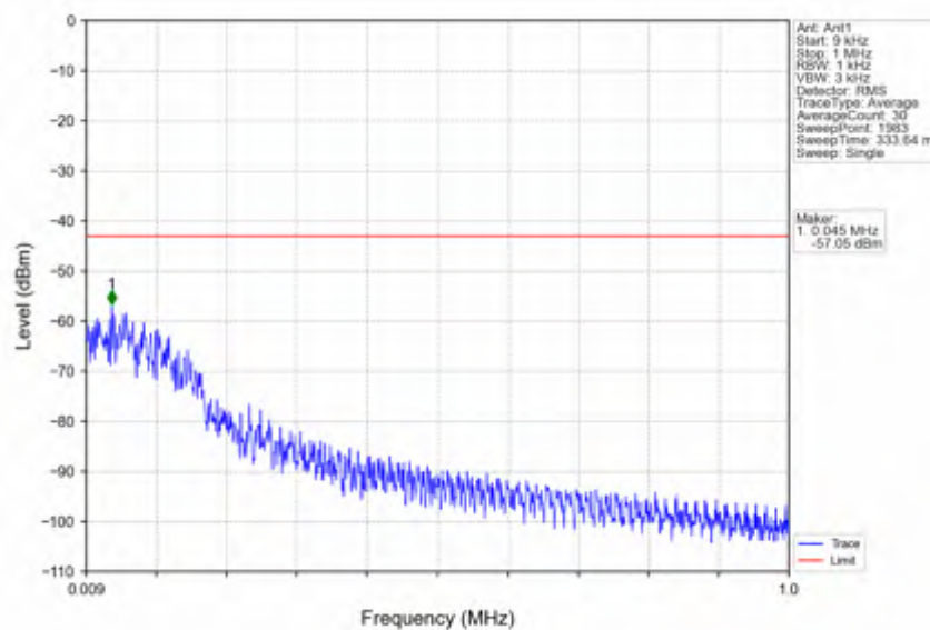
n25_15kHz_SISO_NTNV_30MHz_CP-OFDM QPSK_1900MHz_Inner_1RB_Right
