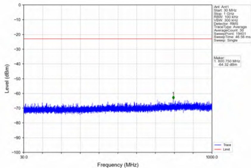
n25_15kHz_SISO_NTNV_40MHz_DFT-s-OFDM QPSK_1870MHz_Edge_1RB_Left
