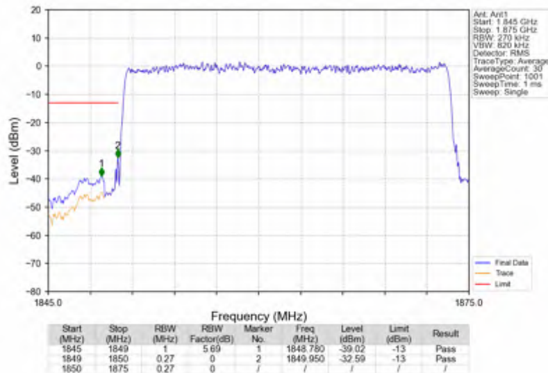
n25_15kHz_SISO_NTNV_25MHz_DFT-s-OFDM PI/2 BPSK_1862.5MHz_Outer_Full
