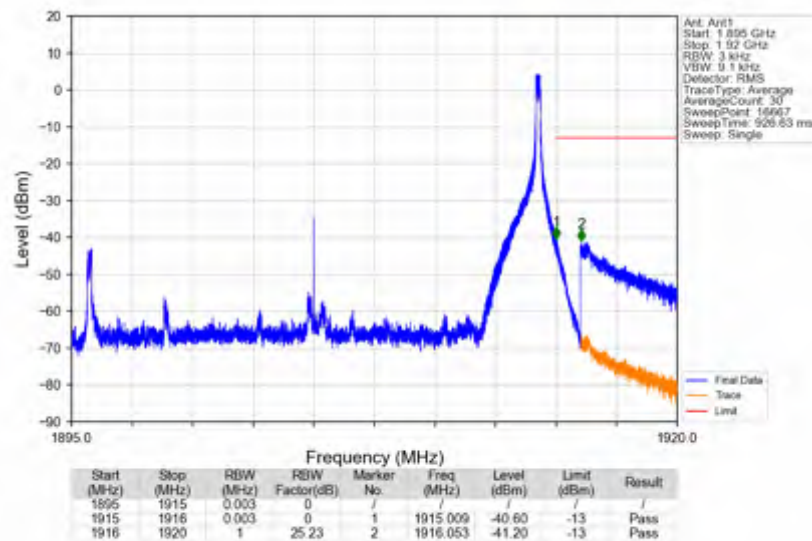
n25_15kHz_SISO_NTNV_20MHz_DFT-s-OFDM QPSK_1905MHz_Inner_1RB_Right
