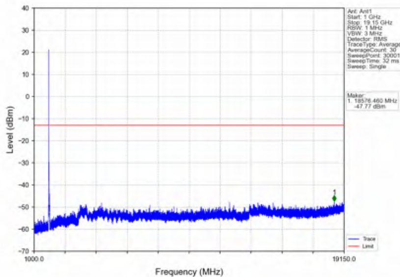
n25_15kHz_SISO_NTV_25MHz_CP-OFDM QPSK_1882.5MHz_Edge_1RB_Left
