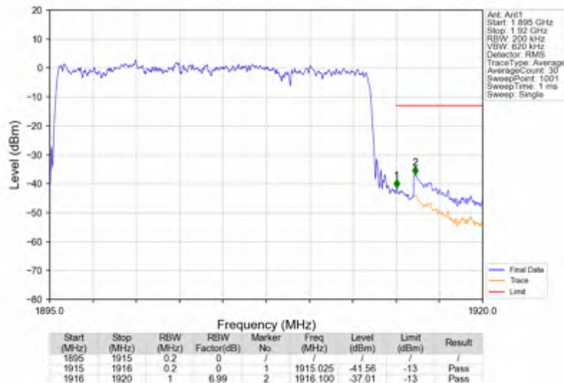
n25_15kHz_SISO_NTNV_20MHz_DFT-s-OFDM PI/2 BPSK_1905MHz_Outer_Full
