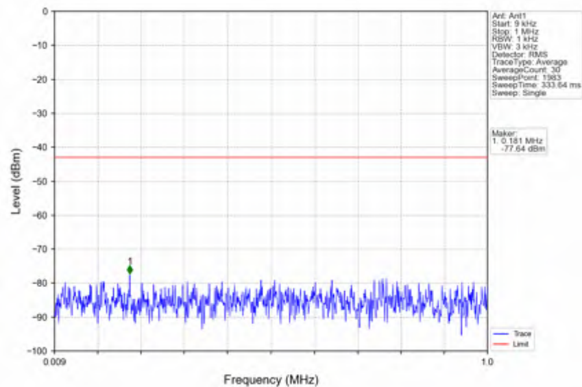
n25_15kHz_SISO_NTNV_20MHz_CP-OFDM_QPSK_1860MHz_Outer_Full
