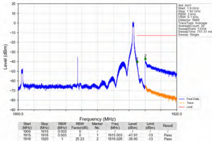
n25_15kHz_SISO_NTNV_15MHz_CP-OFDM QPSK_1907.5MHz_Edge_1RB_Right
