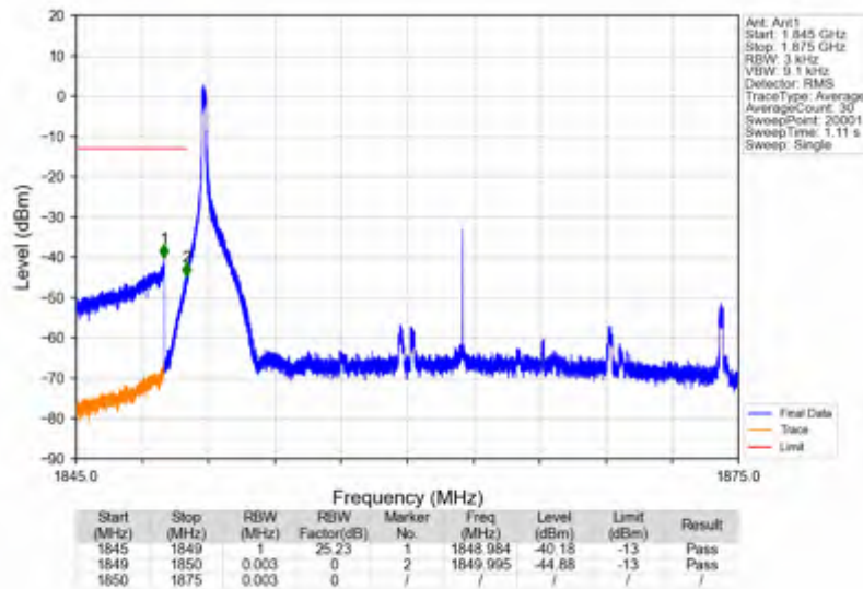
n25_15kHz_SISO_NTV_25MHz_CP-OFDM_QPSK_1862.5MHz_Inner_1RB_Left
