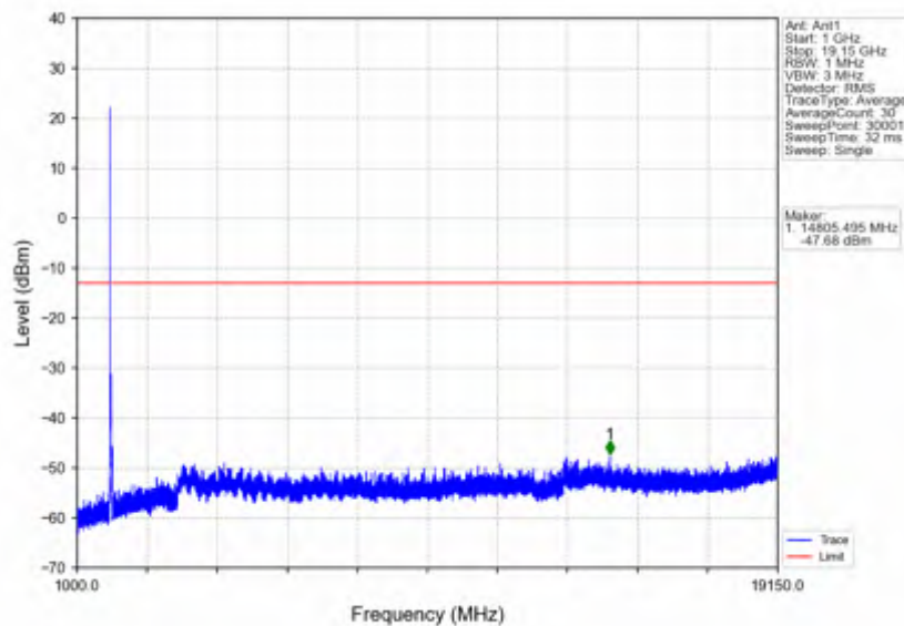
n25_15kHz_SISO_NTNV_30MHz_DFT-s-OFDM PI/2 BPSK_1865MHz_Outer_Full
