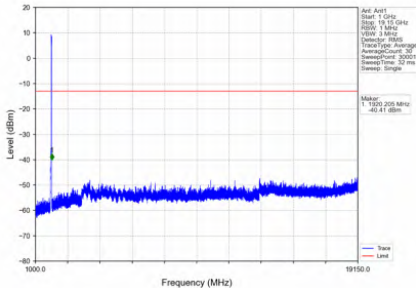
n25_15kHz_SISO_NTNV_40MHz_DFT-s-OFDM_PI/2_BPSK_1895MHz_Outer_Full
