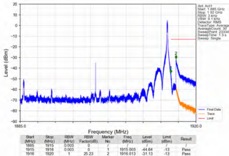
n25_15kHz_SISO_NTNV_30MHz_DFT-s-OFDM_QPSK_1900MHz_Edge_1RB_Right
