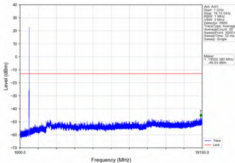
n25_15kHz_SISO_NTNV_20MHz_DFT-s-OFDM QPSK_1905MHz_Inner_1RB_Right
