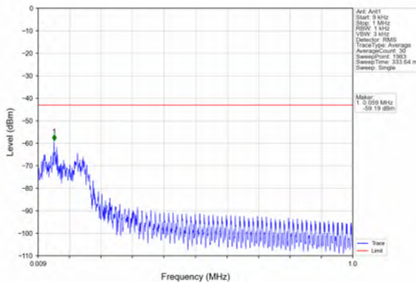
n25_15kHz_SISO_NTNV_40MHz_DFT-s-OFDM PI/2 BPSK_1895MHz_Edge_1RB_Right
