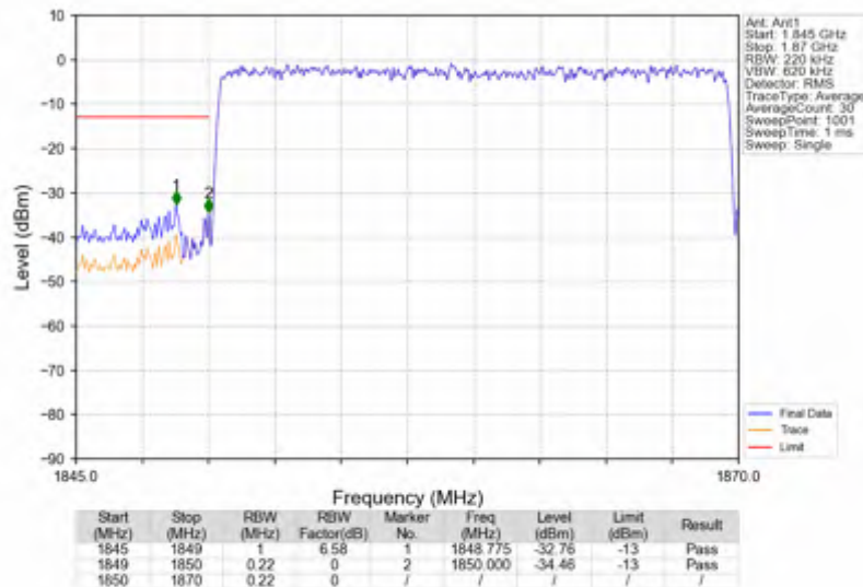
n25_15kHz_SISO_NTNV_20MHz_CP-OFDM QPSK_1860MHz_Outer_Full
