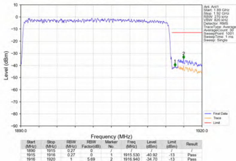
n25_15kHz_SISO_NTNV_25MHz_CP-OFDM QPSK_1902.5MHz_Outer_Full
