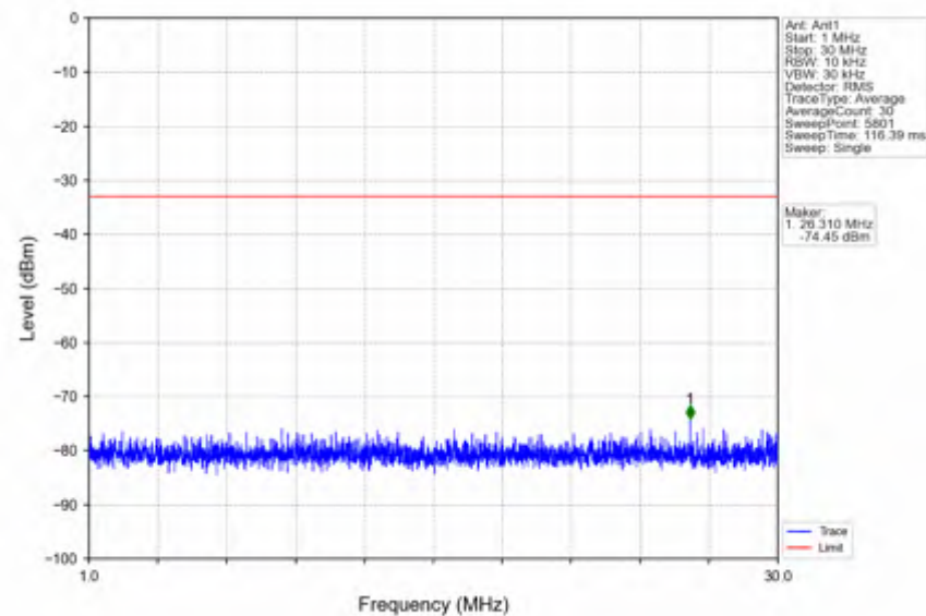
n25_15kHz_SISO_NTNV_30MHz_DFT-s-OFDM QPSK_1900MHz_Outer_Full
