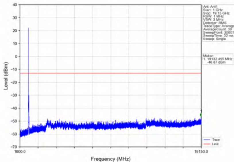
n25_15kHz_SISO_NTNV_40MHz_DFT-s-OFDM PI/2 BPSK_1870MHz_Outer_Full
