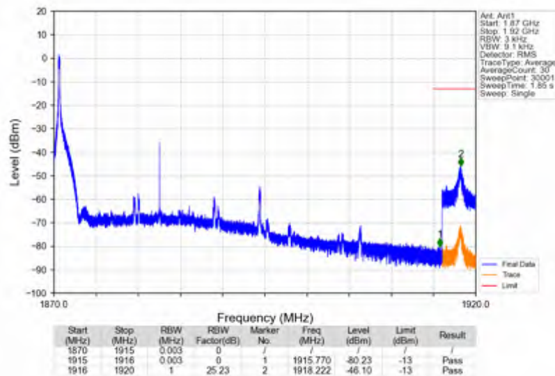
n25_15kHz_SISO_NTV_25MHz_CP-OFDM QPSK_1882.5MHz_Edge_1RB_Left
