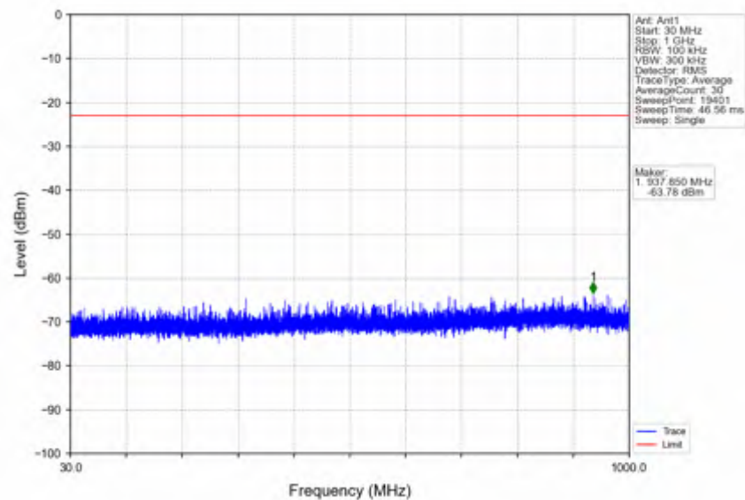
n25_15kHz_SISO_NTNV_15MHz_CP-OFDM QPSK_1907.5MHz_Inner_1RB_Right
