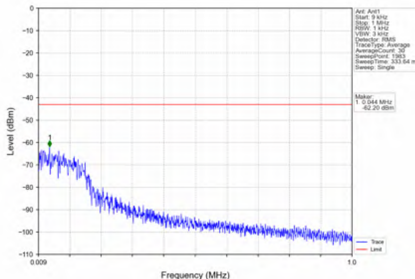
n25_15kHz_SISO_NTNV_20MHz_CP-OFDM_QPSK_1905MHz_Edge_1RB_Right
