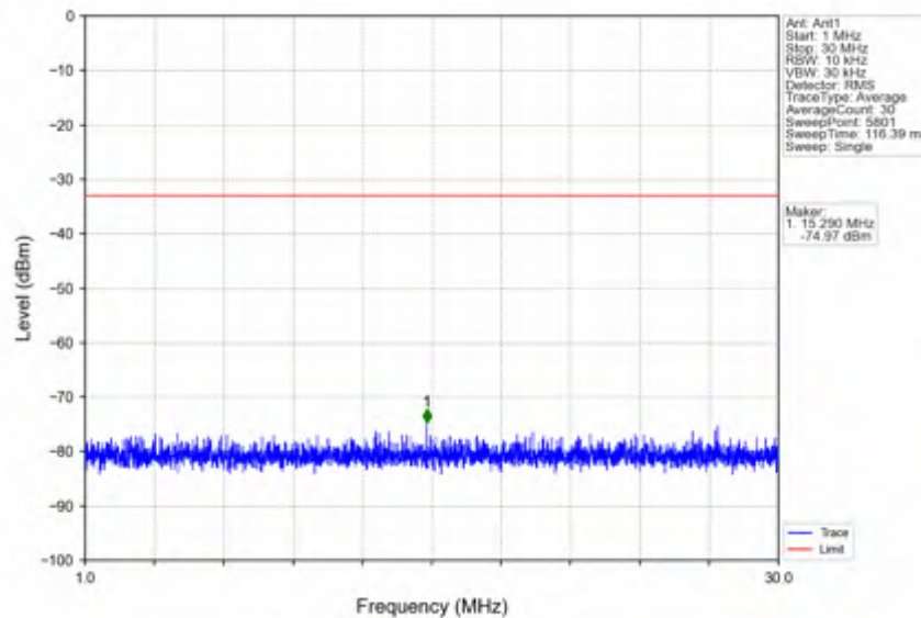
n25_15kHz_SISO_NTNV_25MHz_CP-OFDM_QPSK_1882.5MHz_Edge_1RB_Left
