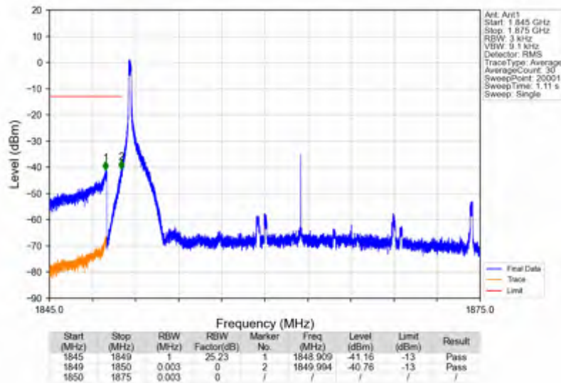
n25_15kHz_SISO_NTNV_25MHz_CP-OFDM_QPSK_1862.5MHz_Edge_1RB_Left
