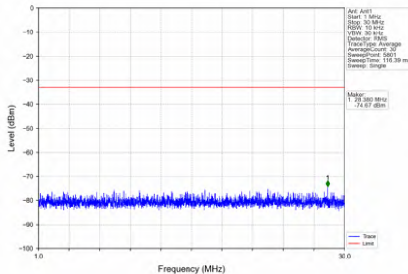
n25_15kHz_SISO_NTNV_30MHz_CP-OFDM QPSK_1900MHz_Edge_1RB_Right
