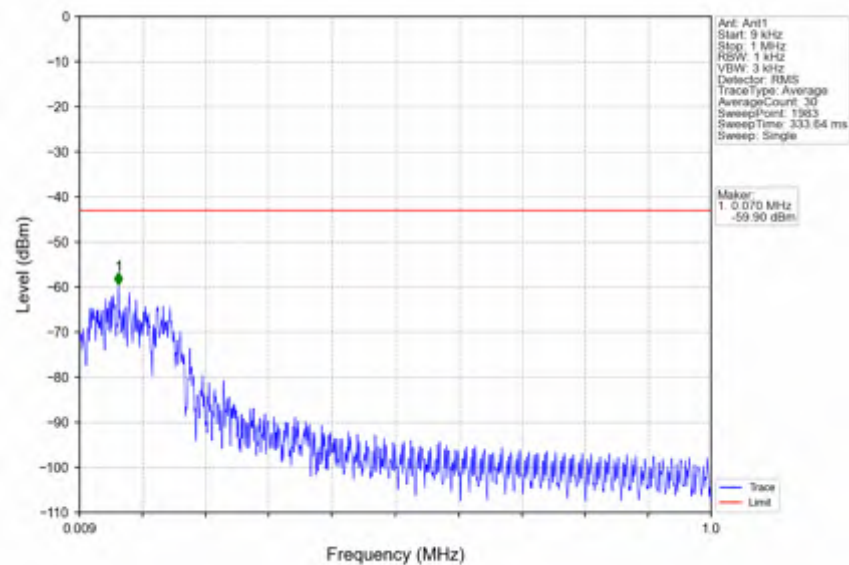
n25_15kHz_SISO_NTNV_25MHz_DFT-s-OFDM QPSK_1902.5MHz_Edge_1RB_Right
