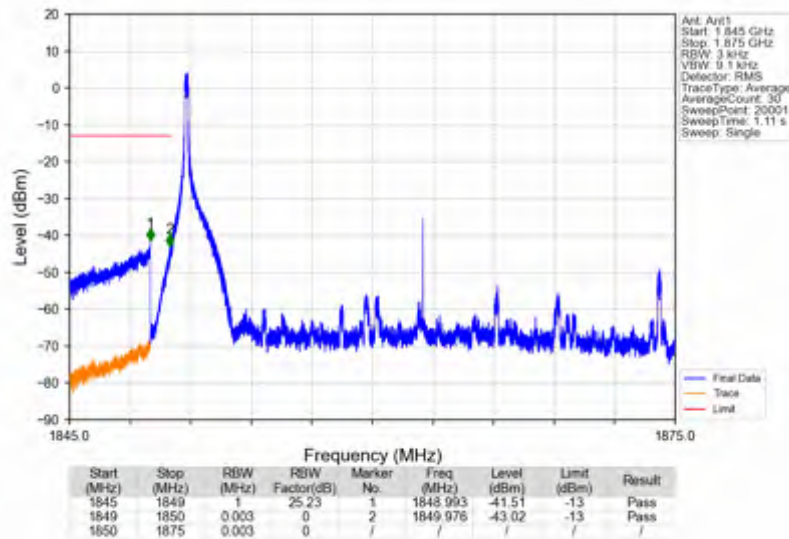
n25_15kHz_SISO_NTNV_25MHz_DFT-s-OFDM_QPSK_1862.5MHz_Inner_1RB_Left
