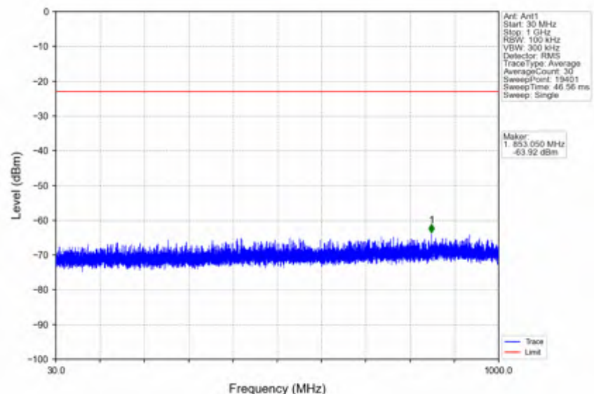
n25_15kHz_SISO_NTNV_20MHz_DFT-s-OFDM QPSK_1905MHz_Outer_Full
