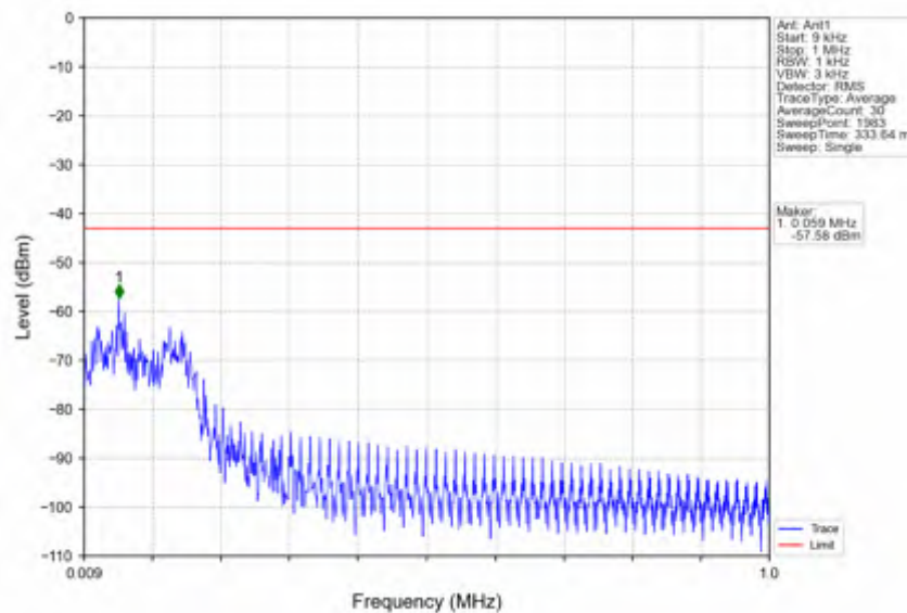
n25_15kHz_SISO_NTNV_30MHz_DFT-s-OFDM PI/2 BPSK_1900MHz_Inner_1RB_Right
