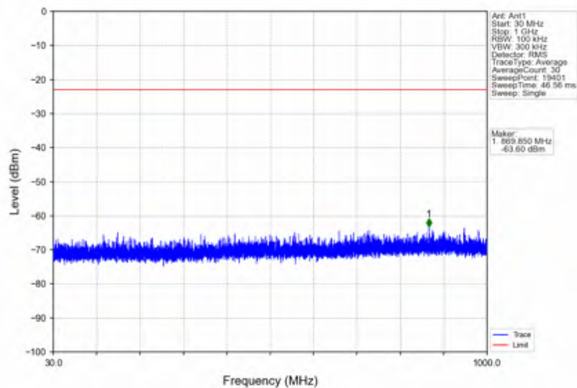
n25_15kHz_SISO_NTNV_20MHz_DFT-s-OFDM PI/2 BPSK_1905MHz_Outer_Full
