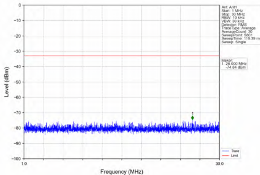
n25_15kHz_SISO_NTNV_20MHz_CP-OFDM_QPSK_1860MHz_Edge_1RB_Left
