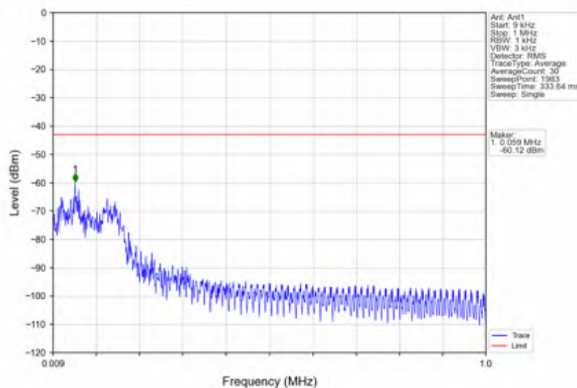
n25_15kHz_SISO_NTNV_25MHz_DFT-s-OFDM PI/2 BPSK_1862.5MHz_Edge_1RB_Left
