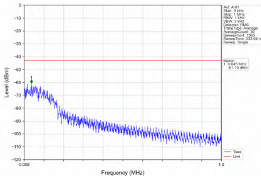
n25_15kHz_SISO_NTNV_30MHz_CP-OFDM_QPSK_1900MHz_Edge_1RB_Right
