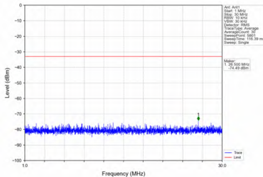
n25_15kHz_SISO_NTNV_30MHz_DFT-s-OFDM_QPSK_1865MHz_Edge_1RB_Left
