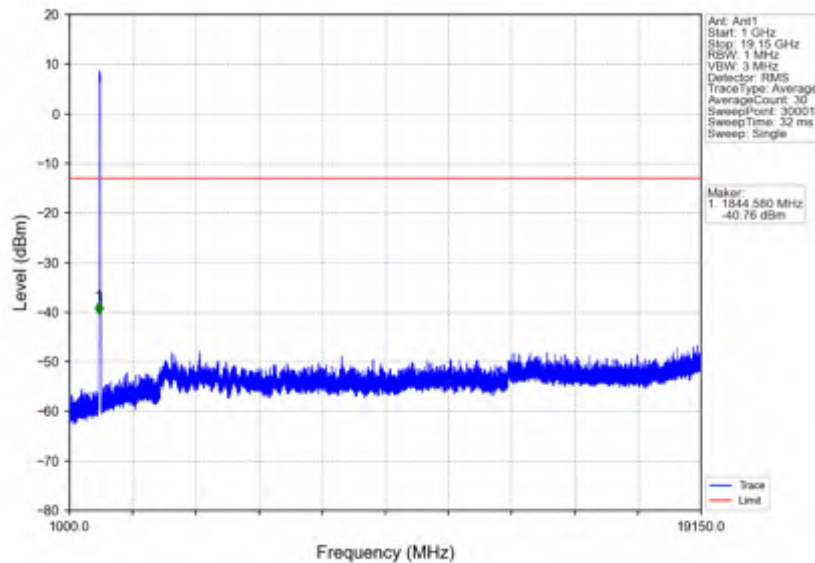
n25_15kHz_SISO_NTNV_40MHz_DFT-s-OFDM_PI/2_BPSK_1870MHz_Outer_Full
