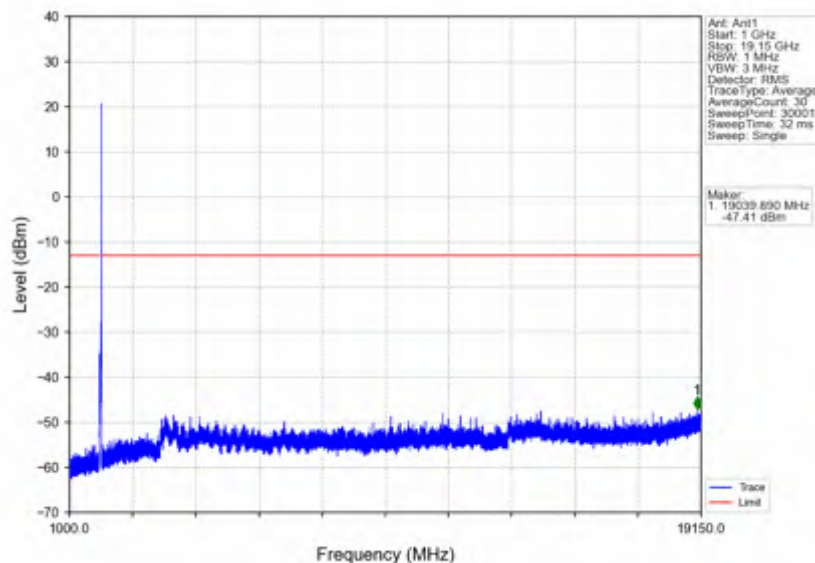
n25_15kHz_SISO_NTNV_25MHz_CP-OFDM QPSK_1902.5MHz_Outer_Full
