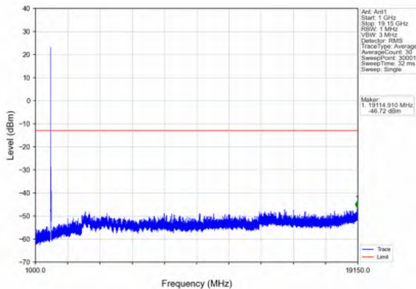
n25_15kHz_SISO_NTNV_20MHz_DFT-s-OFDM PI/2 BPSK_1882.5MHz_Edge_1RB_Left
