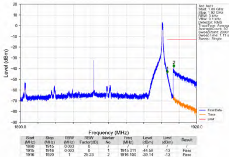
n25_15kHz_SISO_NTNV_25MHz_CP-OFDM_QPSK_1902.5MHz_Inner_1RB_Right
