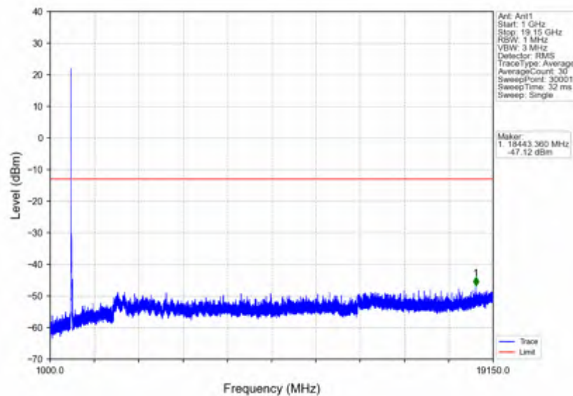
n25_15kHz_SISO_NTNV_30MHz_DFT-s-OFDM_QPSK_1865MHz_Edge_1RB_Left
