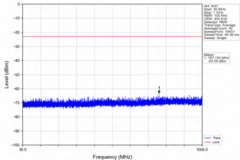
n25_15kHz_SISO_NTNV_15MHz_CP-OFDM QPSK_1907.5MHz_Edge_1RB_Right
