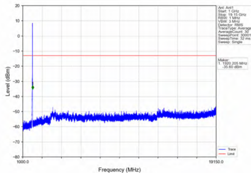
n25 15kHz SISO NTNV 25MHz CP-OFDM QPSK 1902.5MHz Outer Full
