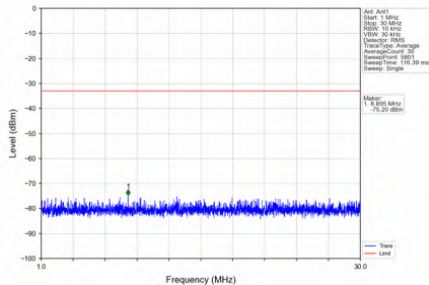
n25_15kHz_SISO_NTNV_20MHz_DFT-s-OFDM QPSK_1860MHz_Outer_Full
