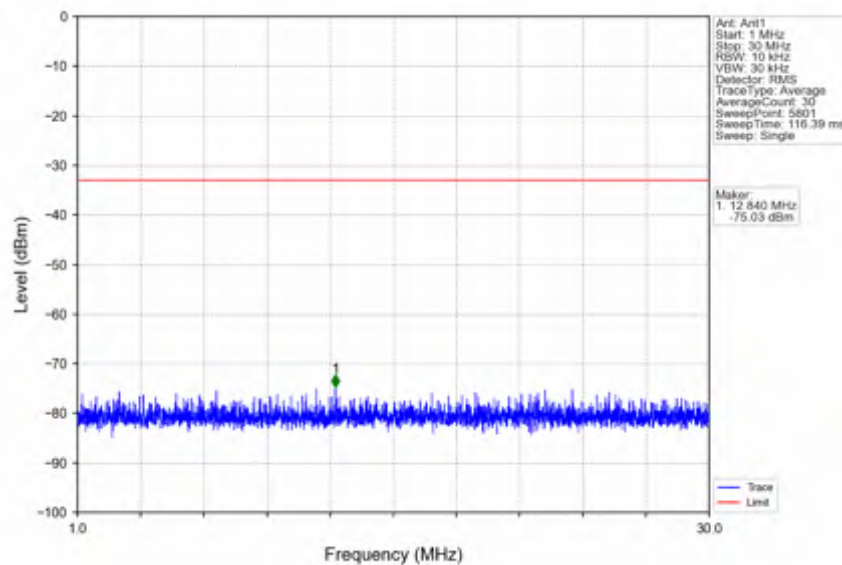
n25_15kHz_SISO_NTNV_40MHz_DFT-s-OFDM_PI/2_BPSK_1870MHz_Outer_Full
