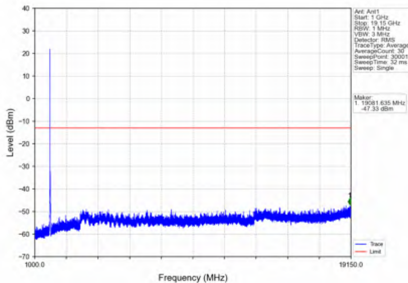
n25_15kHz_SISO_NTNV_30MHz_DFT-s-OFDM_QPSK_1900MHz_Edge_1RB_Right
