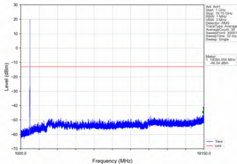
n25_15kHz_SISO_NTNV_20MHz_CP-OFDM QPSK_1905MHz_Outer_Full
