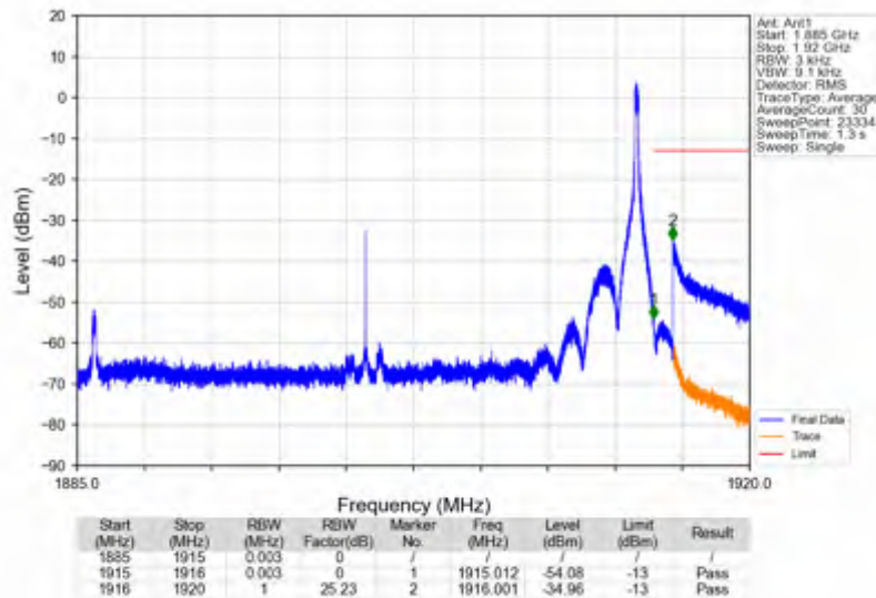
n25_15kHz_SISO_NTNV_30MHz_CP-OFDM QPSK_1900MHz_Inner_1RB_Right
