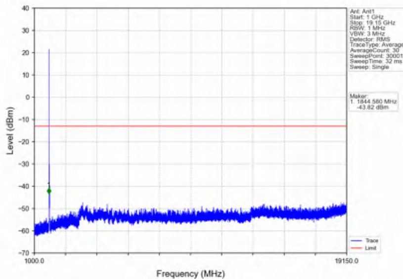
n25_15kHz_SISO_NTNV_20MHz_CP-OFDM QPSK_1882.5MHz_Edge_1RB_Left
