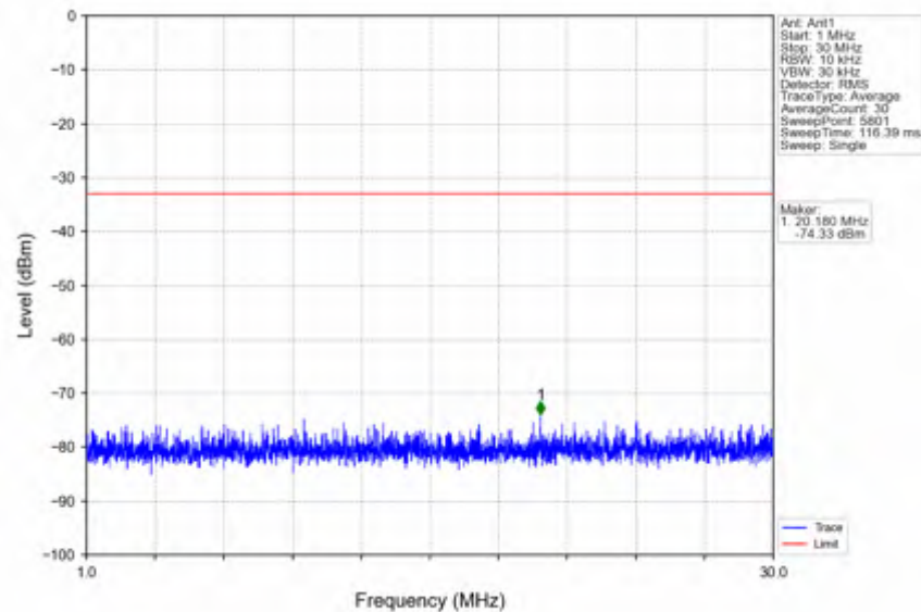
n25_15kHz_SISO_NTNV_20MHz_CP-OFDM QPSK_1905MHz_Edge_1RB_Right
