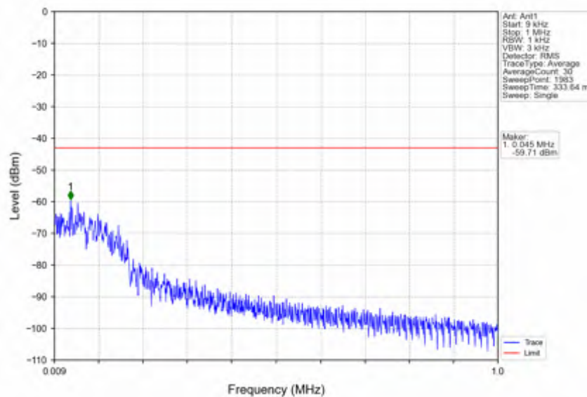
n25_15kHz_SISO_NTNV_25MHz_CP-OFDM_QPSK_1902.5MHz_Edge_1RB_Right
