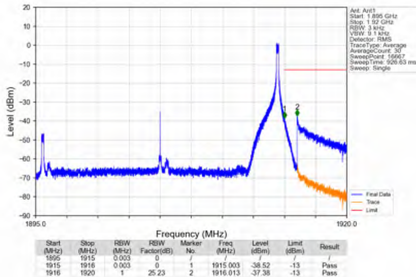
n25_15kHz_SISO_NTNV_20MHz_CP-OFDM_QPSK_1905MHz_Edge_1RB_Right
