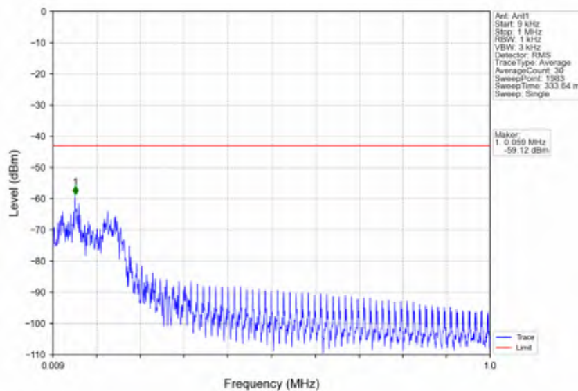
n25_15kHz_SISO_NTNV_30MHz_DFT-s-OFDM PI/2 BPSK_1900MHz_Edge_1RB_Right
