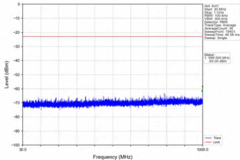
n25_15kHz_SISO_NTNV_25MHz_DFT-s-OFDM QPSK_1902.5MHz_Inner_1RB_Right
