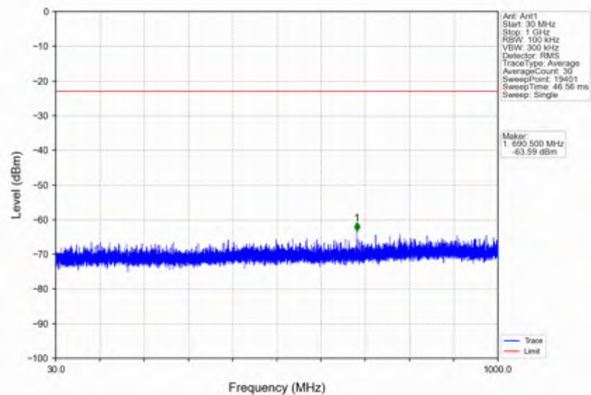
n25_15kHz_SISO_NTNV_25MHz_DFT-s-OFDM_QPSK_1862.5MHz_Outer_Full
