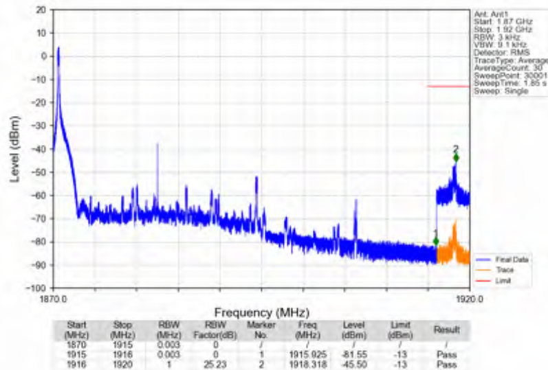
n25_15kHz_SISO_NTNV_25MHz_DFT-s-OFDM PI/2 BPSK_1882.5MHz_Edge_1RB_Left
