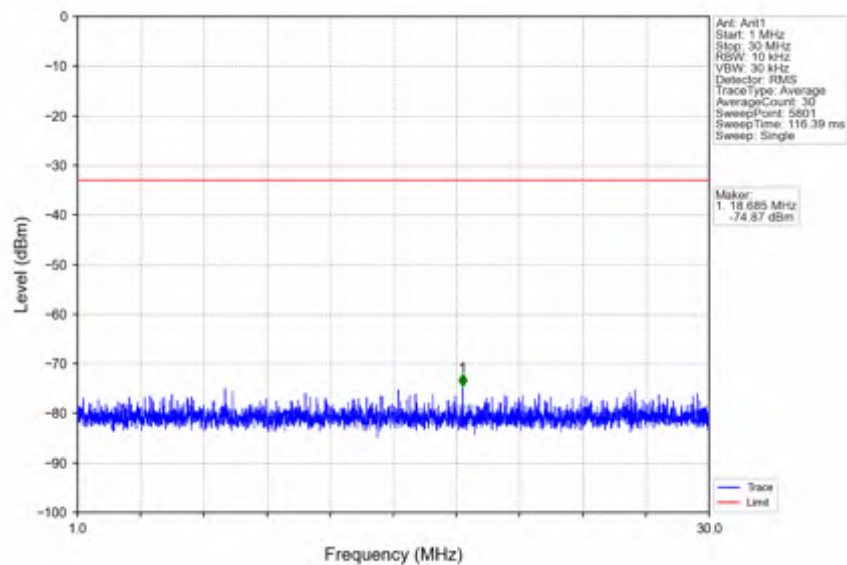
n25_15kHz_SISO_NTNV_30MHz_CP-OFDM QPSK_1865MHz_Outer_Full
