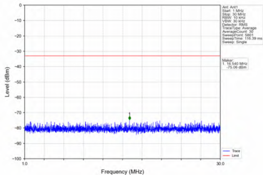
n25_15kHz_SISO_NTNV_15MHz_CP-OFDM_QPSK_1907.5MHz_Outer_Full
