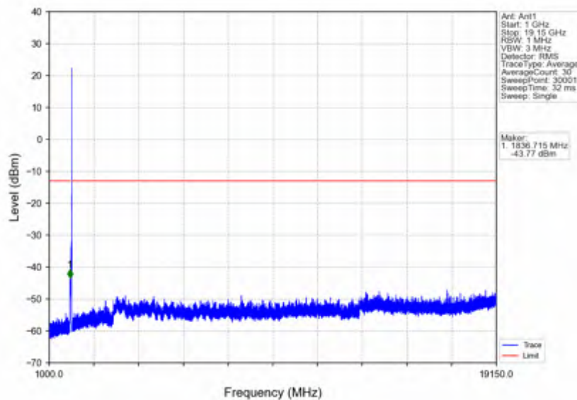
n25_15kHz_SISO_NTNV_40MHz_DFT-s-OFDM PI/2 BPSK_1895MHz_Outer_Full
