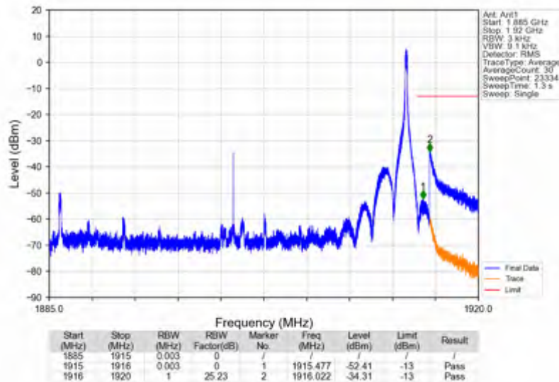
n25_15kHz_SISO_NTNV_30MHz_DFT-s-OFDM QPSK_1900MHz_Inner_1RB_Right
