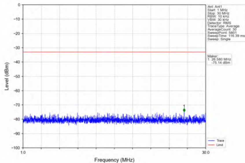
n25_15kHz_SISO_NTNV_20MHz_DFT-s-OFDM_PI/2_BPSK_1860MHz_Outer_Full
