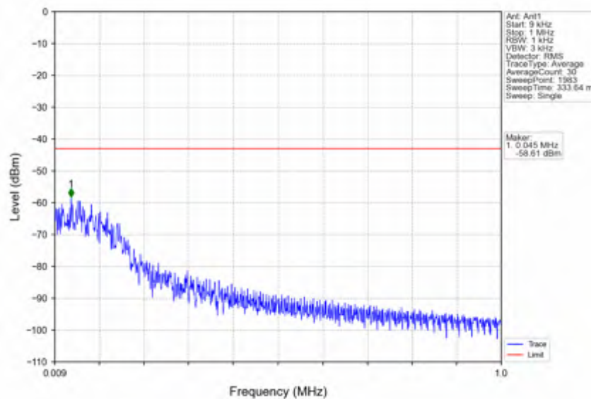
n25_15kHz_SISO_NTV_25MHz_CP-OFDM_QPSK_1862.5MHz_Inner_1RB_Left
