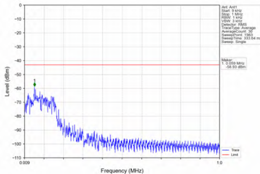
n25_15kHz_SISO_NTNV_20MHz_DFT-s-OFDM QPSK_1905MHz_Edge_1RB_Right
