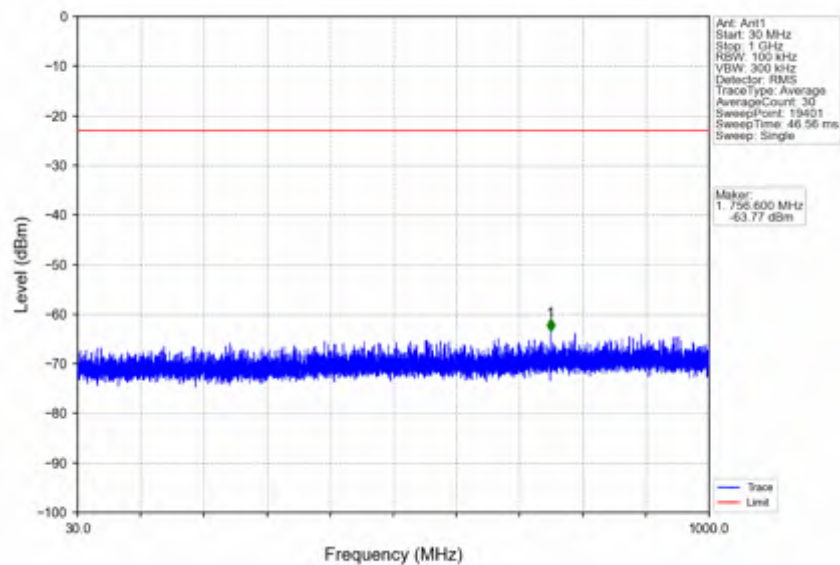
n25_15kHz_SISO_NTNV_20MHz_DFT-s-OFDM_PI/2_BPSK_1905MHz_Edge_1RB_Right
