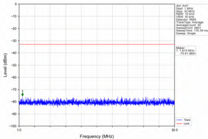
n25_15kHz_SISO_NTNV_30MHz_CP-OFDM QPSK_1865MHz_Edge_1RB_Left
