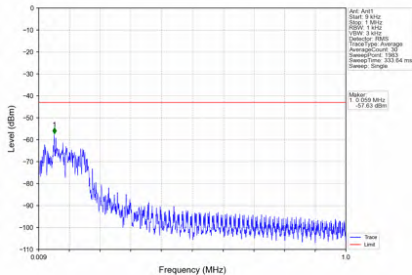
n25_15kHz_SISO_NTNV_20MHz_DFT-s-OFDM QPSK_1905MHz_Inner_1RB_Right
