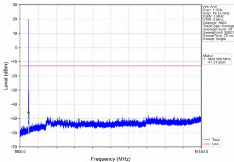
n25_15kHz_SISO_NTNV_30MHz_CP-OFDM QPSK_1865MHz_Outer_Full
