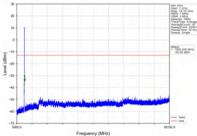
n25_15kHz_SISO_NTNV_25MHz_DFT-s-OFDM QPSK_1902.5MHz_Inner_1RB_Right
