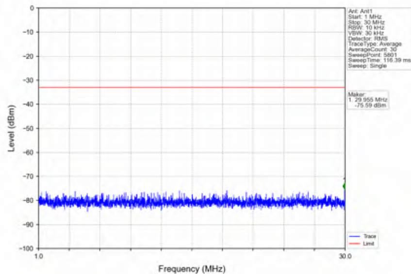
n25_15kHz_SISO_NTNV_25MHz_DFT-s-OFDM_QPSK_1902.5MHz_Outer_Full
