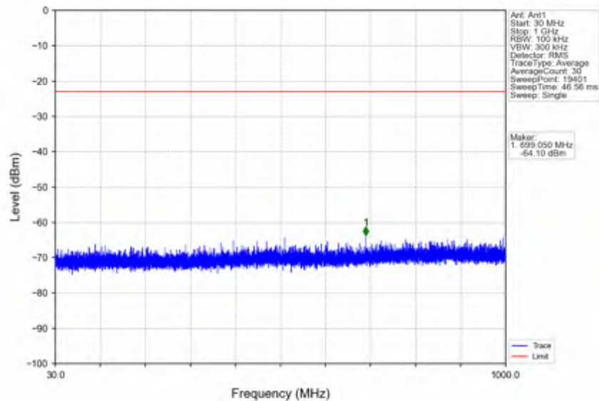
n25_15kHz_SISO_NTNV_40MHz_DFT-s-OFDM_PI/2_BPSK_1895MHz_Outer_Full
