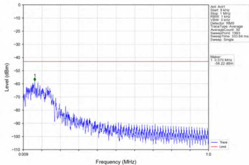
n25_15kHz_SISO_NTNV_25MHz_DFT-s-OFDM QPSK_1902.5MHz_Inner_1RB_Right
