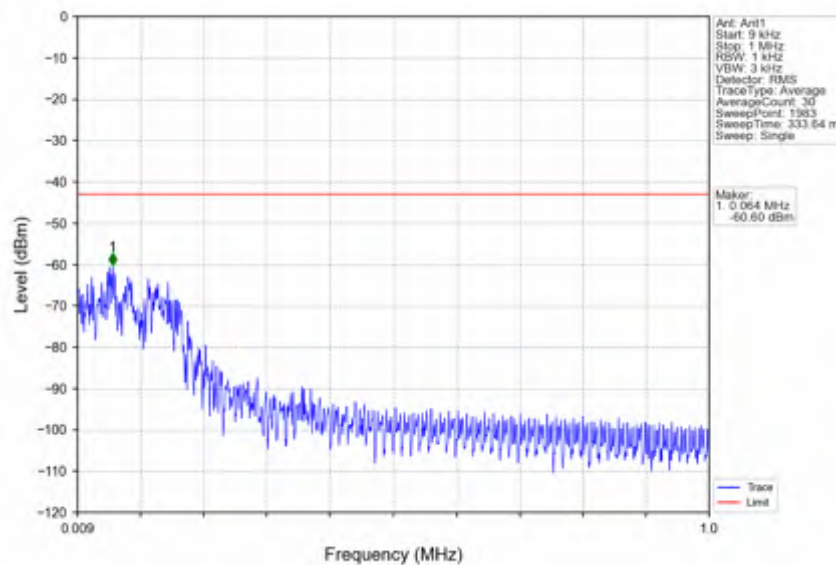
n25_15kHz_SISO_NTNV_20MHz_DFT-s-OFDM_PI/2_BPSK_1905MHz_Edge_1RB_Right
