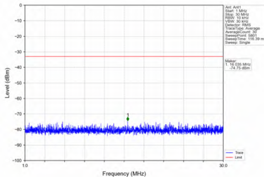
n25_15kHz_SISO_NTNV_20MHz_CP-OFDM QPSK_1905MHz_Inner_1RB_Right
