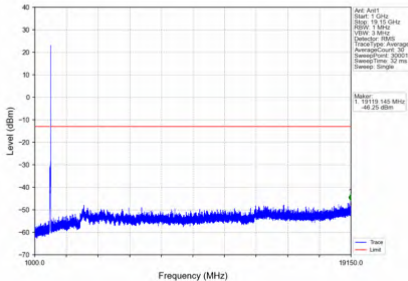
n25_15kHz_SISO_NTNV_30MHz_DFT-s-OFDM QPSK_1900MHz_Inner_1RB_Right
