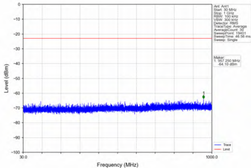
n25_15kHz_SISO_NTNV_40MHz_DFT-s-OFDM_PI/2_BPSK_1870MHz_Outer_Full
