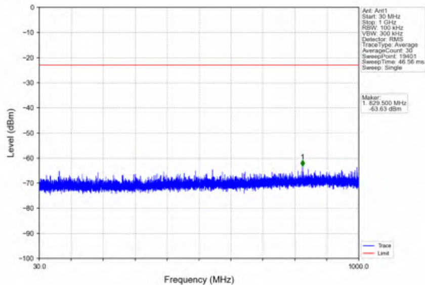
n25_15kHz_SISO_NTNV_25MHz_CP-OFDM QPSK_1862.5MHz_Edge_1RB_Left
