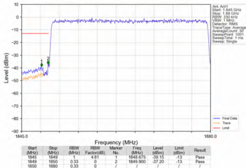
n25_15kHz_SISO_NTNV_30MHz_CP-OFDM QPSK_1865MHz_Outer_Full
