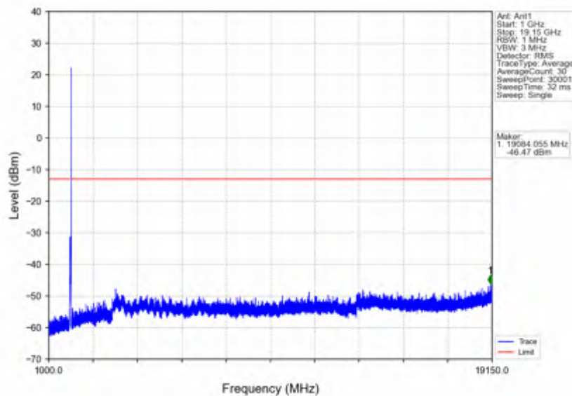
n25_15kHz_SISO_NTNV_25MHz_DFT-s-OFDM PI/2 BPSK_1902.5MHz_Outer_Full
