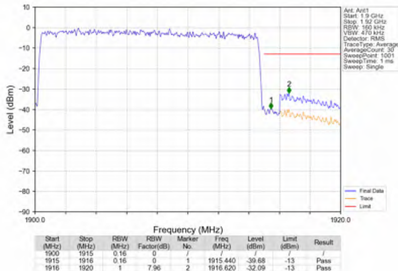
n25_15kHz_SISO_NTNV_15MHz_CP-OFDM QPSK_1907.5MHz_Outer_Full
