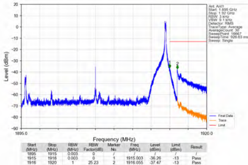
n25_15kHz_SISO_NTNV_20MHz_DFT-s-OFDM QPSK_1905MHz_Edge_1RB_Right
