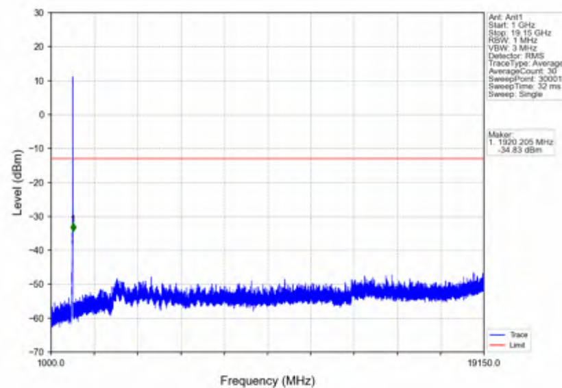
n25 15kHz SISO NTNV 15MHz CP-OFDM QPSK 1907.5MHz Outer Full
