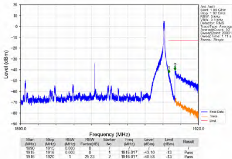
n25_15kHz_SISO_NTNV_25MHz_DFT-s-OFDM QPSK_1902.5MHz_Inner_1RB_Right
