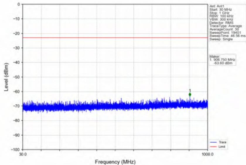
n25_15kHz_SISO_NTNV_20MHz_CP-OFDM QPSK_1905MHz_Outer_Full
