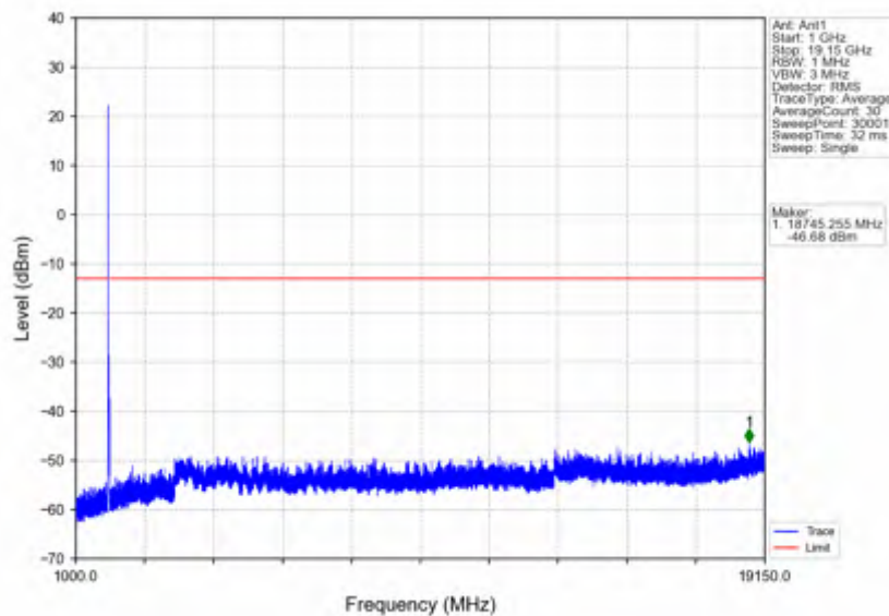
n25_15kHz_SISO_NTNV_20MHz_DFT-s-OFDM PI/2 BPSK_1860MHz_Outer_Full
