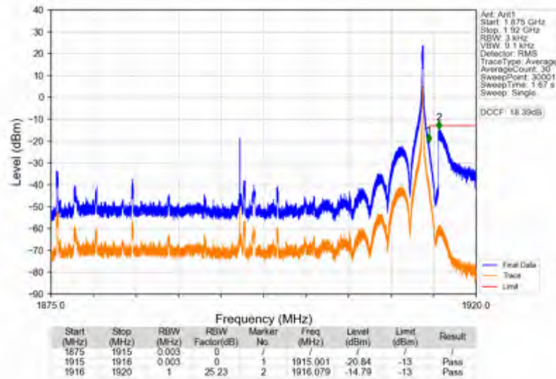
n25_15kHz_SISO_NTNV_40MHz_DFT-s-OFDM PI/2 BPSK_1895MHz_Edge_1RB_Right
