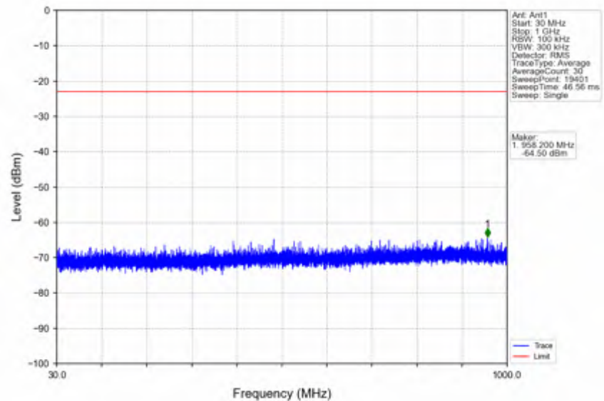
n25_15kHz_SISO_NTNV_25MHz_CP-OFDM QPSK_1902.5MHz_Edge_1RB_Right
