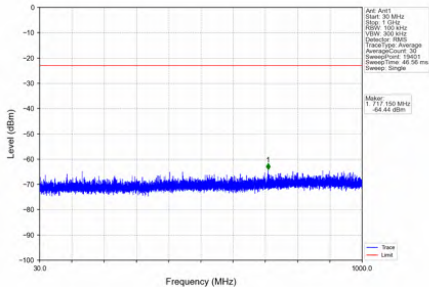
n25_15kHz_SISO_NTNV_25MHz_DFT-s-OFDM QPSK_1902.5MHz_Edge_1RB_Right
