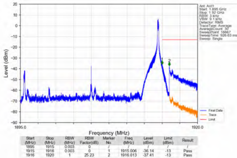
n25_15kHz_SISO_NTNV_20MHz_DFT-s-OFDM_PI/2_BPSK_1905MHz_Edge_1RB_Right
