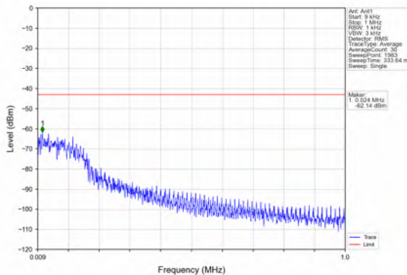
n25_15kHz_SISO_NTNV_15MHz_CP-OFDM QPSK_1907.5MHz_Edge_1RB_Right
