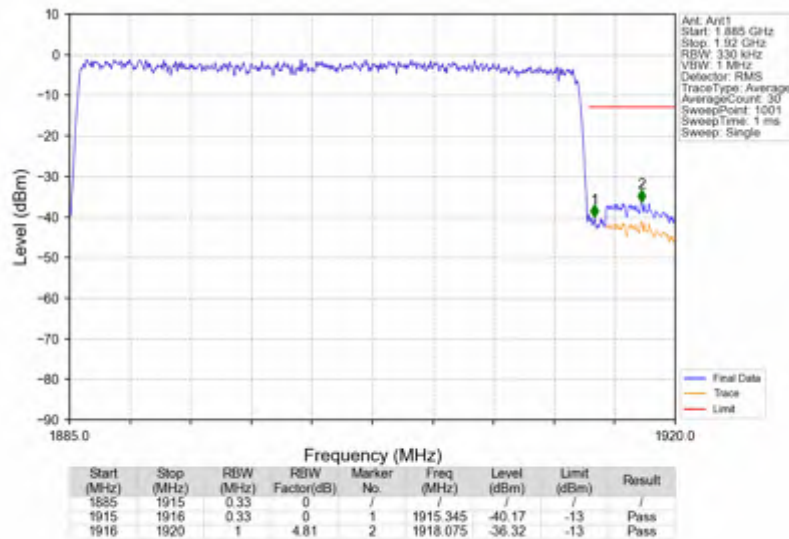
n25_15kHz_SISO_NTNV_30MHz_CP-OFDM QPSK_1900MHz_Outer_Full
