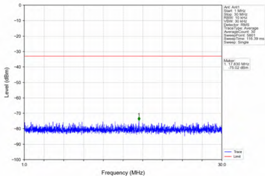
n25_15kHz_SISO_NTNV_20MHz_CP-OFDM QPSK_1905MHz_Outer_Full
