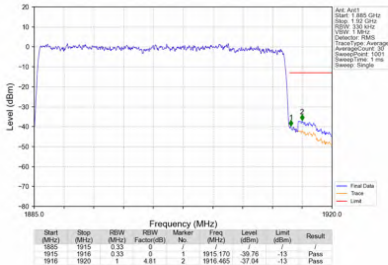
n25_15kHz_SISO_NTNV_30MHz_DFT-s-OFDM PI/2 BPSK_1900MHz_Outer_Full
