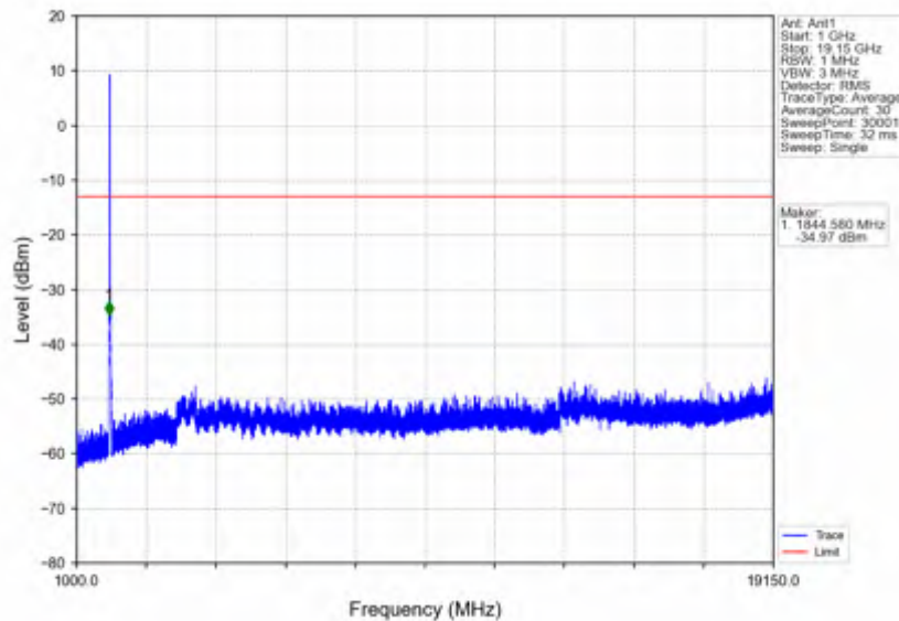
n25_15kHz_SISO_NTNV_20MHz_CP-OFDM QPSK_1860MHz_Outer_Full
