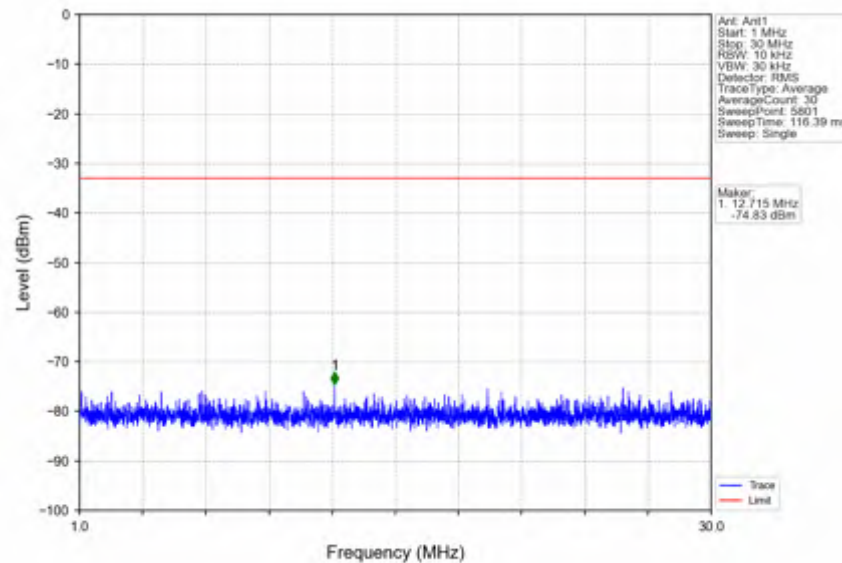
n25_15kHz_SISO_NTV_25MHz_CP-OFDM_QPSK_1862.5MHz_Inner_1RB_Left
