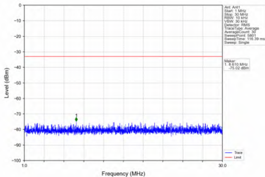
n25_15kHz_SISO_NTNV_20MHz_DFT-s-OFDM_PI/2_BPSK_1905MHz_Edge_1RB_Right
