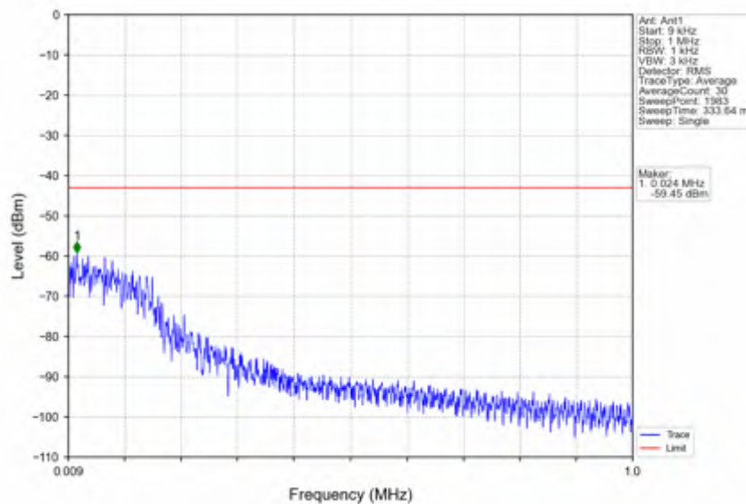
n25_15kHz_SISO_NTNV_20MHz_CP-OFDM QPSK_1905MHz_Inner_1RB_Right
