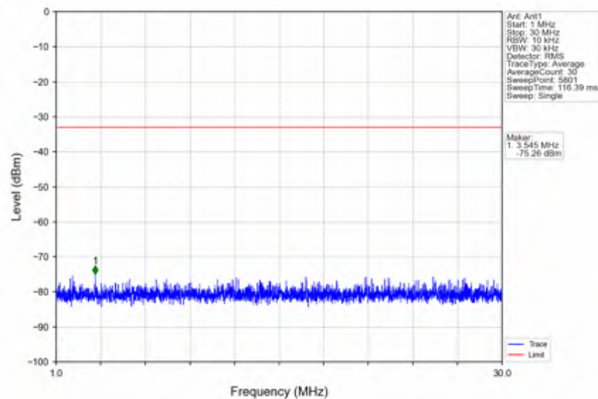
n25_15kHz_SISO_NTNV_30MHz_DFT-s-OFDM QPSK_1900MHz_Edge_1RB_Right
