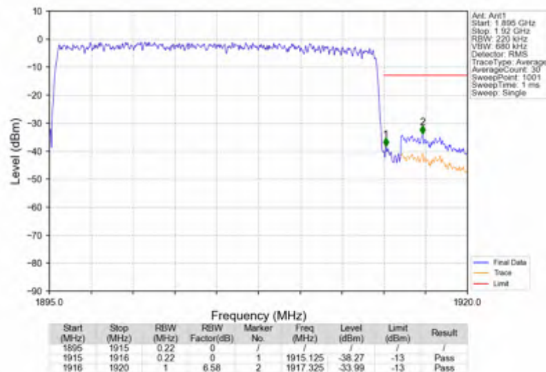
n25_15kHz_SISO_NTNV_20MHz_CP-OFDM QPSK_1905MHz_Outer_Full
