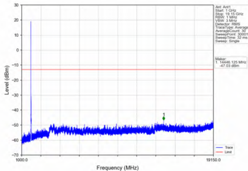
n25_15kHz_SISO_NTNV_30MHz_CP-OFDM QPSK_1882.5MHz_Edge_1RB_Left
