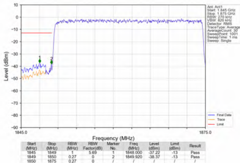
n25_15kHz_SISO_NTV_25MHz_CP-OFDM QPSK_1862.5MHz_Outer_Full
