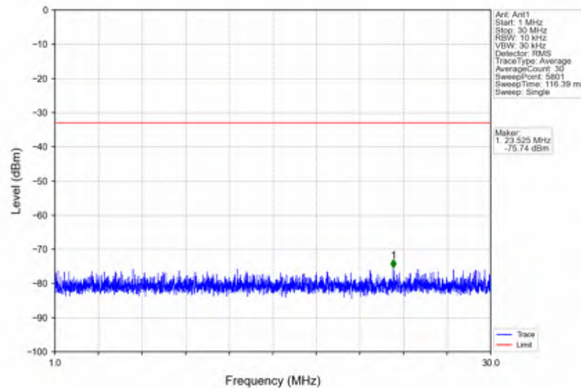
n25_15kHz_SISO_NTNV_30MHz_CP-OFDM QPSK_1900MHz_Inner_1RB_Right
