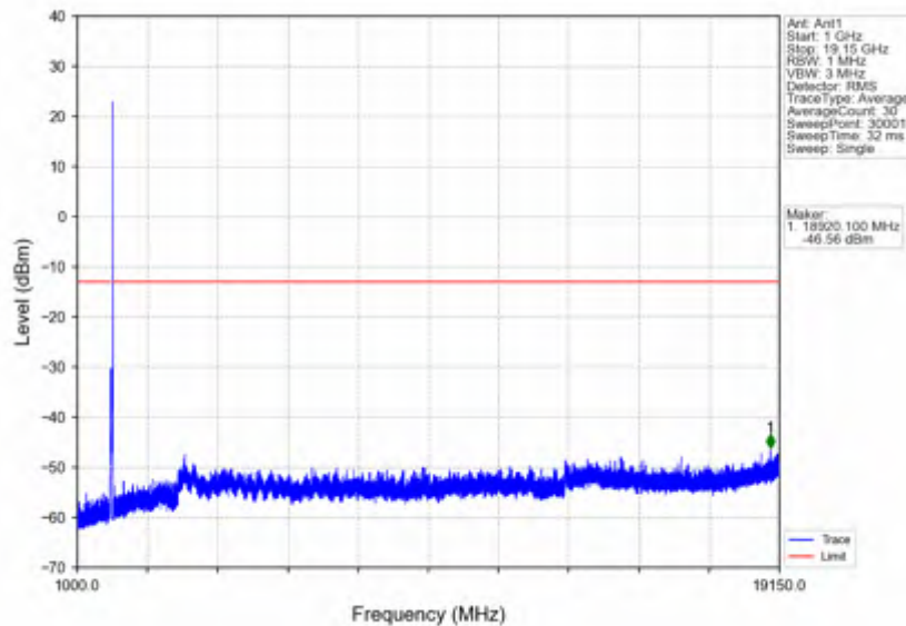
n25_15kHz_SISO_NTNV_25MHz_DFT-s-OFDM QPSK_1902.5MHz_Edge_1RB_Right
