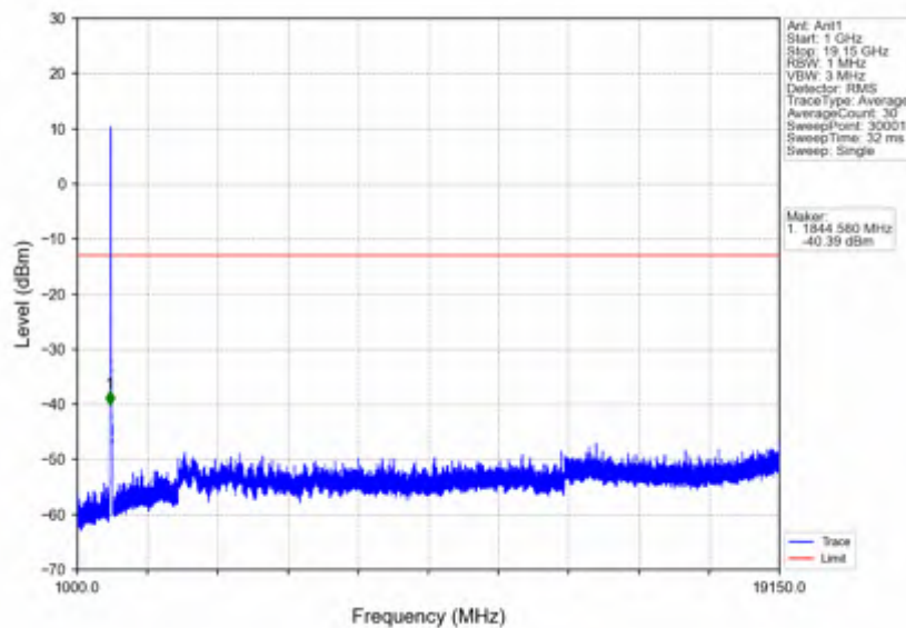
n25_15kHz_SISO_NTNV_25MHz_DFT-s-OFDM_QPSK_1862.5MHz_Inner_1RB_Left
