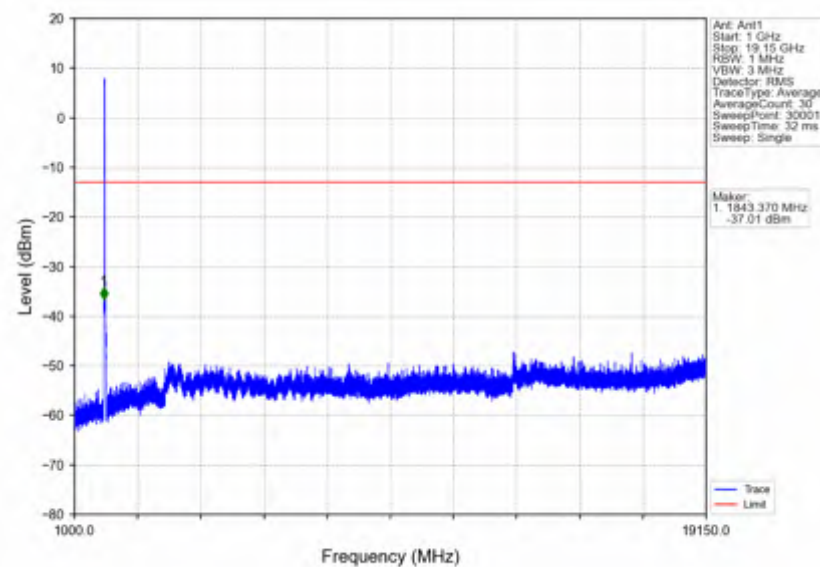
n25_15kHz_SISO_NTNV_25MHz_CP-OFDM QPSK_1862.5MHz_Outer_Full
