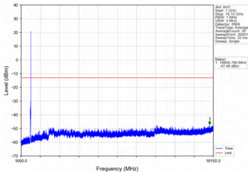
n25_15kHz_SISO_NTNV_30MHz_CP-OFDM QPSK_1900MHz_Outer_Full
