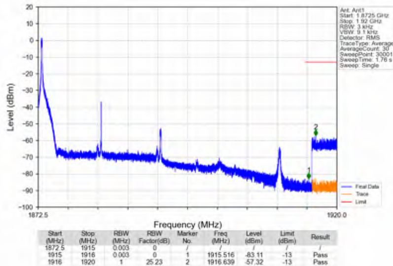
n25_15kHz_SISO_NTNV_20MHz_CP-OFDM QPSK_1882.5MHz_Edge_1RB_Left
