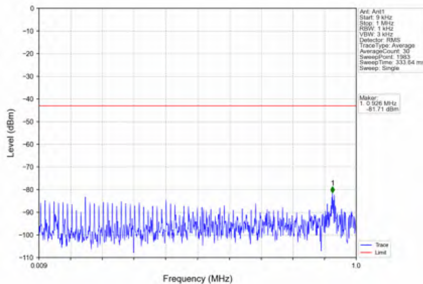
n25_15kHz_SISO_NTNV_30MHz_DFT-s-OFDM PI/2 BPSK_1900MHz_Outer_Full
