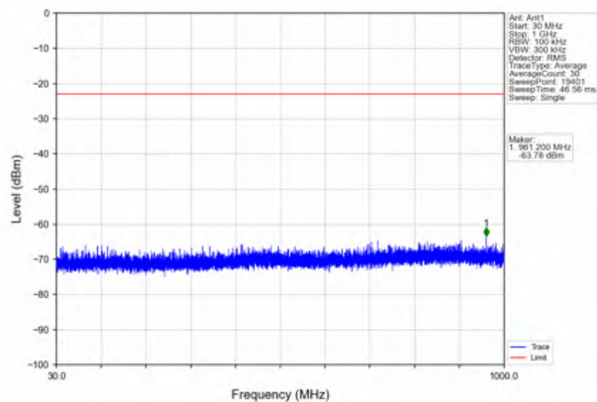
n25_15kHz_SISO_NTNV_30MHz_CP-OFDM QPSK_1900MHz_Edge_1RB_Right
