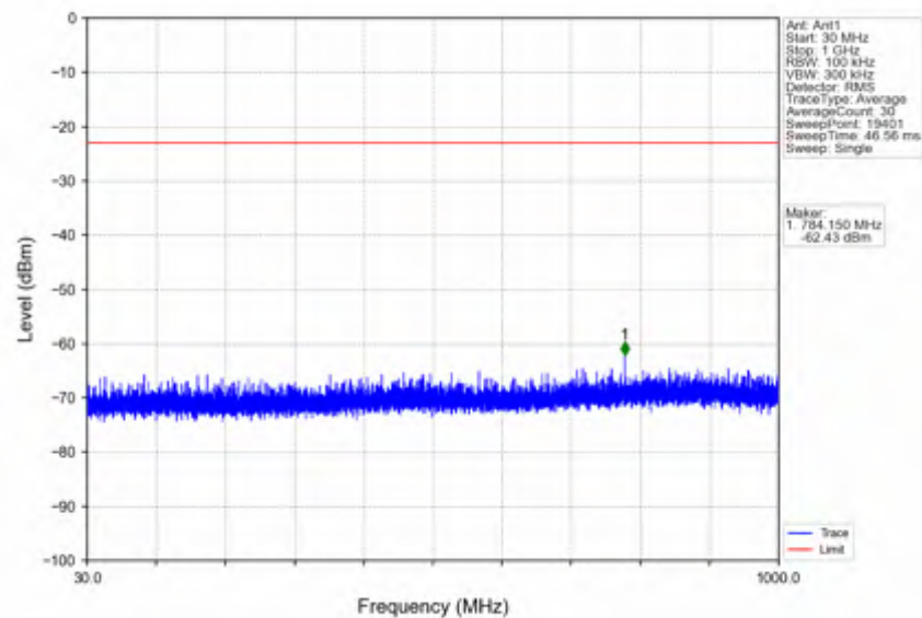
n25 15kHz SISO NTNV 15MHz CP-OFDM QPSK 1907.5MHz Outer Full
