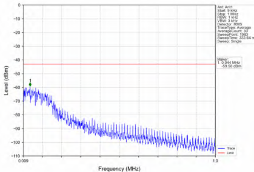
n25_15kHz_SISO_NTNV_15MHz_CP-OFDM_QPSK_1907.5MHz_Inner_1RB_Right
