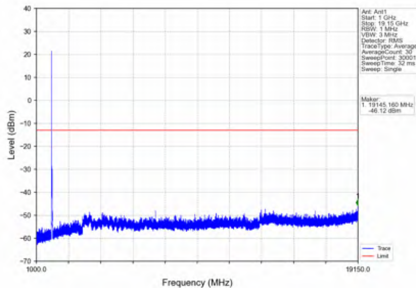
n25_15kHz_SISO_NTNV_40MHz_DFT-s-OFDM QPSK_1870MHz_Edge_1RB_Left
