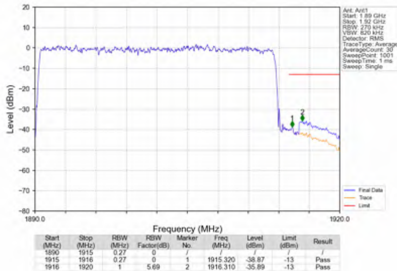
n25_15kHz_SISO_NTNV_25MHz_DFT-s-OFDM PI/2 BPSK_1902.5MHz_Outer_Full
