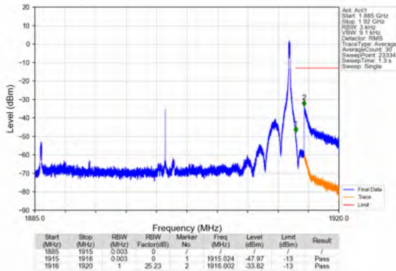
n25_15kHz_SISO_NTNV_30MHz_CP-OFDM_QPSK_1900MHz_Edge_1RB_Right
