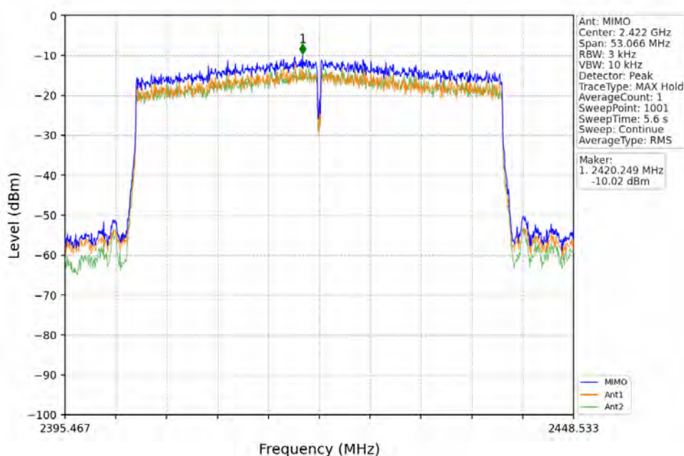
802.11ax(HEW40)_LCH_2422MHz_RU484_Left_MIMO_NTNV
