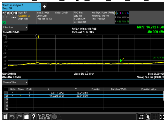
N48(30M)_DFT-s- OFDM_BPSK_Edge_1RB_Left_Mid_CH
