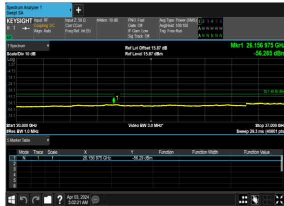
N48(30M)_DFT-s- OFDM_QPSK_Edge_1RB_Left_Low_CH
