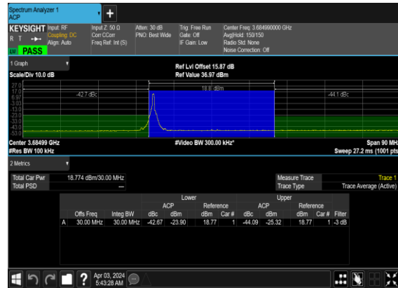
N48(30M)_DFT-s-OFDM_PI_2-BPSK_Edge_1RB_Left_High_CH
