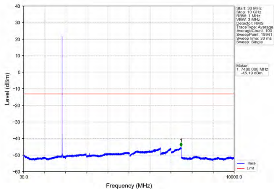
Band2_5MHz_QPSK_LCH_1852.5MHz_RB_1_0_NTNV
