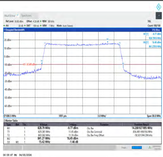
1-N5-15-15-M-8-CP-64QAM-Outer_Full-79@ 0-Ant1-14.201-15.420≤15-PASS
