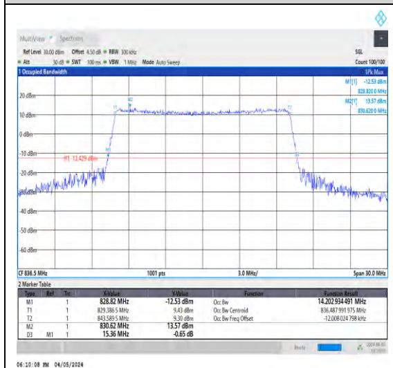
1-N5-15-15-M-9-CP-256QAM-Outer_Full-79 @0-Ant1-14.203-15.360≤15-PASS
