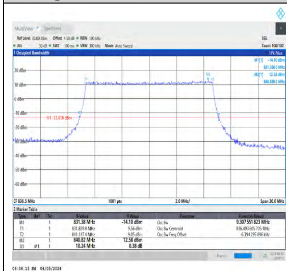
1-N5-15-10-M-6-CP-QPSK-Outer_Full-52@0 -Ant1-9.308-10.240-≤10-PASS
