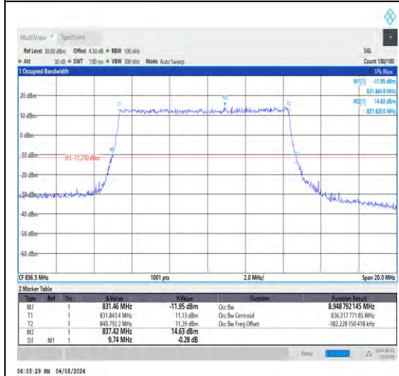
1-N5-15-10-M-4-DFT-64QAM-Outer_Full-50 @0-Ant1-8.949-9.740-≤10-PASS
