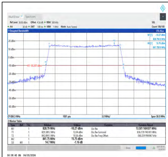
1-N5-15-15-M-5-DFT-256QAM-Outer_Full-75 @0-Ant1-13.501-14.700≤15-PASS
