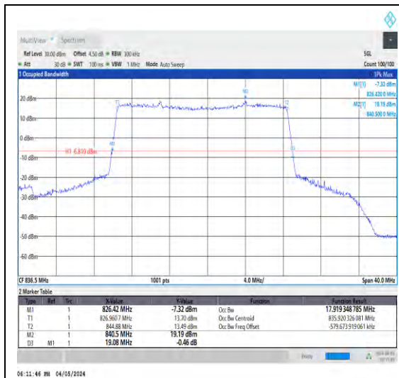
1-N5-15-20-M-2-DFT-PI2BPSK-Outet_Full-1 00@0-Ant1-17.919-19.080-≤20-PASS
