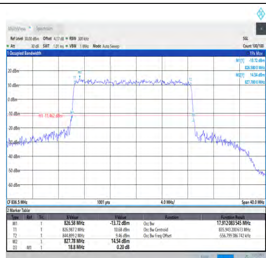
1-N5-15-20-M-3-DFT-16QAM-Outet_Full-100 @0-Ant1-17.912-18.800-≤20-PASS
