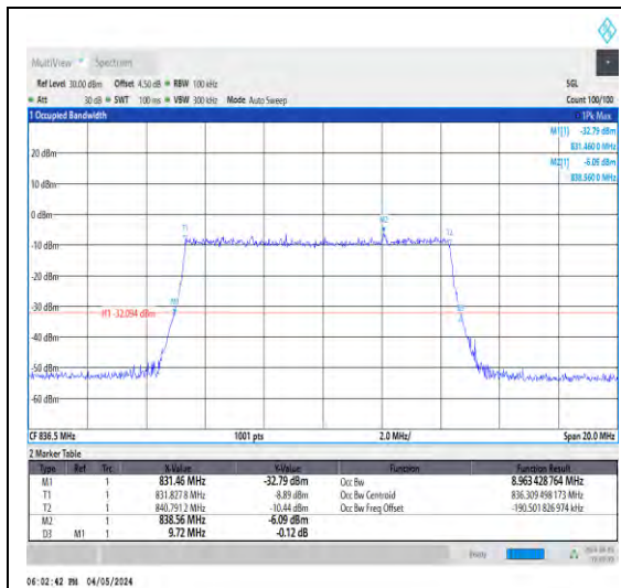
1-N5-15-10-M-2-DFT-PI2BPSK-Outer_Full-5 0@0-Ant1-8.963-9.720-≤10-PASS
