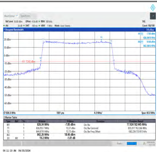
1-N5-15-20-M-1-DFT-QPSK-Outer_Full-100 @0-Ant1-17.924-19.200≤20-PASS
