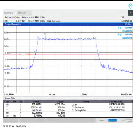
1-N5-15-10-M-5-DFT-256QAM-Outer_Full-50 @0-Ant1-8.952-9.740-≤10-PASS
