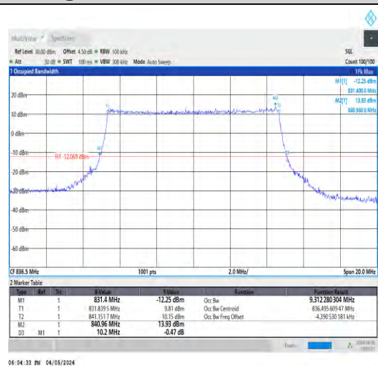
1-N5-15-10-M-7-CP-16QAM-Outer_Full-52@ 0-Ant1-9.312-10.200-≤10-PASS
