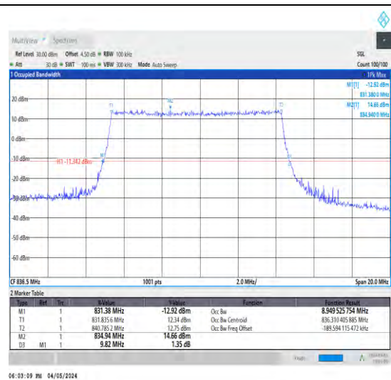
1-N5-15-10-M-3-DFT-16QAM-Outer_Full-50 @0-Ant1-8.95-9.820-≤10-PASS
