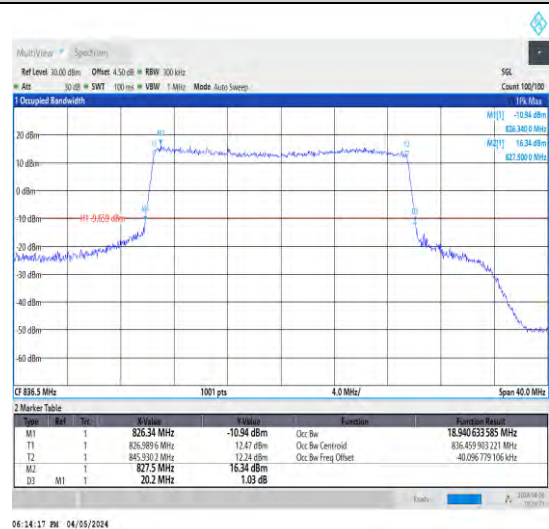
1-N5-15-20-M-7-CP-16QAM-Outet_Full-106 @0-Ant1-18.941-20.200-≤20-PASS
