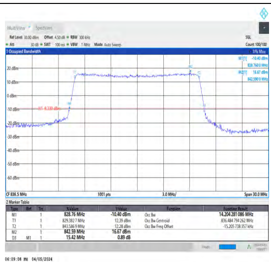
1-N5-15-15-M-6-CP-QPSK-Outer_Full-79@0 -Ant1-14.204-15.420≤15-PASS
