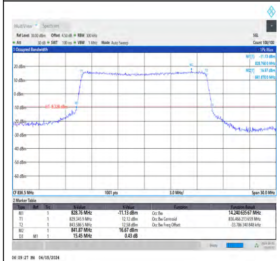
1-N5-15-15-M-7-CP-16QAM-Outer_Full-79@ 0-Ant1-14.241-15.450≤15-PASS
