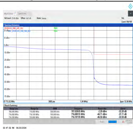
1-N12-15-10-H-6-CP-QPSK-Outer_Full-52@0-Ant1-1--PASS-see graph
