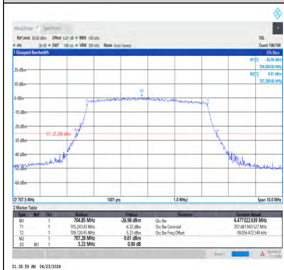
1-N12-15-5-M-9-CP-256QAM-Outer_Full-25 @0-Ant1-4.477-5.220-≤5-PASS
