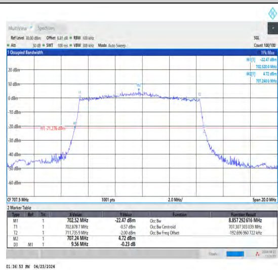
1-N12-15-10-M-1-DFT-QPSK-Outer_Full-50 @0-Ant1-8.857-9.560-≤10-PASS
