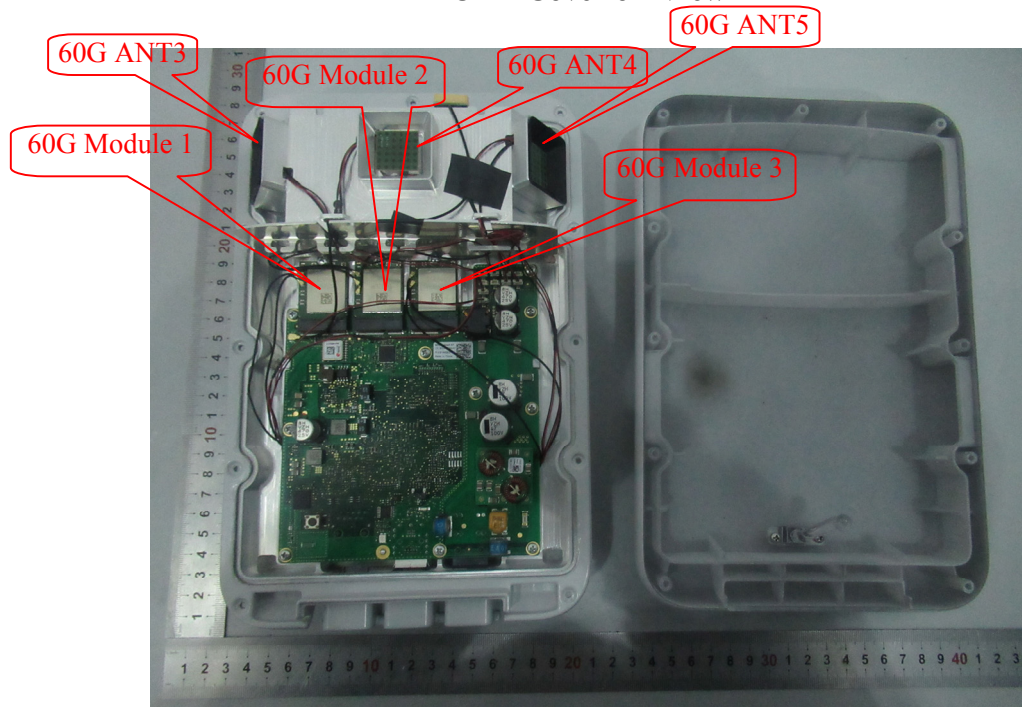
EUT – Cover off View-2
