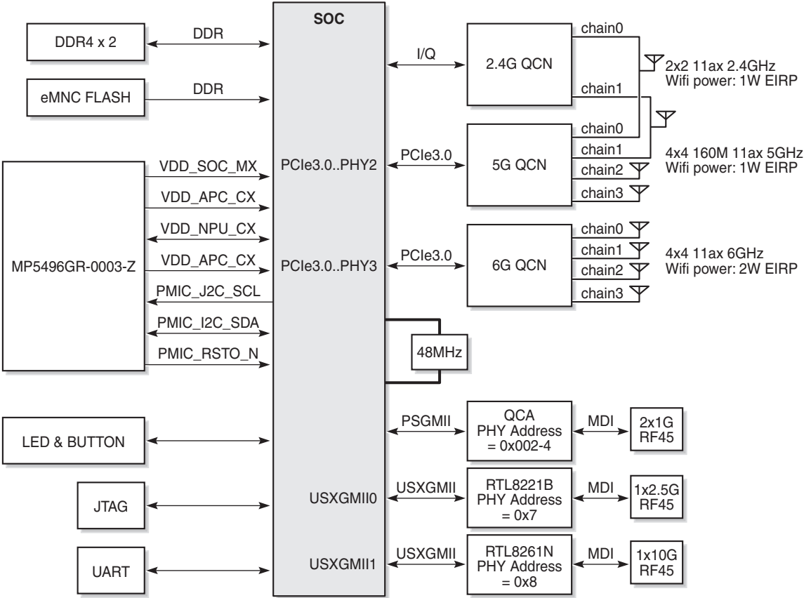
Figure 5-4 Single-residence WiFi CPE with Gigabit Ethernet
