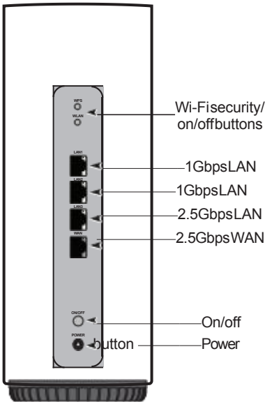
Figure 5-2 Beacon G6 connections and components
