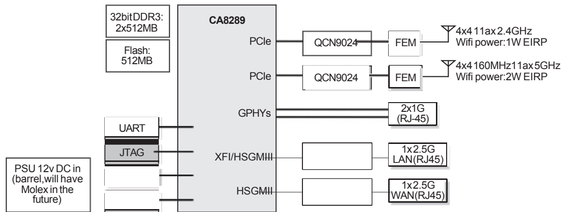
Figure 5-4 Beacon G6 functional block
