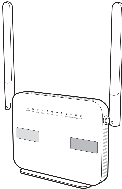
Figure 5-1 G-1425G-B ONT (external antenna)
