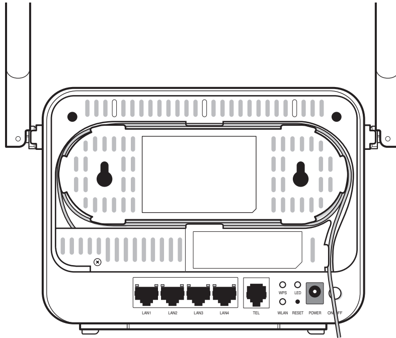
Figure 5-3 G-1425G-B indoor ONT with fiber optic connector
