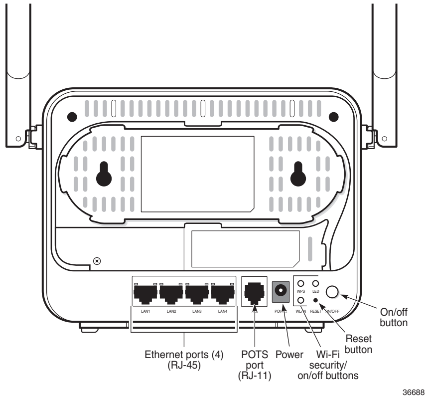
Figure 6-2 G-1425G-B indoor ONT connections
