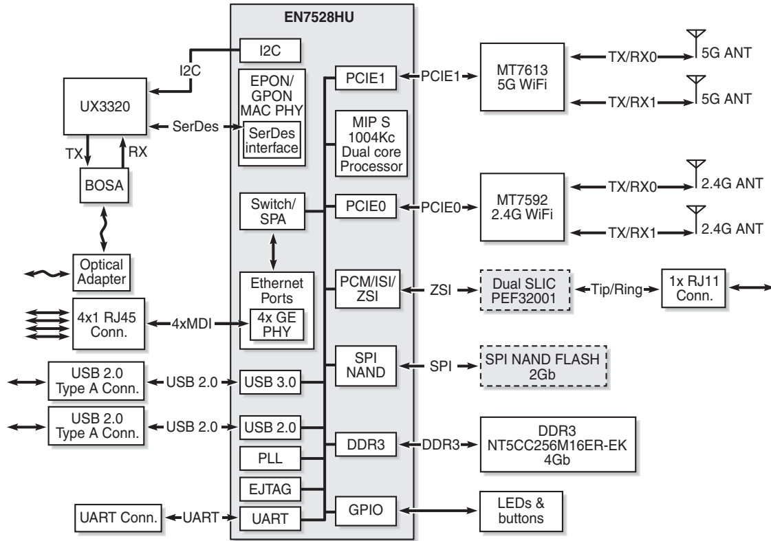
Figure 5-6 G-1425G-B ONT functional block
