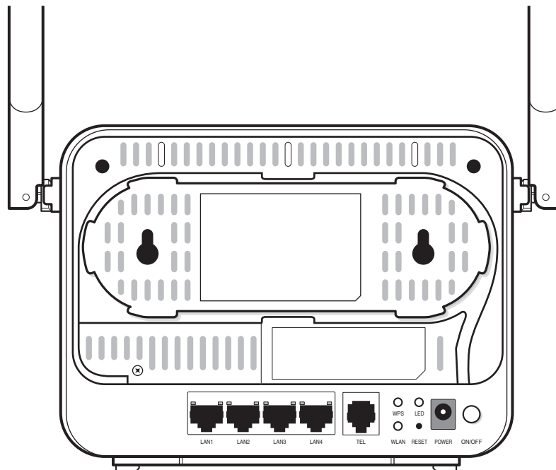
Figure 5-2 G-1425G-B indoor ONT physical connections (back)
