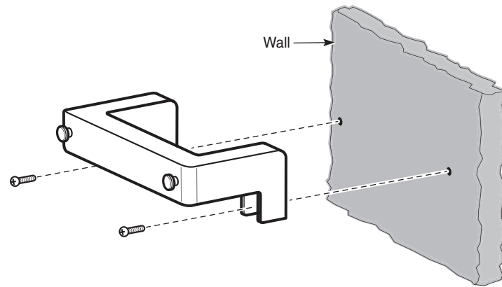
Figure 6-5 Wall mount bracket power cord placement
