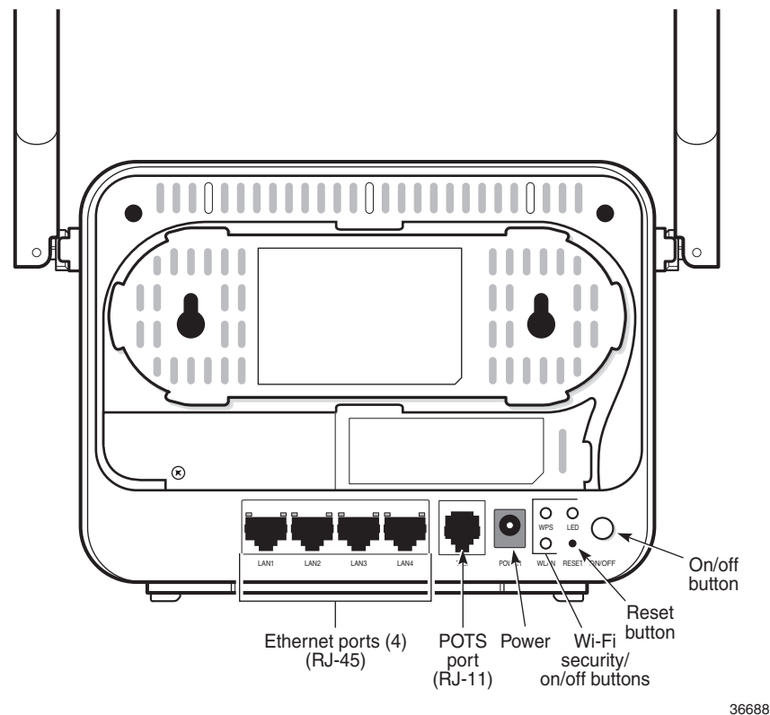
Figure 6-1 G-1425G-B ONT connections
