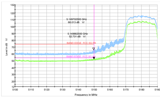
802.11n HT40-Channel 38: Peak + Average
