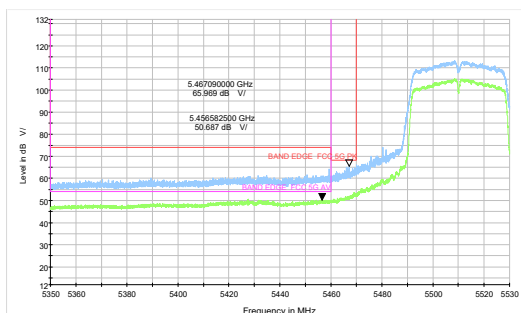
802.11n HT40-Channel 102: Peak + Average
