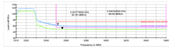
802.11n HT20-Channel 64: Peak + Average
