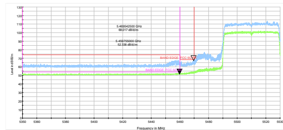
802.11ax HE40-Channel 102: Peak + Average
