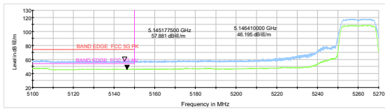
802.11n HT20-Channel 52: Peak + Average
