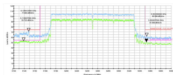
802.11ax HE160-Channel 50: Peak + Average
