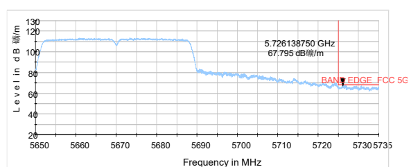
802.11n HT40-Channel 134: Peak
