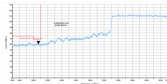
802.11ax HE160-Channel 114: Peak + Average
