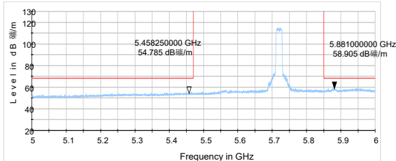
802.11a-Channel 144: Peak
