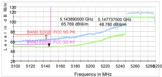
802.11ac VHT80 -Channel 58: Peak + Average
