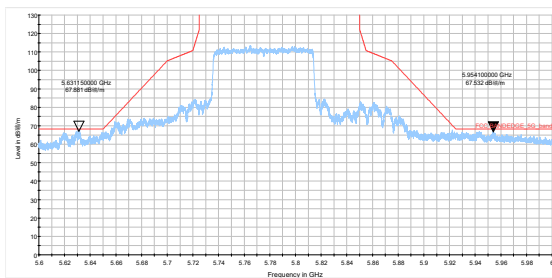
802.11ax HE80- Channel 155: Peak
