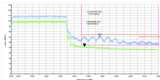
802.11ax HE80 -Channel 58: Peak + Average
