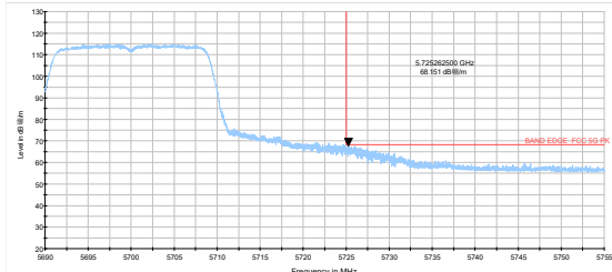
802.11n HT20-Channel 140: Peak
