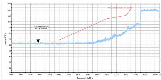
802.11ax HE40-Channel 151: Peak
