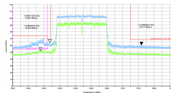
802.11ax HE160-Channel 114: Peak + Average
