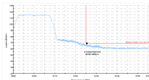
802.11a-Channel 140: Peak
