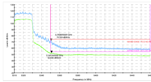
802.11ax HE20 -Channel 64: Peak + Average
