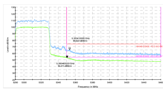
802.11ax HE40 -Channel 62: Peak + Average
