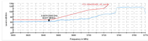
802.11ac VHT20-Channel 149: Peak
