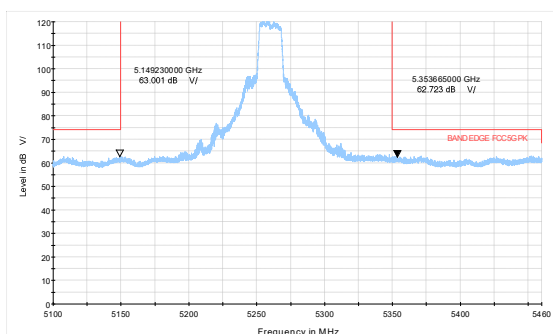
802.11a-Channel 52: Peak
