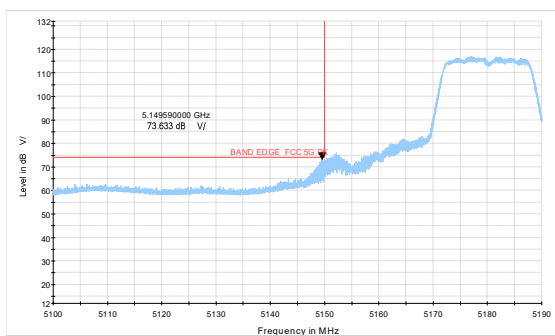
802.11a-Channel 36: Average
