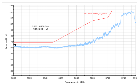
802.11a-Channel 149: Peak
