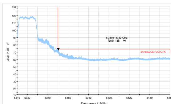
802.11a-Channel 64: Peak
