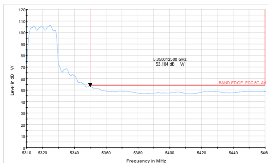
802.11a-Channel 64: Average
