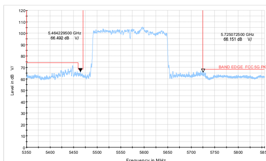
802.11ax HE160-Channel 114: Peak
