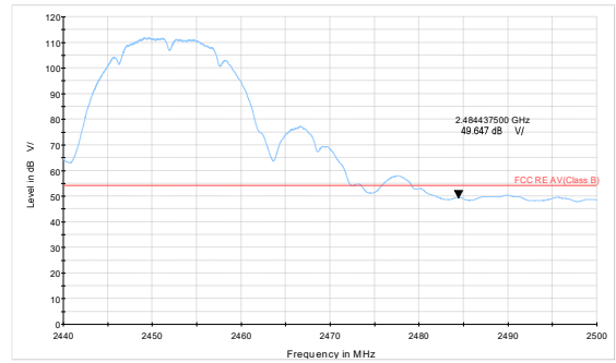
802.11b-Channel 9 Average
