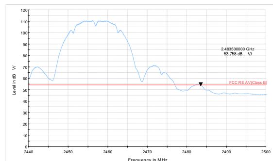
802.11b-Channel 10 Average
