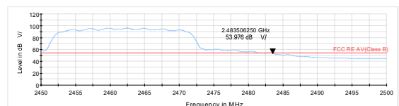
802.11ax HE20-Channel 11 Average
