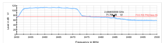
802.11ax HE20-Channel 11 Peak
