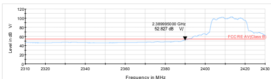
802.11g-Channel 1 Average
