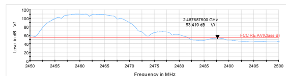
802.11b-Channel 11 Average
