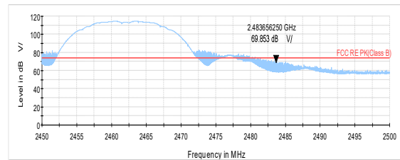
802.11b-Channel 11 Peak
