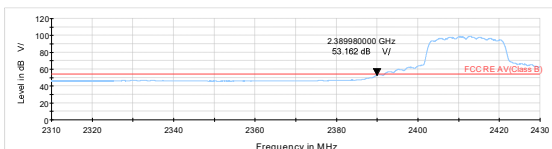
802.11n HT20-Channel 1 Average
