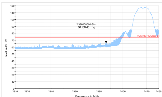
802.11b-Channel 2 Peak
