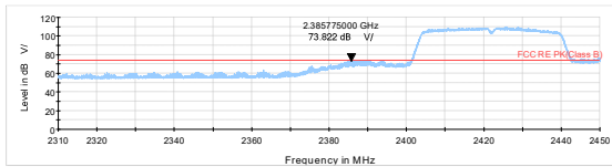
802.11n HT40-Channel 3 Peak
