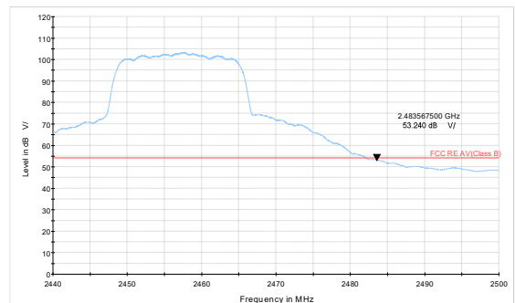
802.11g-Channel 10 Average
