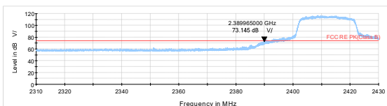
802.11ax HE20-Channel 1 Peak
