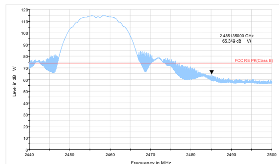
802.11b-Channel 10 Peak
