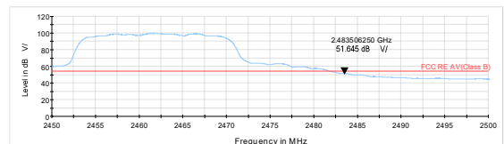
802.11g-Channel 11 Average
