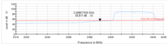
802.11n HT40-Channel 3 Average
