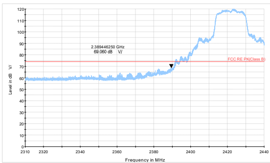
802.11g-Channel 3 Peak
