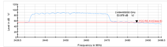
802.11n HT40-Channel 9 Average
