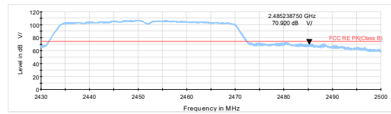
802.11n HT40-Channel 9 Peak
