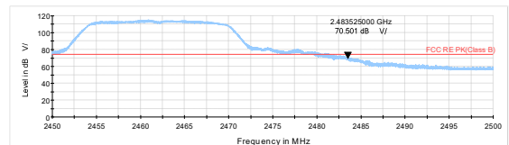
802.11g-Channel 11 Peak
