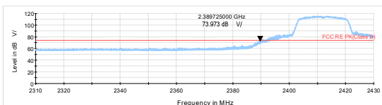
802.11n HT20-Channel 1 Peak
