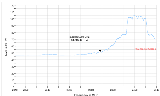
802.11g-Channel 3 Average
