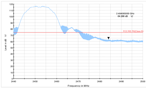
802.11b-Channel 9 Peak
