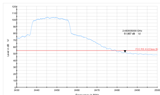
802.11n HT20-Channel 8 Average
