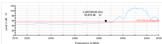
802.11b-Channel 1 Average
