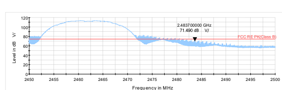
802.11n HT20-Channel 11 Peak
