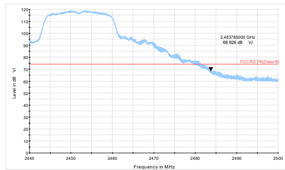
802.11g-Channel 9 Peak
