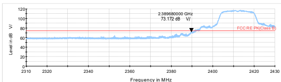
802.11g-Channel 1 Peak
