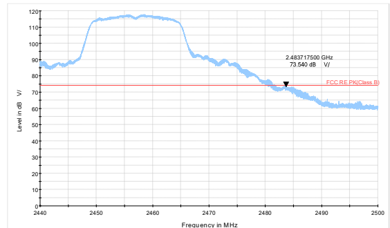
802.11g-Channel 10 Peak
