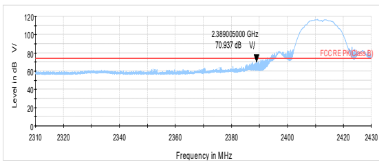
802.11b-Channel 1 Peak
