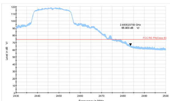
802.11n HT20-Channel 8 Peak
