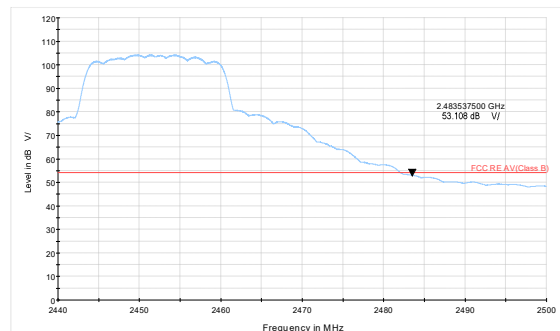
802.11g-Channel 9 Average
