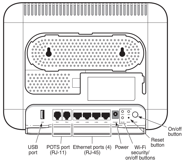
Figure 6-1 G-2426G-A indoor ONT connections
