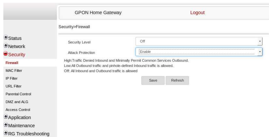
Figure 7-29 Firewall page
