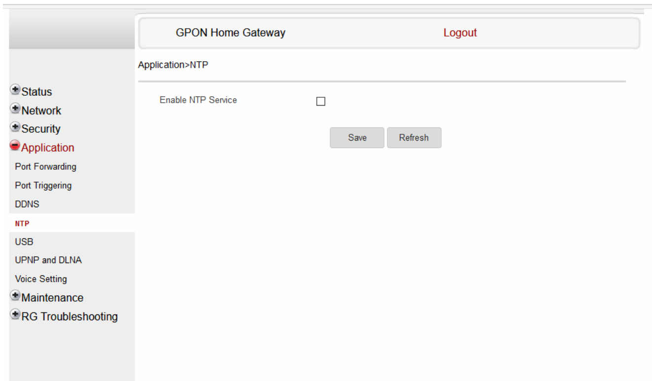
Figure 7-39 NTP page
