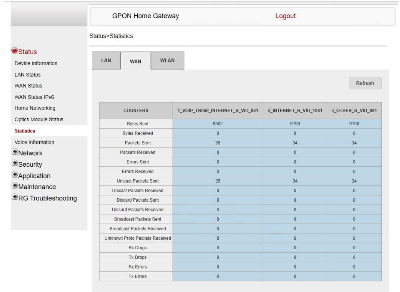
Figure 7-9 WAN Statistics page
