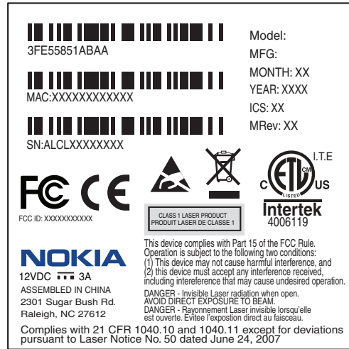
Figure 3-2 Sample laser product label showing CDRH 21 CFR compliance
