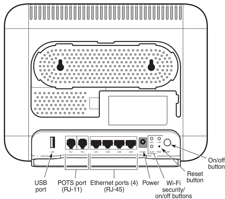
Figure 5-1 G-2426G-A ONT connections
