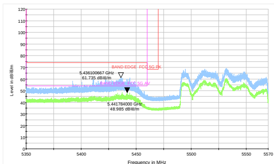
802.11ax HE160-Channel 114: Peak &amp; Average
