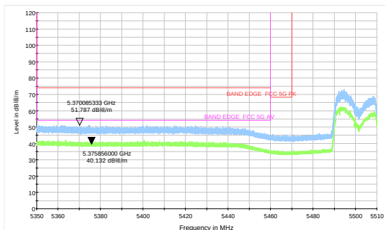
802.11ax HE40-Channel 102: Peak &amp; Average
