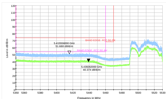
802.11ax HE80-Channel 106: Peak &amp; Average
