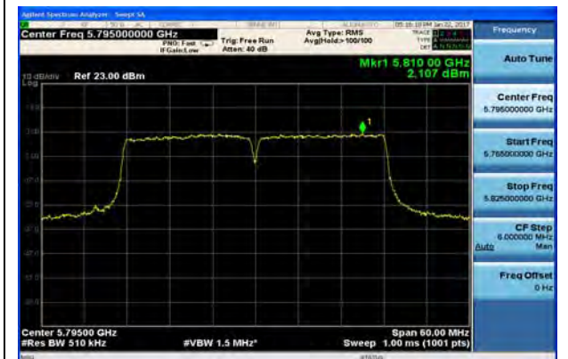
U-NII-3, 802.11n HT40, Channel No.: 159
