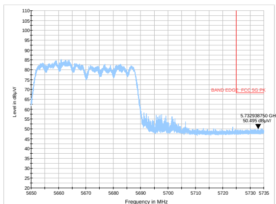
802.11ac HT40-Channel 134: Peak
