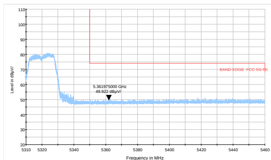
802.11a-Channel 64: Average
