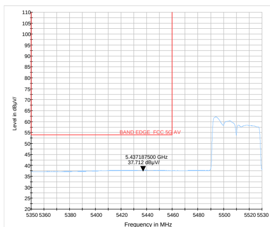
802.11ac HT40-Channel 102: Average
