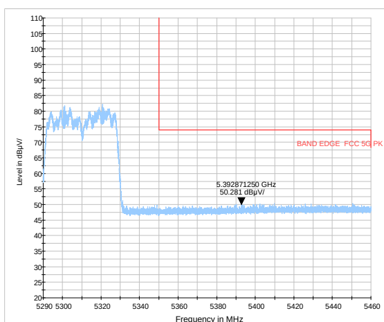
802.11n HT40-Channel 62: Average
