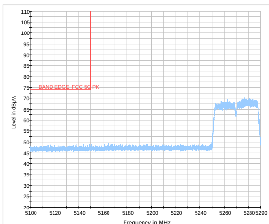
802.11ac HT40-Channel 54: Peak
