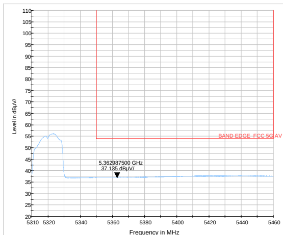
802.11ac HT40-Channel 62: Peak
