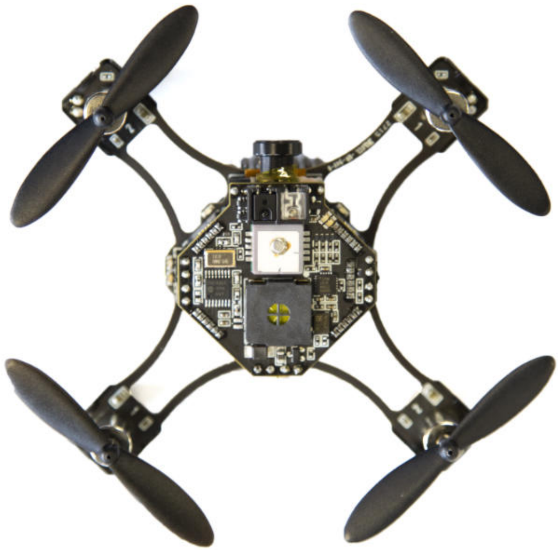
All Boards Assembled, Top view
