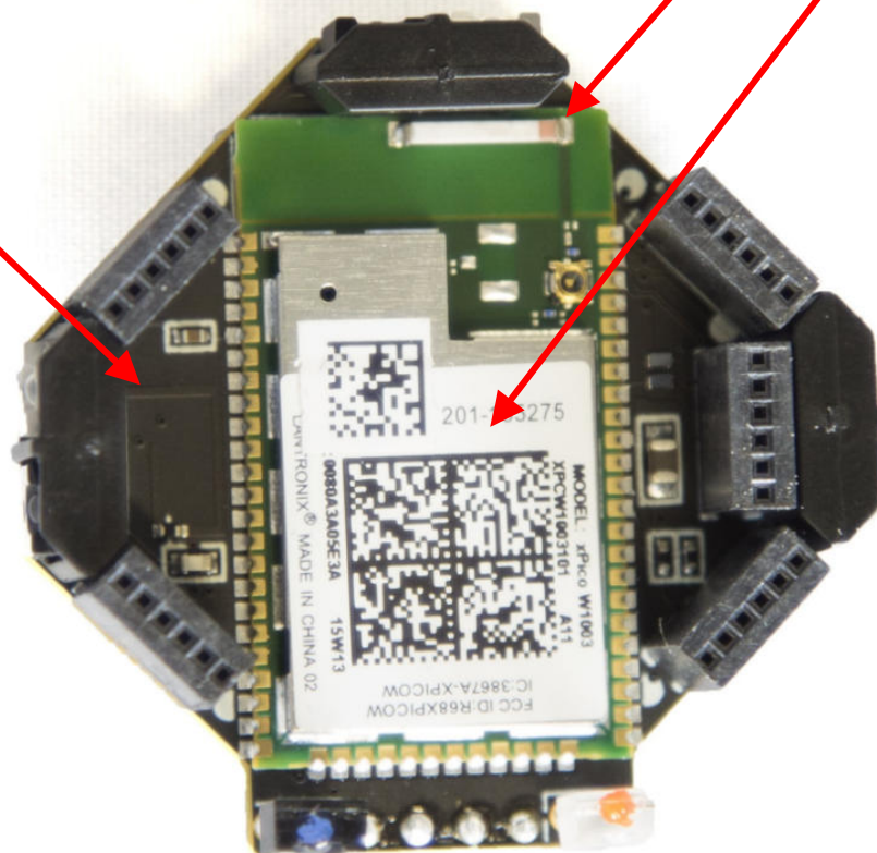
RF (Top) Board, Bottom view
