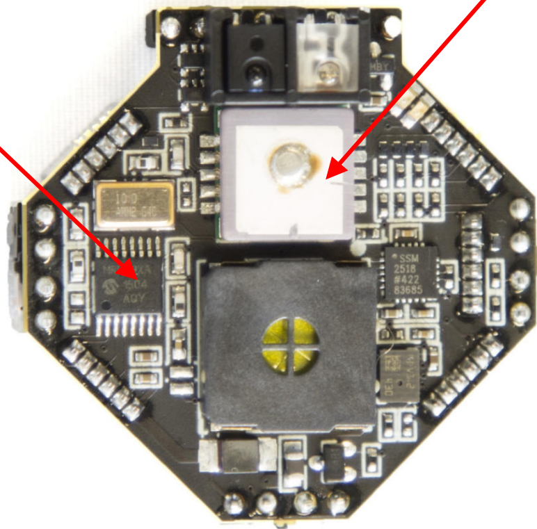
RF (Top) Board, Top view
