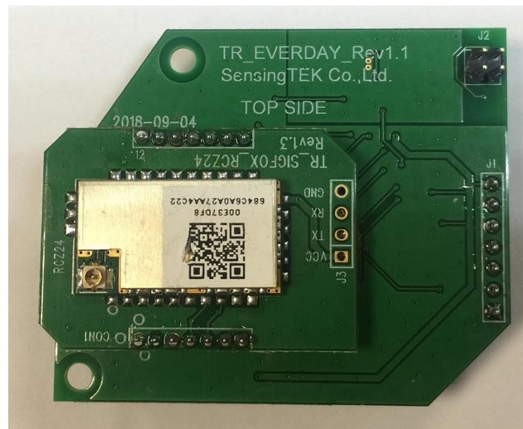
Fig.5 Module_Sigfox_RCZ2 hardware installation diagram
