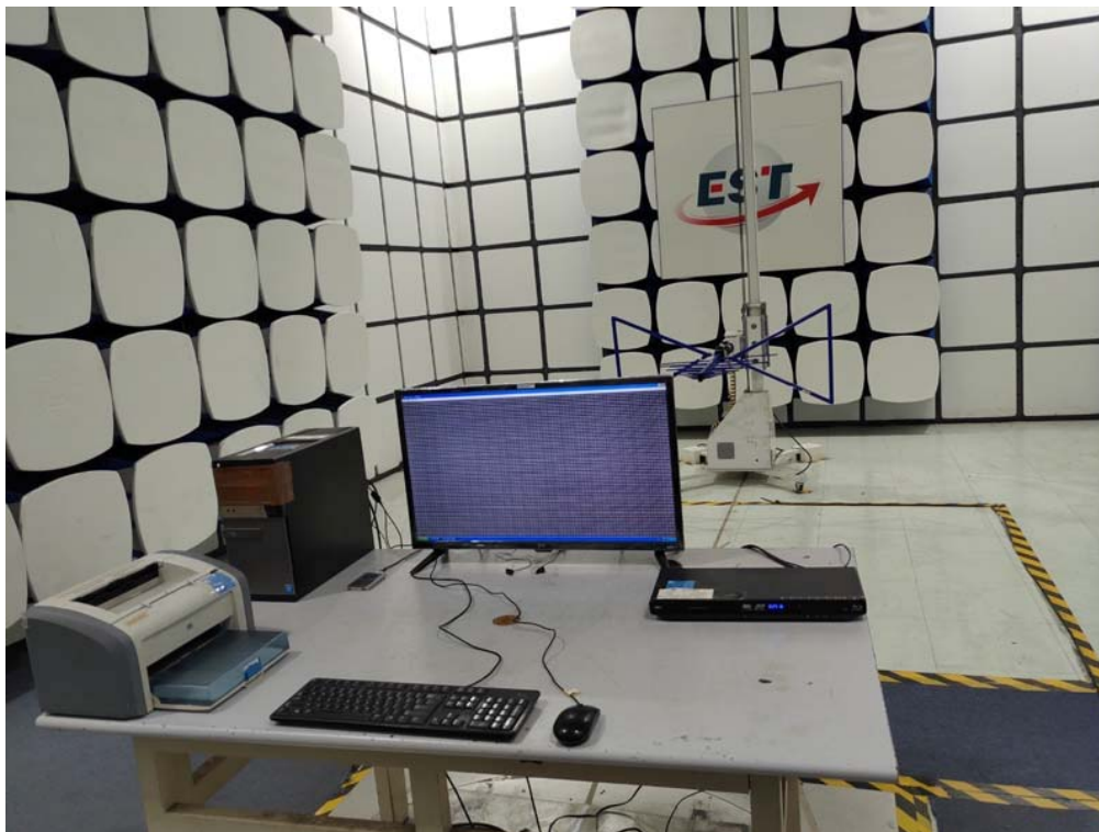
Set-up for radiated emission test (30-1000MHz)
