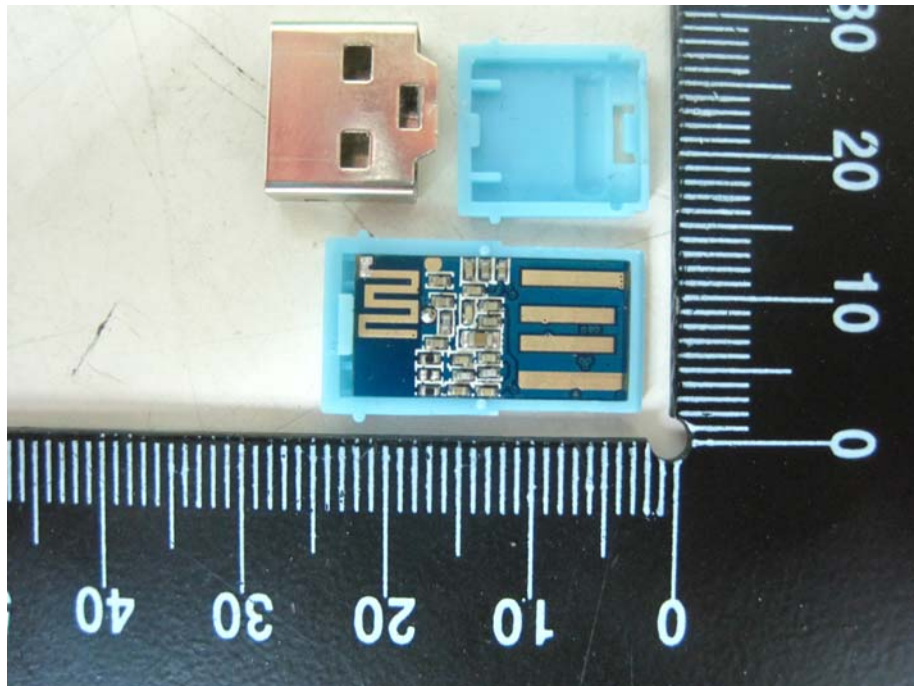
Inside View of the Dongle
