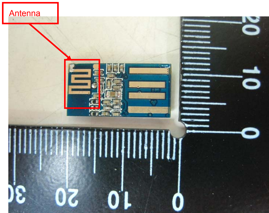
Rear View of the Dongle's PCB
