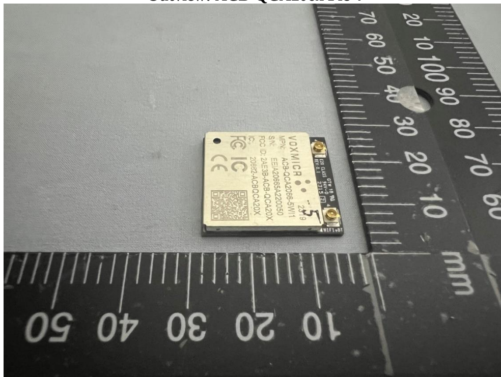
Outview: ACB-QCA206x Pic 4
