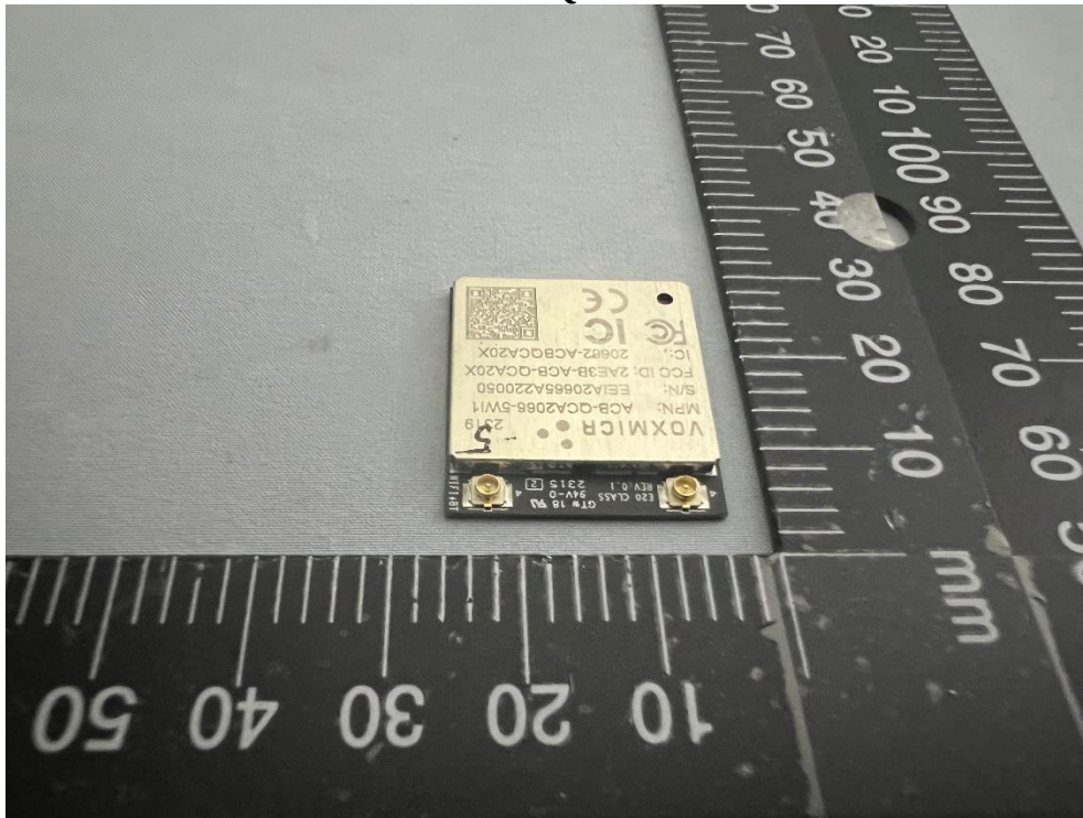
Outview: ACB-QCA206x Pic 5
