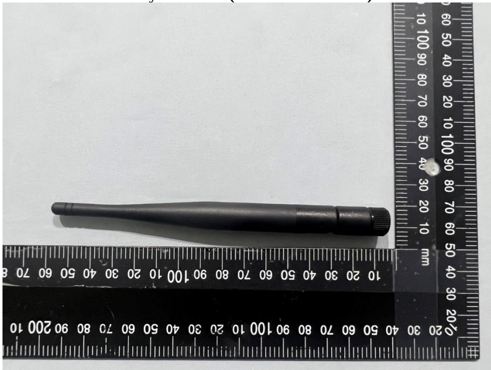
Accessory: Antenna (WANT-4DBI-SMA) Pic 4
