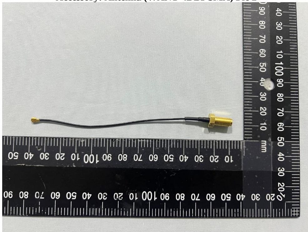
Accessory: Antenna (WANT-4DBI-SMA) Pic 2
