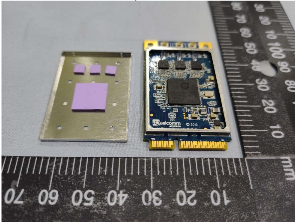
Internal Photos AEX-QCA98x0 Pic 1
