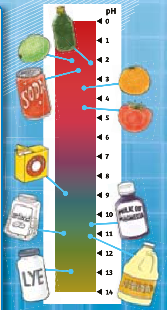
pH scale with the pH of some common items.
