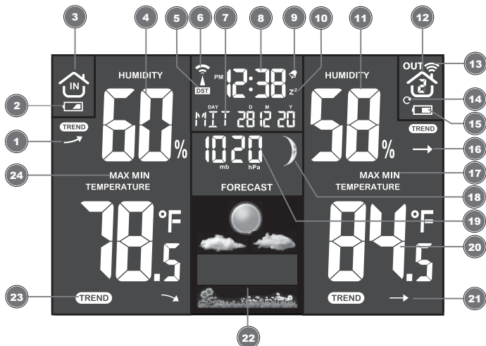
Illustration 2: Screen display for the base station
