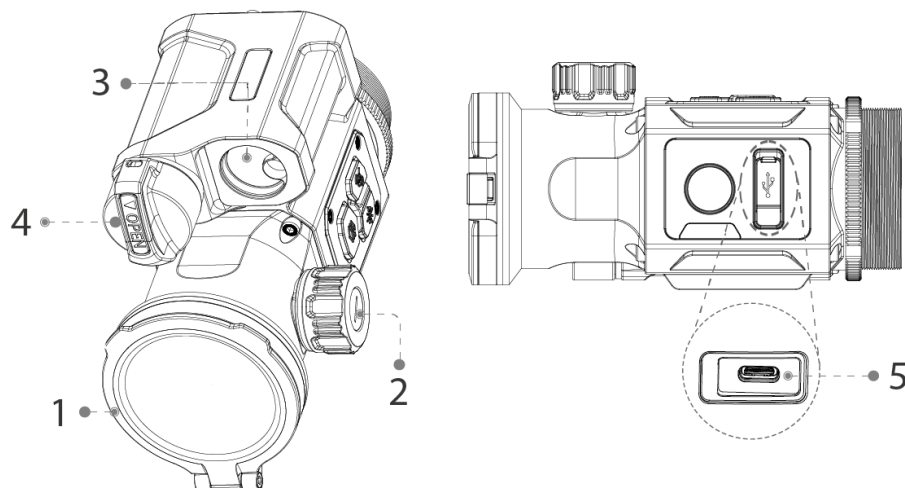
Figure 2-4 Component description (with LRF)
