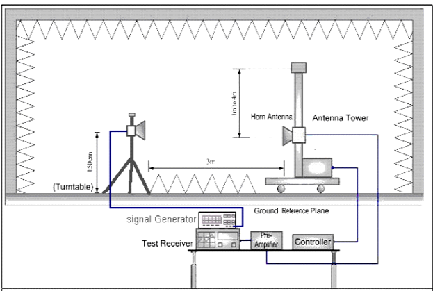
EIRP Test Setup
