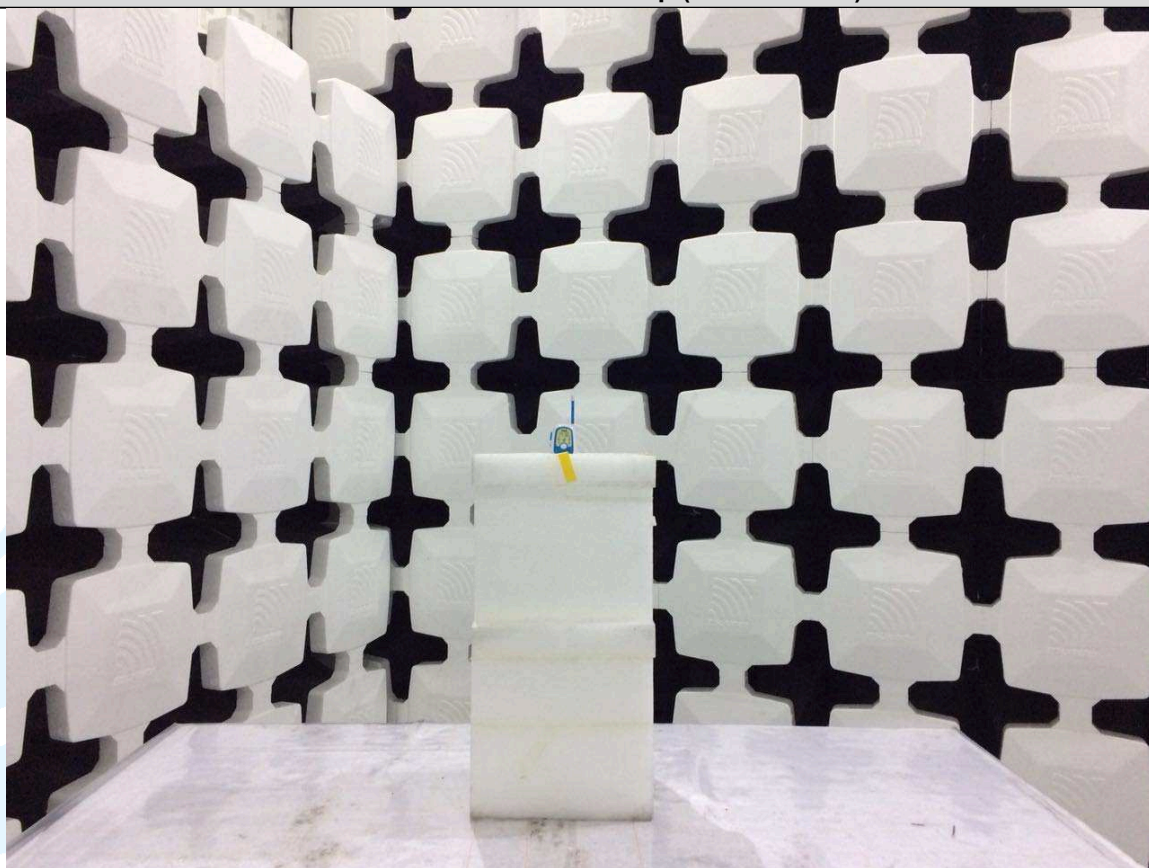
Radiated emission Test Setup (Above 1 GHz)
