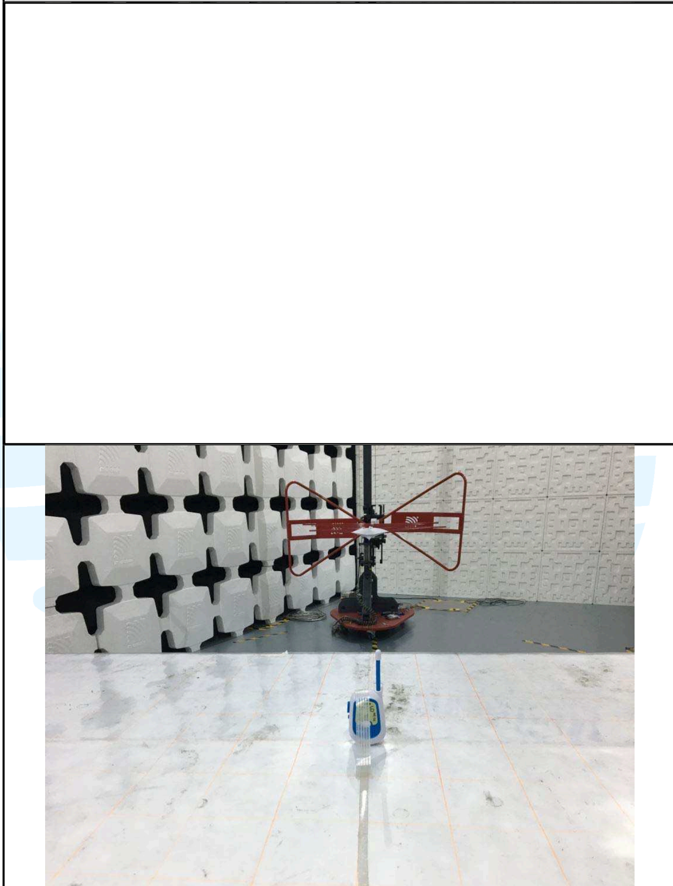
Radiated emission Test Setup (30 MHz~1 GHz)
