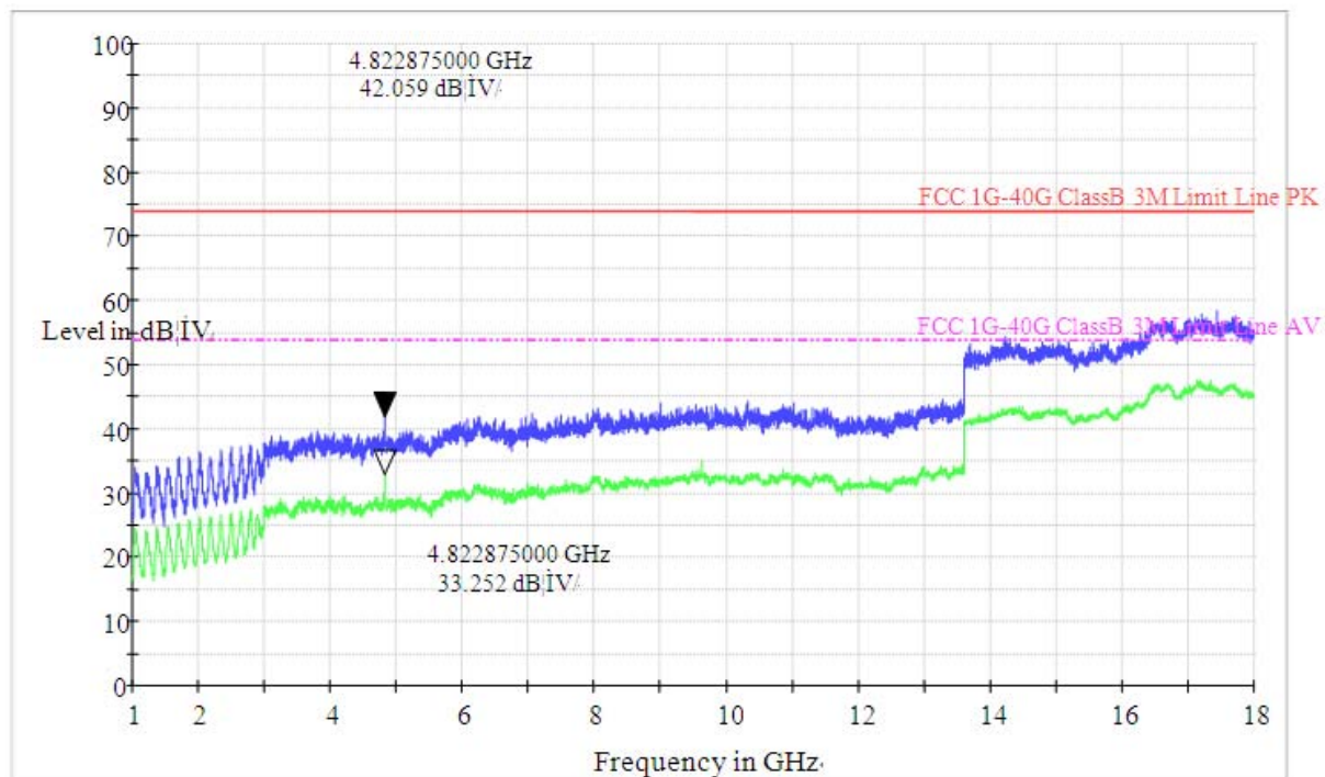
(Plot E: Test Antenna Horizontal 1G – 18G)
