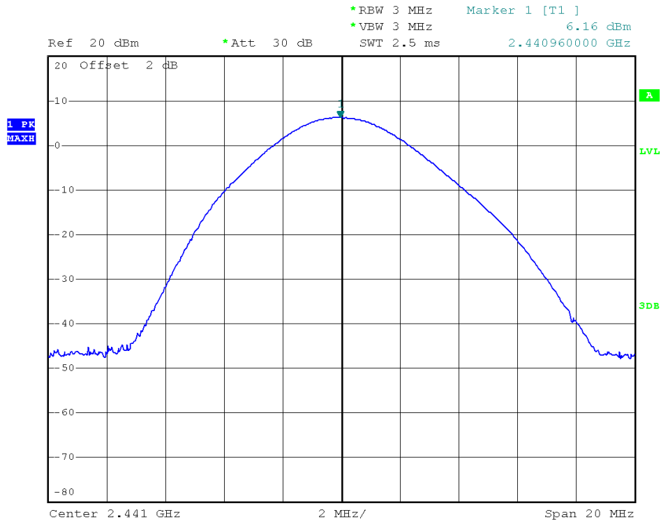
Plot C2:8-DPSK
