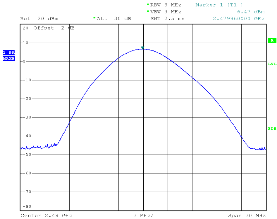
Plot C3:8-DPSK
