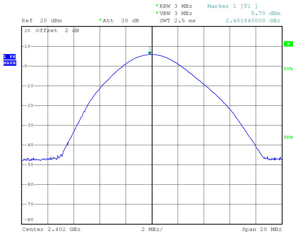
Plot C1:8-DPSK
