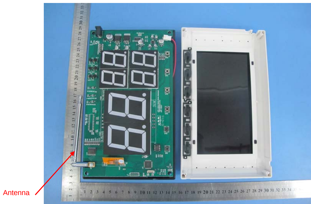
Photo 6 Internal of EUT
