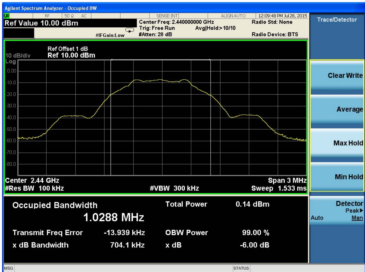
(Plot 4.5.1 B: Channel 19: 2440MHz @ GFSK)
