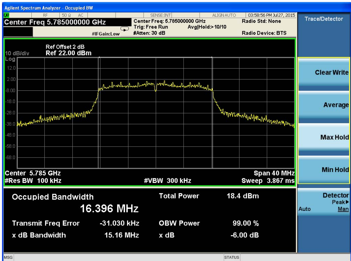
(Plot 4.6.1 B: Channel 157: 5785MHz @ 802.11a)
