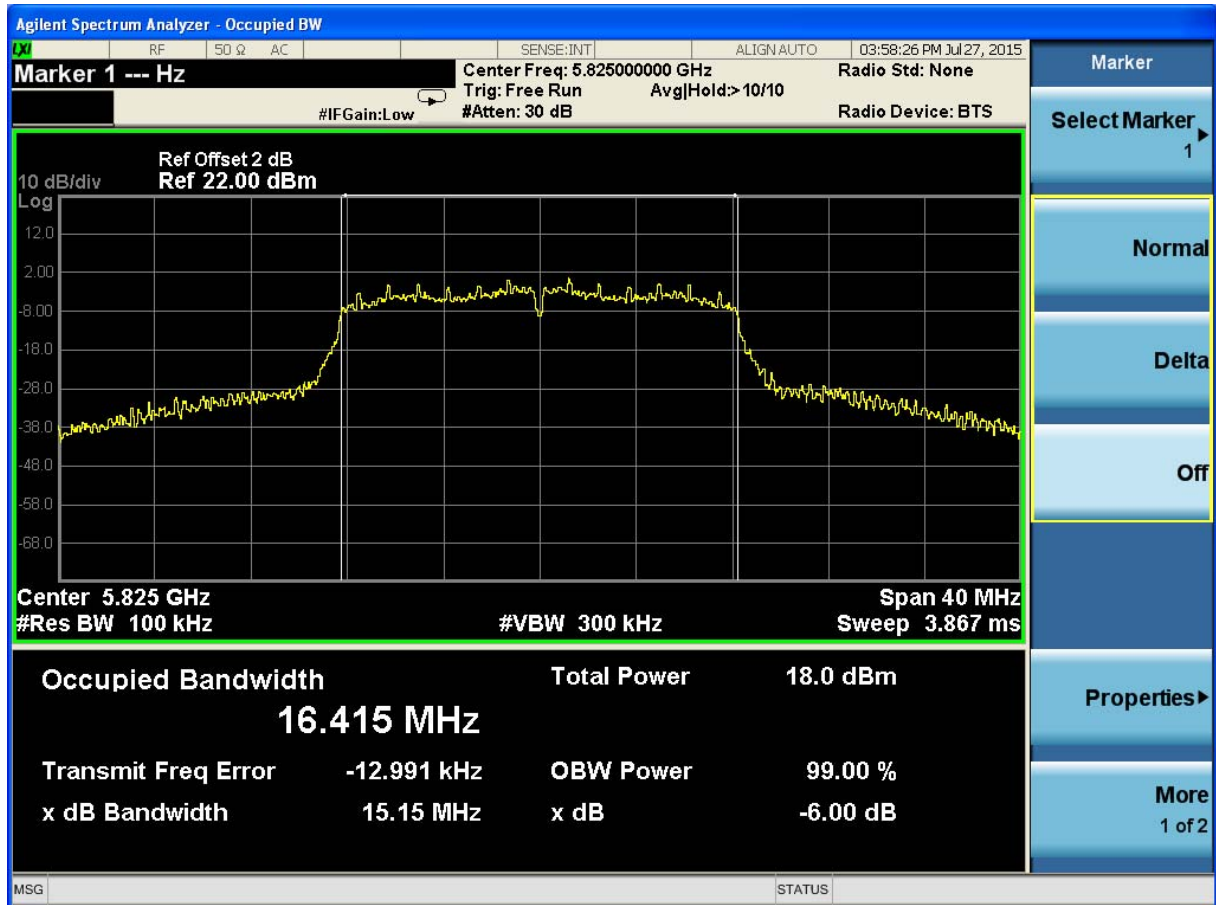
(Plot 4.6.1 C: Channel 165: 5825MHz @ 802.11a)
