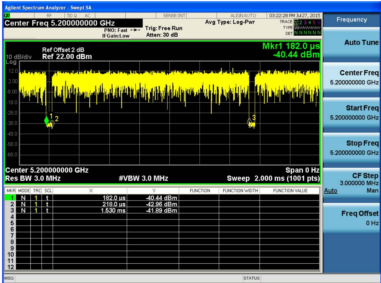
(Plot 4.3.2 B: Channel 40: 5200MHz @ 802.11n HT20)
