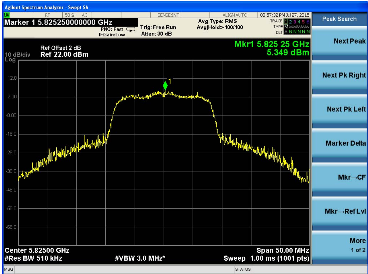
(Plot 4.5.3 C: Channel 165: 5825MHz @ 802.11a)
