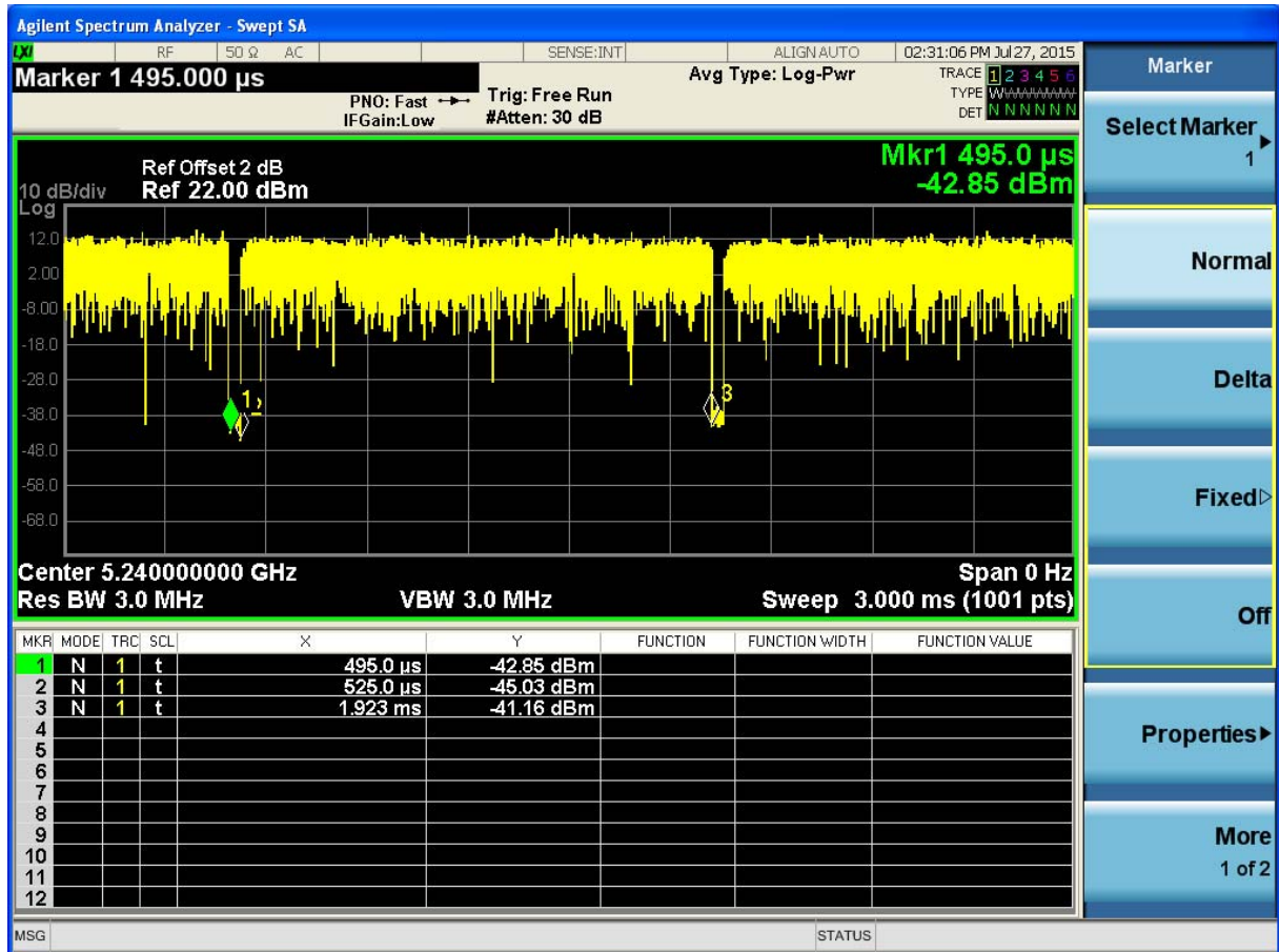
(Plot 4.3.1 C: Channel 48: 5240MHz @ 802.11a)
