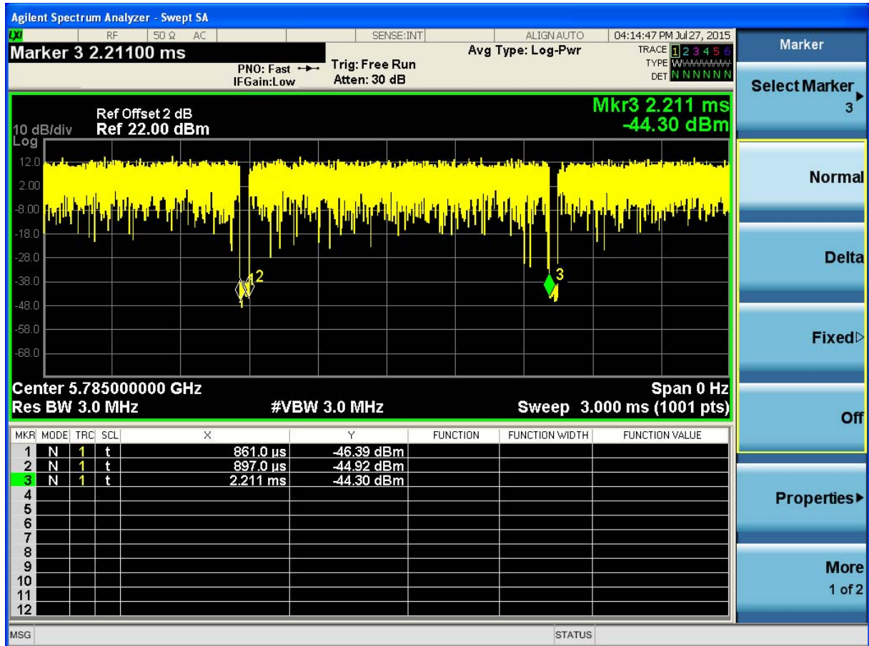
(Plot 4.3.4 B: Channel 157: 5785MHz @ 802.11n HT20)
