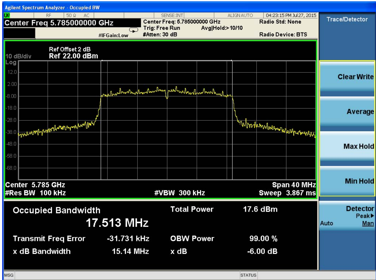
(Plot 4.6.2 B: Channel 157: 5785MHz @ 802.11n HT20)
