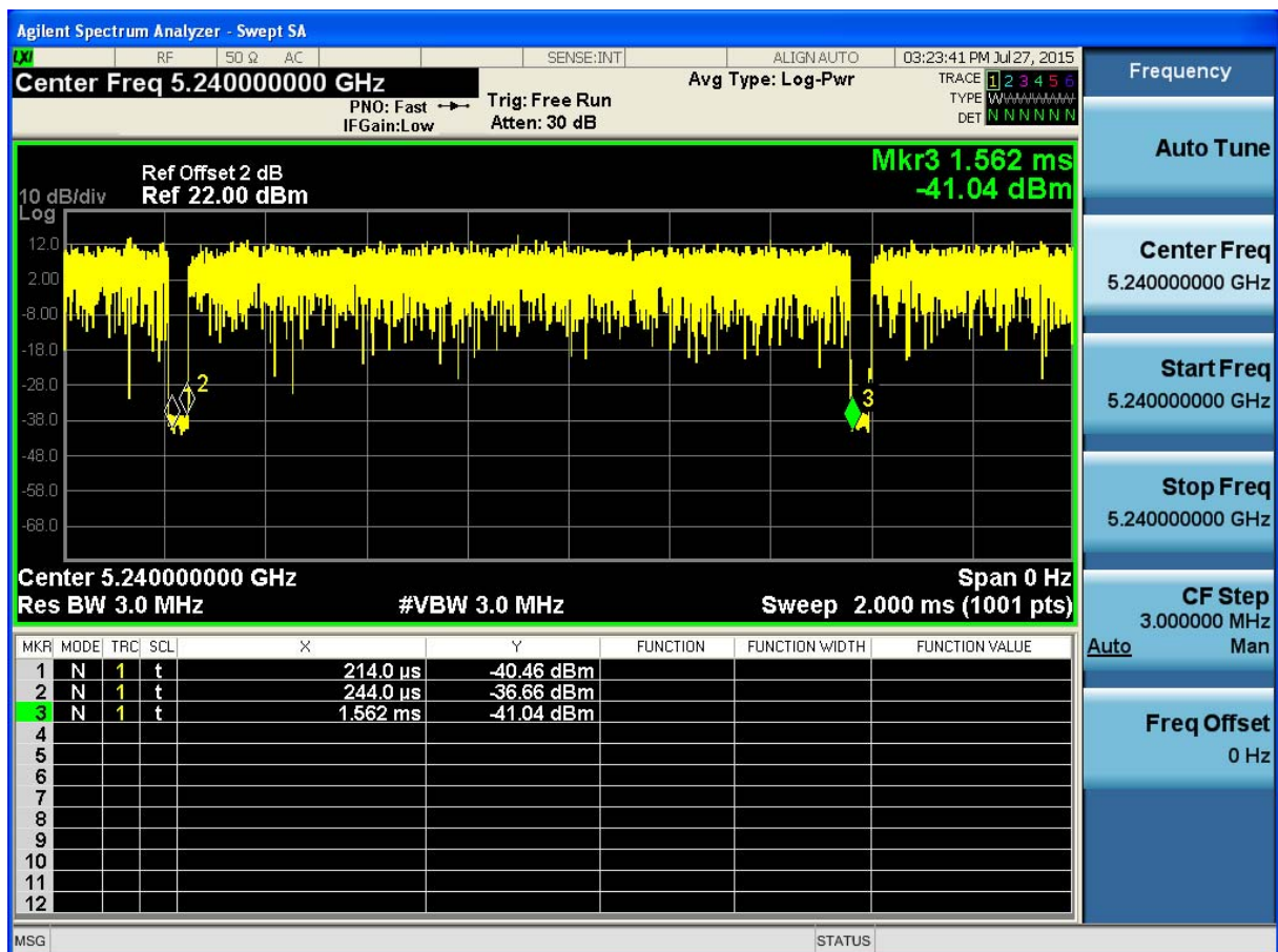
(Plot 4.3.2 C: Channel 48: 5240MHz @ 802.11n HT20)
