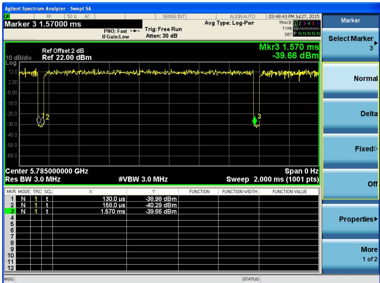
(Plot 4.3.3 B: Channel 157: 5785MHz @ 802.11a)
