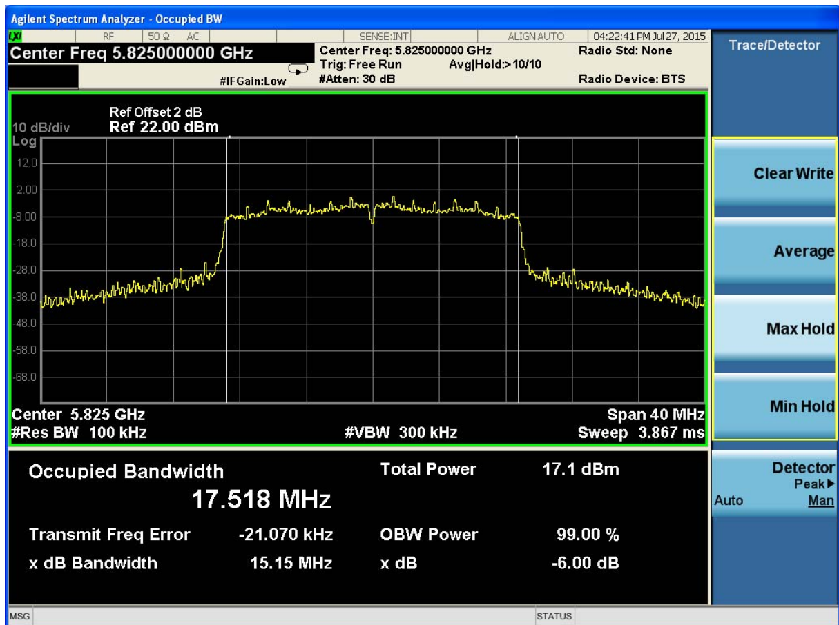
(Plot 4.6.2 C: Channel 135: 5825MHz @ 802.11n HT20)
