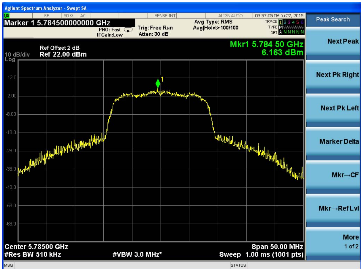
(Plot 4.5.3 B: Channel 157: 5785MHz @ 802.11a)
