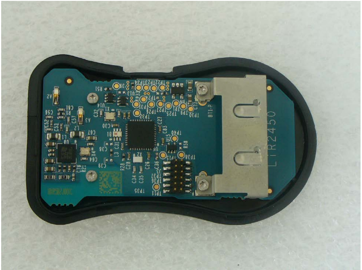
Figure 4: Internal View 4
