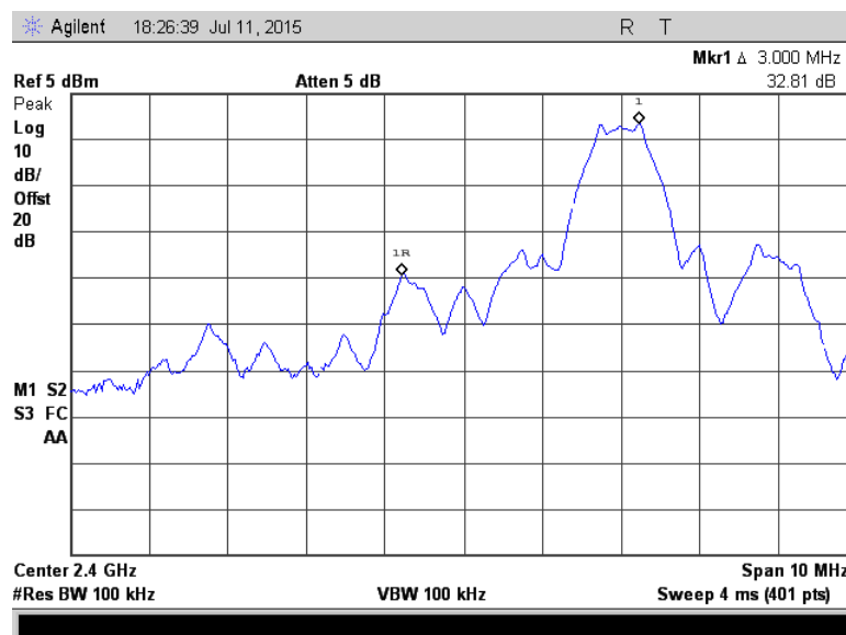
Figure 7.4.1.2-1: Lower Band-edge
