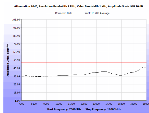
Plot 43. Radiated Spurious Emissions, High Channel, 7 GHz – 18 GHz, Average, 802.11g
