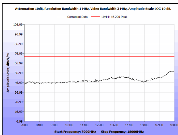
Plot 48. Radiated Spurious Emissions, Low Channel, 7 GHz – 18 GHz, Peak, 802.11n
