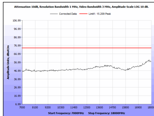
Plot 44. Radiated Spurious Emissions, High Channel, 7 GHz – 18 GHz, Peak, 802.11g
