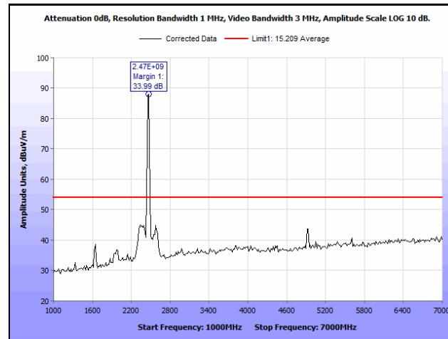
Plot 42. Radiated Spurious Emissions, High Channel, 1 GHz – 7 GHz, Peak Measurement with Average Limit, 802.11g
