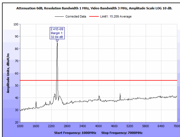
Plot 34. Radiated Spurious Emissions, Low Channel, 1 GHz – 7 GHz, Peak Measurement with Average Limit, 802.11g
