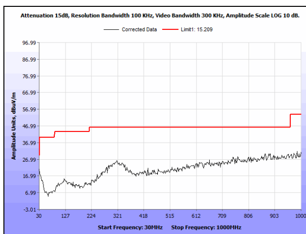
Plot 49. Radiated Spurious Emissions, Mid Channel, 30 MHz – 1 GHz, 802.11n
