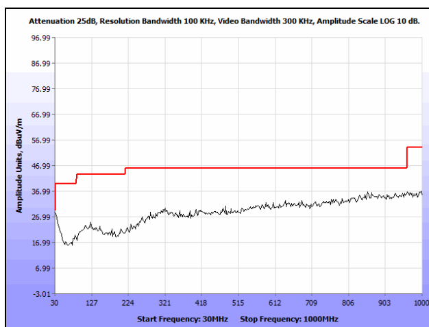
Plot 41. Radiated Spurious Emissions, High Channel, 30 MHz – 1 GHz, 802.11g
