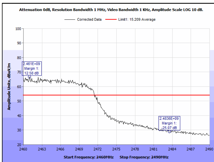
Plot 67. Radiated Restricted Band Edge, High Channel, Average, 802.11n
