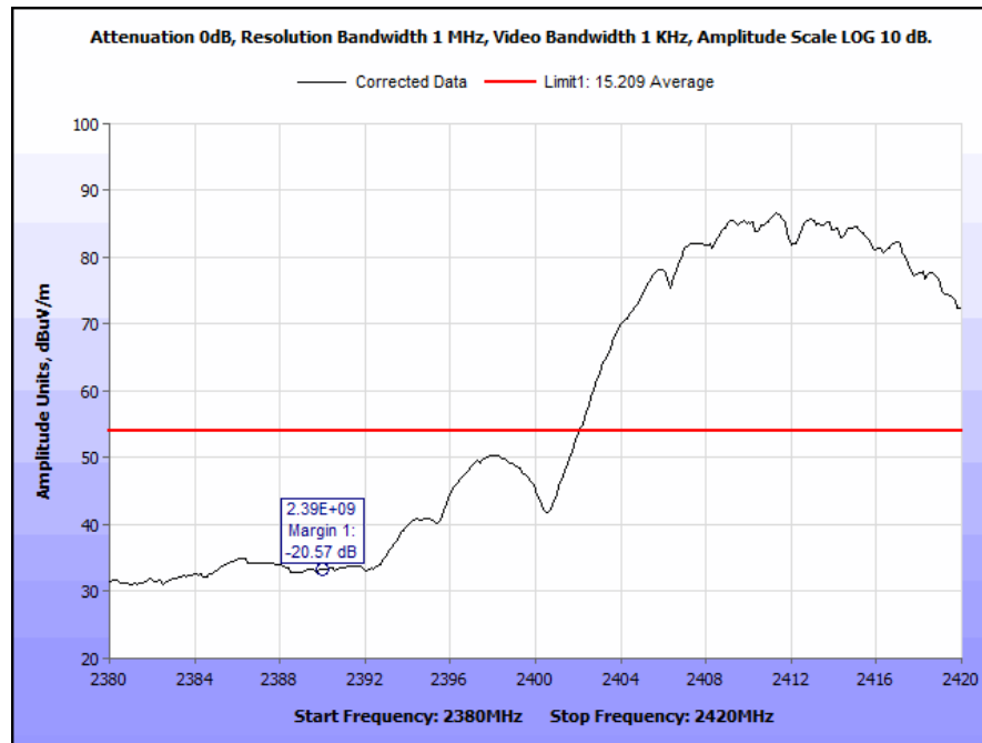
Plot 57. Radiated Restricted Band Edge, Low Channel, Average, 802.11b
