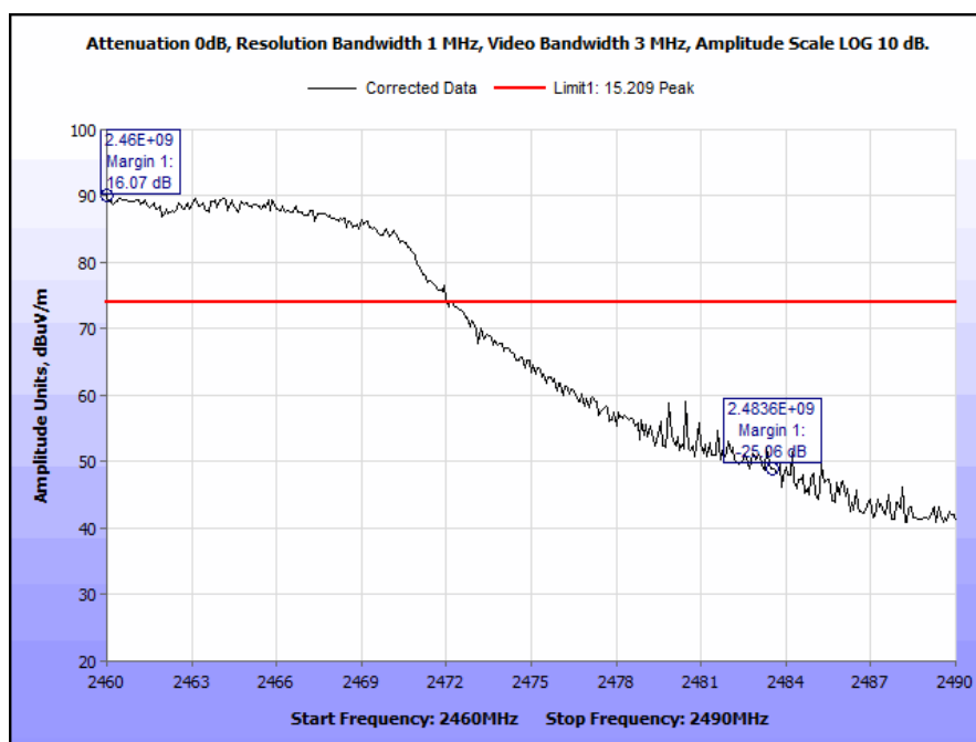
Plot 68. Radiated Restricted Band Edge, High Channel, Peak, 802.11n
