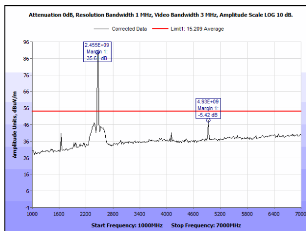
Plot 30. Radiated Spurious Emissions, High Channel, 1 GHz – 7 GHz, Peak Measurement with Average Limit, 802.11b
