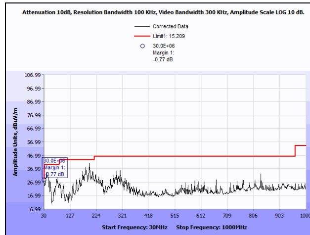
Plot 21. Radiated Spurious Emissions, Low Channel, 30 MHz – 1 GHz, 802.11b
