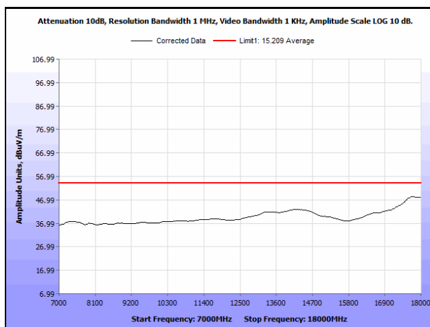
Plot 39. Radiated Spurious Emissions, Mid Channel, 7 GHz – 18 GHz, Average, 802.11g
