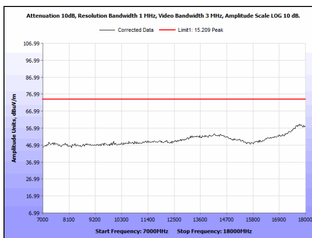
Plot 40. Radiated Spurious Emissions, Mid Channel, 7 GHz – 18 GHz, Peak, 802.11g
