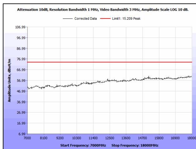
Plot 32. Radiated Spurious Emissions, High Channel, 7 GHz – 18 GHz, Peak, 802.11b
