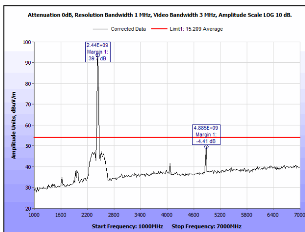
Plot 50. Radiated Spurious Emissions, Mid Channel, 1 GHz – 7 GHz, Peak Measurement with Average Limit, 802.11n
