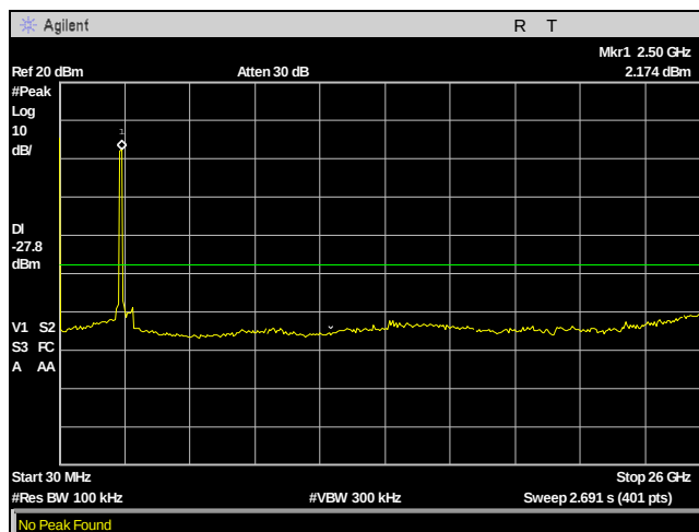
Plot 61. Conducted Spurious Emissions, BW 20 MHz, Ch. 2462 MHz, b mode
