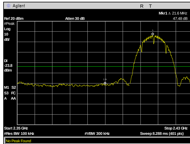
Plot 64. Conducted Band Edge, BW 20 MHz, Ch. 2412 MHz, b mode
