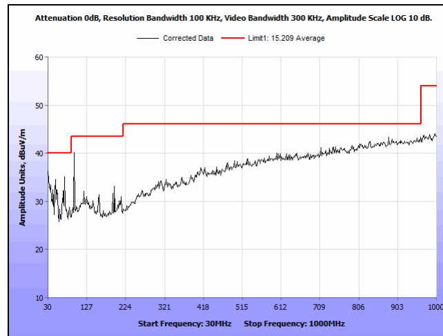
Plot 24. Radiated Spurious Emissions, 30 MHz – 1 GHz, Channel 6, b mode
