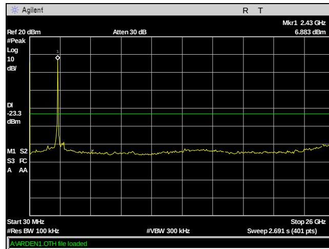
Plot 55. Conducted Spurious Emissions, BW 20 MHz, Ch. 2412 MHz, b mode
