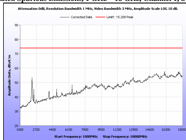
Plot 26. Radiated Spurious Emissions, 1 GHz – 18 GHz, Channel 1, b mode, Peak
