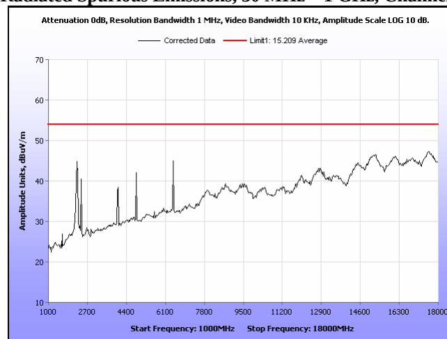
Plot 25. Radiated Spurious Emissions, 1 GHz – 18 GHz, Channel 1, b mode, Average
