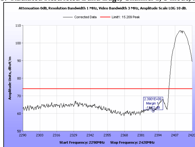
Plot 44. Radiated Restricted Band Edge, Channel 1, b mode, Peak
