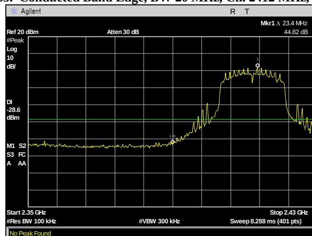
Plot 66. Conducted Band Edge, BW 20 MHz, Ch. 2412 MHz, n mode
