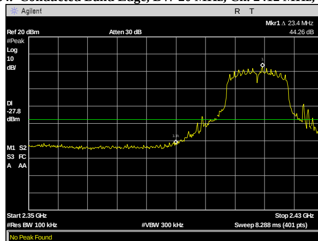
Plot 65. Conducted Band Edge, BW 20 MHz, Ch. 2412 MHz, g mode
