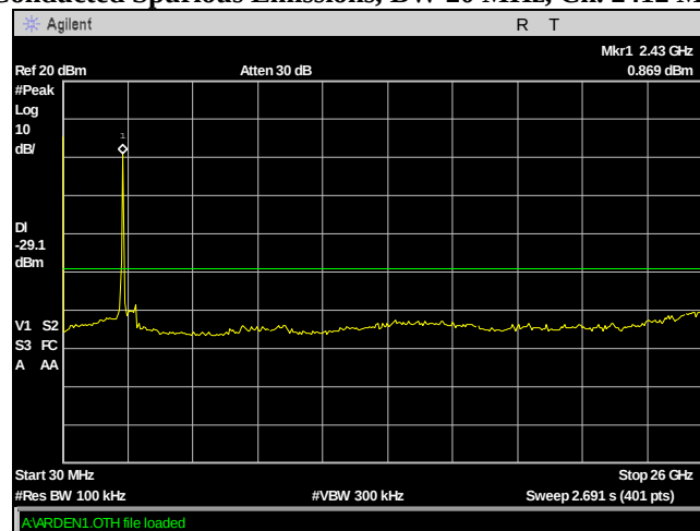
Plot 56. Conducted Spurious Emissions, BW 20 MHz, Ch. 2412 MHz, g mode
