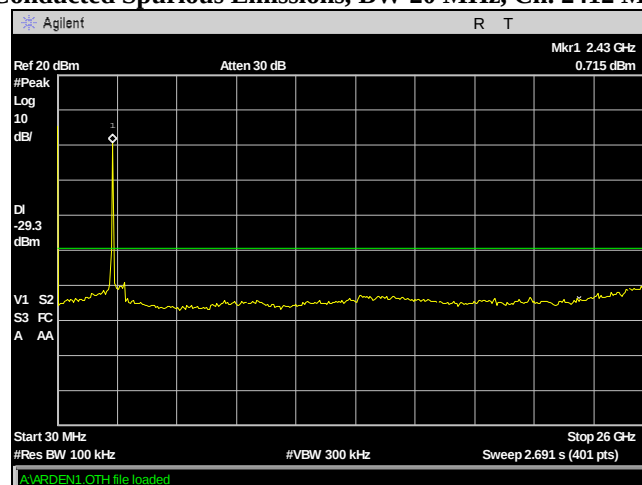
Plot 57. Conducted Spurious Emissions, BW 20 MHz, Ch. 2412 MHz, n mode
