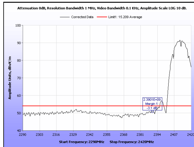
Plot 43. Radiated Restricted Band Edge, Channel 1, b mode, Average
