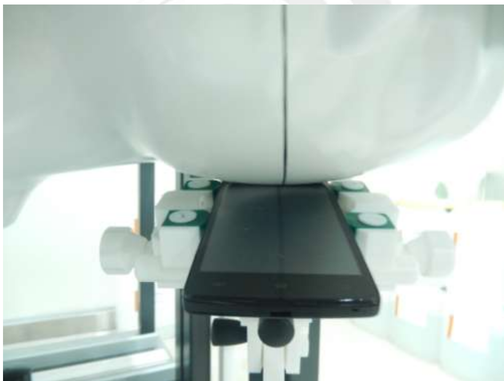
LEFT TILT 150
