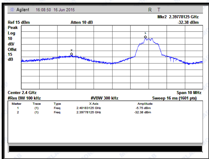
(Channel = 0, Band edge @ \pi/4 -DQPSK)
