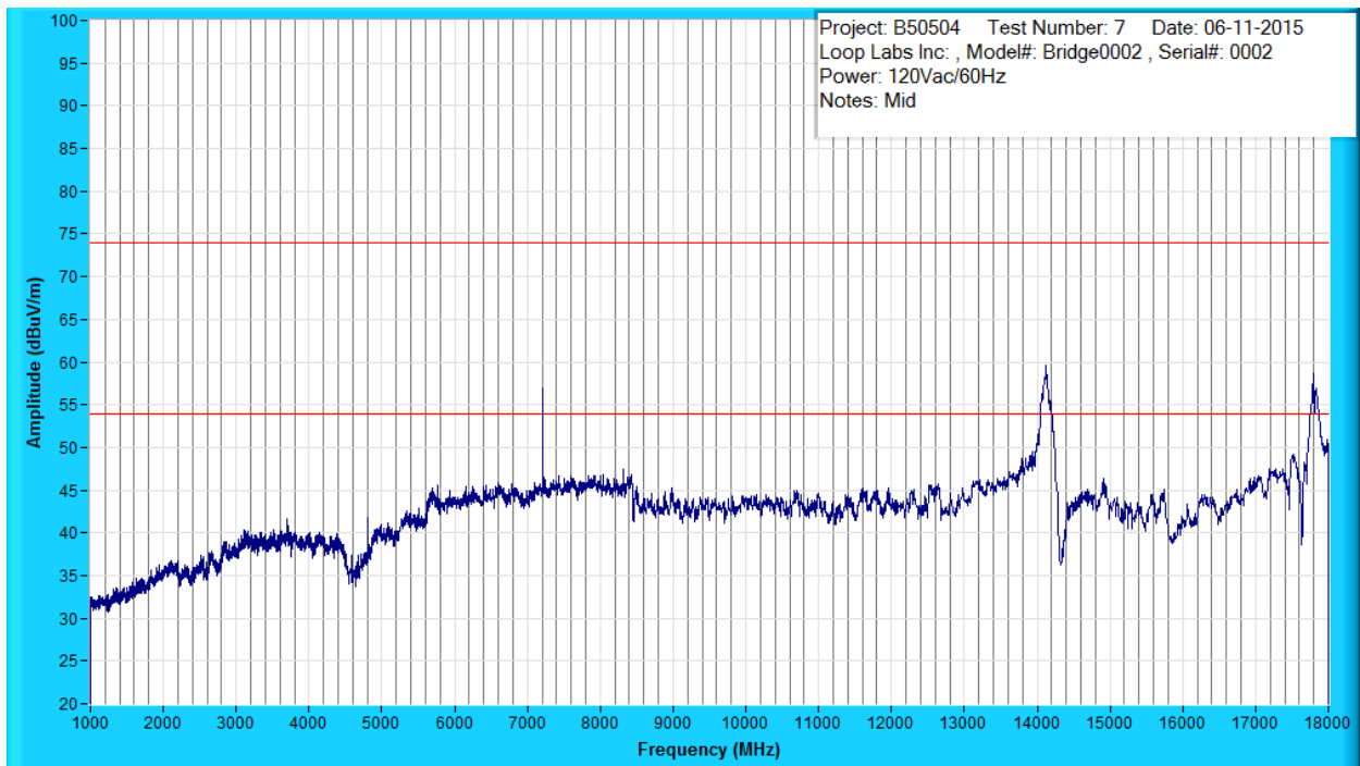
Figure A11: Radiated Emissions Prescan, 1GMHz to 18GMHz, Peak Measurements at 3m Distance, MID
