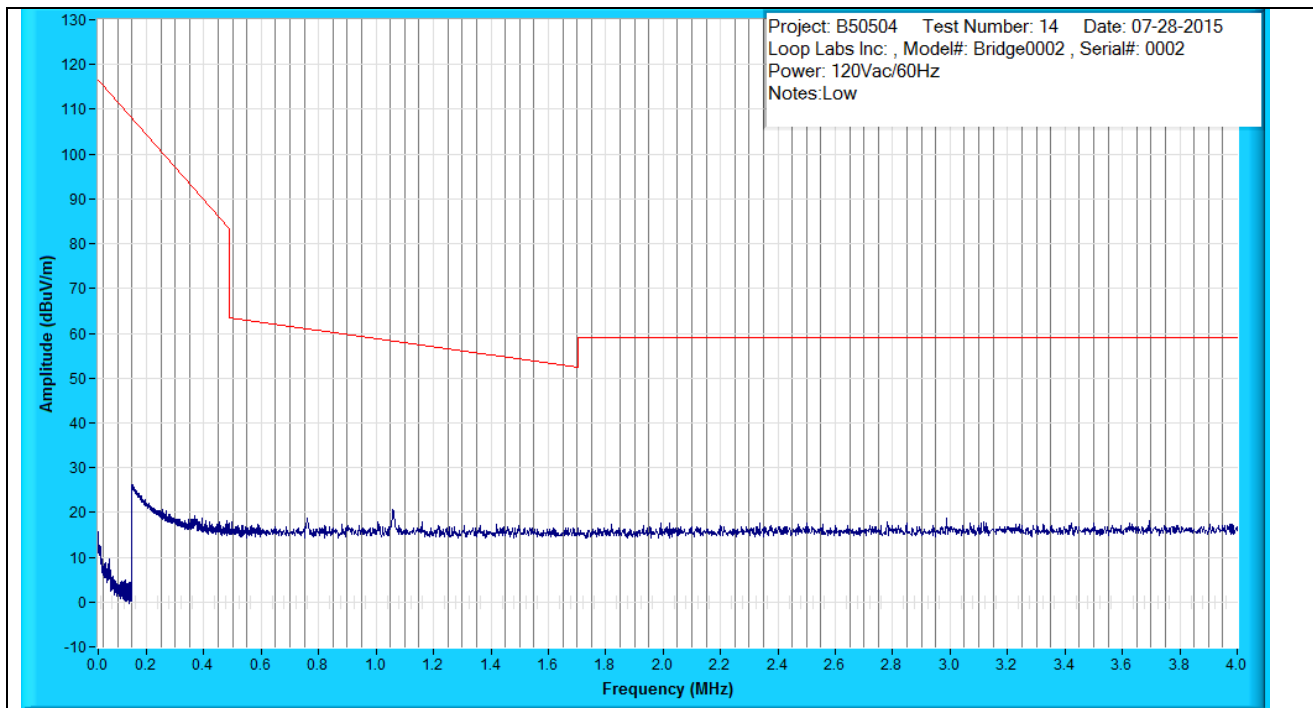
Figure A1: Radiated Emissions Prescan, 32 kHz to 4MHz, Peak Measurements at 10m Distance, LOW
