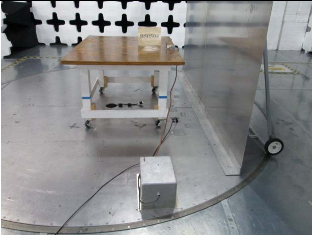
Figure B8: Conducted Emissions Test Setup - Right
