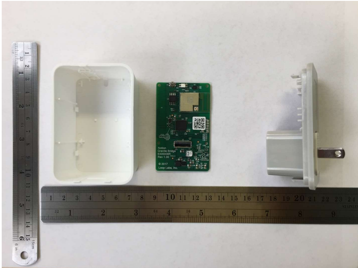
Figure 1- Disassembled View
